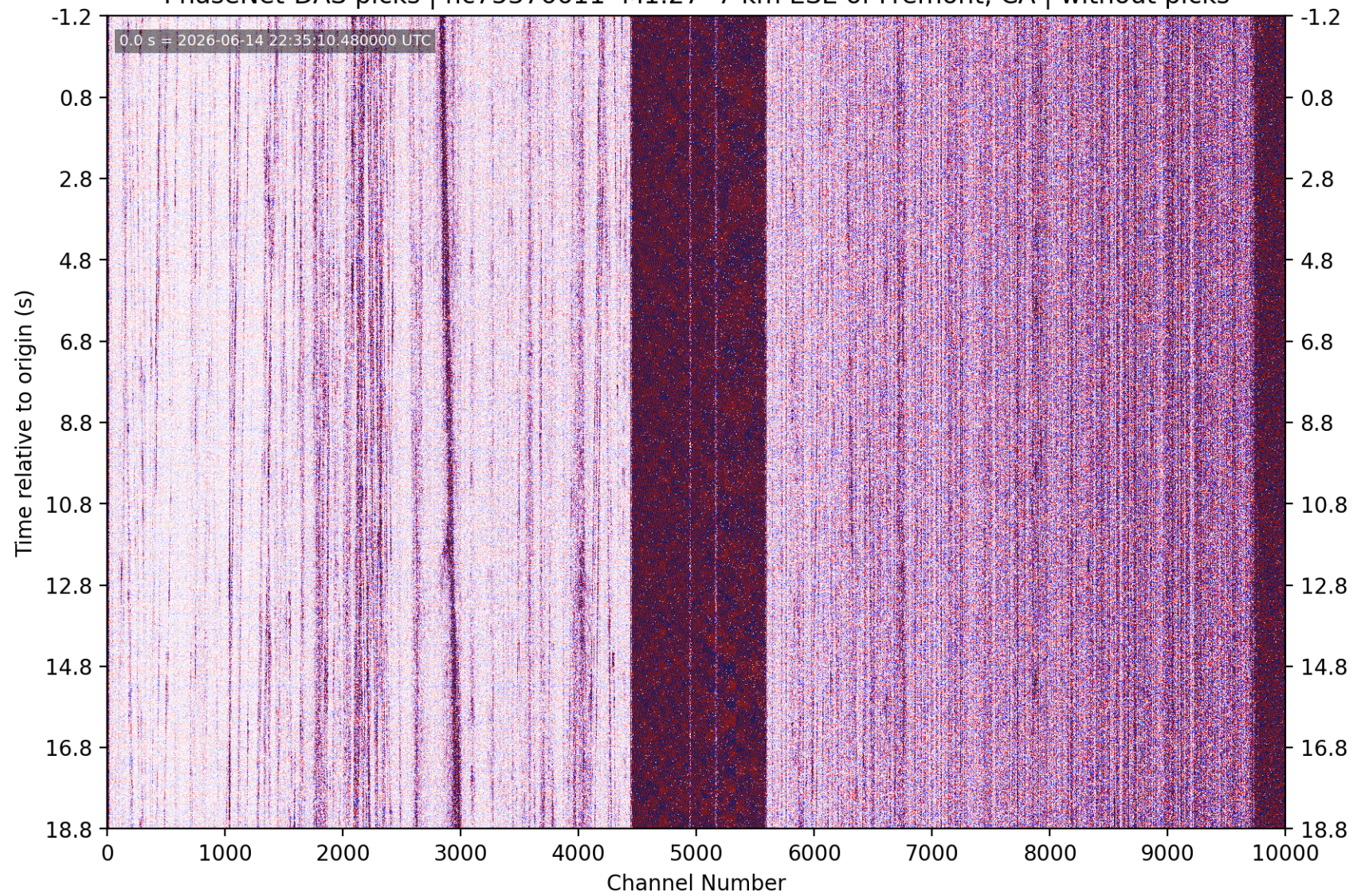
PhaseNet-DAS picks | nc75376611 M1.27 7 km ESE of Fremont, CA | without picks
