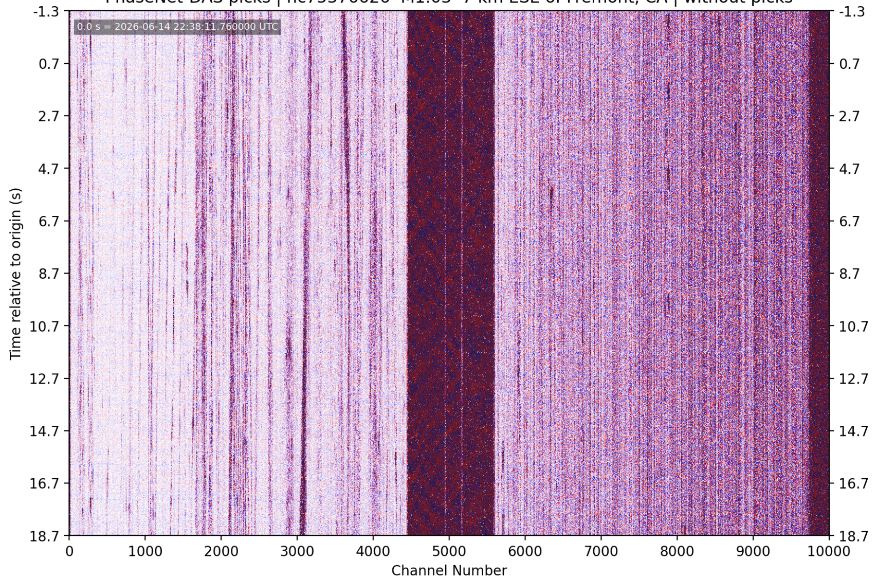
PhaseNet-DAS picks | nc75376626 M1.03 7 km ESE of Fremont, CA | without picks
