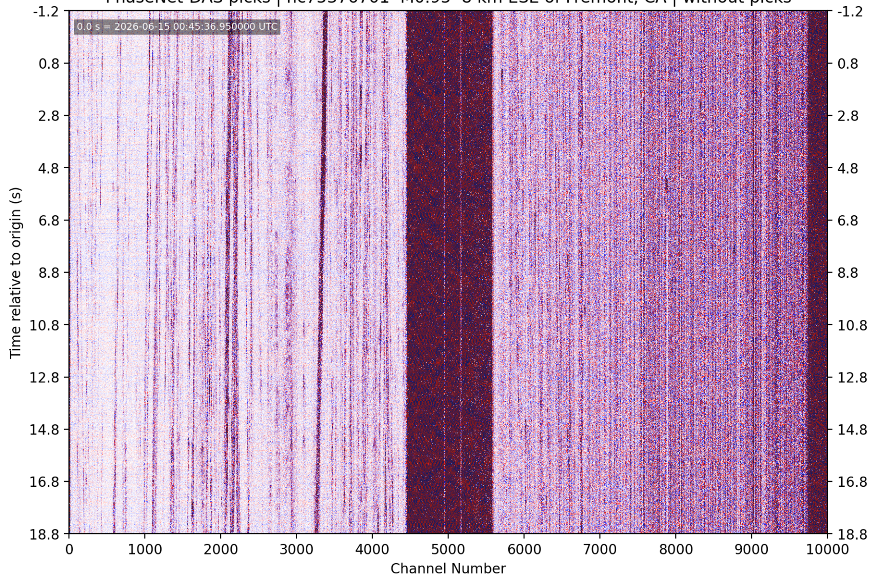
PhaseNet-DAS picks | nc75376701 M0.95 8 km ESE of Fremont, CA | without picks
