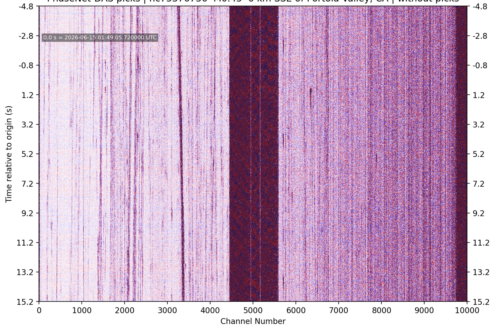
PhaseNet-DAS picks | nc75376736 M0.45 6 km SSE of Portola Valley, CA | without picks
