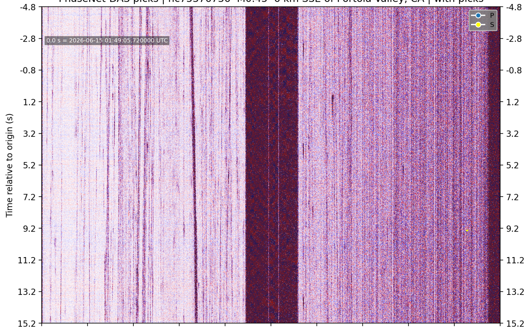
PhaseNet-DAS picks | nc75376736 M0.45 6 km SSE of Portola Valley, CA | without picks
