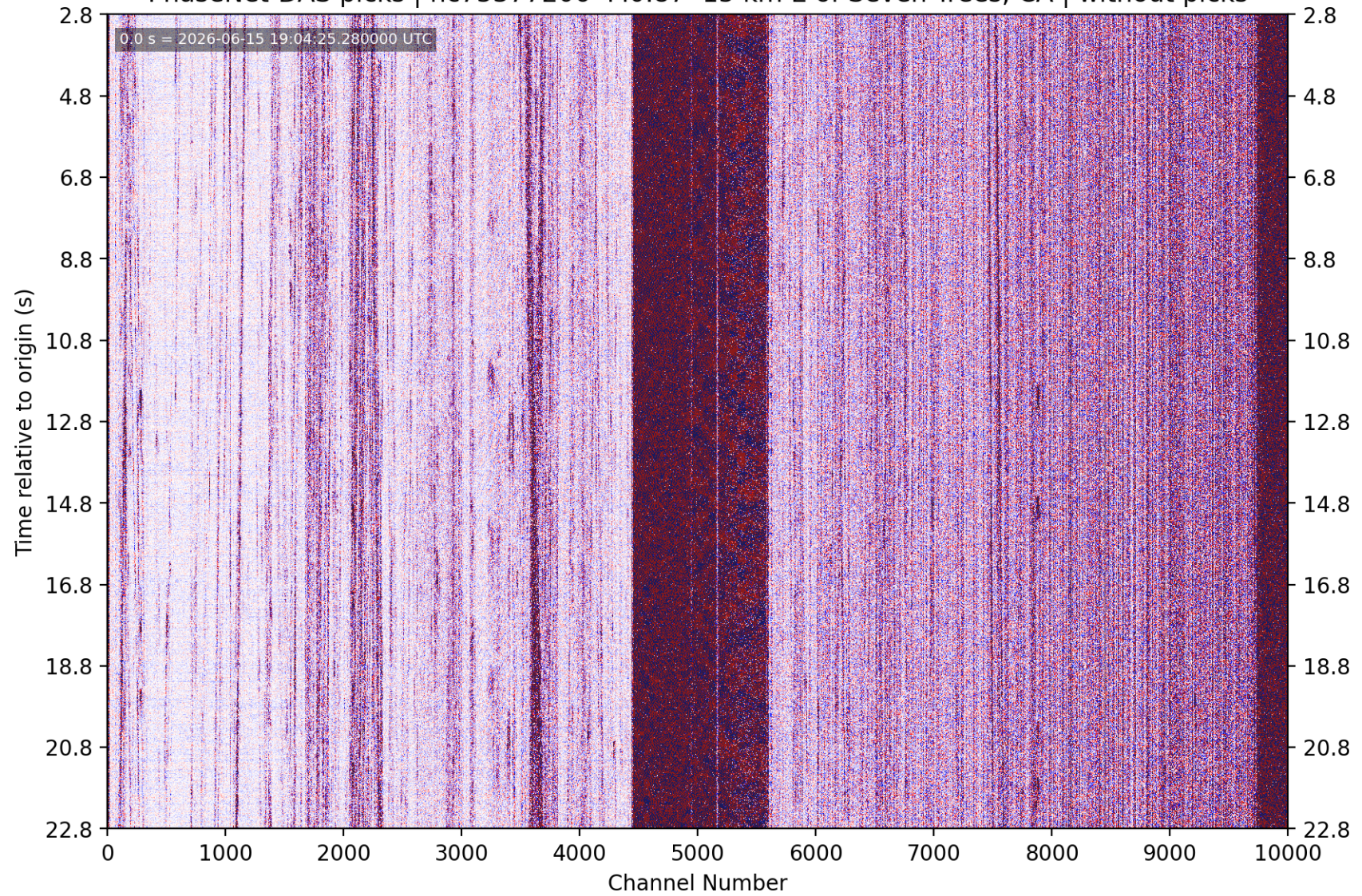
PhaseNet-DAS picks | nc75377206 M0.87 15 km E of Seven Trees, CA | without picks
