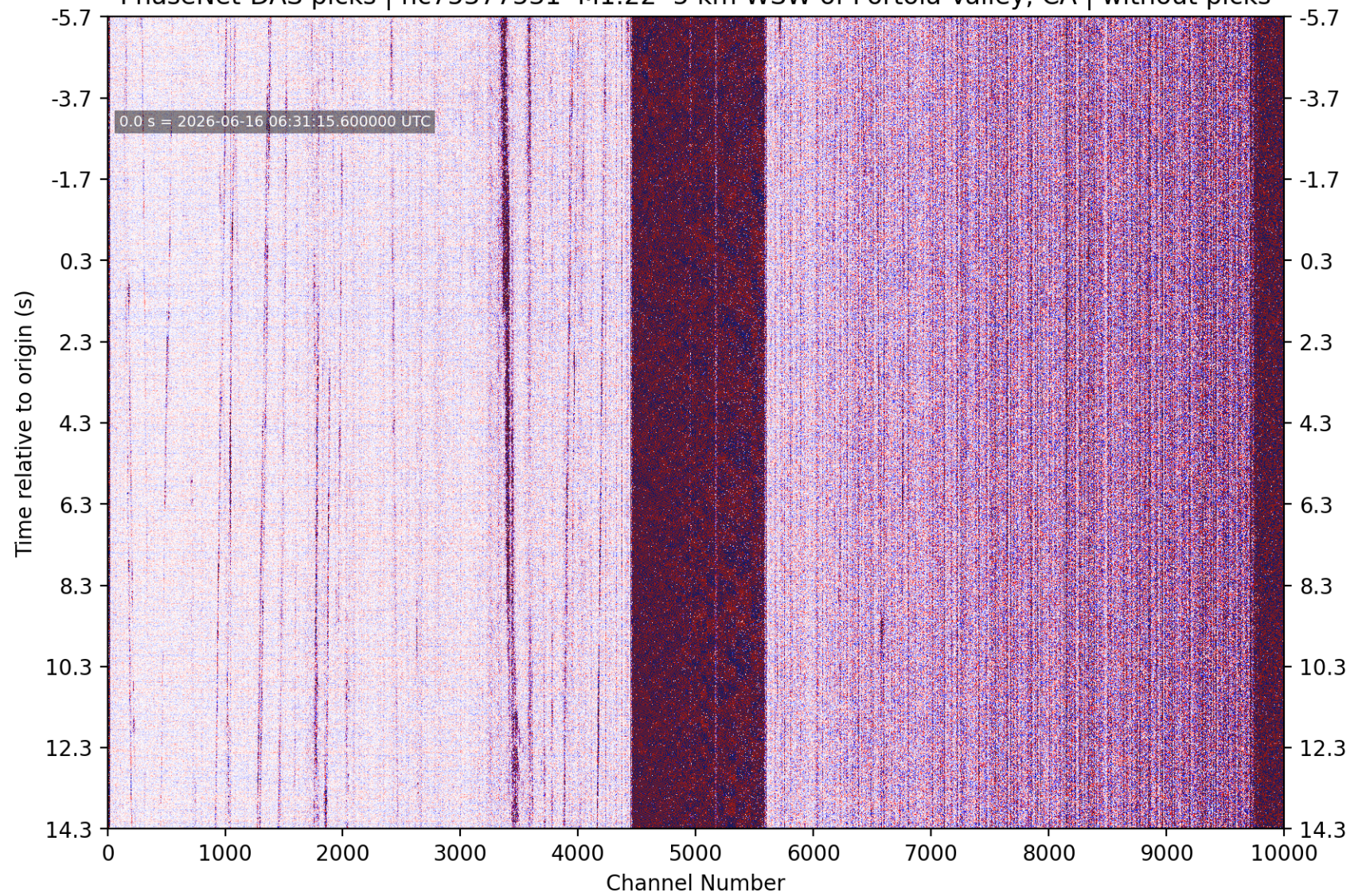
PhaseNet-DAS picks | nc75377531 M1.22 5 km WSW of Portola Valley, CA | without picks
