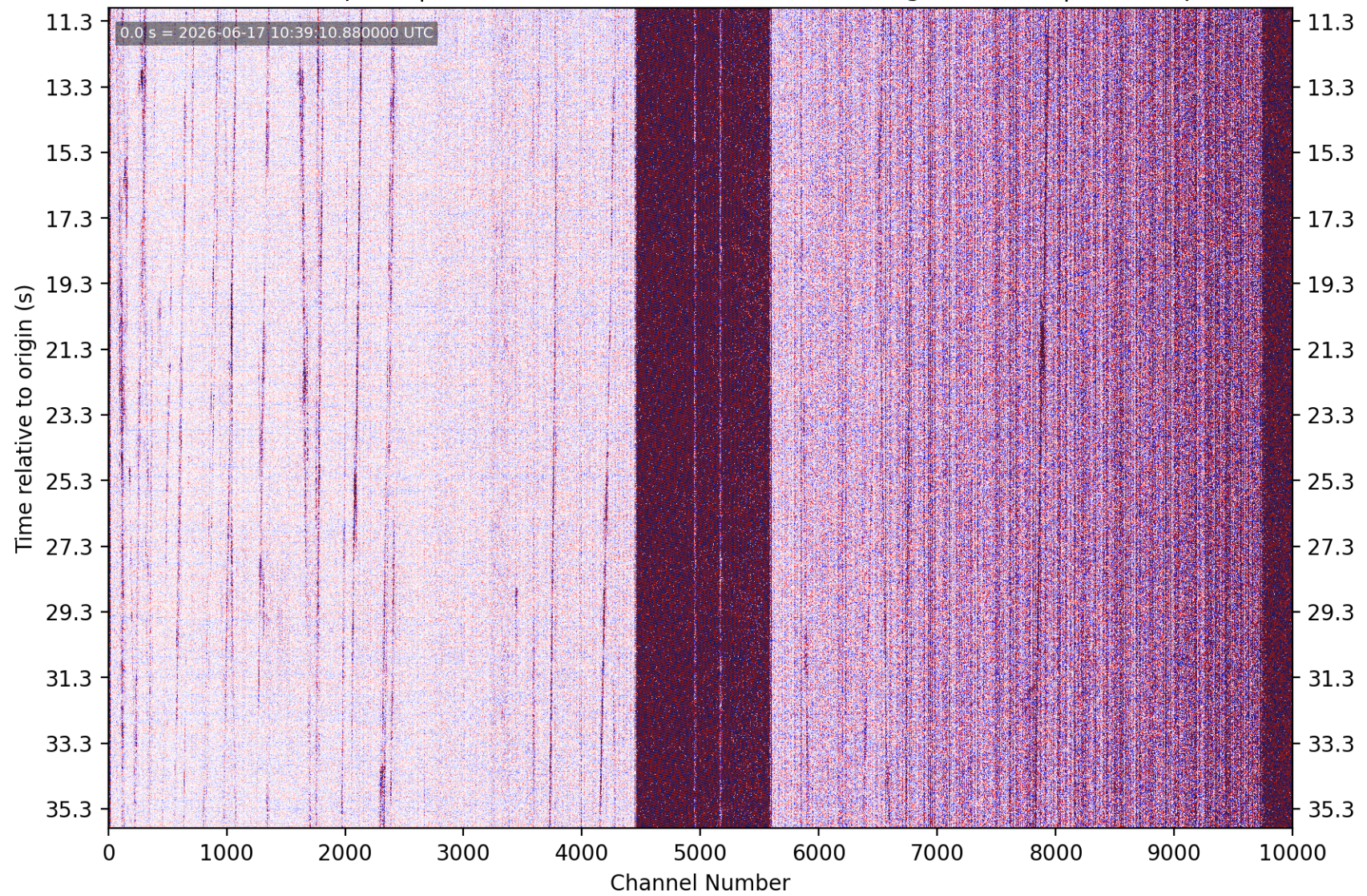
PhaseNet-DAS picks | nc75378466 M1.53 16 km N of Morgan Hill, CA | without picks
