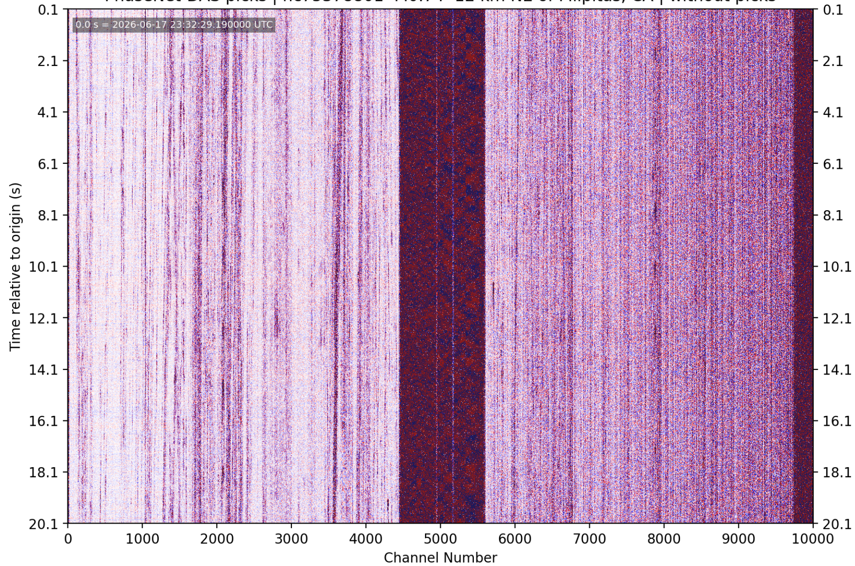
PhaseNet-DAS picks | nc75378801 M0.74 12 km NE of Milpitas, CA | without picks
