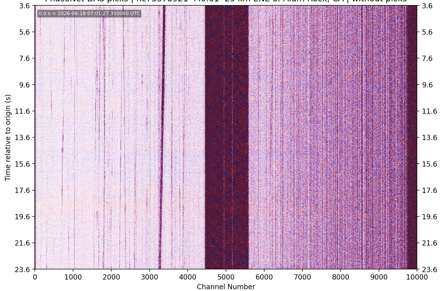
PhaseNet-DAS picks | nc75378921 M0.61 25 km ENE of Alum Rock, CA | without picks
