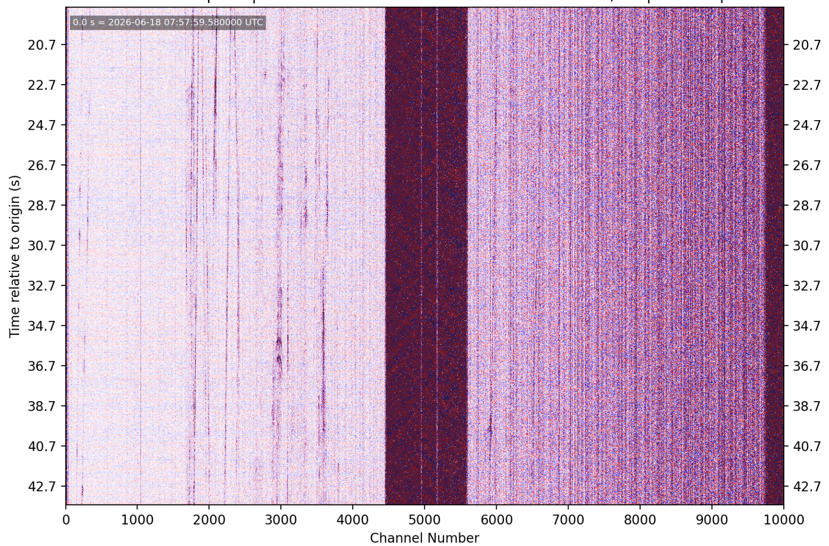
PhaseNet-DAS picks | nc75378946 M1.14 15 km E of Seven Trees, CA | without picks
