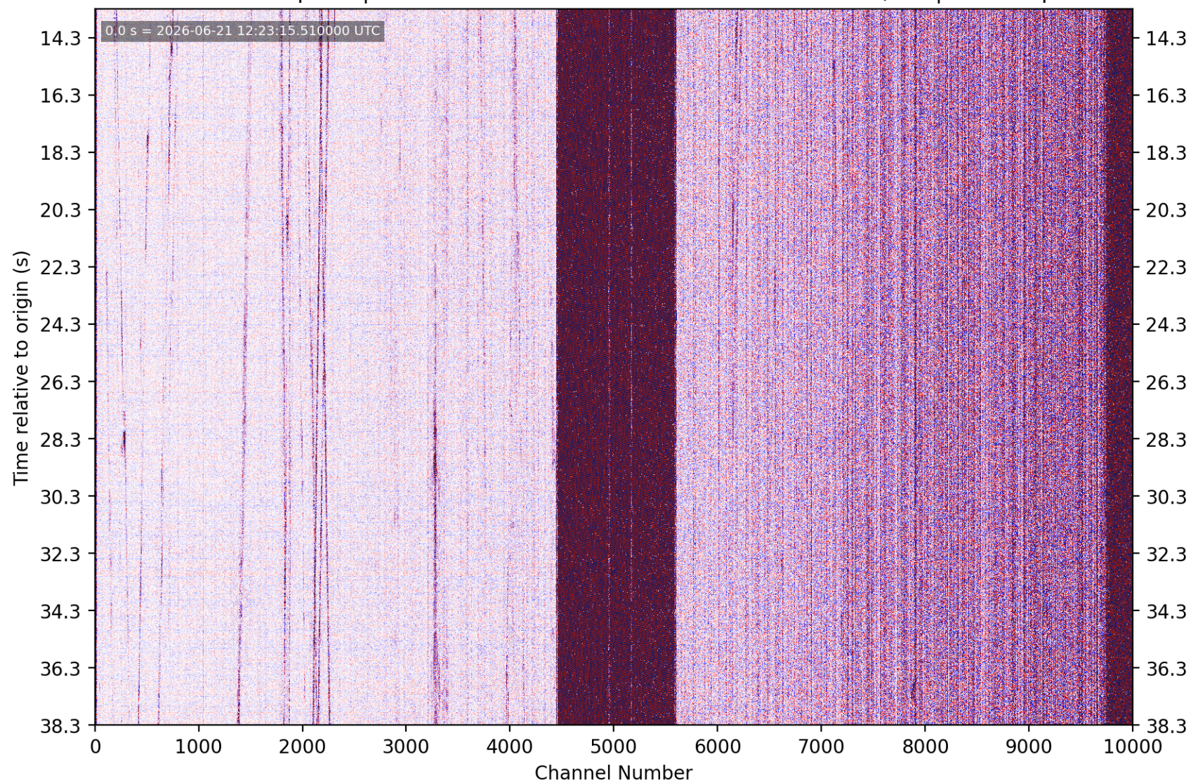
PhaseNet-DAS picks | nc75380656 M1.35 9 km ENE of San Martin, CA | without picks
