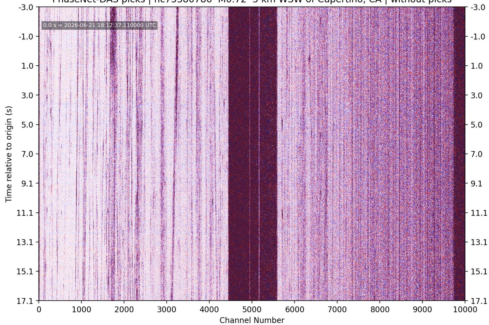
PhaseNet-DAS picks | nc75380786 M0.72 5 km WSW of Cupertino, CA | without picks
