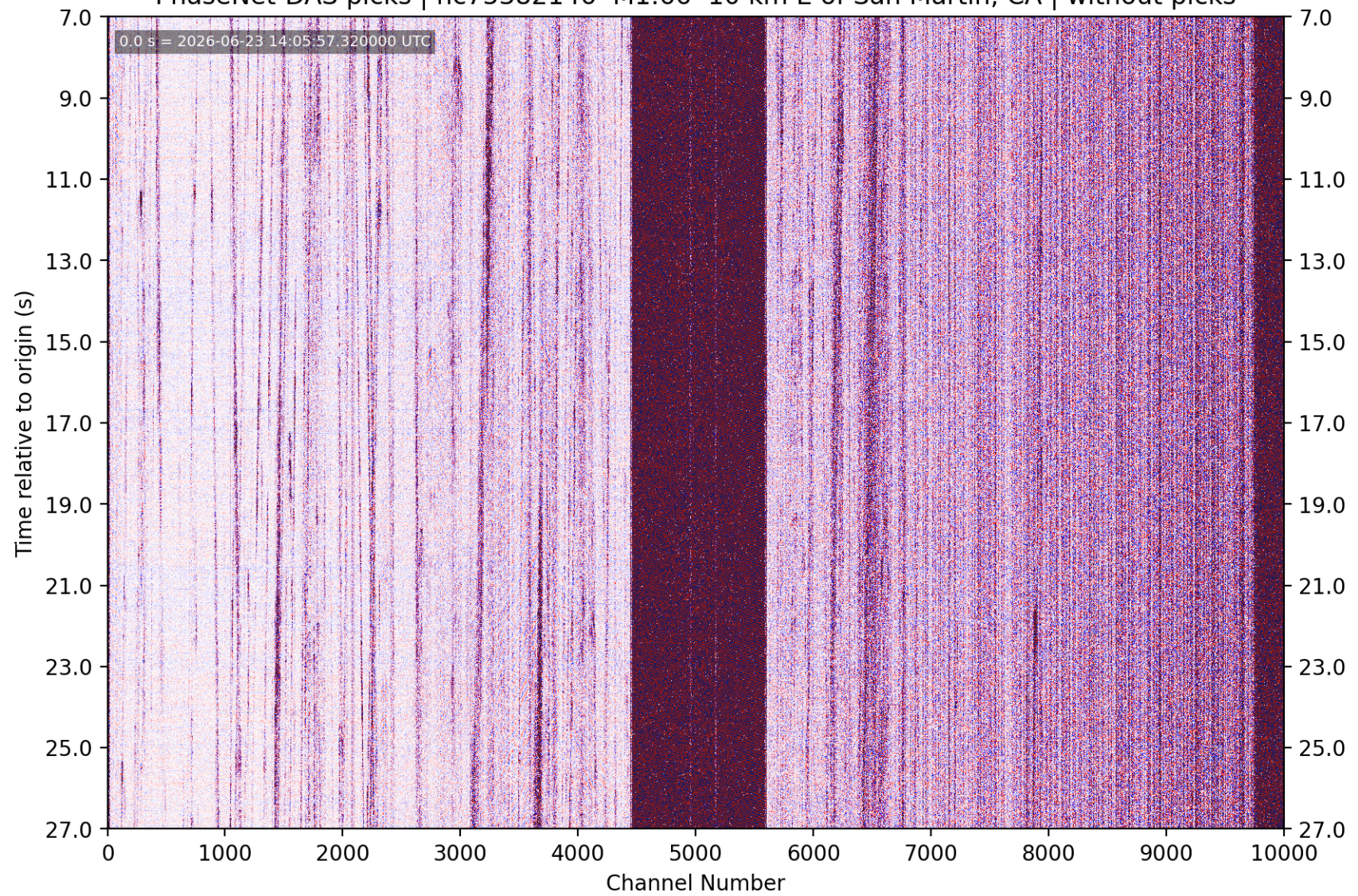
PhaseNet-DAS picks | nc75382146 M1.66 10 km E of San Martin, CA | without picks
