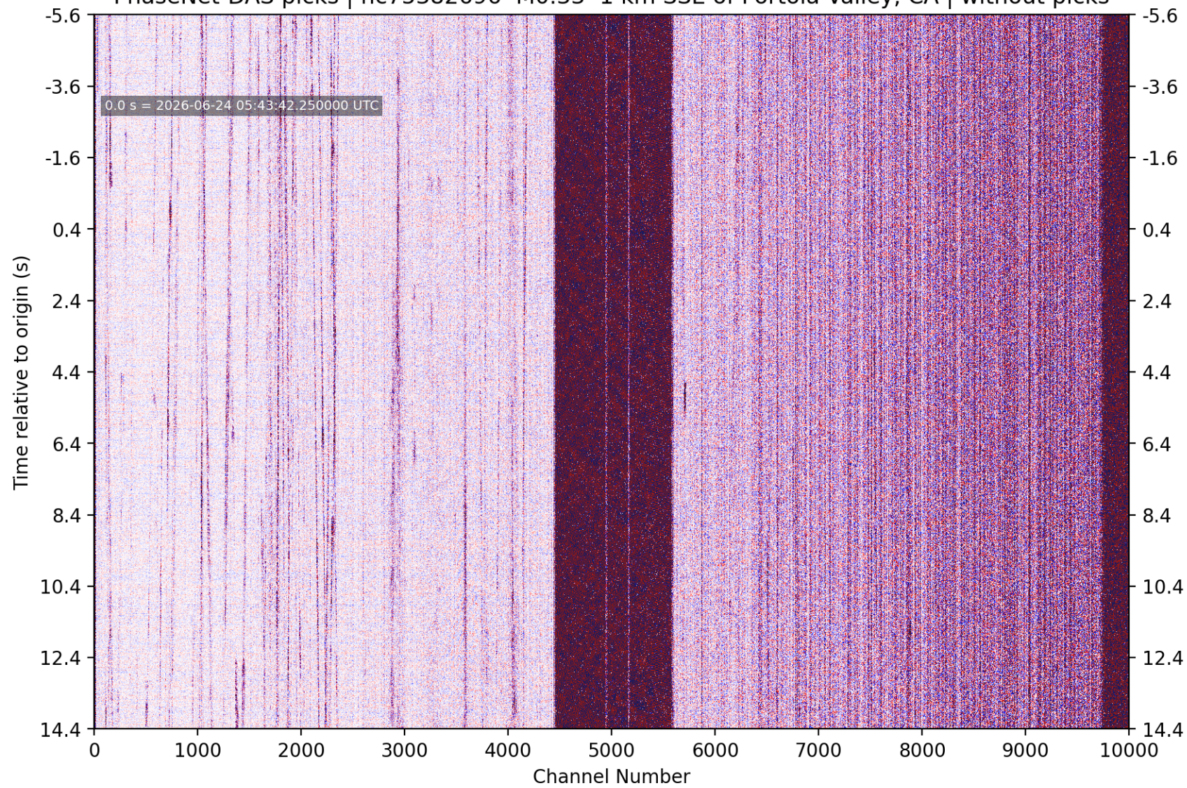
PhaseNet-DAS picks | nc75382696 M0.33 1 km SSE of Portola Valley, CA | without picks
