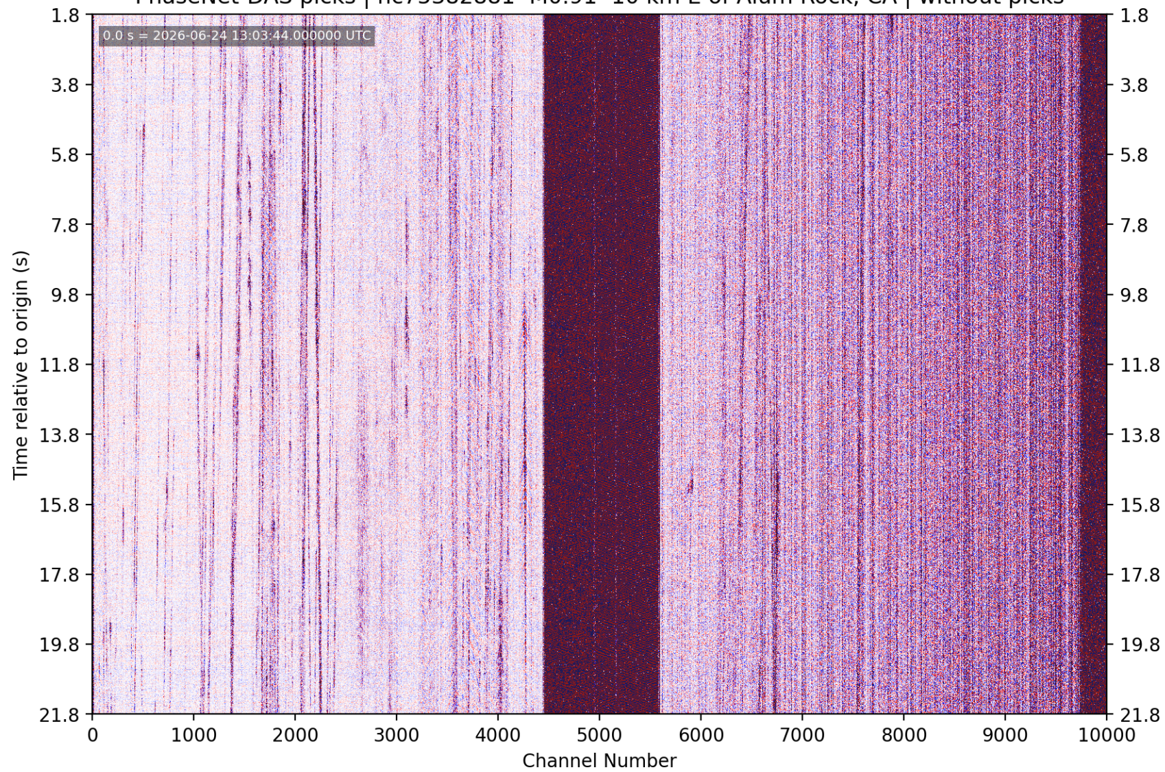
PhaseNet-DAS picks | nc75382881 M0.91 10 km E of Alum Rock, CA | without picks
