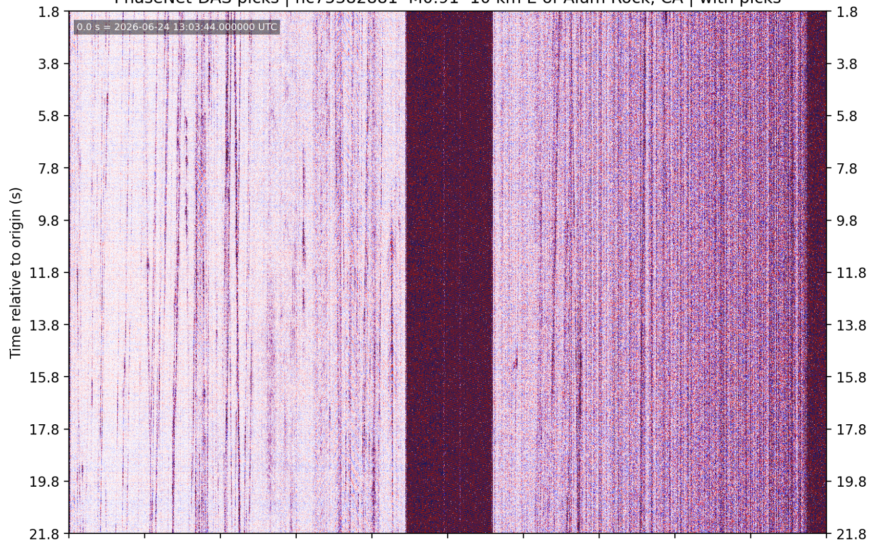
PhaseNet-DAS picks | nc75382881 M0.91 10 km E of Alum Rock, CA | without picks
