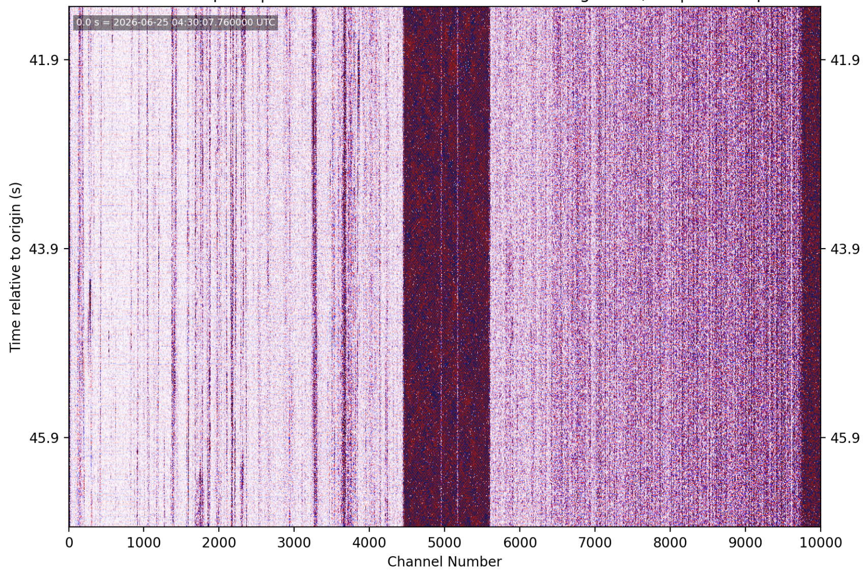
PhaseNet-DAS picks | nc75383711 M1.09 19 km NE of Morgan Hill, CA | without picks
