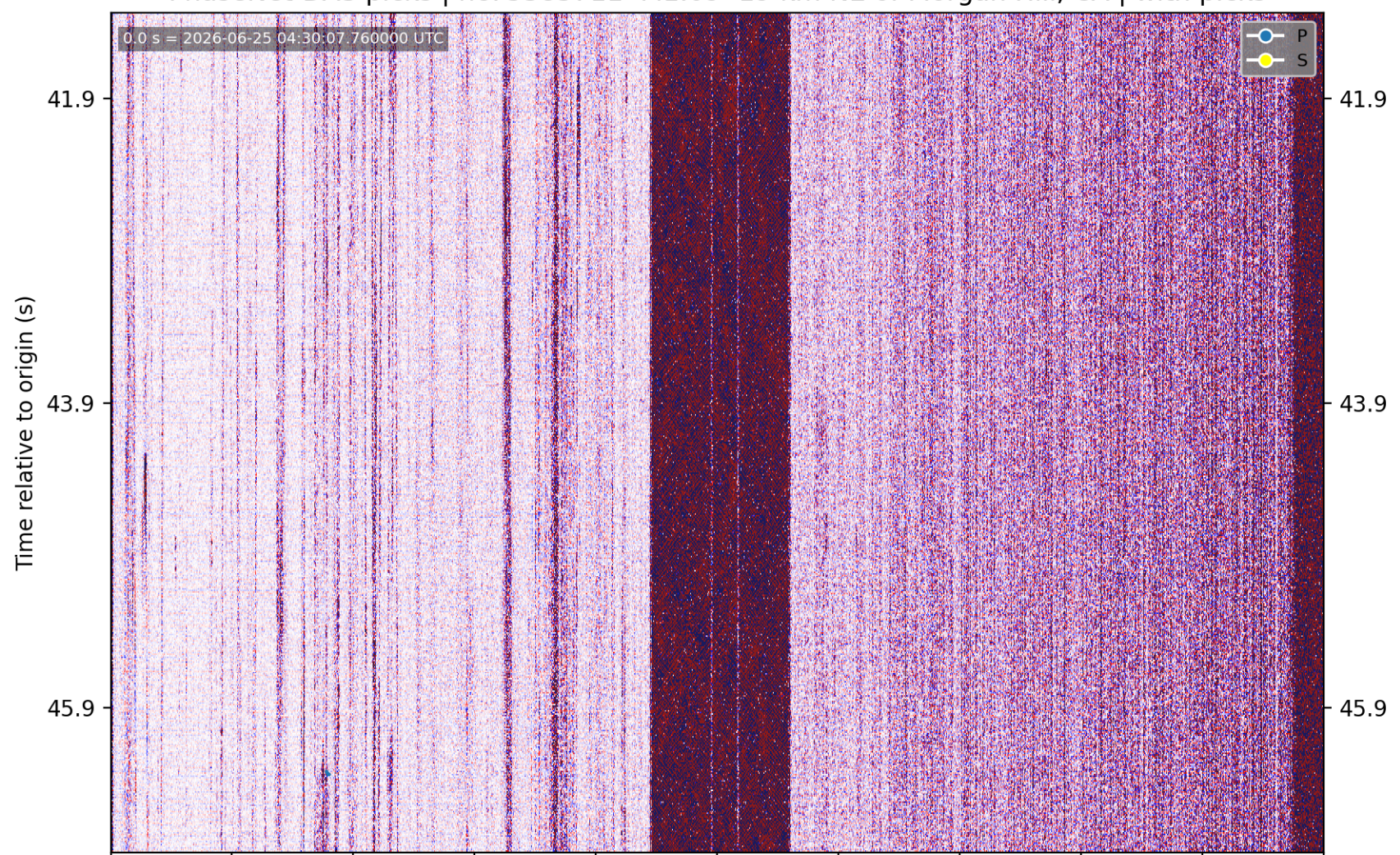
PhaseNet-DAS picks | nc75383711 M1.09 19 km NE of Morgan Hill, CA | without picks
