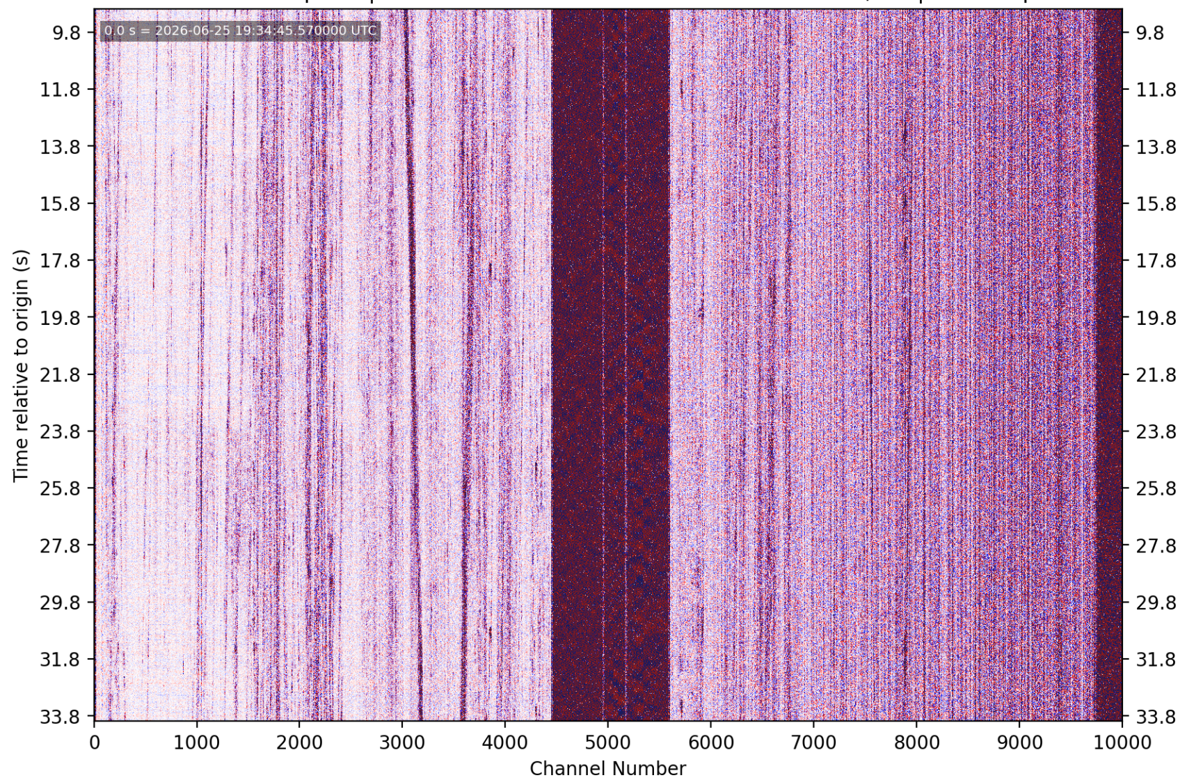
PhaseNet-DAS picks | nc75384271 M1.95 10 km E of Alum Rock, CA | without picks
