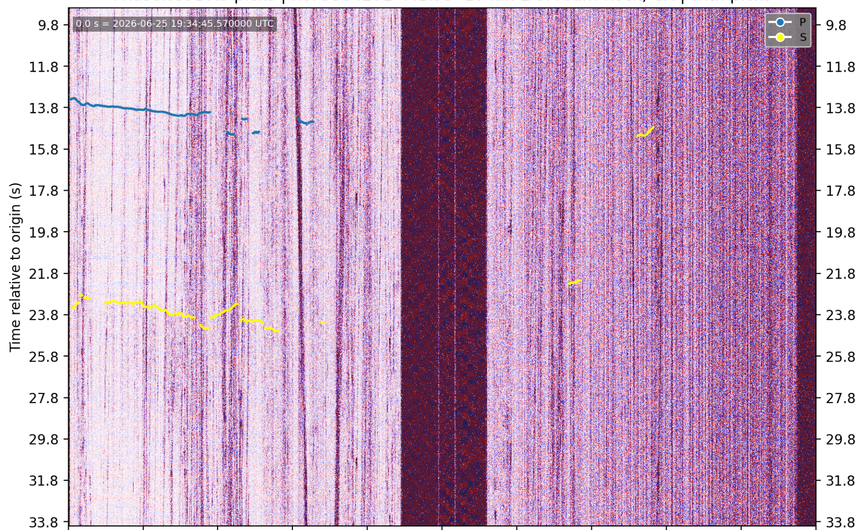
PhaseNet-DAS picks | nc75384271 M1.95 10 km E of Alum Rock, CA | without picks
