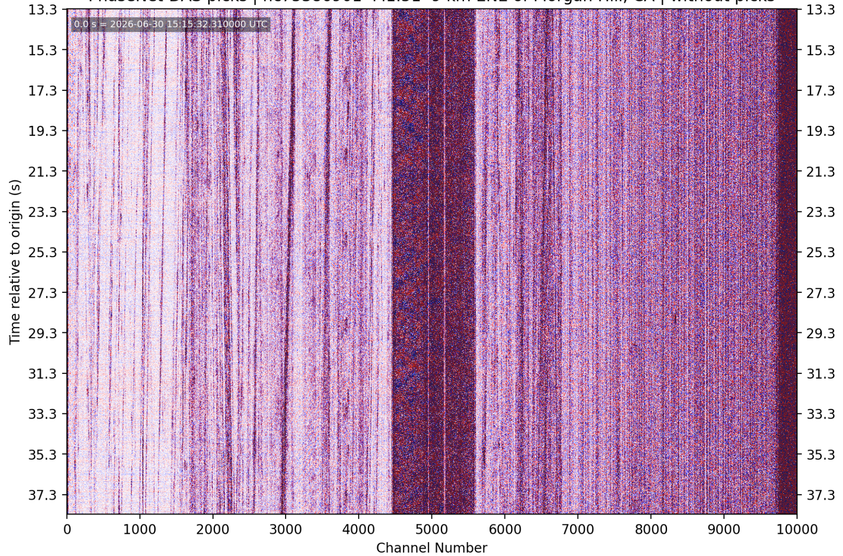
PhaseNet-DAS picks | nc75386901 M1.51 9 km ENE of Morgan Hill, CA | without picks
