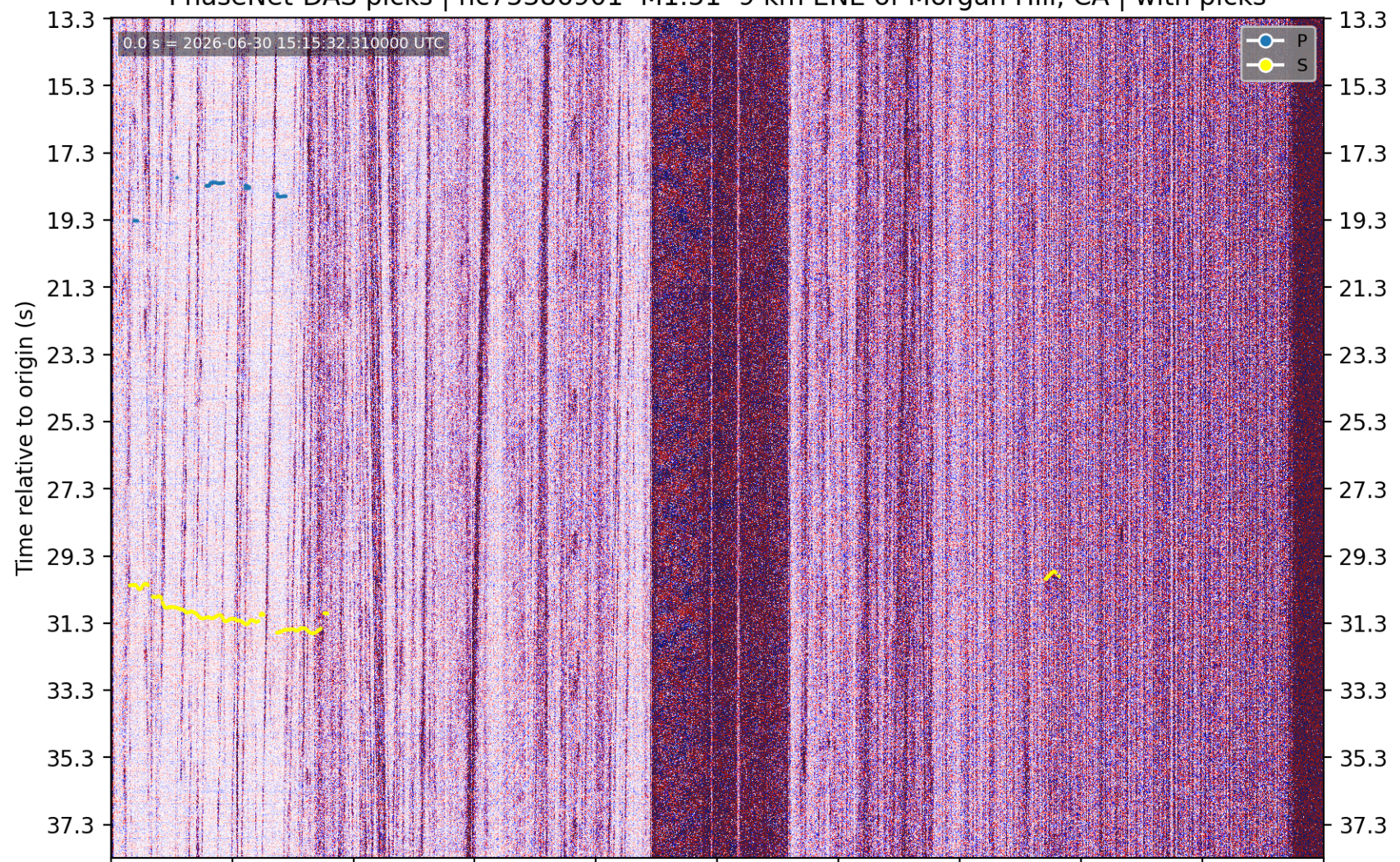
PhaseNet-DAS picks | nc75386901 M1.51 9 km ENE of Morgan Hill, CA | without picks
