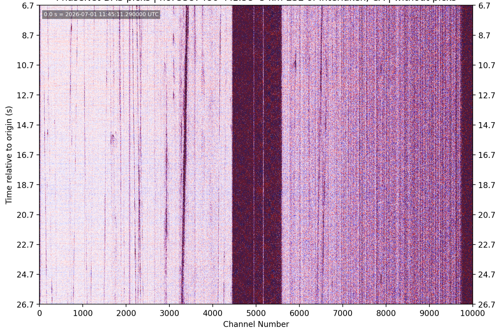
PhaseNet-DAS picks | nc75387486 M1.58 5 km ESE of Interlaken, CA | without picks
