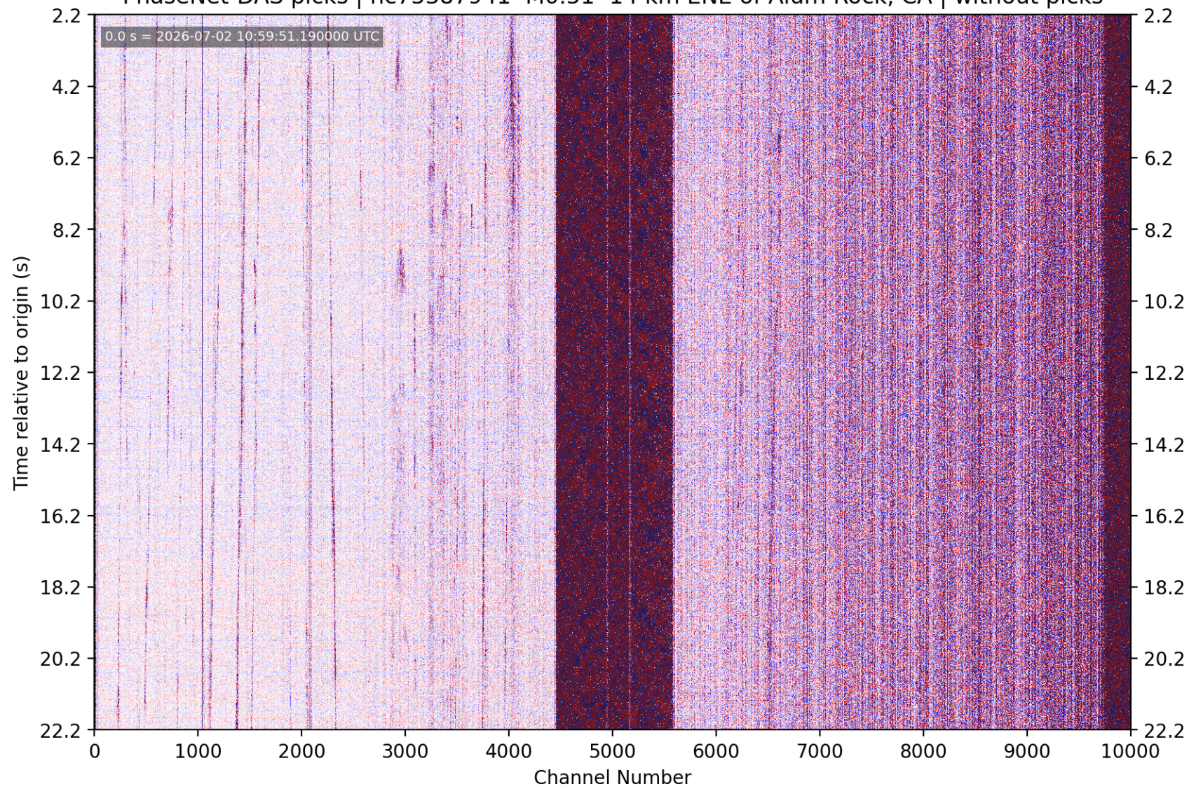
PhaseNet-DAS picks | nc75387941 M0.51 14 km ENE of Alum Rock, CA | without picks
