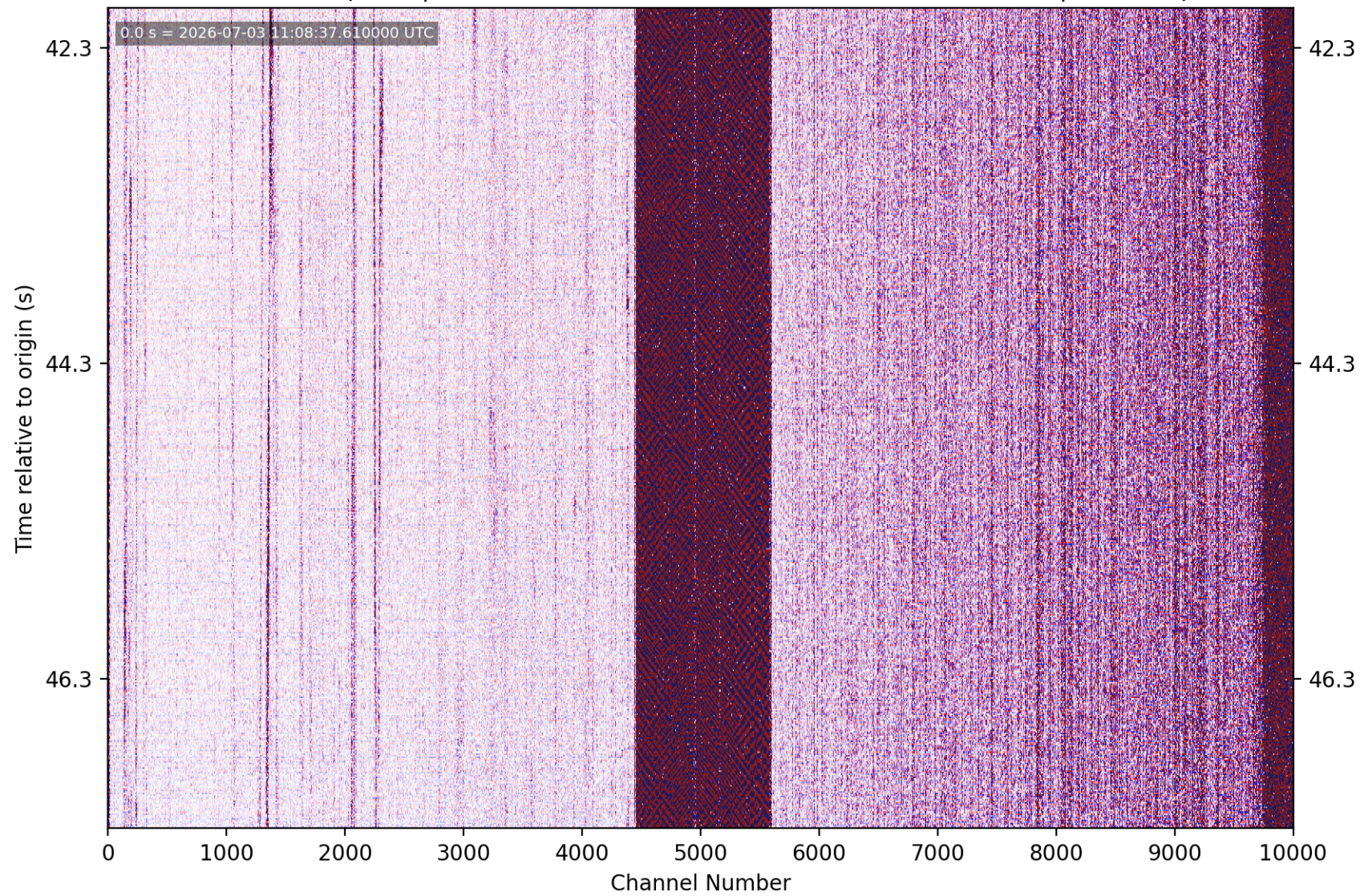
PhaseNet-DAS picks | nc75388531 M1.0 9 km ENE of San Martin, CA | without picks
