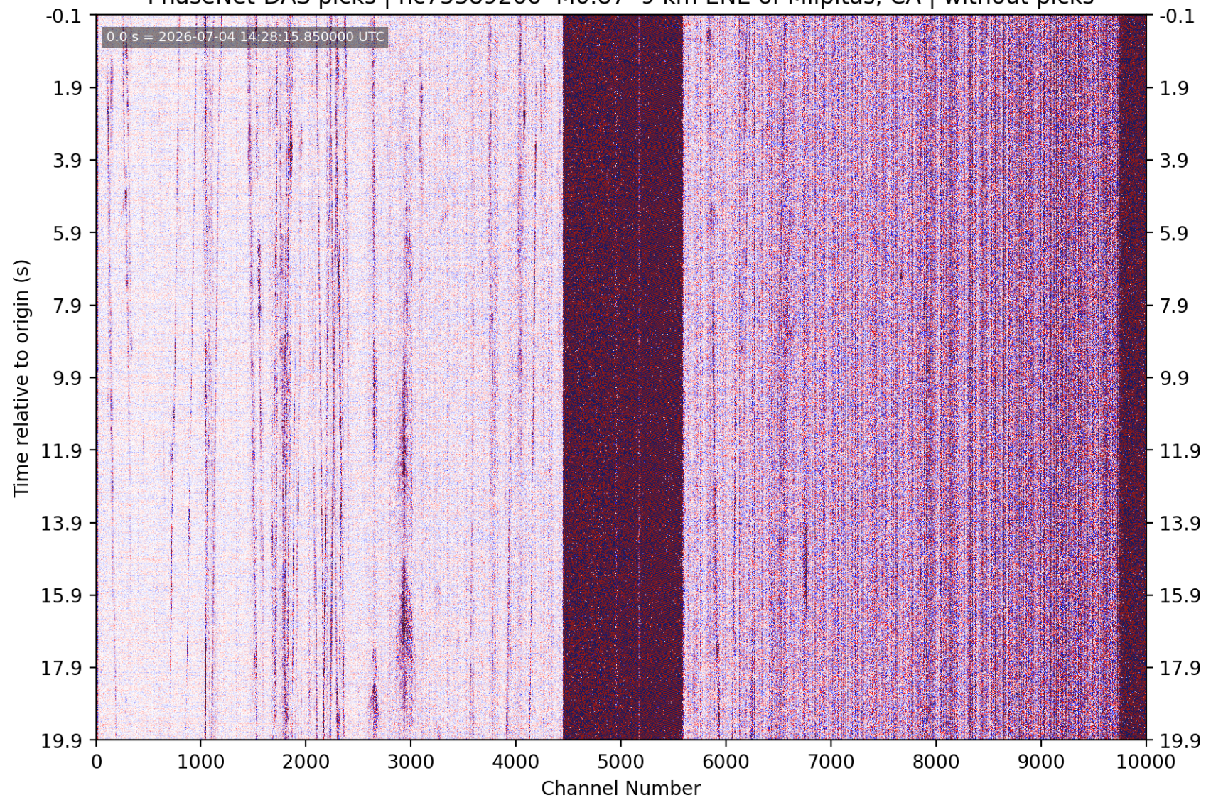
PhaseNet-DAS picks | nc75389266 M0.87 9 km ENE of Milpitas, CA | without picks
