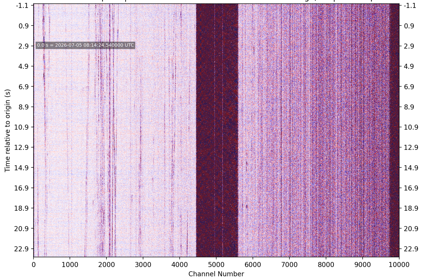
PhaseNet-DAS picks | nc75389906 M0.7 4 km WSW of Hillsborough, CA | without picks
