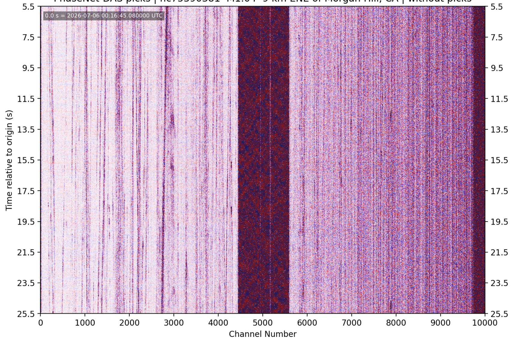
PhaseNet-DAS picks | nc75390381 M1.04 9 km ENE of Morgan Hill, CA | without picks
