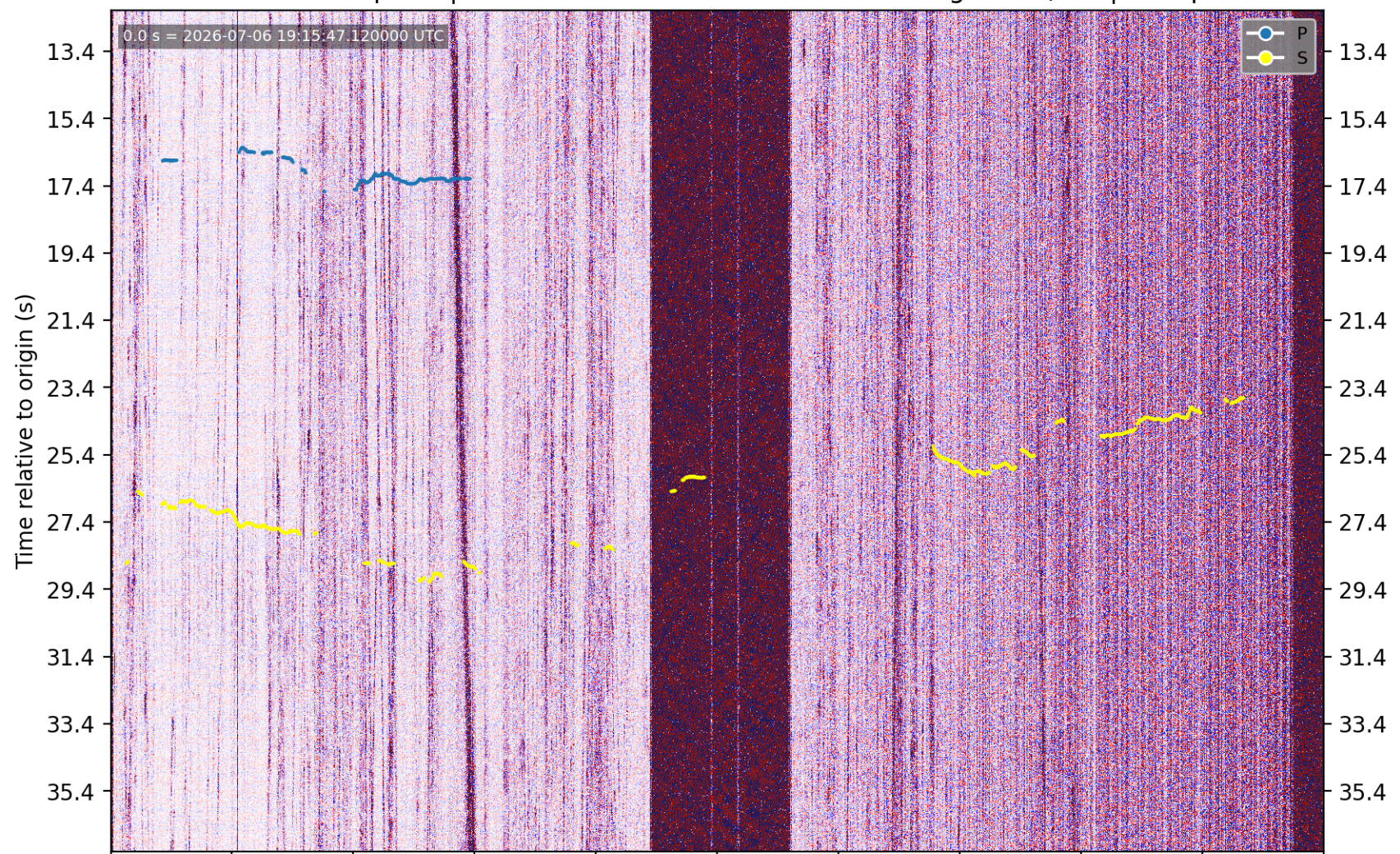
PhaseNet-DAS picks | nc75390856 M2.12 15 km N of Morgan Hill, CA | without picks
