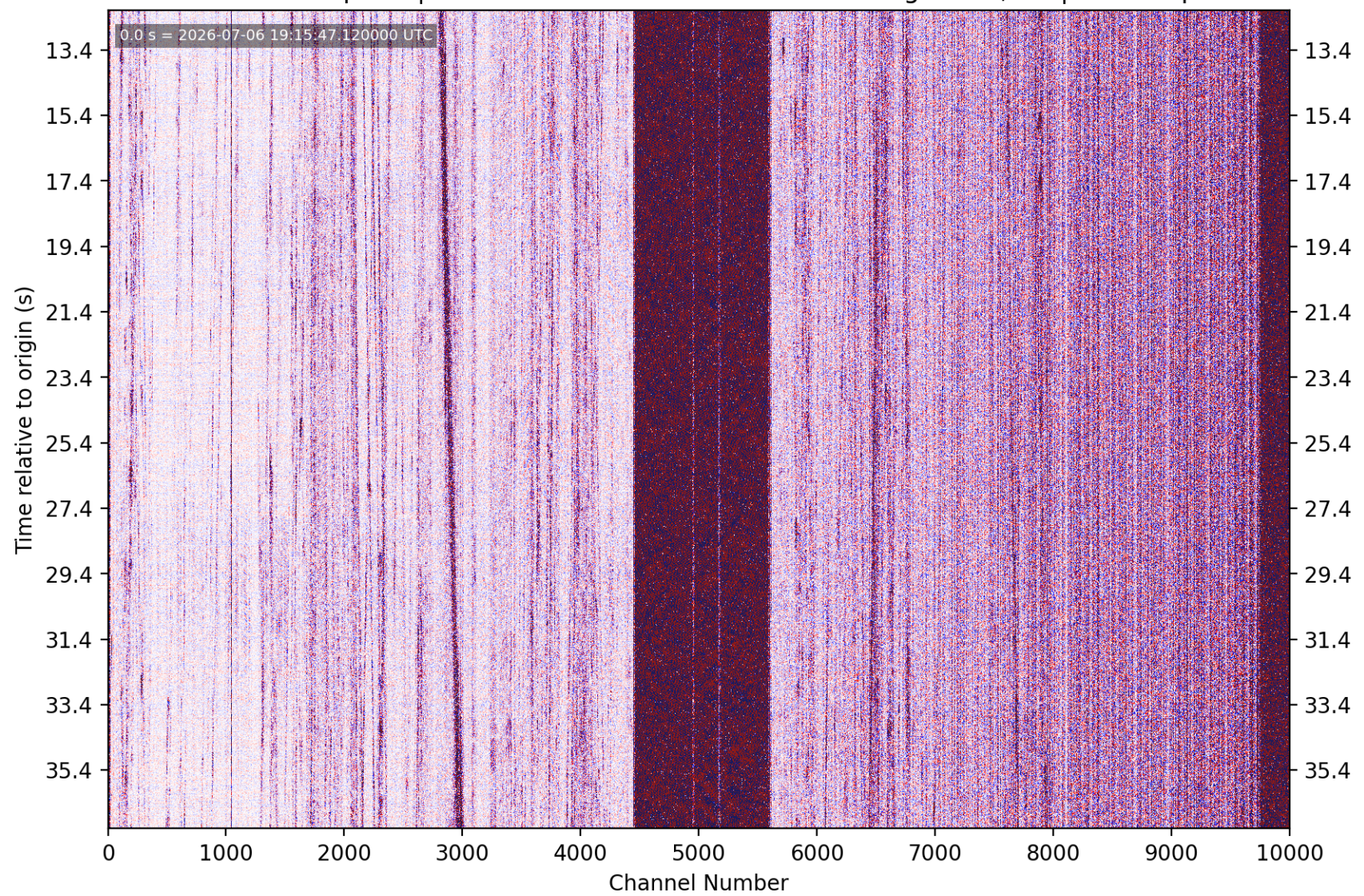
PhaseNet-DAS picks | nc75390856 M2.12 15 km N of Morgan Hill, CA | without picks
