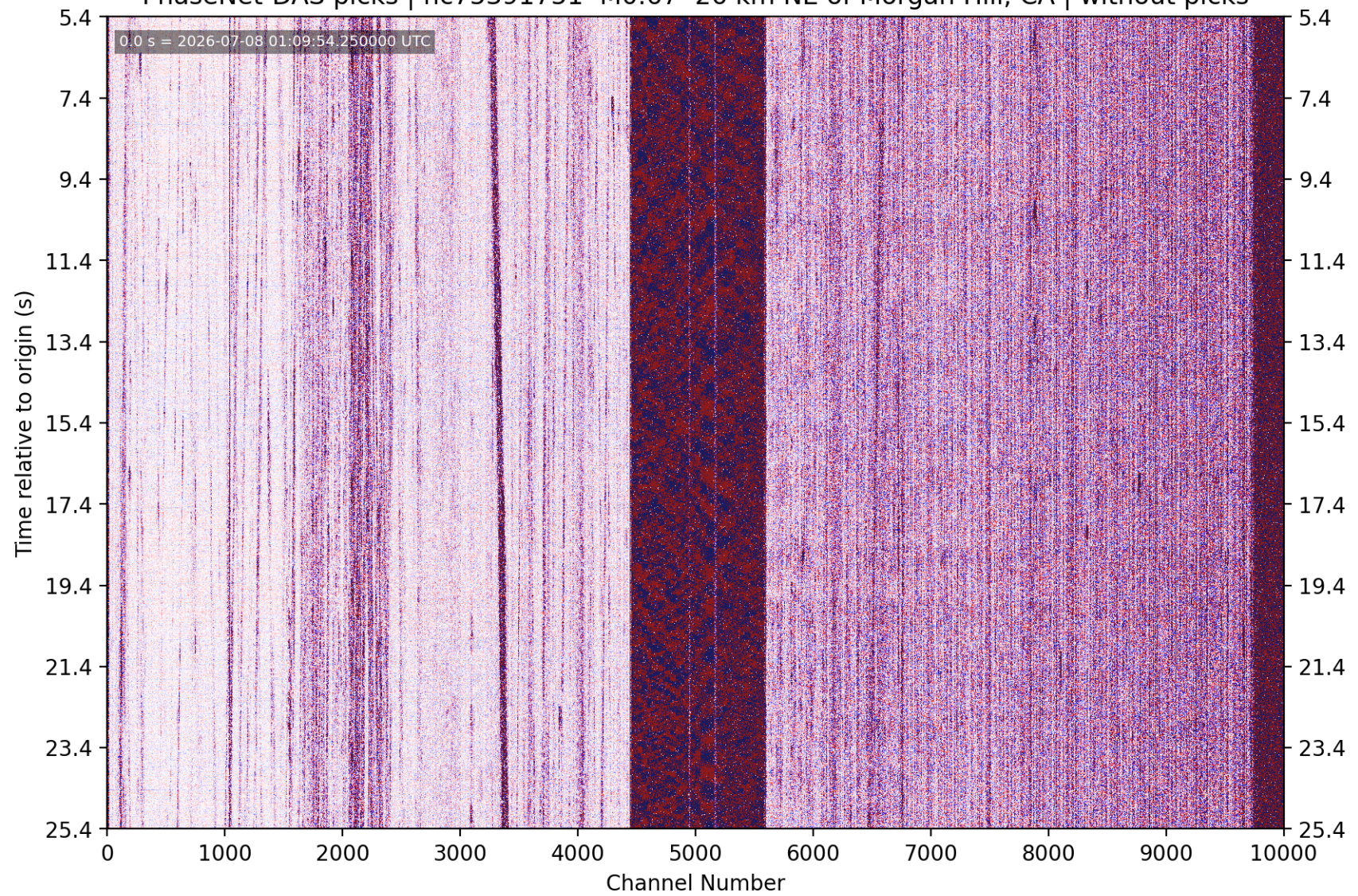
PhaseNet-DAS picks | nc75391751 M0.67 26 km NE of Morgan Hill, CA | without picks
