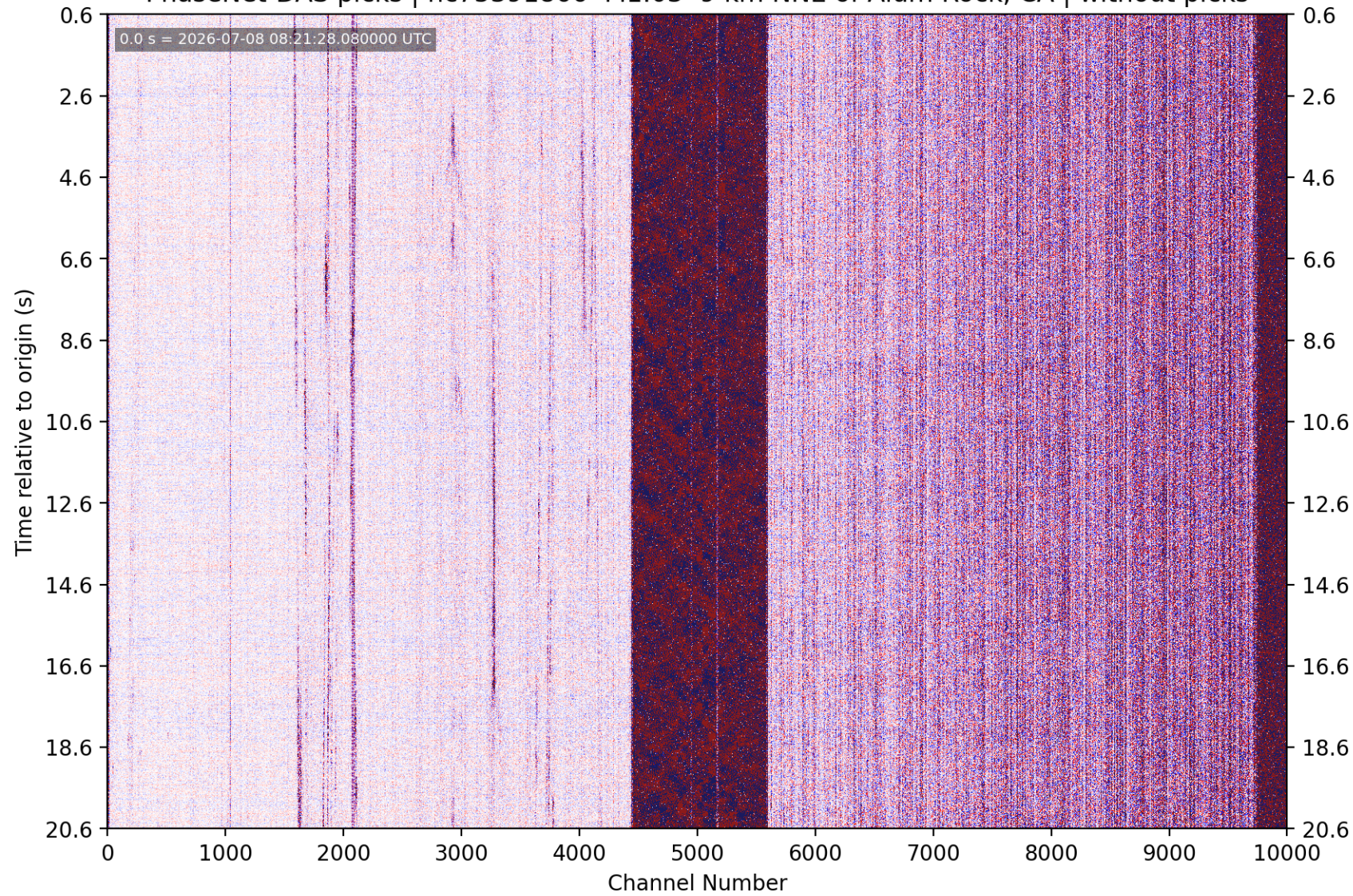
PhaseNet-DAS picks | nc75391866 M1.03 9 km NNE of Alum Rock, CA | without picks
