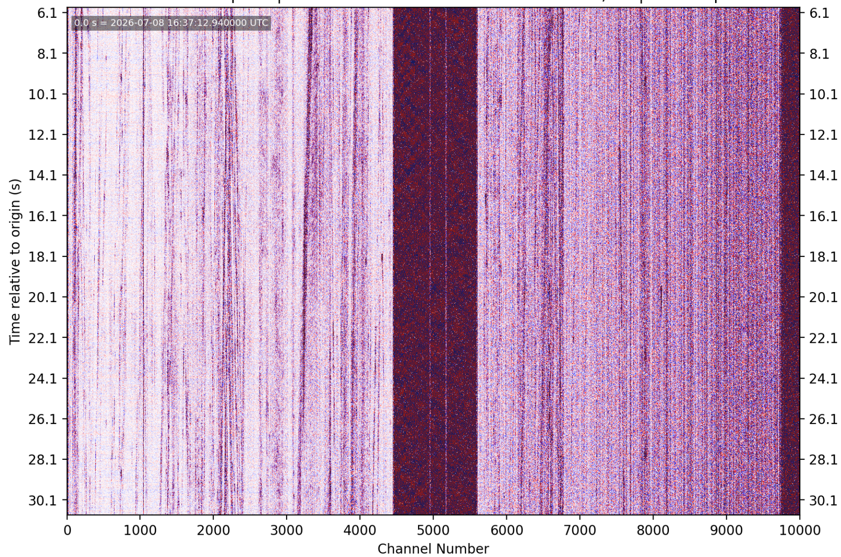
PhaseNet-DAS picks | nc75392071 M2.05 12 km SE of Sunol, CA | without picks
