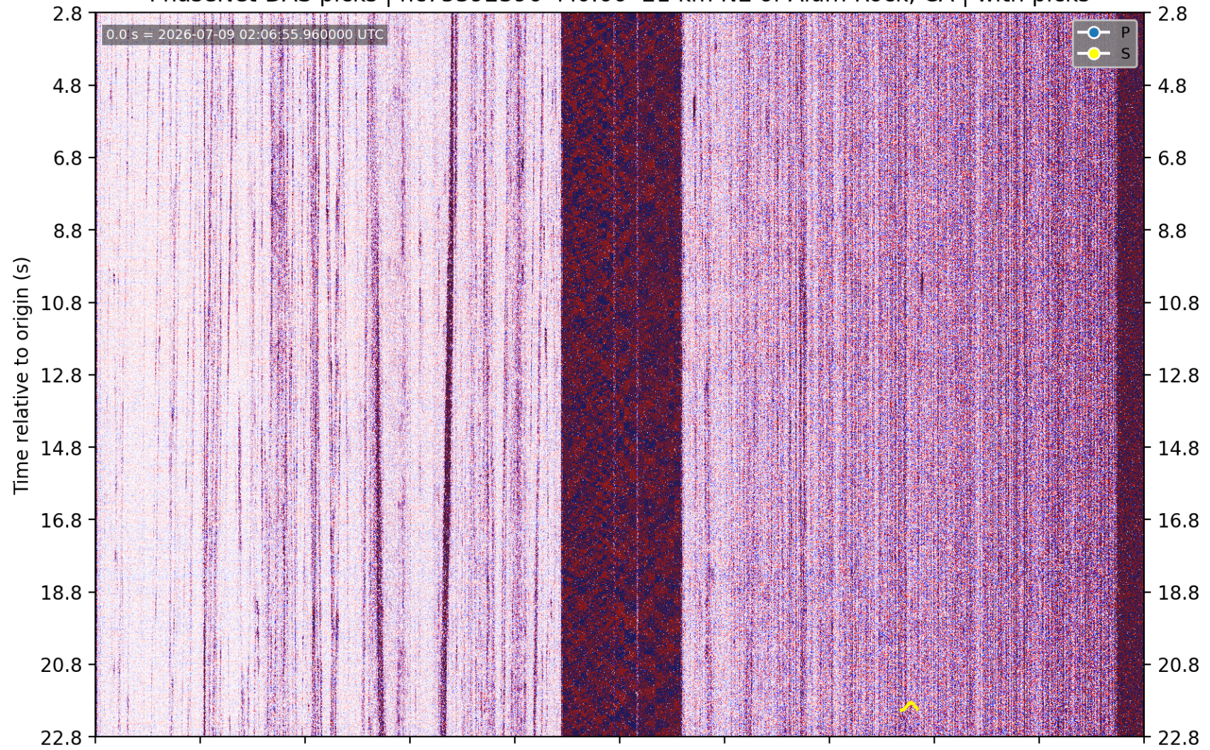
PhaseNet-DAS picks | nc75392396 M0.66 21 km NE of Alum Rock, CA | without picks
