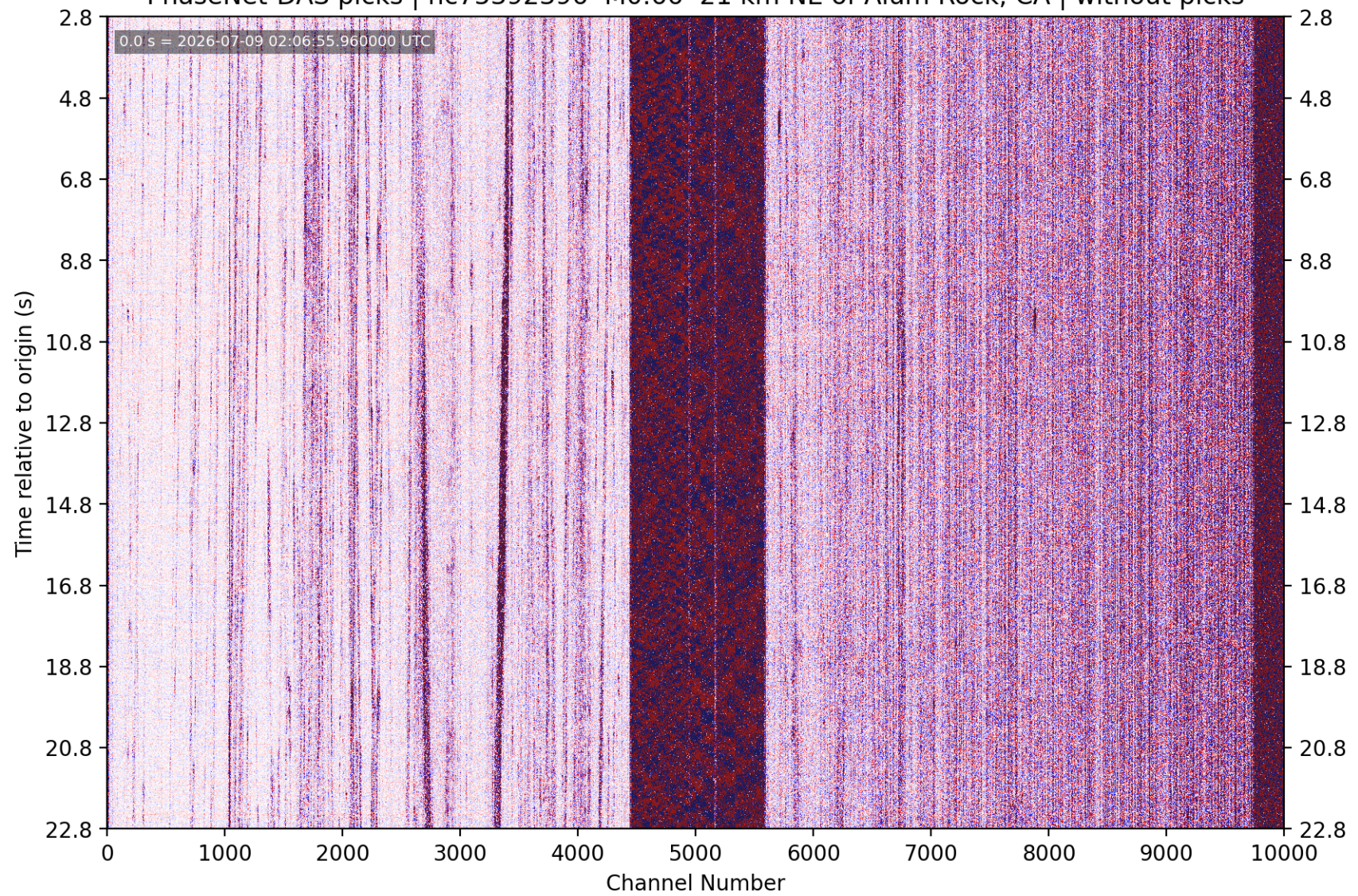
PhaseNet-DAS picks | nc75392396 M0.66 21 km NE of Alum Rock, CA | without picks
