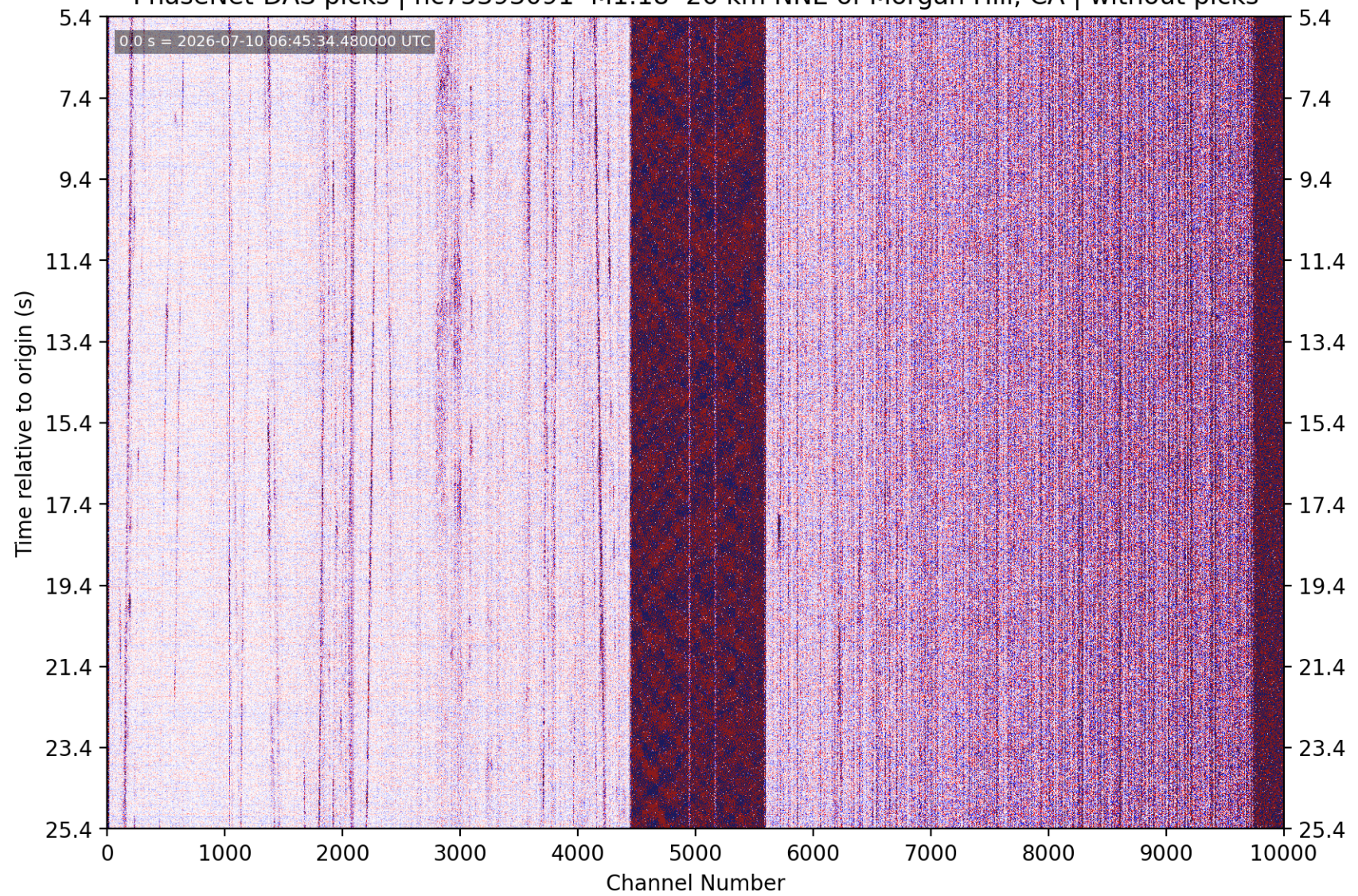
PhaseNet-DAS picks | nc75393091 M1.18 26 km NNE of Morgan Hill, CA | without picks
