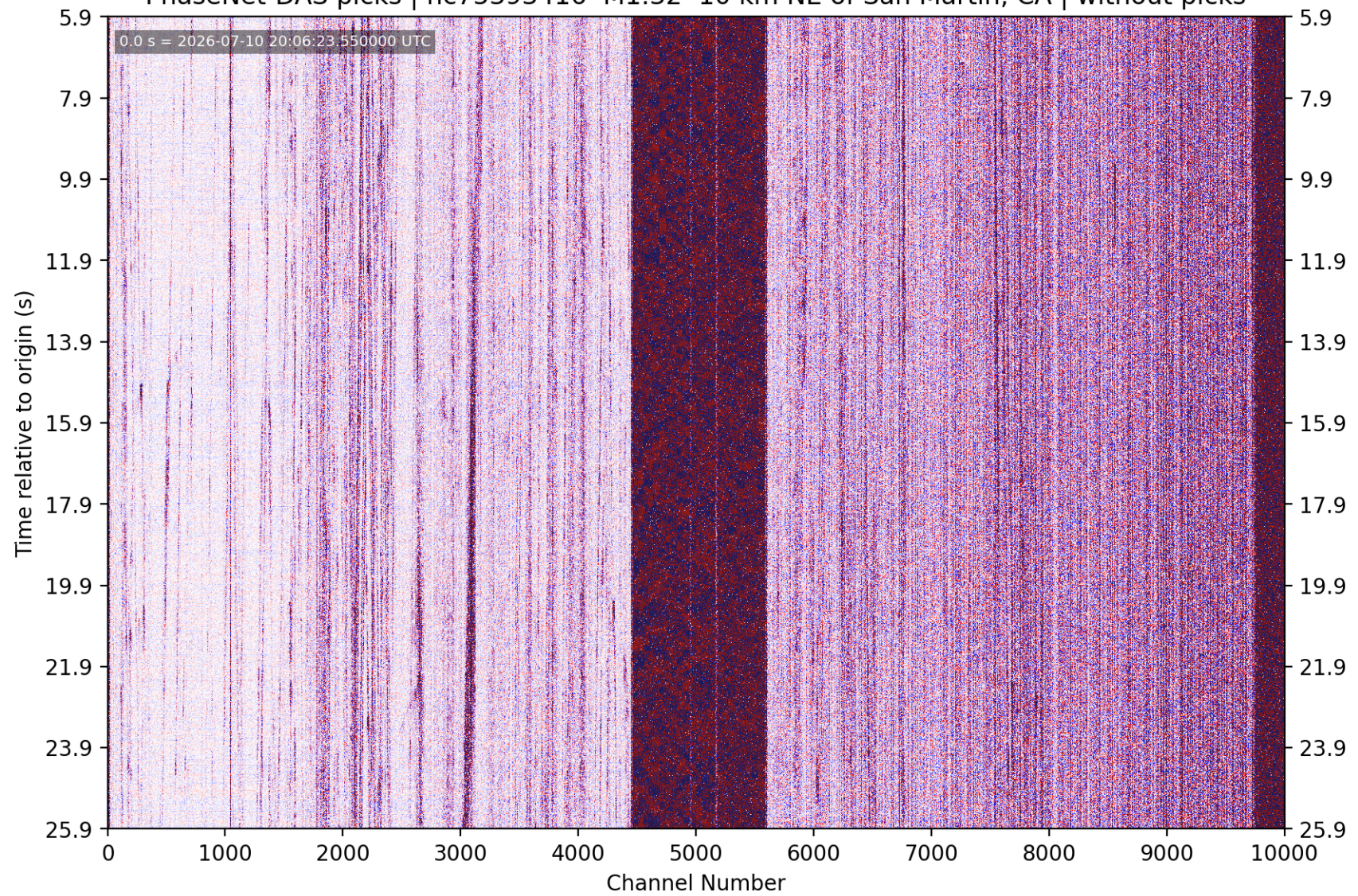
PhaseNet-DAS picks | nc75393416 M1.32 10 km NE of San Martin, CA | without picks
