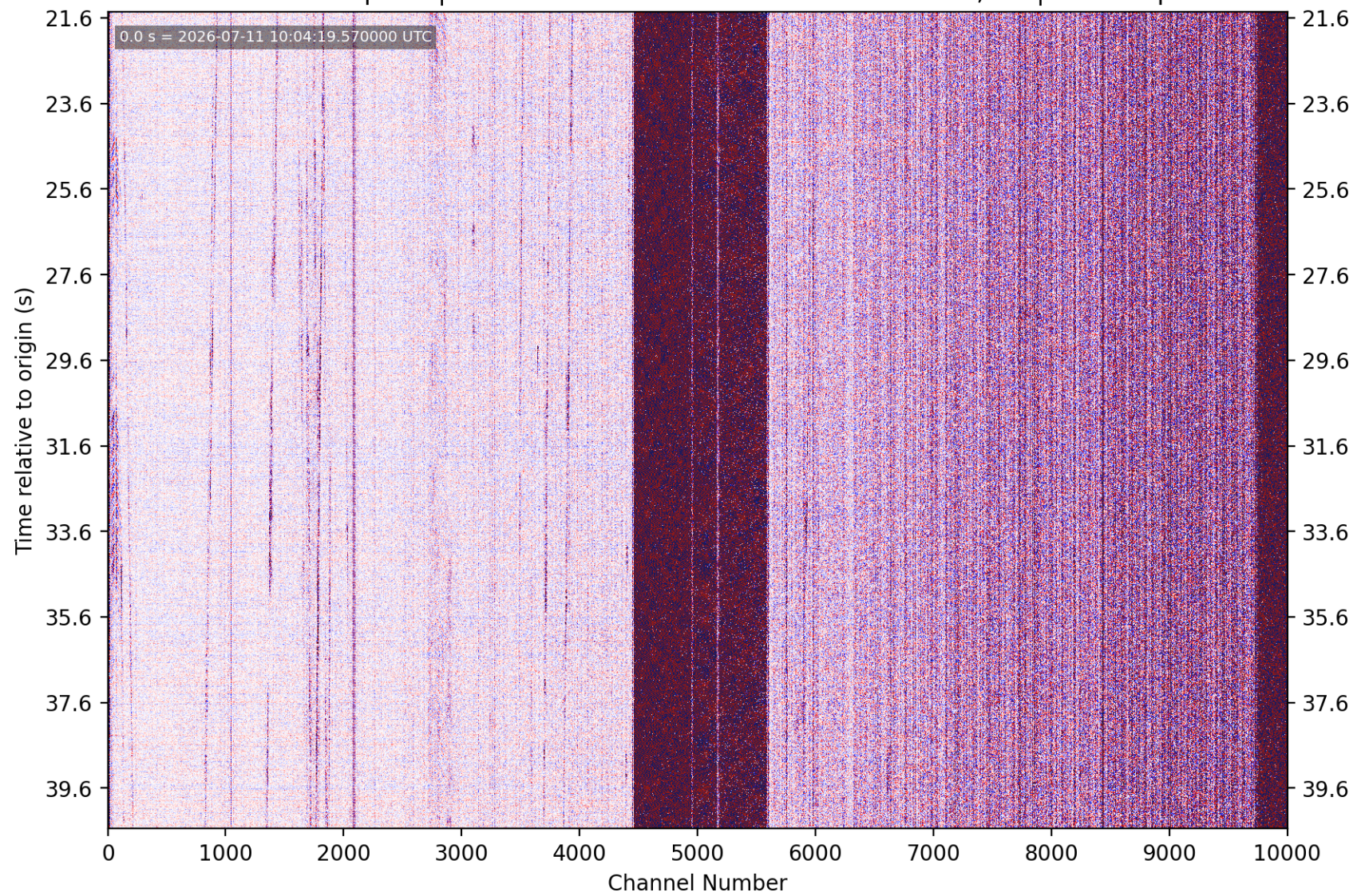
PhaseNet-DAS picks | nc75393816 M0.39 10 km SSE of Sunol, CA | without picks
