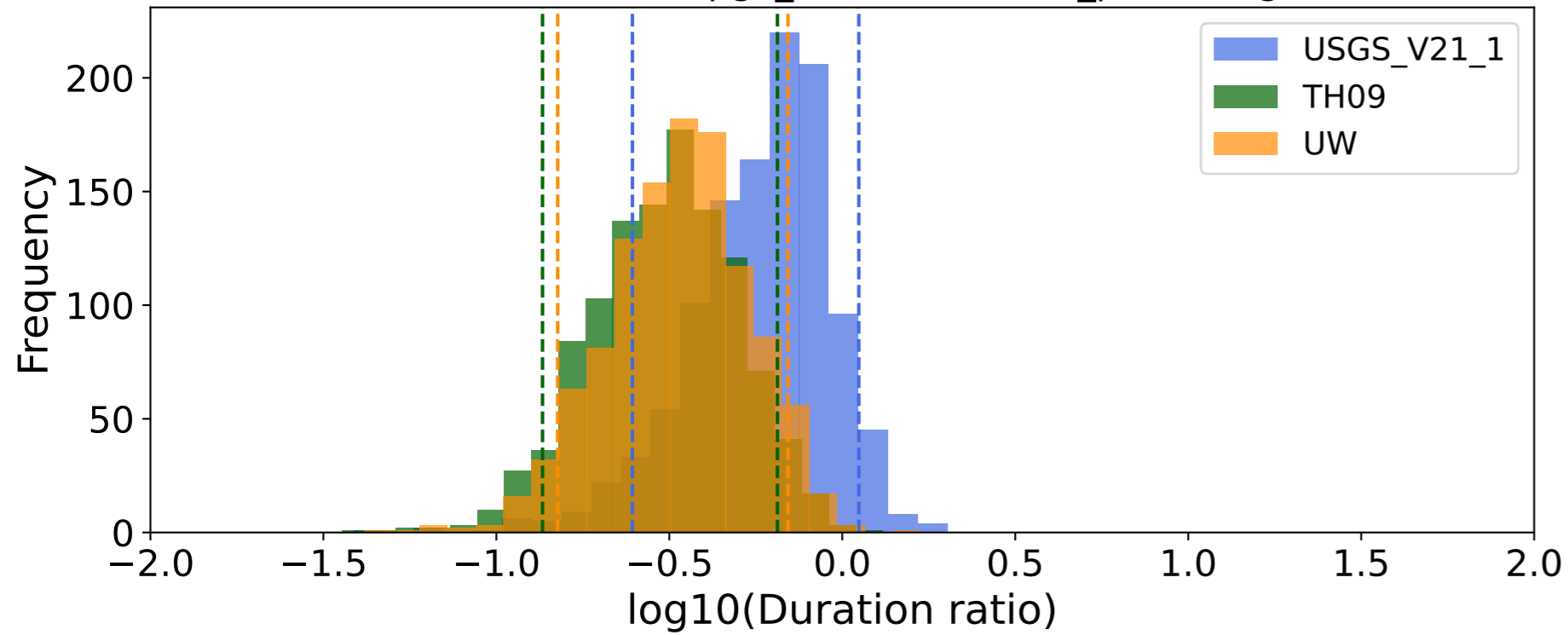
EventALL (0.16-0.5Hz) pgv_tw:60s duration_percentage:90%
