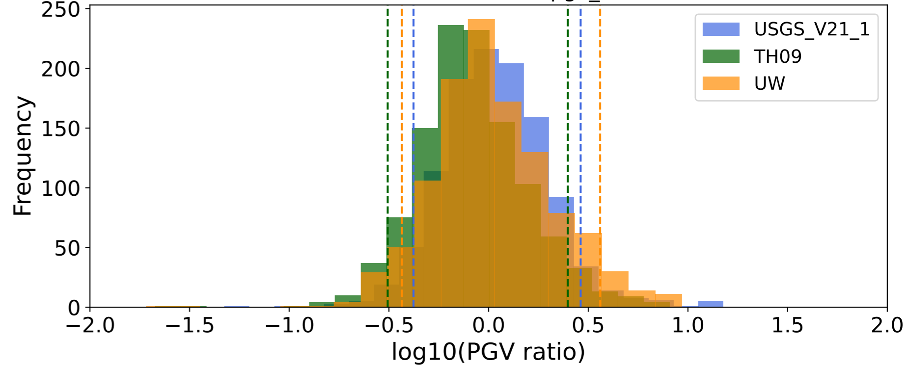
EventALL (0.16-0.5Hz) pgv_tw:60s
