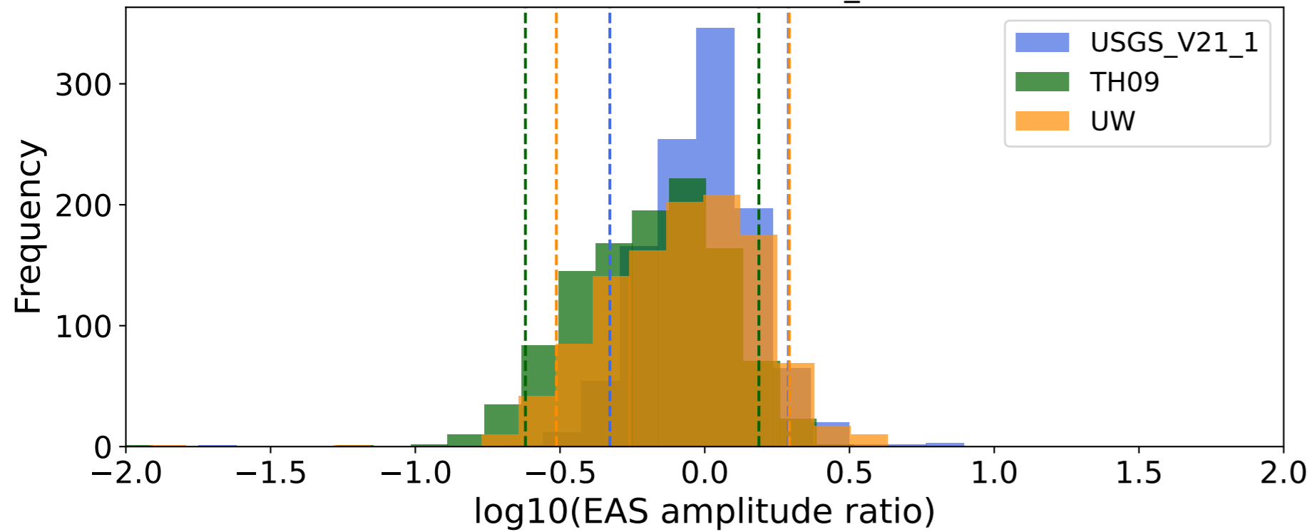
EventALL (0.16-0.5Hz) ko_bw:40
