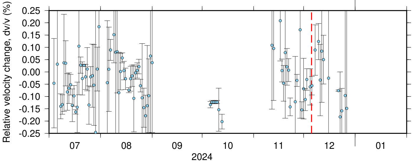
NC_KBU_PB_B046 ZRT 0.10-0.90Hz 011
