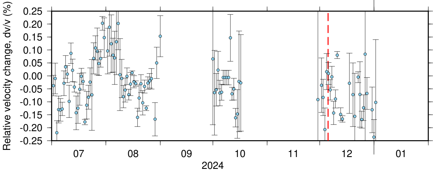
NC_KSM_PB_B046 ZRT 0.10-0.90Hz 011
