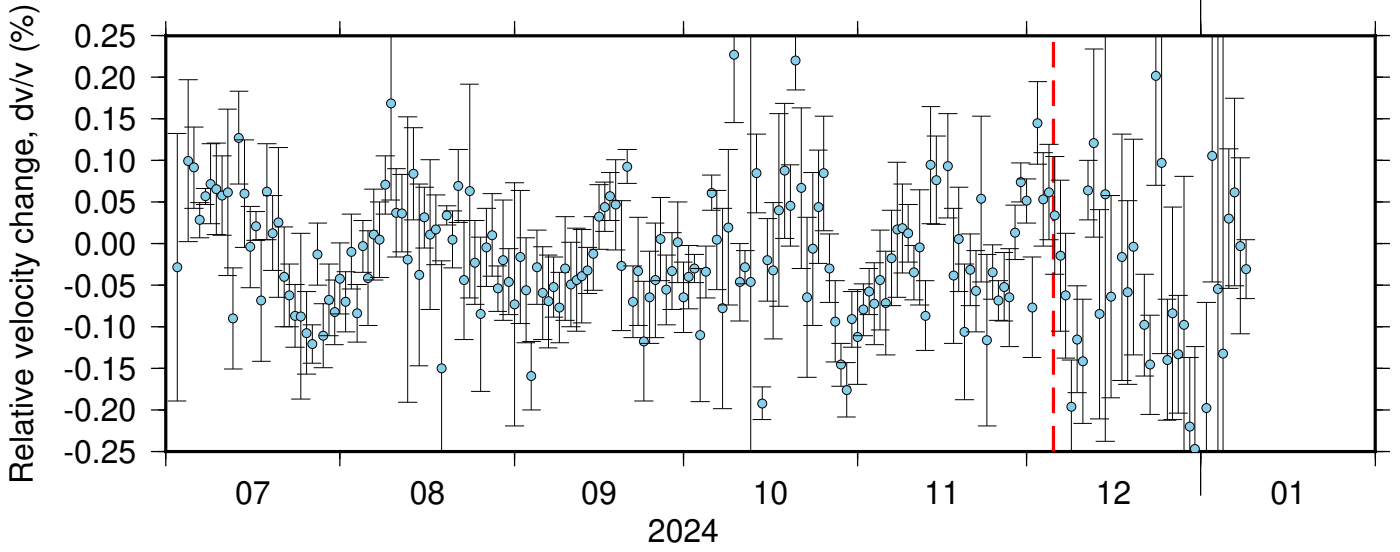
BK_KNEE_NC_KMPB ZRT 0.10-0.90Hz 011
