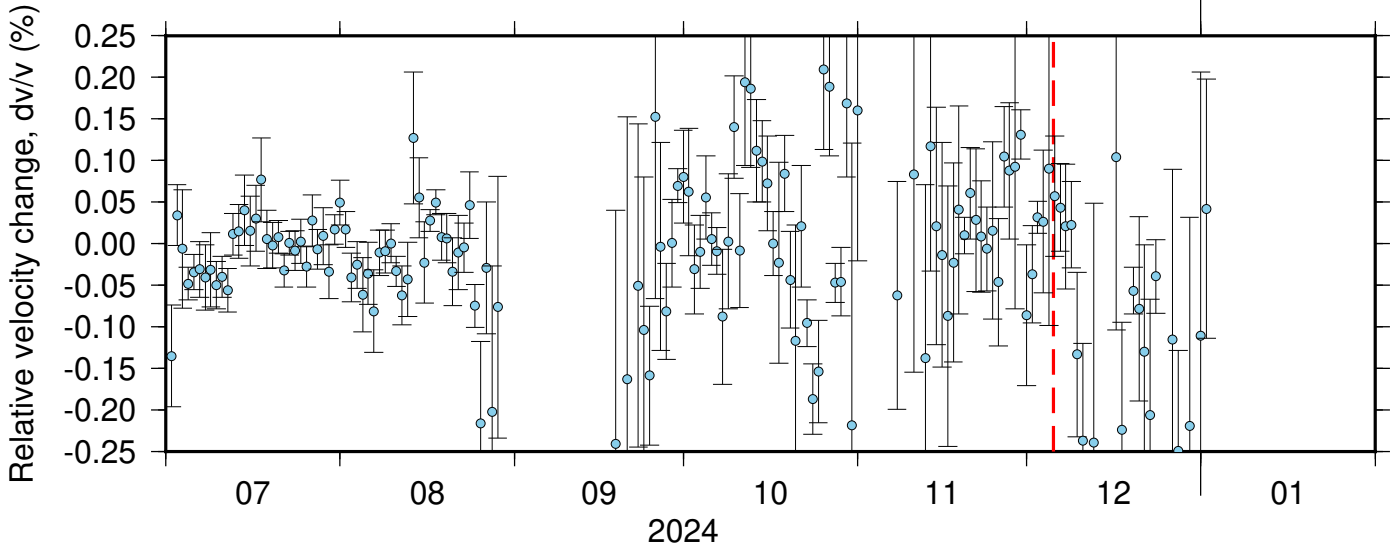
BK_BRIC_PB_B045 ZRT 0.10-0.90Hz 011
