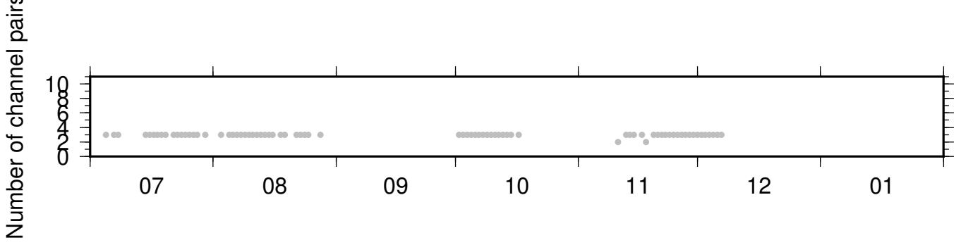
NC_KCR_PB_B046 ZRT 0.10-0.90Hz 011
