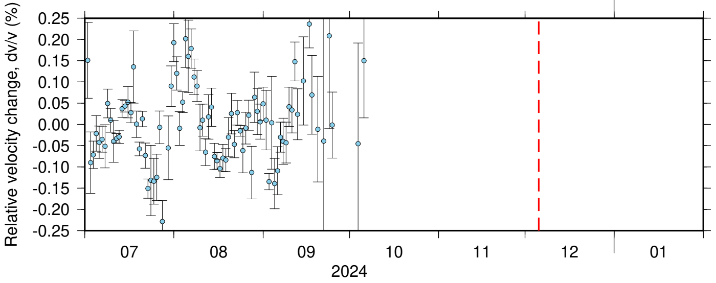
NC_KSM_PB_B932 ZRT 0.10-0.90Hz 011
