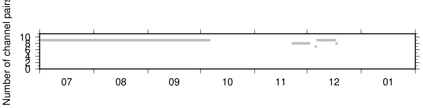
BK_WLKR_PB_B932 ZRT 0.10-0.90Hz 011
