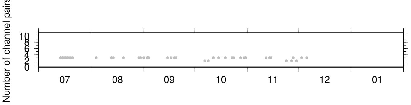
NC_KCR_PB_B934 ZRT 0.10-0.90Hz 011
