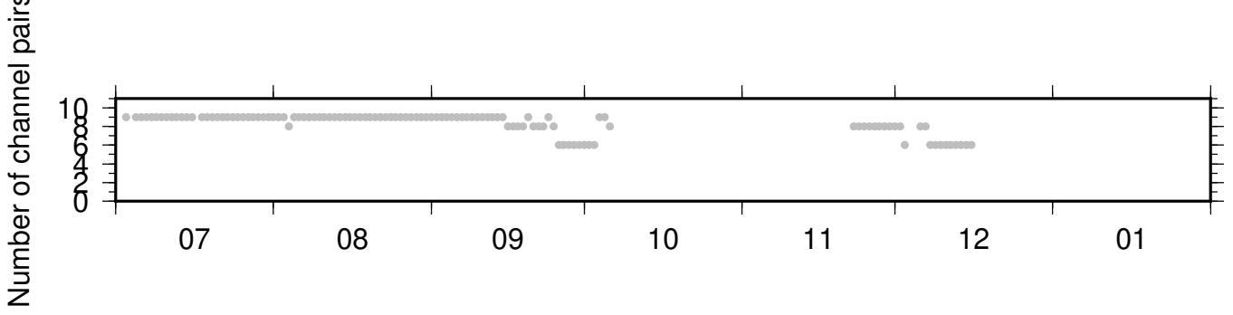
PB_B932_PB_B934 ZRT 0.10-0.90Hz 011
