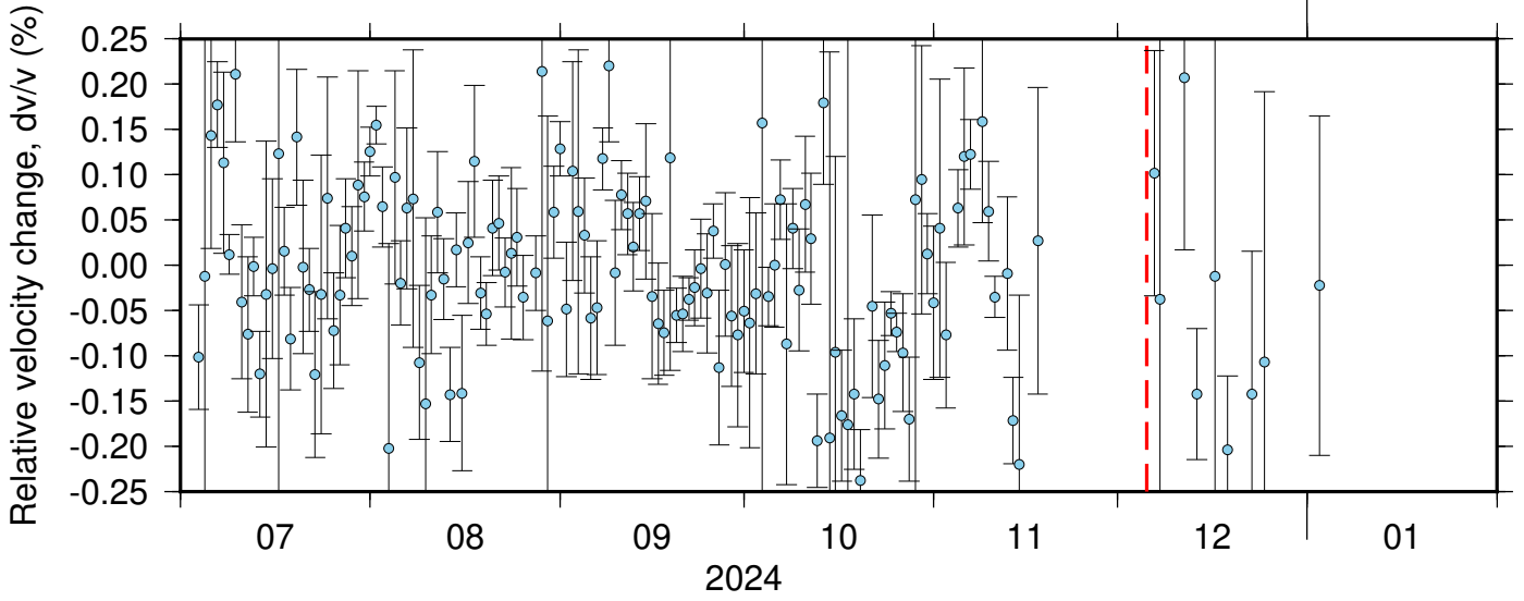
BK_KNEE_PB_B049 ZRT 0.10-0.90Hz 011
