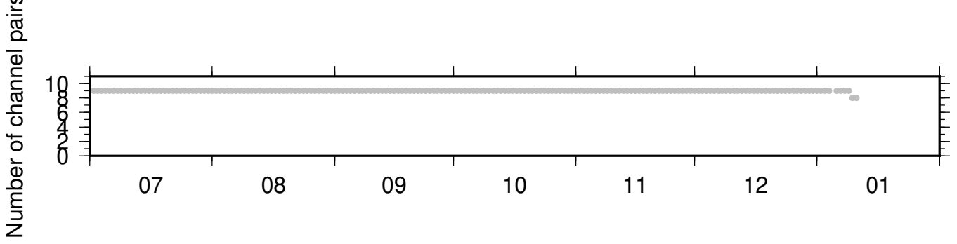
BK_BJES_BK_PRDS ZRT 0.10-0.90Hz 011
