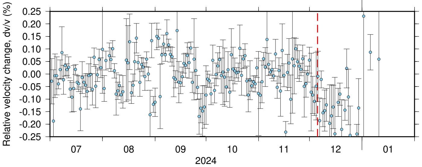
BK_BRIC_BK_PETL ZRT 0.10-0.90Hz 011
