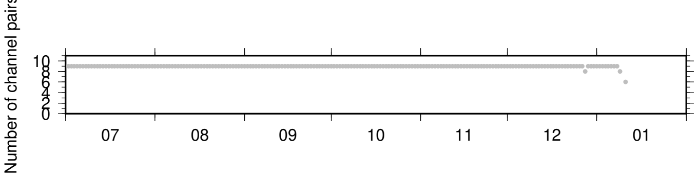
BK_BJES_BK_WLKR ZRT 0.10-0.90Hz 011
