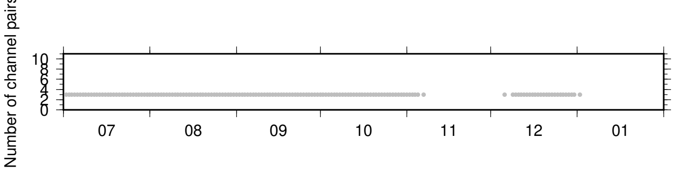
NC_KSM_PB_B049 ZRT 0.10-0.90Hz 011
