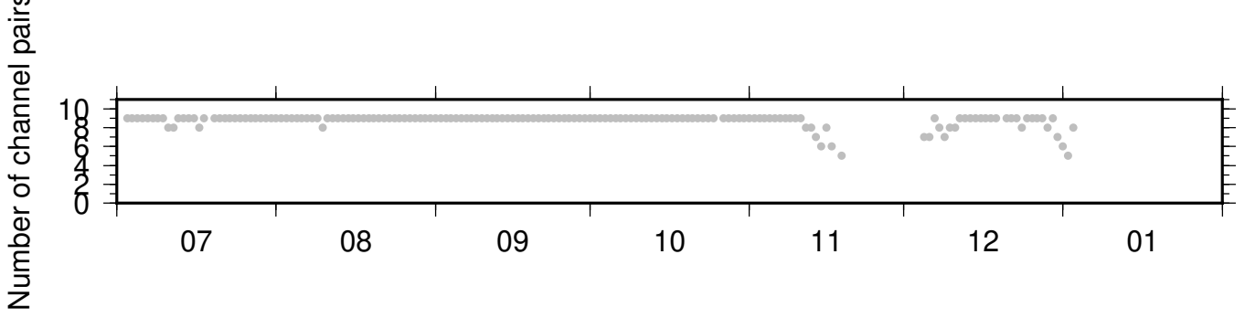
BK_JCC_PB_B049 ZRT 0.10-0.90Hz 011
