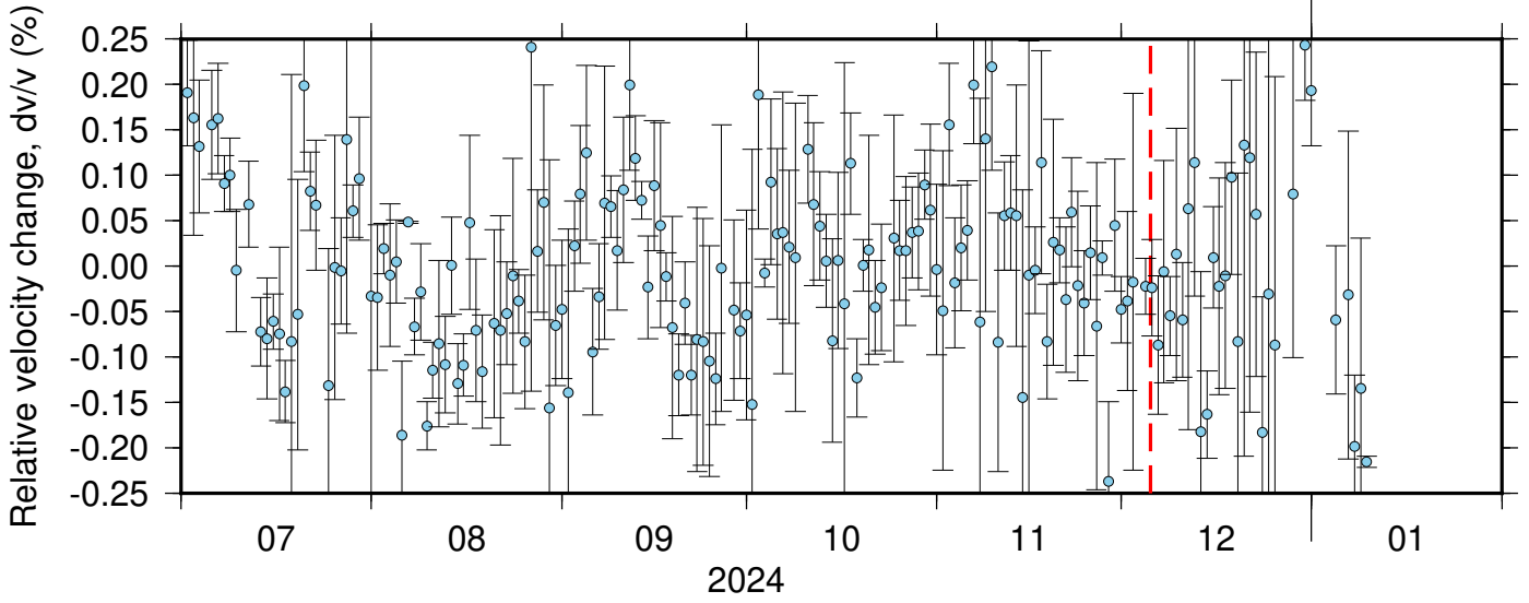
BK_BRIC_BK_JCC ZRT 0.10-0.90Hz 011
