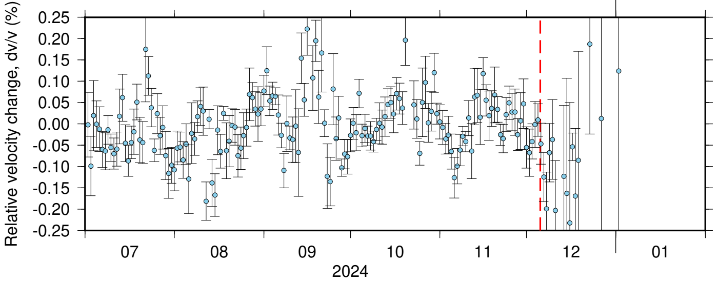
BK_PETL_NC_KCT ZRT 0.10-0.90Hz 011
