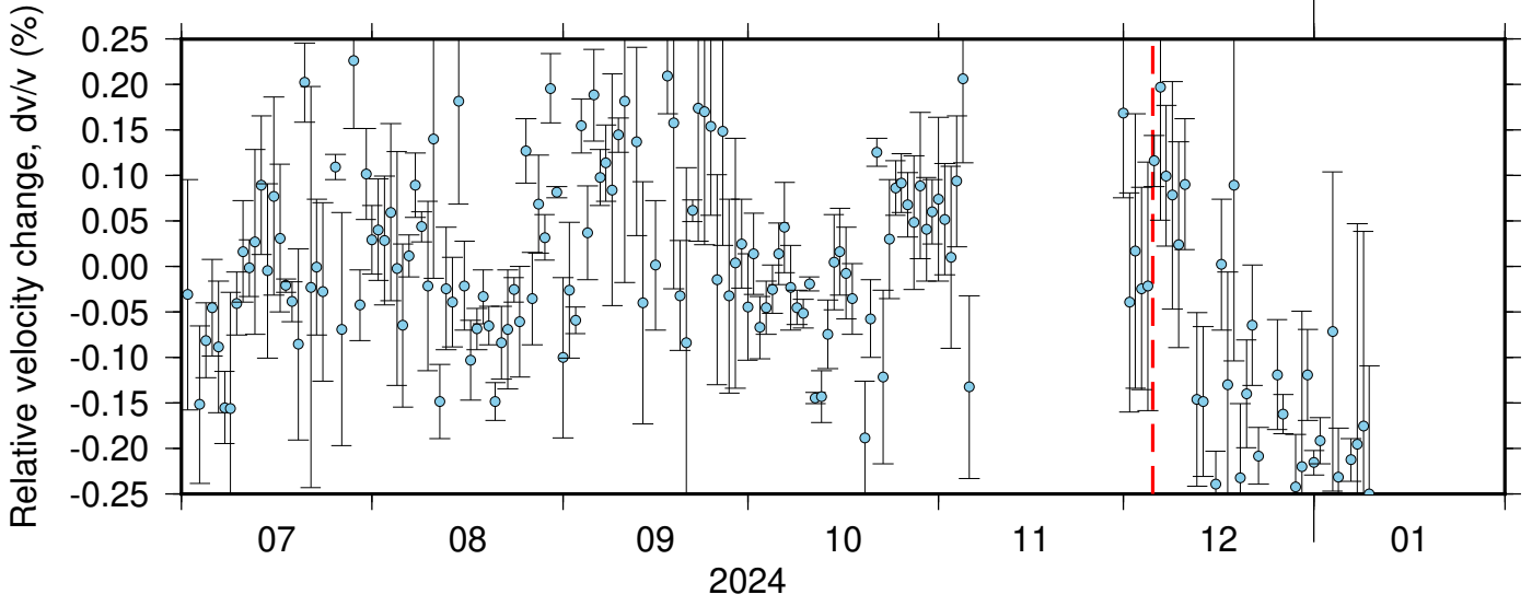
NC_KMPB_NC_KSM ZRT 0.10-0.90Hz 011
