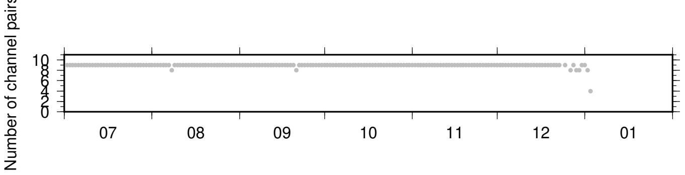
BK_BLAS_PB_B047 ZRT 0.10-0.90Hz 011
