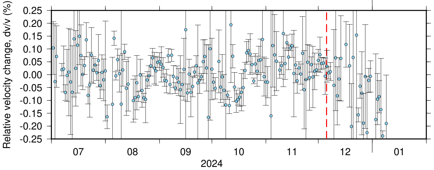
BK_HAYF_BK_PRDS ZRT 0.10-0.90Hz 011
