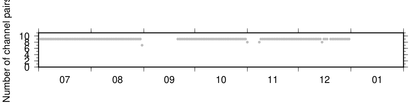
BK_PRDS_PB_B045 ZRT 0.10-0.90Hz 011
