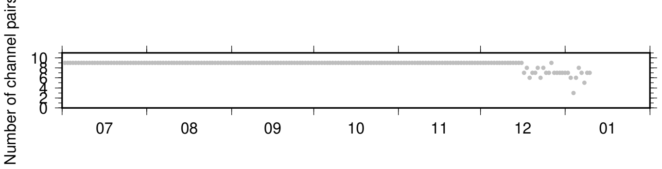
NC_KCT_NC_KMPB ZRT 0.10-0.90Hz 011
