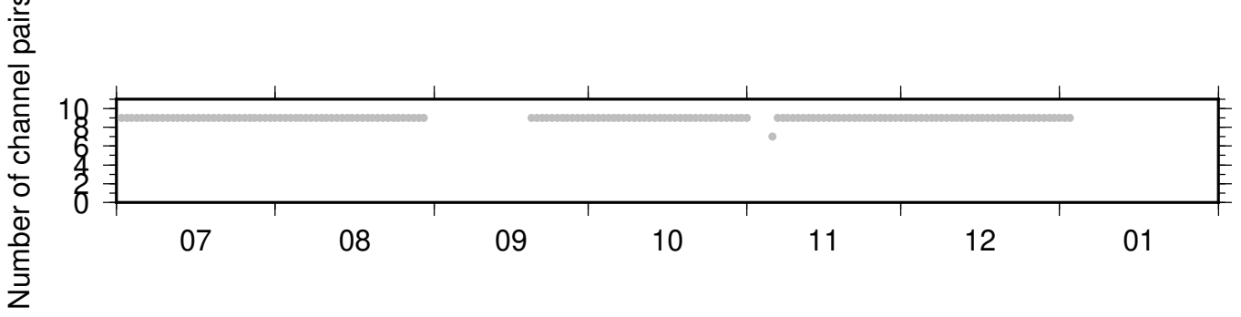
BK_BJES_PB_B045 ZRT 0.10-0.90Hz 011
