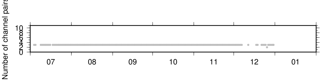
NC_KCR_PB_B047 ZRT 0.10-0.90Hz 011
