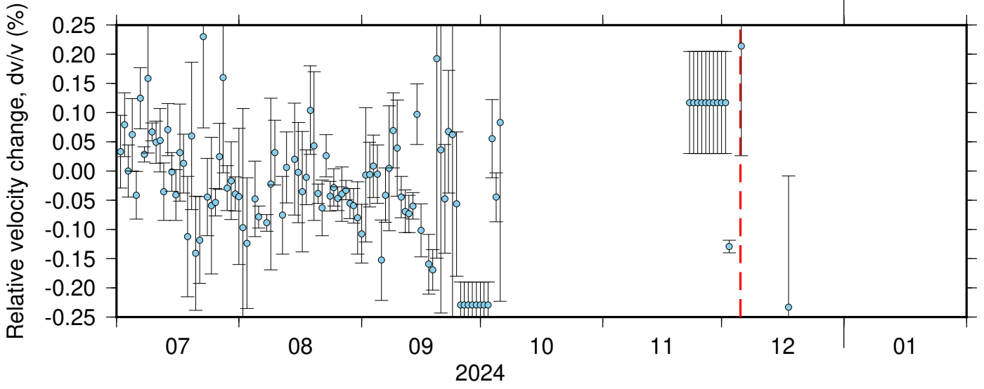
BK_HAYF_PB_B932 ZRT 0.10-0.90Hz 011
