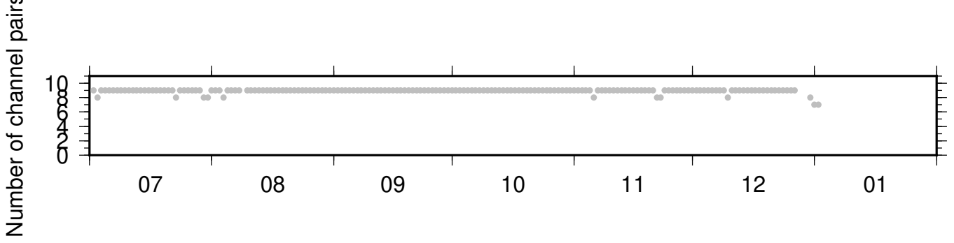
BK_KNEE_PB_B047 ZRT 0.10-0.90Hz 011
