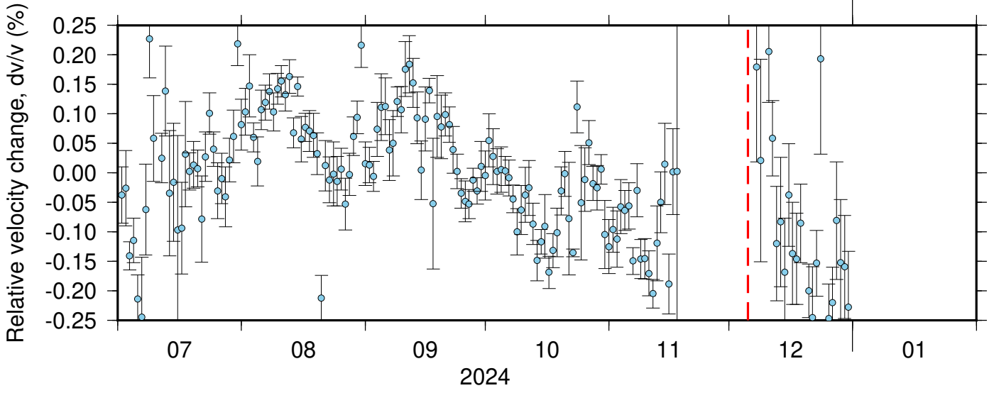
NC_KBU_PB_B049 ZRT 0.10-0.90Hz 011
