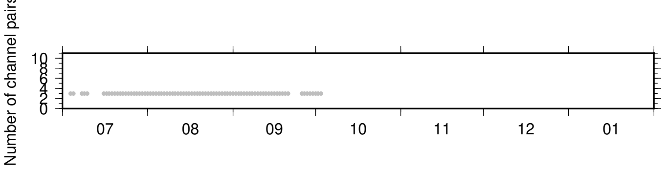
NC_KCR_PB_B932 ZRT 0.10-0.90Hz 011
