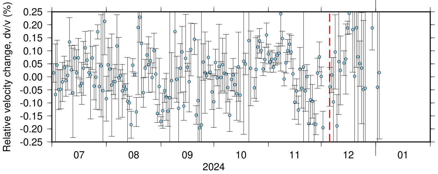
PB_B047_PB_B935 ZRT 0.10-0.90Hz 011
