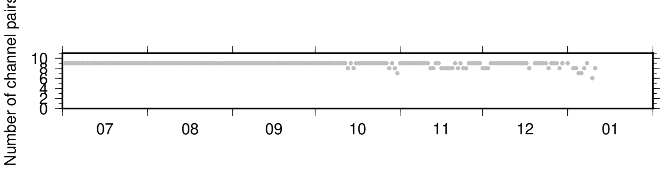
BK_BRIC_BK_KNEE ZRT 0.10-0.90Hz 011
