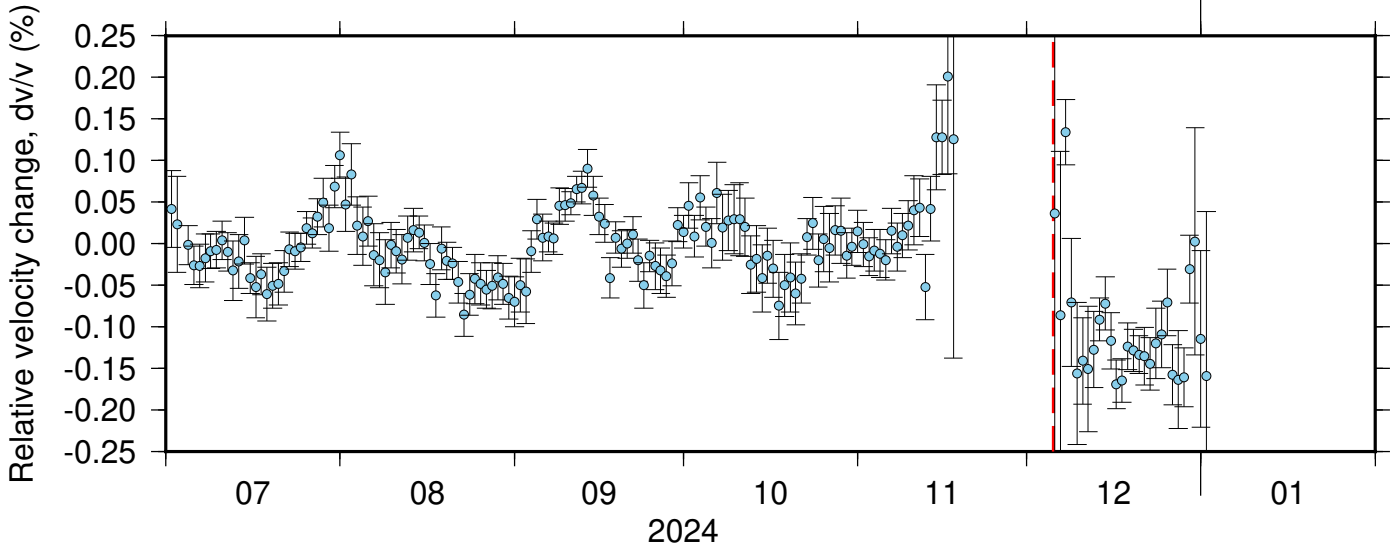
BK_BRIC_PB_B049 ZRT 0.10-0.90Hz 011
