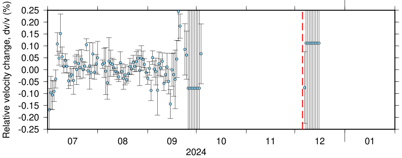
NC_KMR_PB_B932 ZRT 0.10-0.90Hz 011
