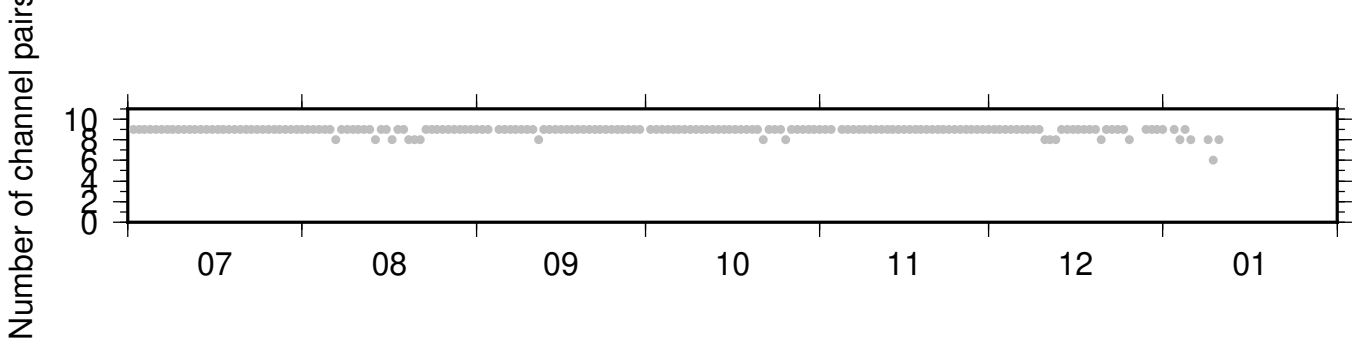
BK_HAYF_BK_JCC ZRT 0.10-0.90Hz 011
