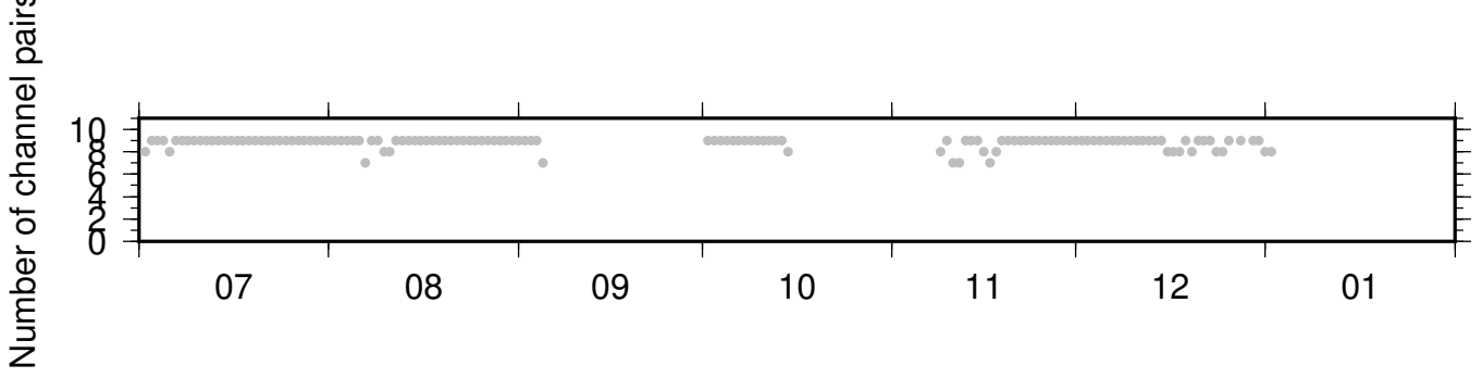
PB_B046_PB_B934 ZRT 0.10-0.90Hz 011
