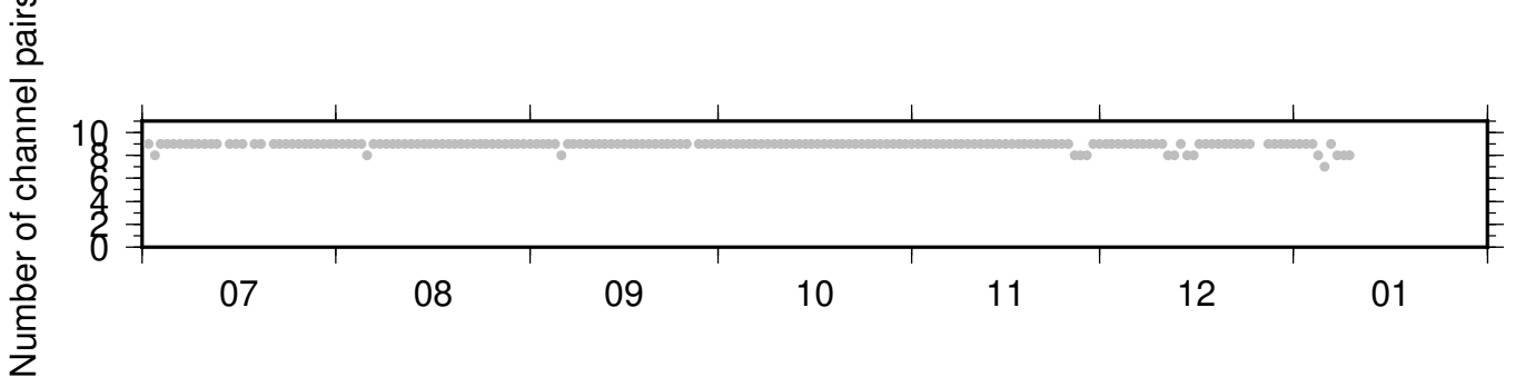
BK_KNEE_BK_PRDS ZRT 0.10-0.90Hz 011
