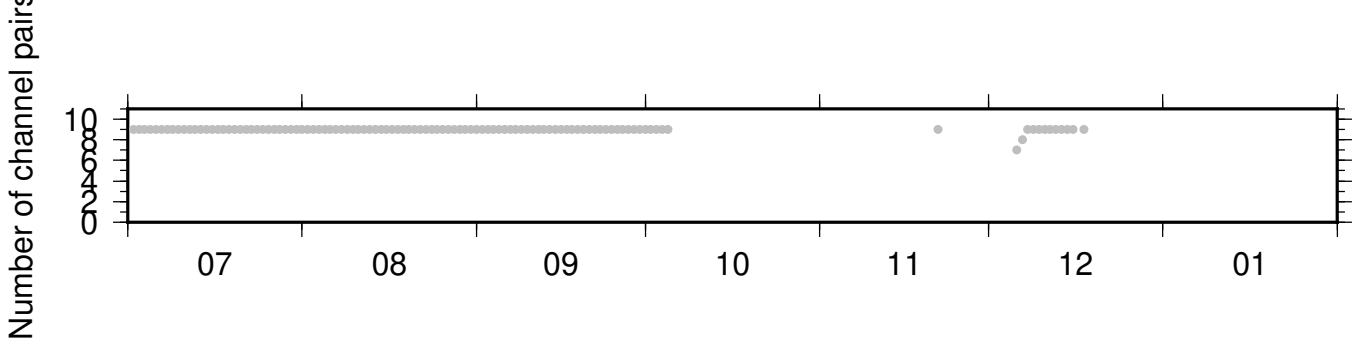
NC_KCT_PB_B932 ZRT 0.10-0.90Hz 011
