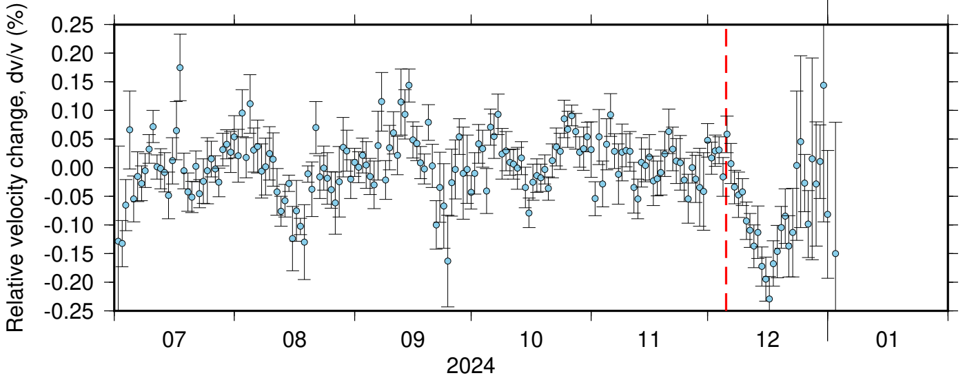
BK_SPRL_PB_B934 ZRT 0.10-0.90Hz 011
