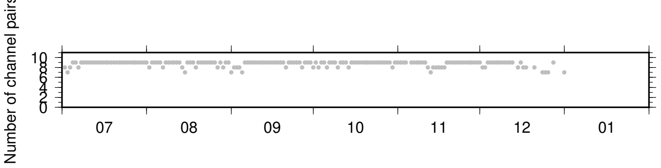
PB_B934_PB_B935 ZRT 0.10-0.90Hz 011
