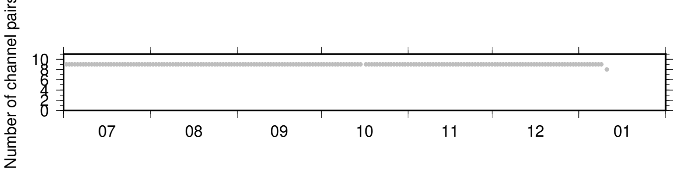
BK_KNEE_BK_RBOW ZRT 0.10-0.90Hz 011
