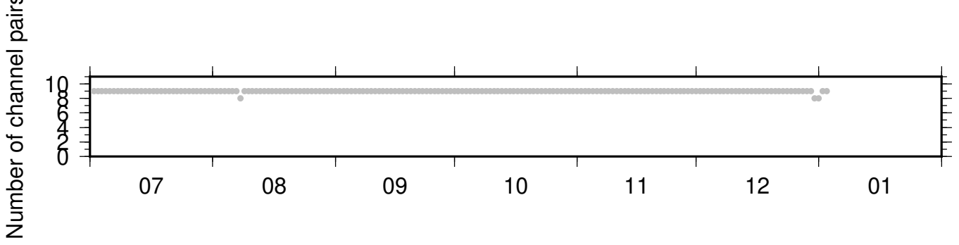
BK_KNEE_PB_B935 ZRT 0.10-0.90Hz 011
