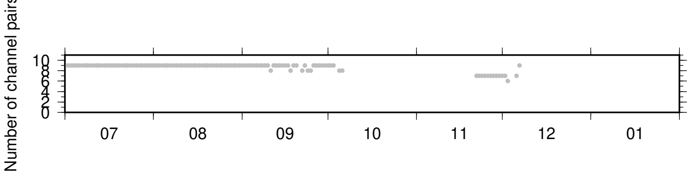
BK_KNEE_PB_B932 ZRT 0.10-0.90Hz 011
