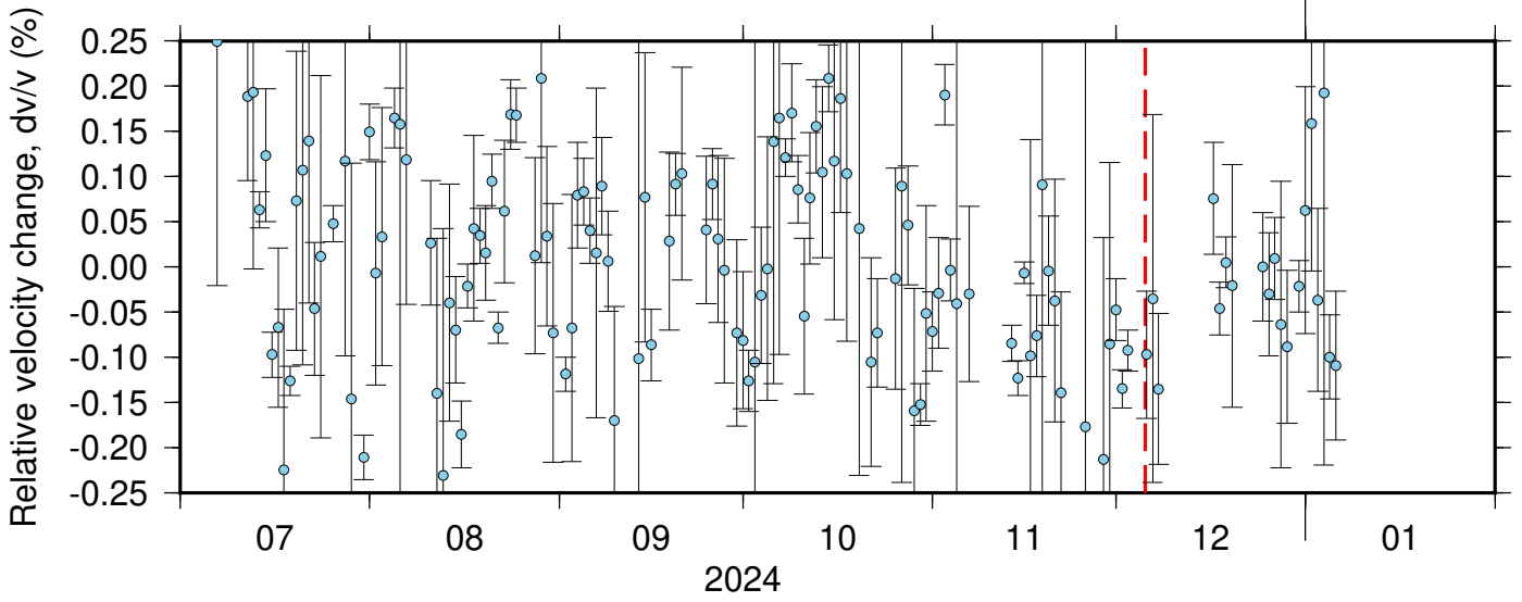
BK_BLAS_NC_KPR ZRT 0.10-0.90Hz 011
