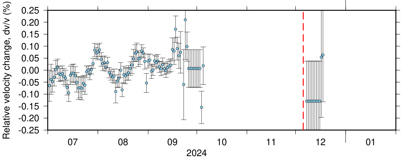
BK_WLKR_PB_B932 ZRT 0.10-0.90Hz 011
