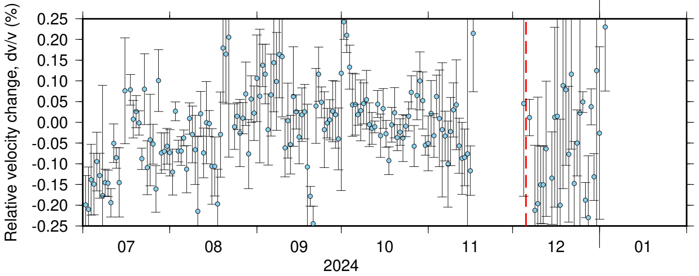
BK_WLKR_PB_B049 ZRT 0.10-0.90Hz 011
