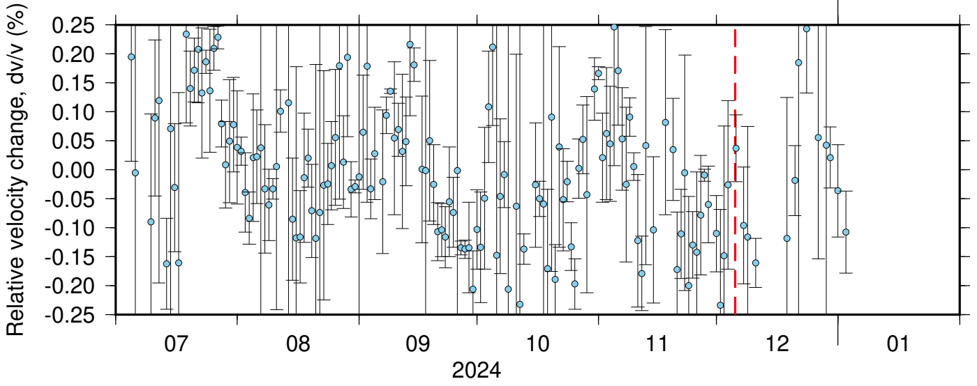
BK_WLKR_NC_KBU ZRT 0.10-0.90Hz 011
