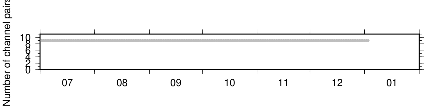
NC_KMR_PB_B935 ZRT 0.10-0.90Hz 011
