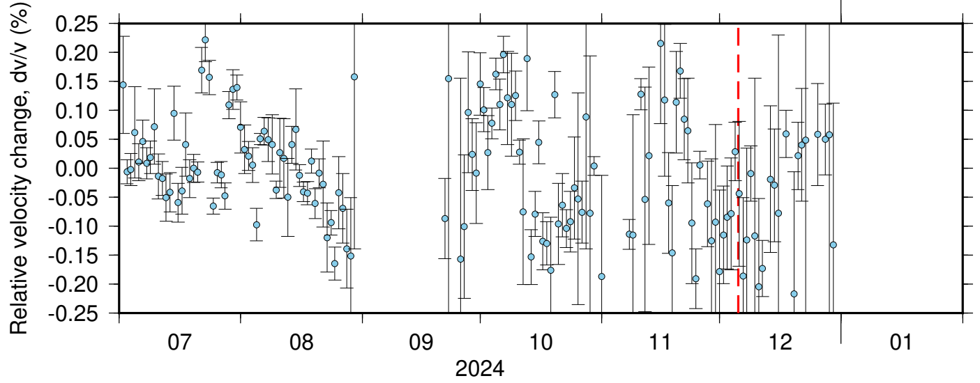
BK_PRDS_PB_B045 ZRT 0.10-0.90Hz 011
