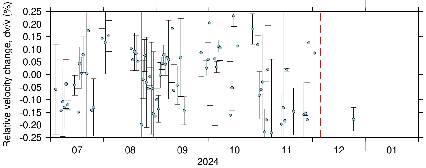
BK_KNEE_NC_KBU ZRT 0.10-0.90Hz 011
