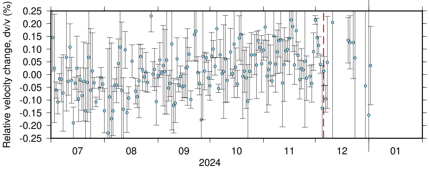
BK_WLKR_PB_B935 ZRT 0.10-0.90Hz 011
