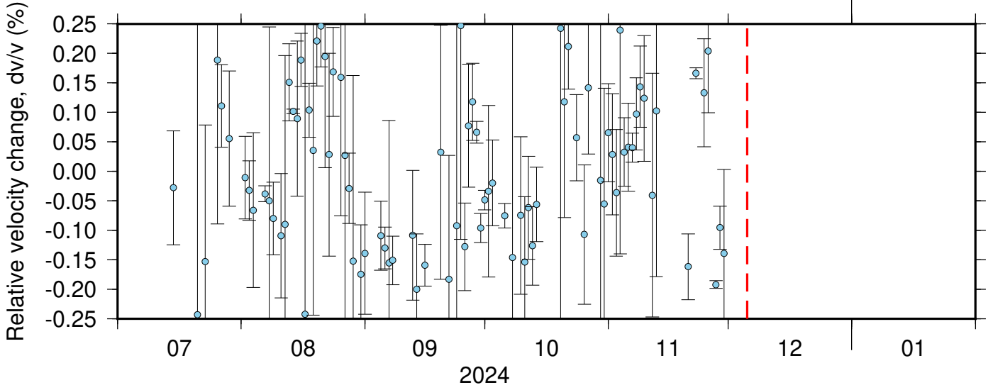
NC_KCR_NC_KCT ZRT 0.10-0.90Hz 011
