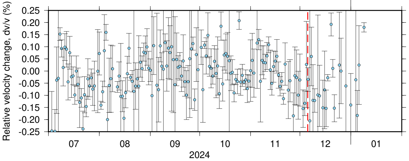
BK_HAYF_BK_JCC ZRT 0.10-0.90Hz 011
