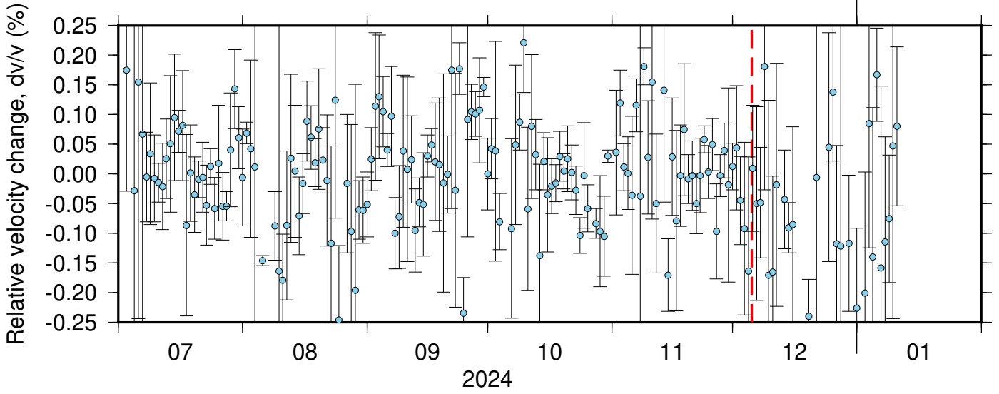
BK_KNEE_NC_KMR ZRT 0.10-0.90Hz 011
