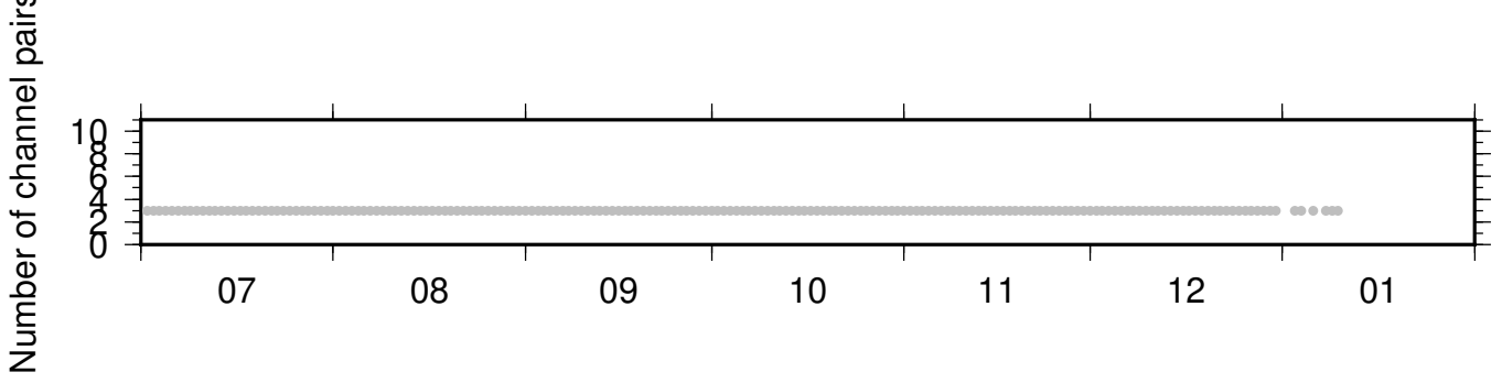
BK_PETL_NC_KPR ZRT 0.10-0.90Hz 011
