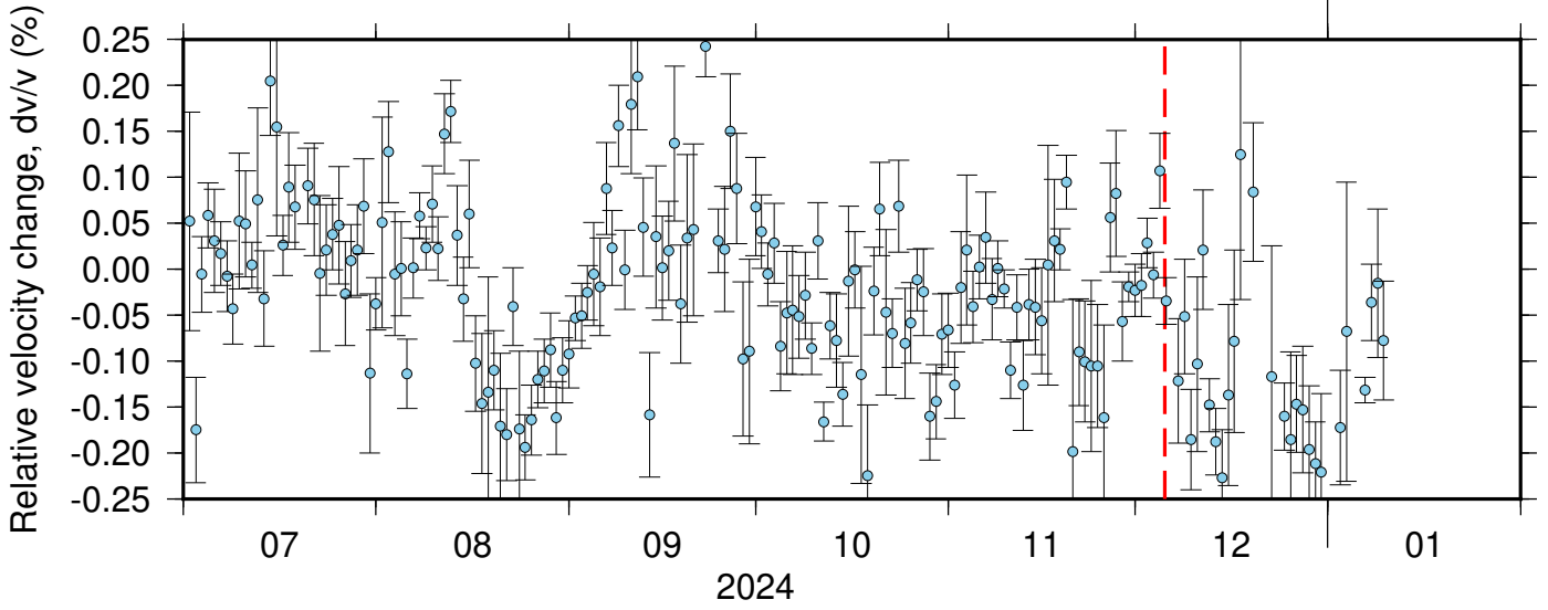
BK_BJES_BK_JCC ZRT 0.10-0.90Hz 011
