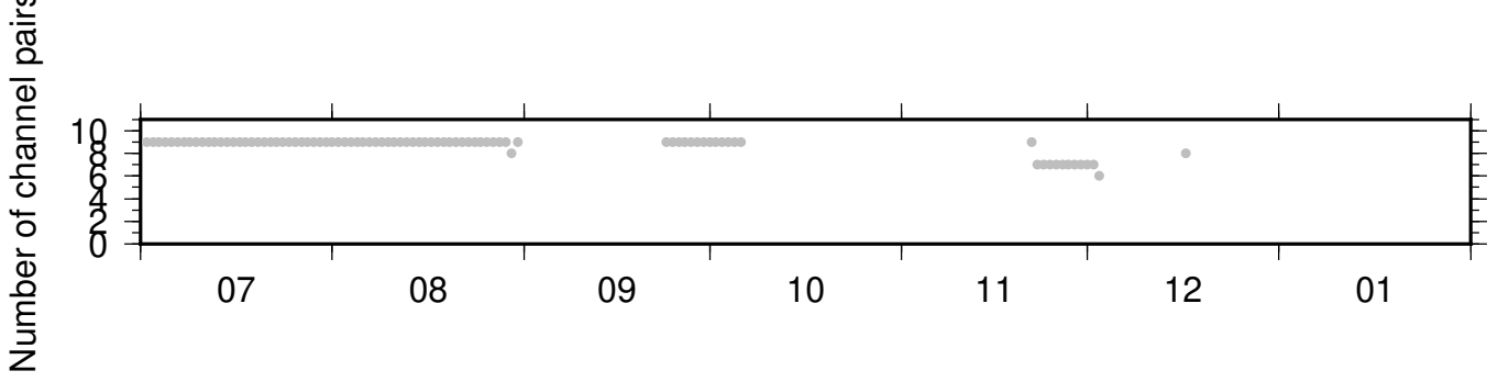
PB_B045_PB_B932 ZRT 0.10-0.90Hz 011
