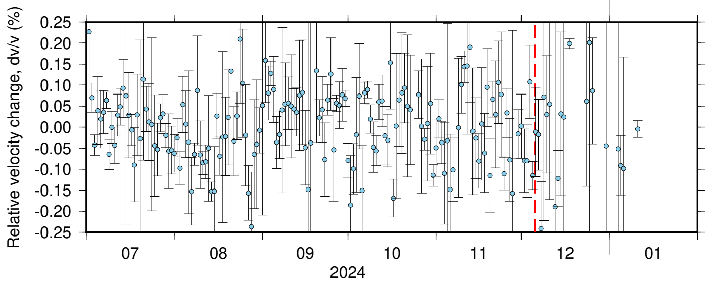
BK_BRIC_NC_KCT ZRT 0.10-0.90Hz 011
