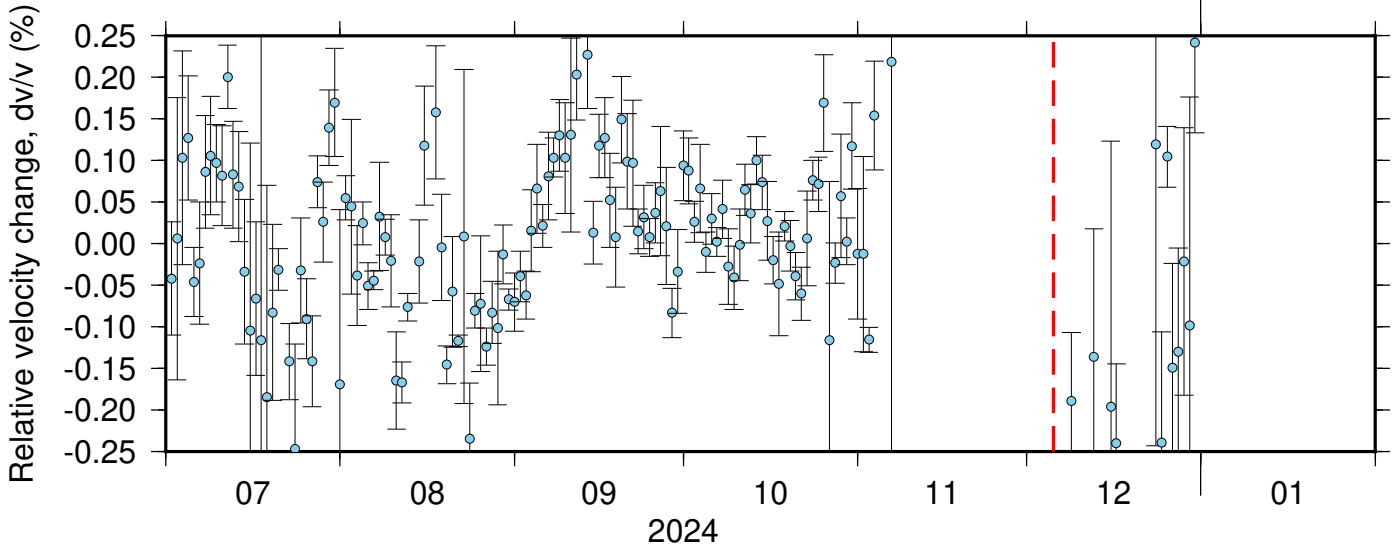
NC_KSM_PB_B049 ZRT 0.10-0.90Hz 011
