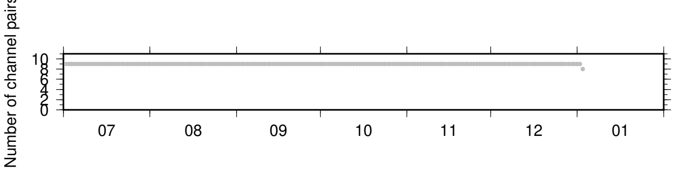
BK_SPRL_PB_B047 ZRT 0.10-0.90Hz 011
