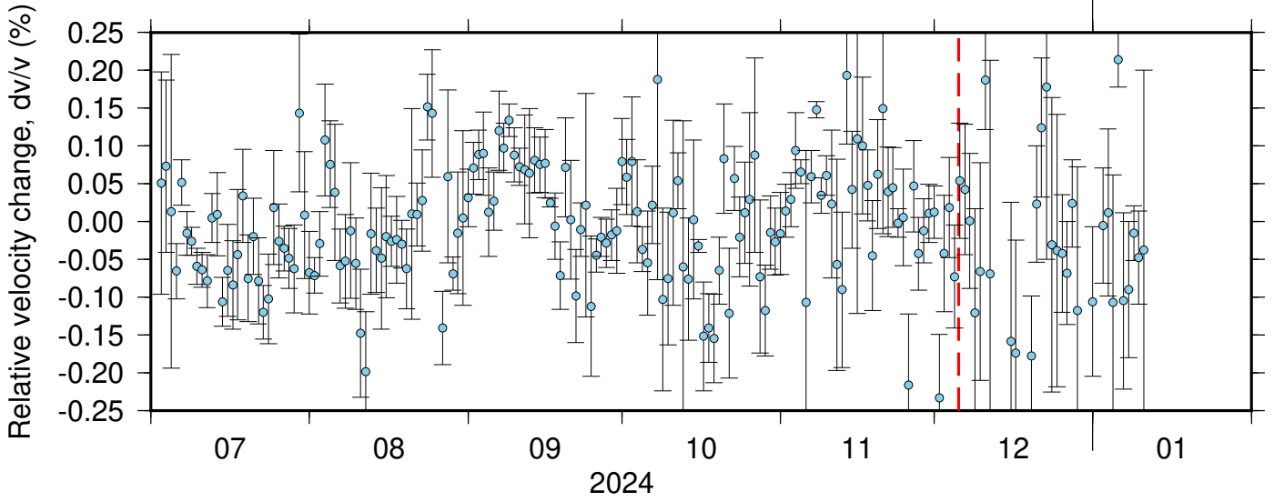
BK_BLAS_BK_RBOW ZRT 0.10-0.90Hz 011
