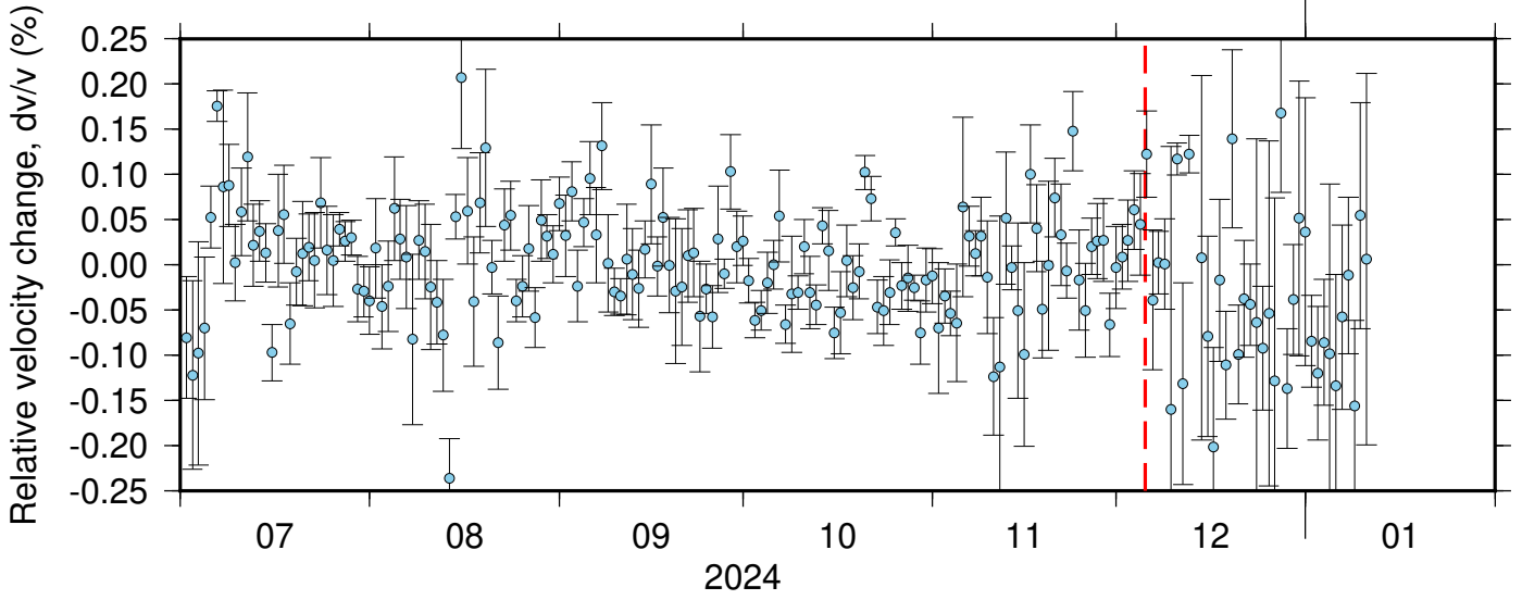
BK_BJES_NC_KMR ZRT 0.10-0.90Hz 011
