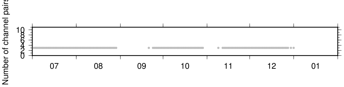
NC_KBU_PB_B045 ZRT 0.10-0.90Hz 011
