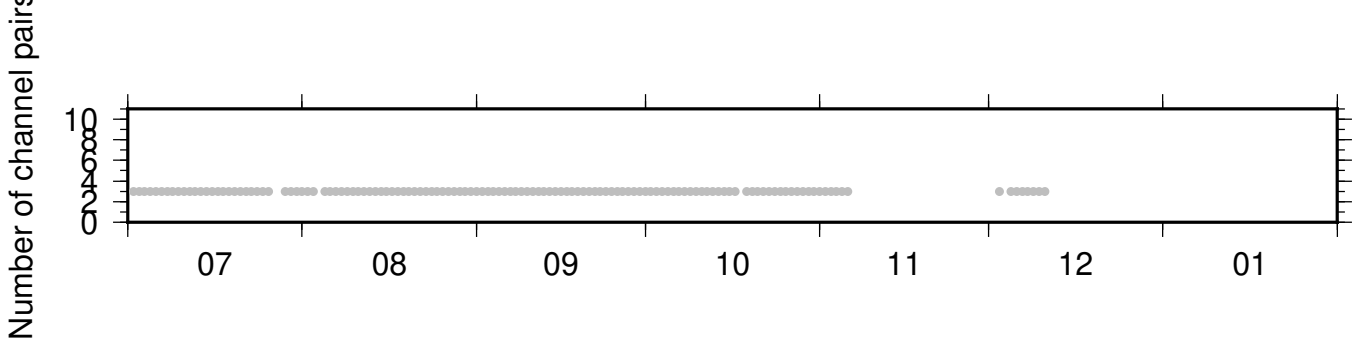
NC_KCT_NC_KSM ZRT 0.10-0.90Hz 011
