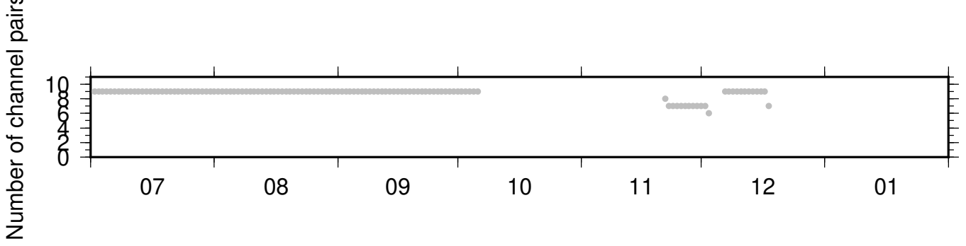
BK_PRDS_PB_B932 ZRT 0.10-0.90Hz 011
