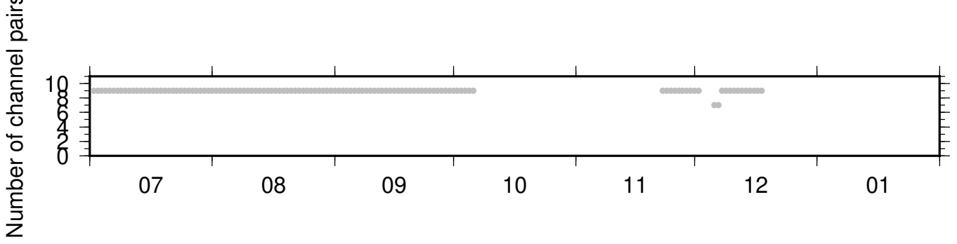
BK_PETL_PB_B932 ZRT 0.10-0.90Hz 011
