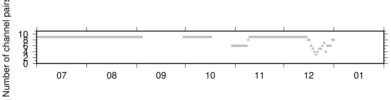
NC_KCT_PB_B046 ZRT 0.10-0.90Hz 011
