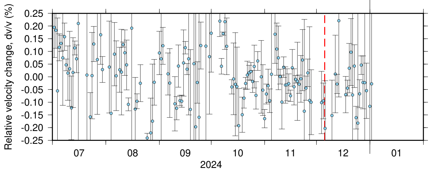
NC_KBU_PB_B935 ZRT 0.10-0.90Hz 011
