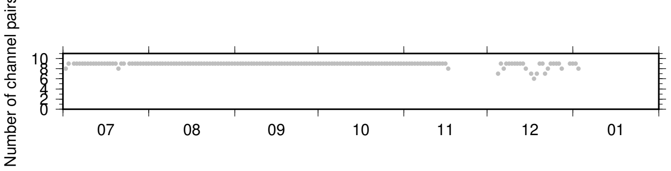
BK_HAYF_PB_B049 ZRT 0.10-0.90Hz 011
