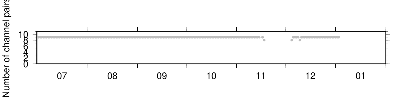
BK_BJES_PB_B049 ZRT 0.10-0.90Hz 011
