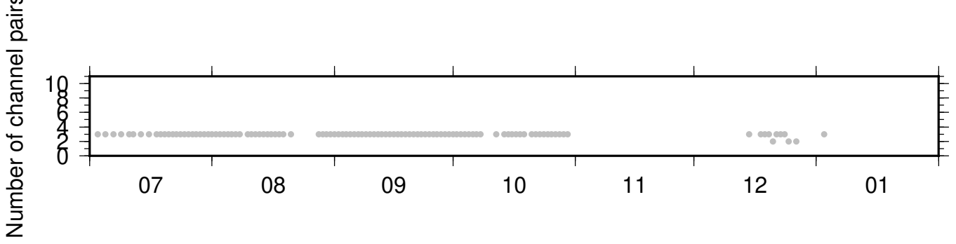
NC_KSM_PB_B934 ZRT 0.10-0.90Hz 011
