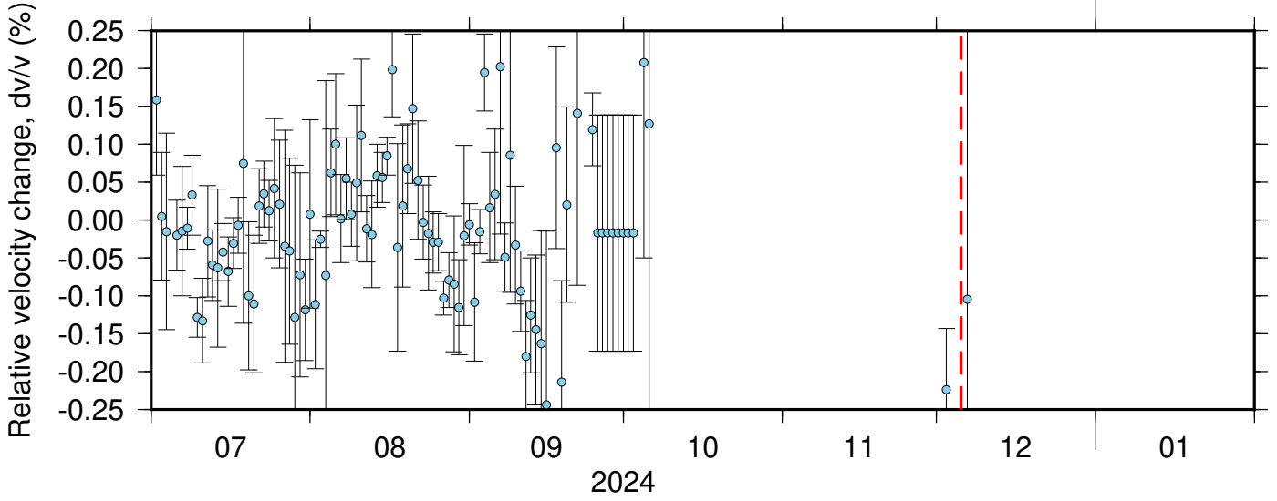
BK_KNEE_PB_B932 ZRT 0.10-0.90Hz 011
