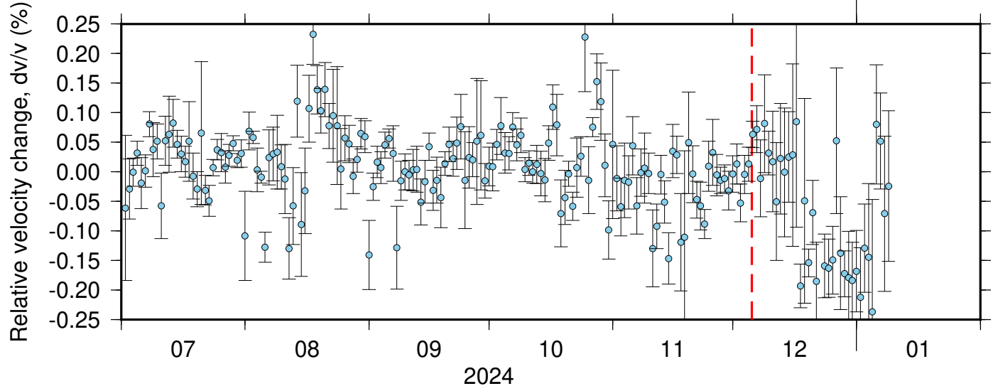
BK_BJES_BK_RBOW ZRT 0.10-0.90Hz 011
