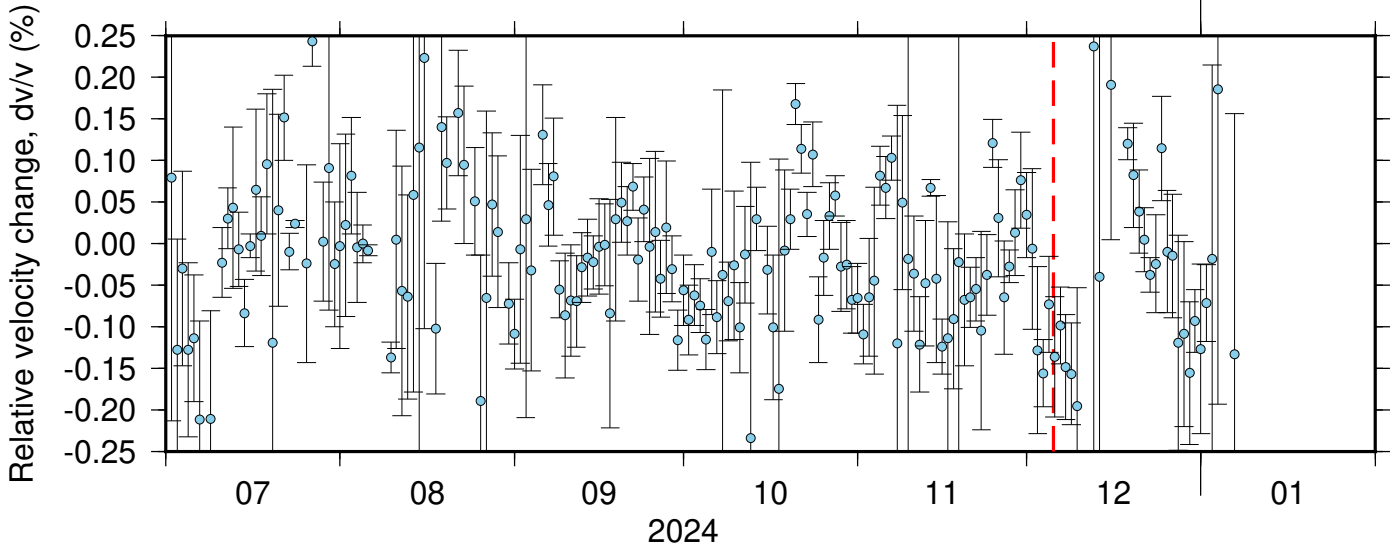
BK_BJES_NC_KBU ZRT 0.10-0.90Hz 011
