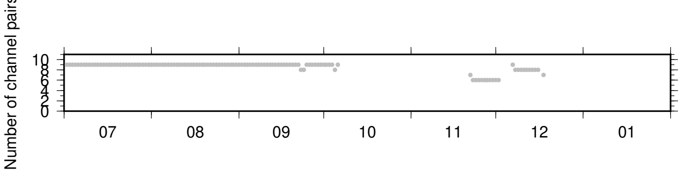
NC_KMR_PB_B932 ZRT 0.10-0.90Hz 011
