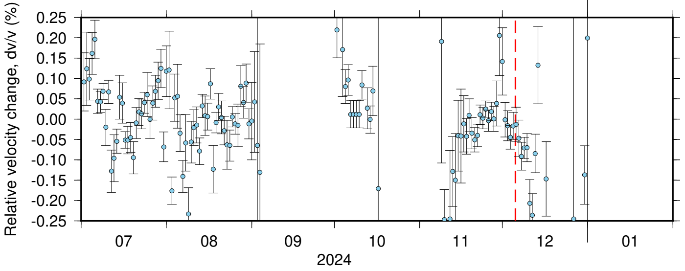
NC_KCT_PB_B046 ZRT 0.10-0.90Hz 011
