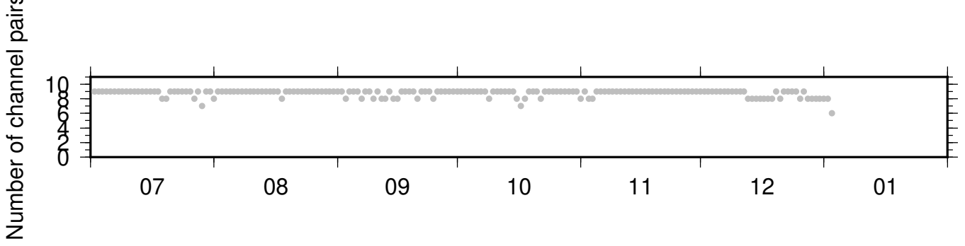
BK_BLAS_PB_B934 ZRT 0.10-0.90Hz 011
