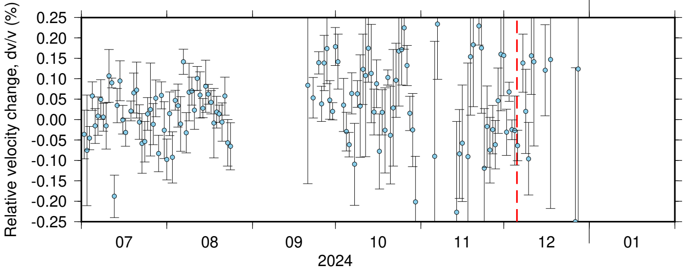
NC_KCT_PB_B045 ZRT 0.10-0.90Hz 011
