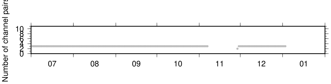
NC_KSM_PB_B047 ZRT 0.10-0.90Hz 011
