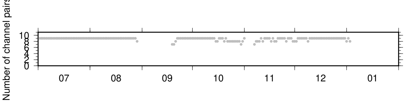
BK_BRIC_PB_B045 ZRT 0.10-0.90Hz 011
