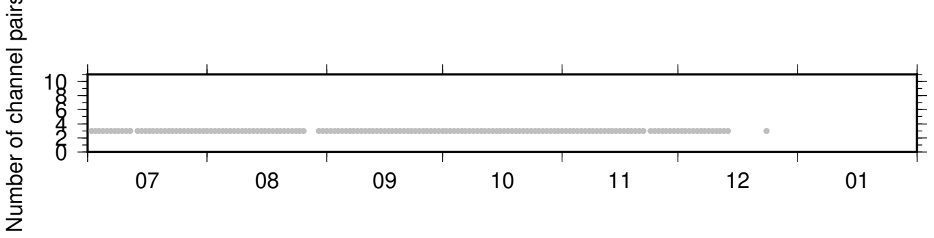
NC_KCT_NC_KPR ZRT 0.10-0.90Hz 011
