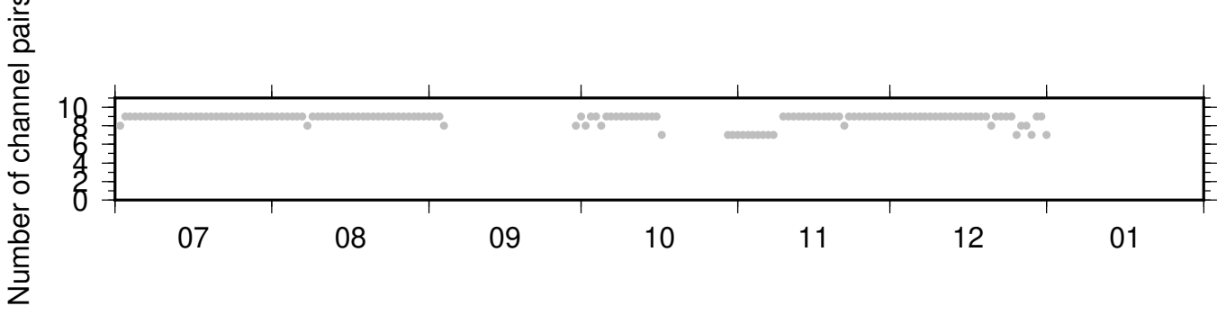
BK_KNEE_PB_B046 ZRT 0.10-0.90Hz 011
