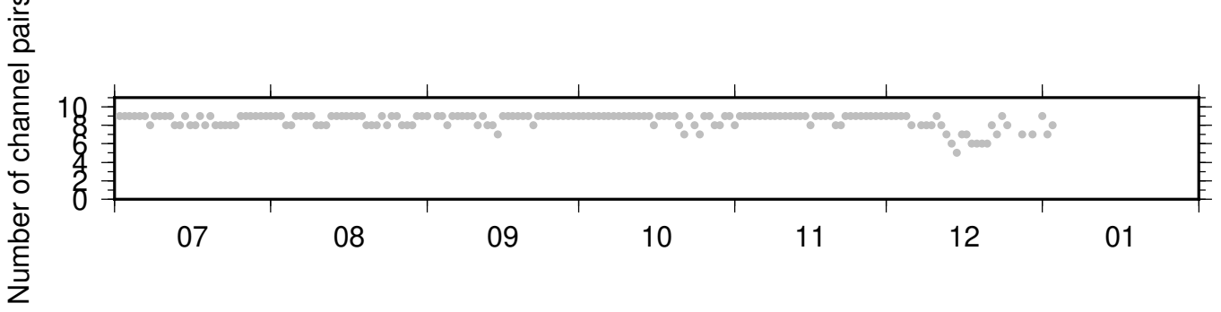
BK_HAYF_PB_B934 ZRT 0.10-0.90Hz 011
