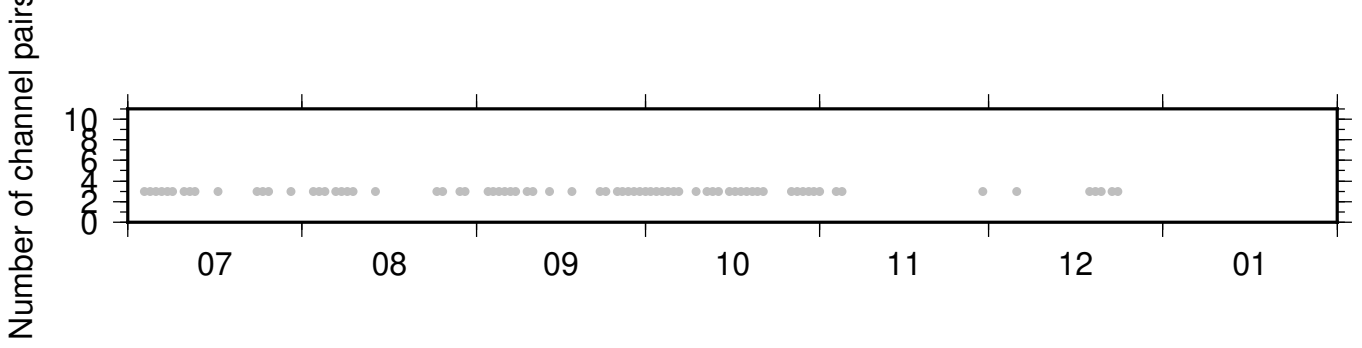
BK_HAYF_NC_KSM ZRT 0.10-0.90Hz 011
