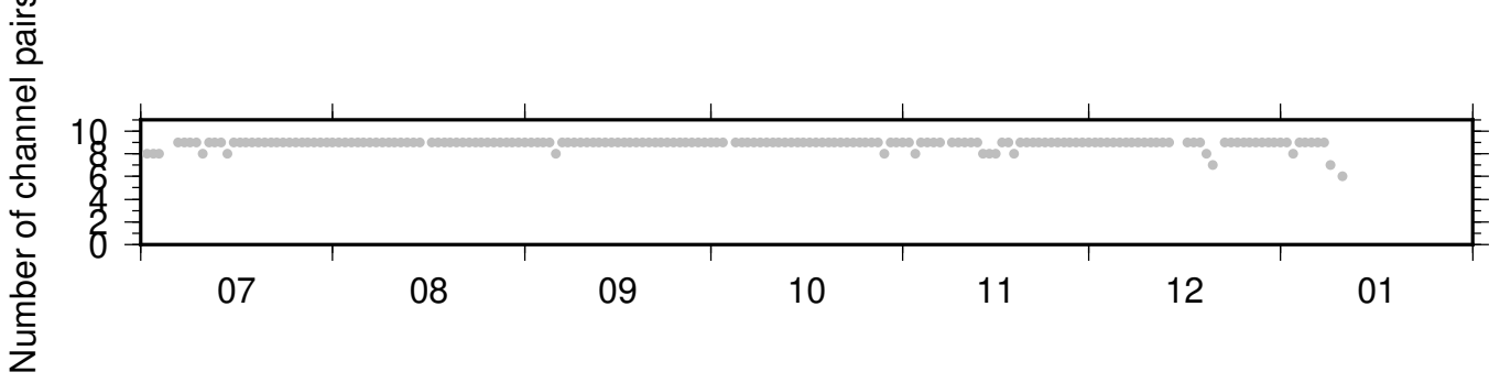
BK_HAYF_BK_PRDS ZRT 0.10-0.90Hz 011
