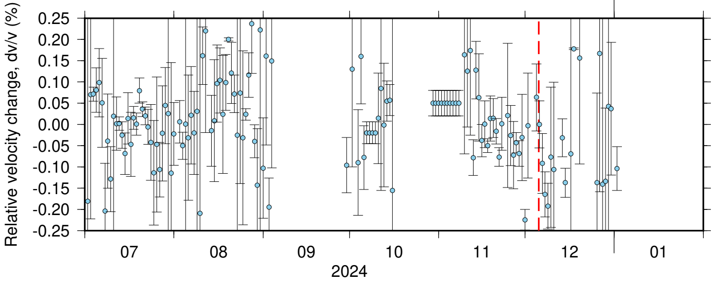
PB_B046_PB_B935 ZRT 0.10-0.90Hz 011
