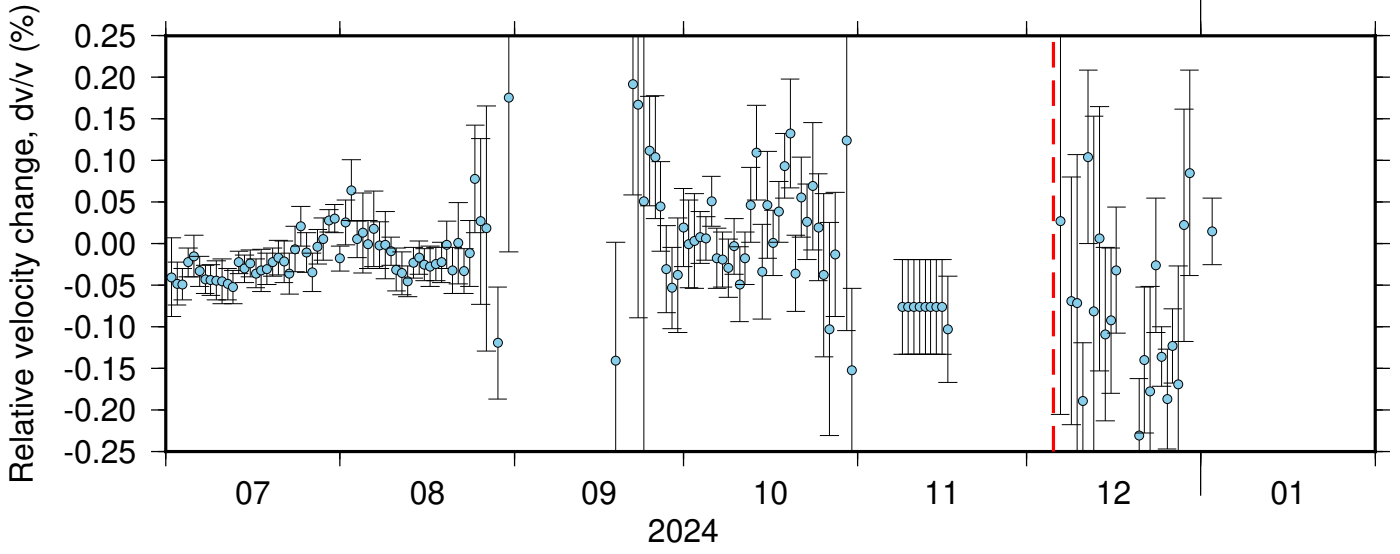
PB_B045_PB_B049 ZRT 0.10-0.90Hz 011
