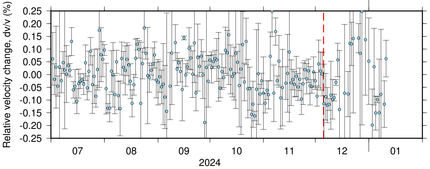
BK_BRIC_BK_KNEE ZRT 0.10-0.90Hz 011
