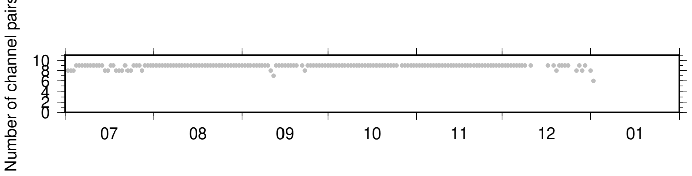
BK_WLKR_PB_B935 ZRT 0.10-0.90Hz 011
