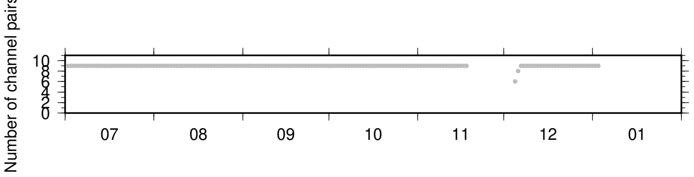
BK_BLAS_PB_B049 ZRT 0.10-0.90Hz 011
