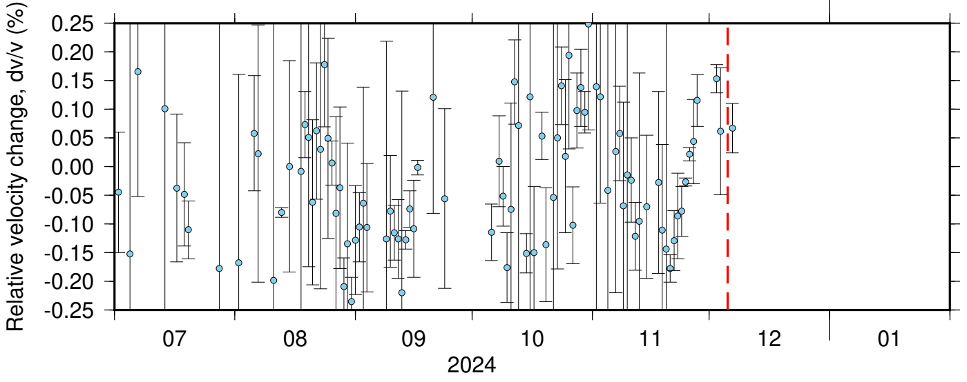
NC_KBU_PB_B934 ZRT 0.10-0.90Hz 011
