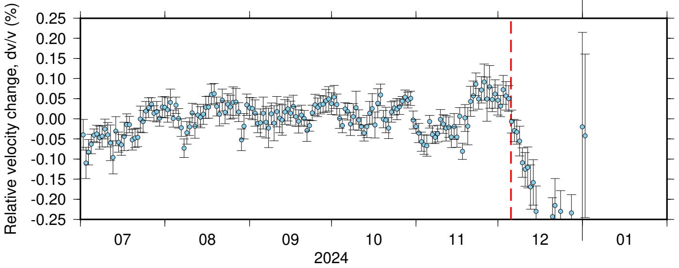
BK_PETL_PB_B047 ZRT 0.10-0.90Hz 011
