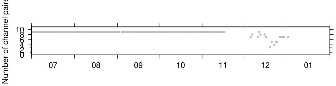
NC_KCT_PB_B049 ZRT 0.10-0.90Hz 011
