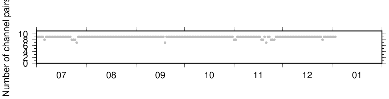
BK_PRDS_PB_B935 ZRT 0.10-0.90Hz 011
