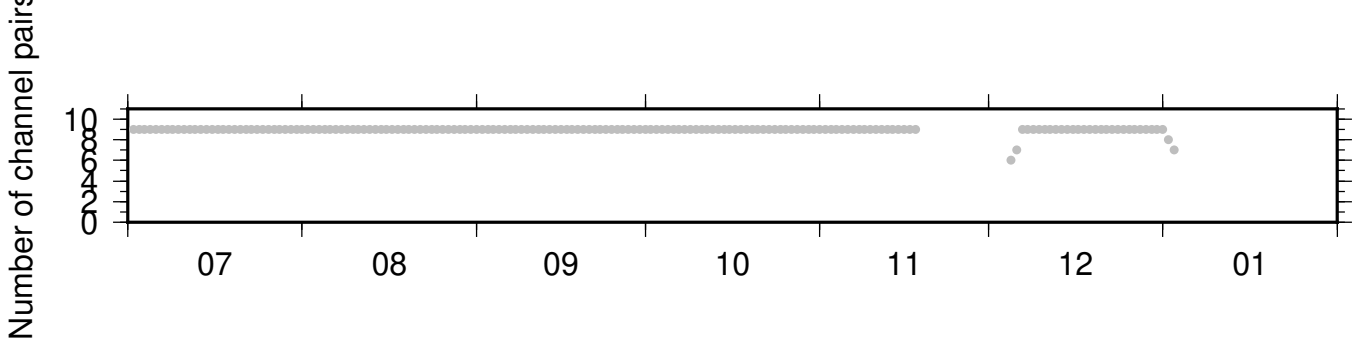
PB_B047_PB_B049 ZRT 0.10-0.90Hz 011
