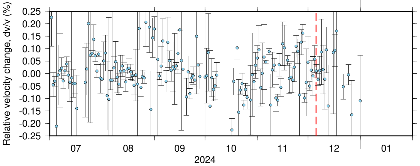
BK_JCC_PB_B934 ZRT 0.10-0.90Hz 011
