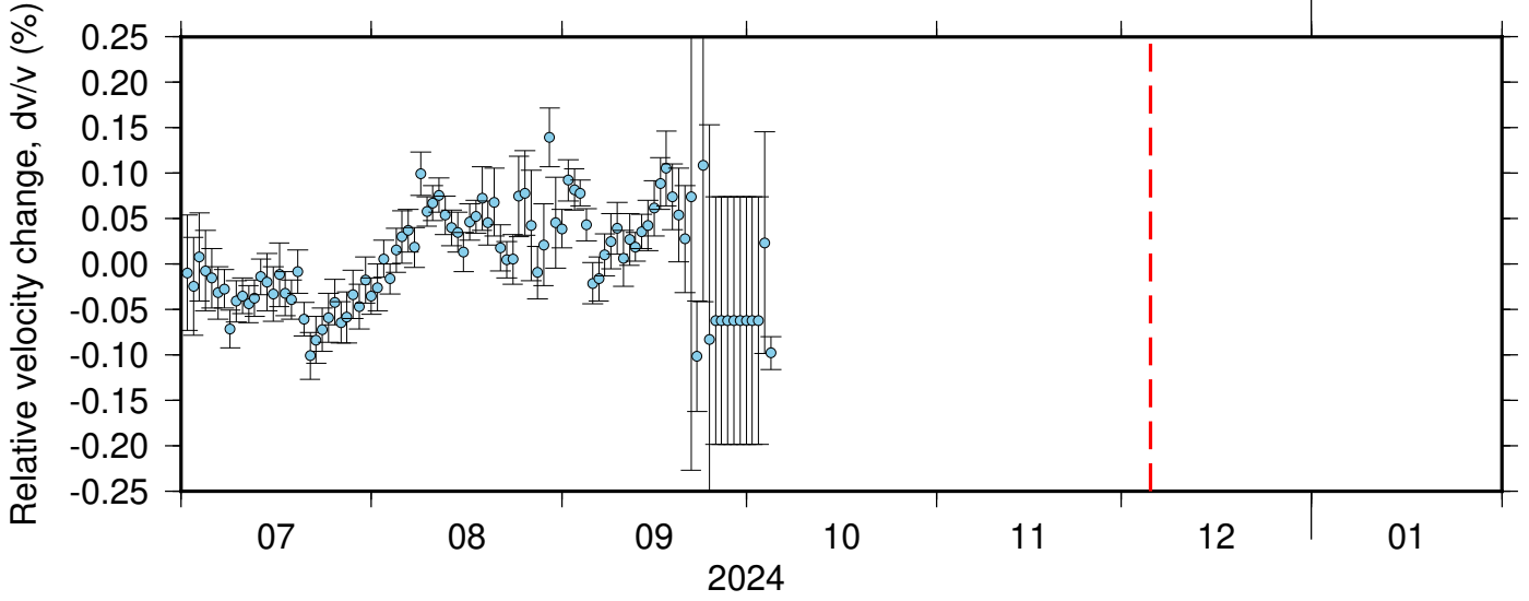
BK_GHOP_PB_B932 ZRT 0.10-0.90Hz 011
