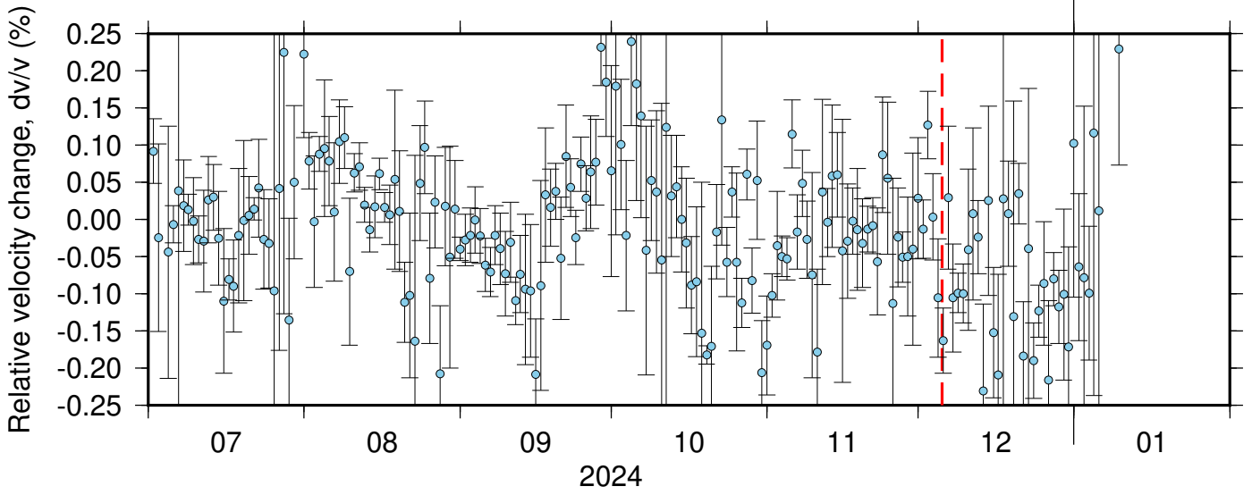
BK_GHOP_BK_KNEE ZRT 0.10-0.90Hz 011
