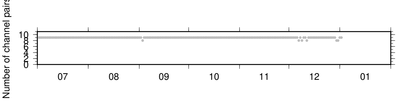
BK_BRIC_PB_B935 ZRT 0.10-0.90Hz 011
