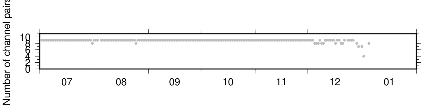
BK_JCC_BK_PETL ZRT 0.10-0.90Hz 011
