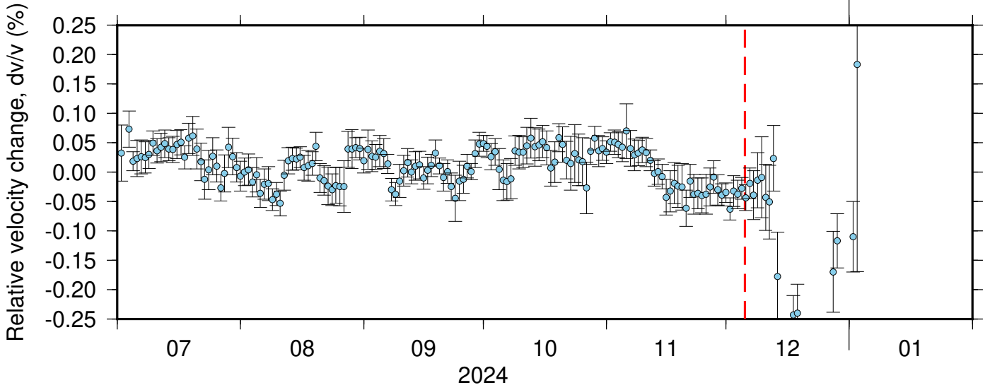
BK_PRDS_PB_B047 ZRT 0.10-0.90Hz 011
