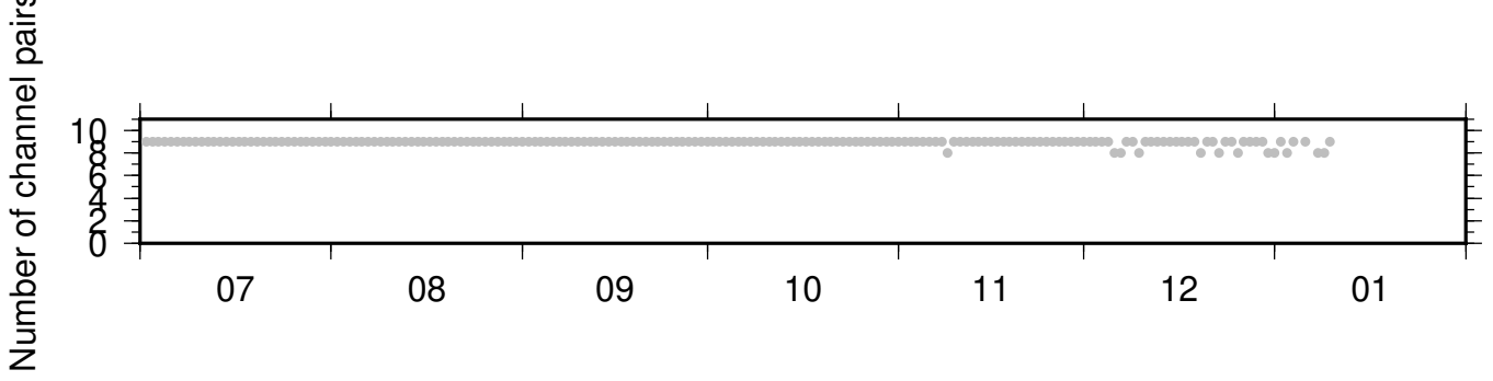
BK_BJES_BK_SPRL ZRT 0.10-0.90Hz 011
