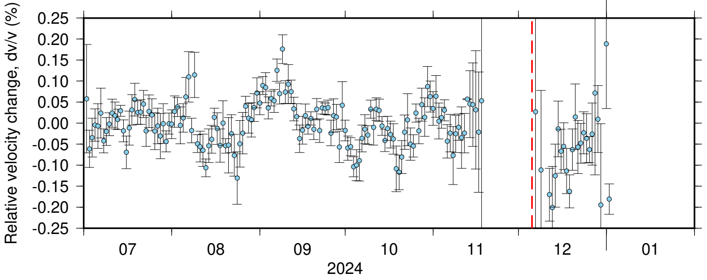
PB_B047_PB_B049 ZRT 0.10-0.90Hz 011
