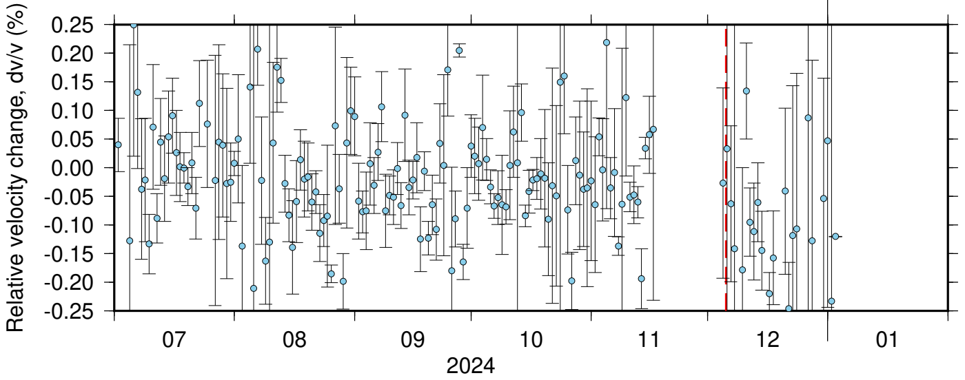
BK_HAYF_PB_B049 ZRT 0.10-0.90Hz 011
