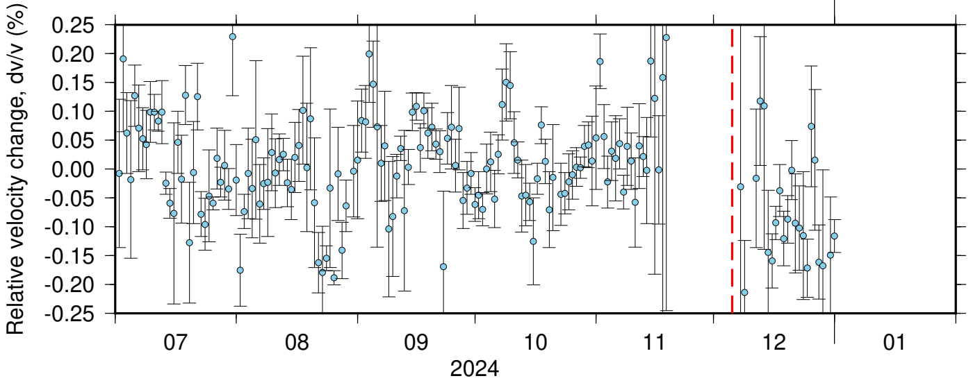
PB_B049_PB_B935 ZRT 0.10-0.90Hz 011
