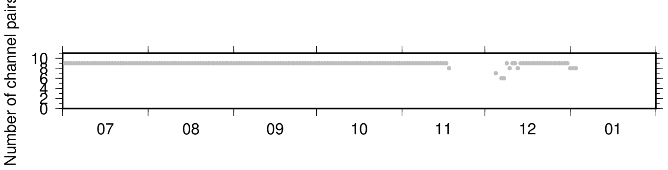
BK_WLKR_PB_B049 ZRT 0.10-0.90Hz 011
