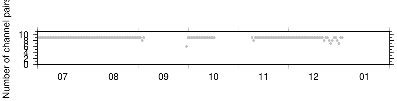
BK_BJES_PB_B046 ZRT 0.10-0.90Hz 011
