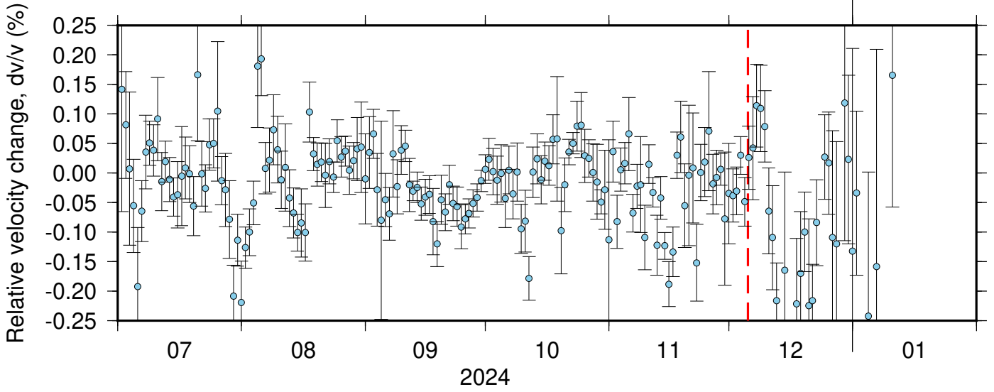
BK_PETL_BK_PRDS ZRT 0.10-0.90Hz 011
