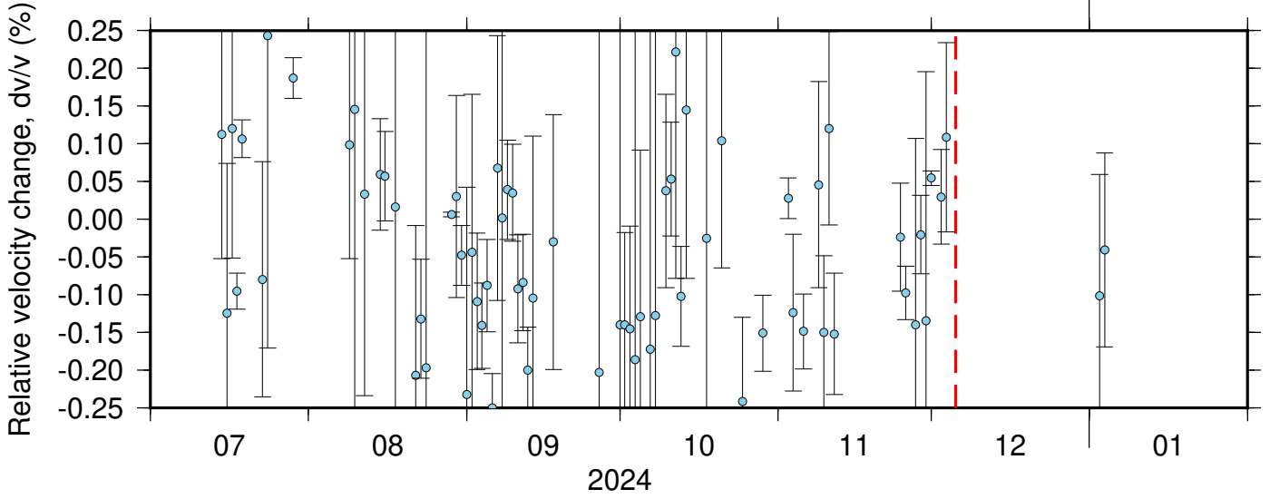
BK_WLKR_NC_KCR ZRT 0.10-0.90Hz 011
