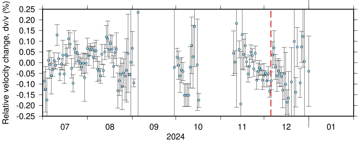
BK_BRIC_PB_B046 ZRT 0.10-0.90Hz 011
