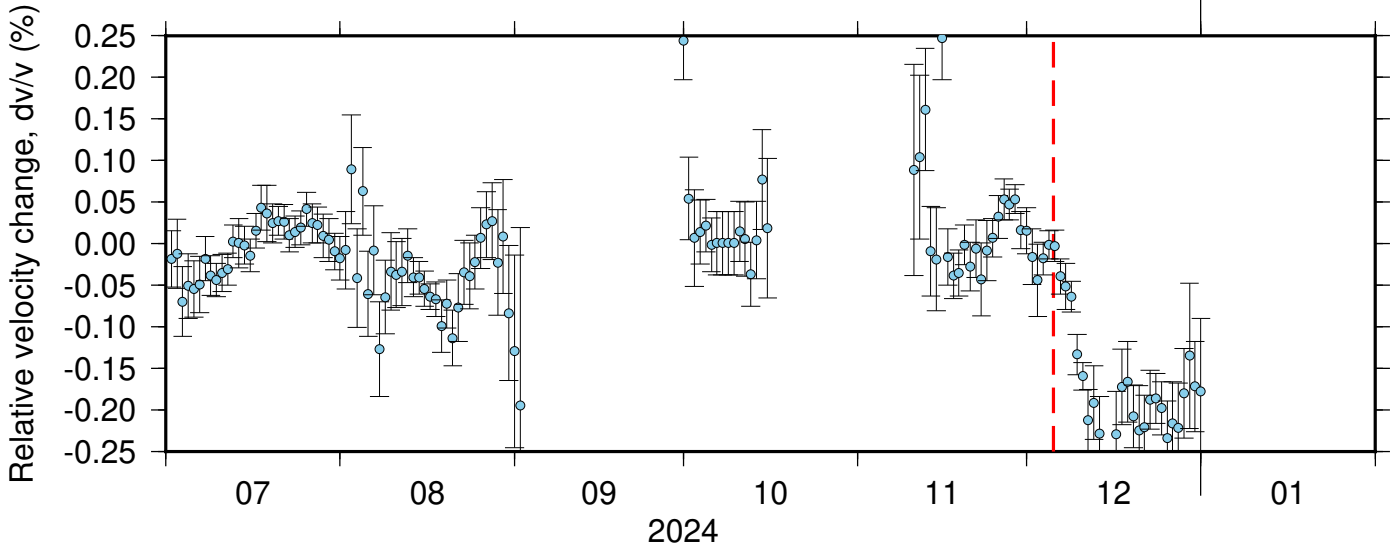
PB_B046_PB_B047 ZRT 0.10-0.90Hz 011
