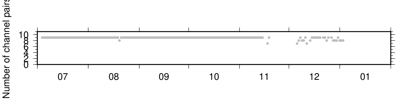
BK_KNEE_PB_B049 ZRT 0.10-0.90Hz 011
