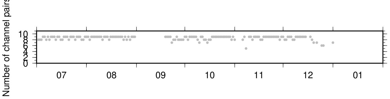
PB_B045_PB_B934 ZRT 0.10-0.90Hz 011
