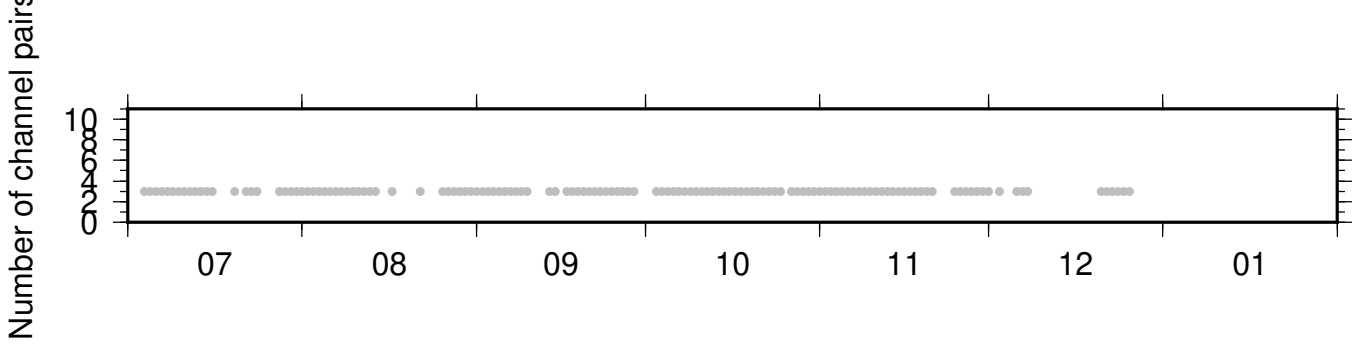
BK_HAYF_NC_KPR ZRT 0.10-0.90Hz 011
