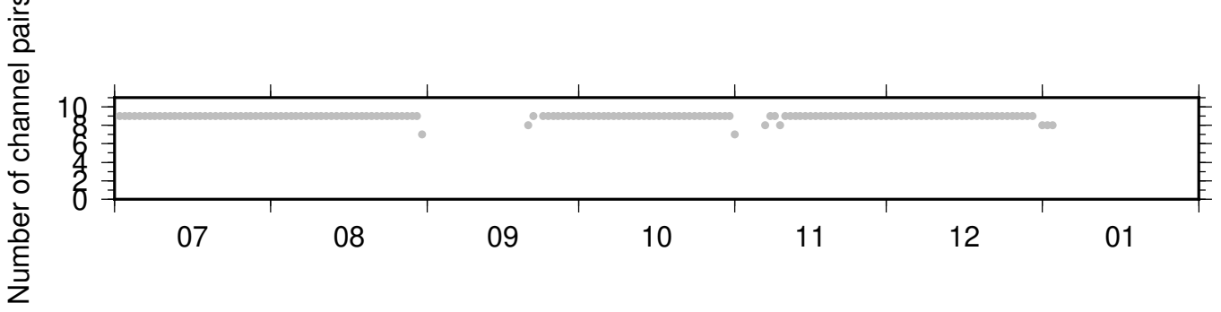
BK_SPRL_PB_B045 ZRT 0.10-0.90Hz 011
