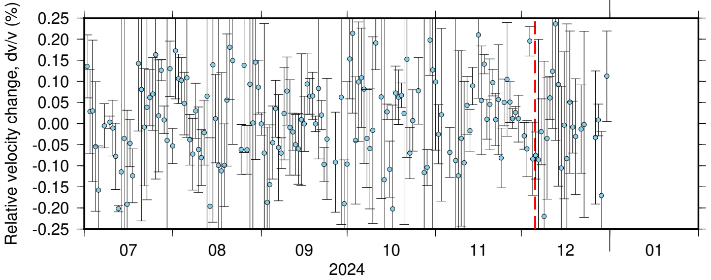
BK_PETL_PB_B935 ZRT 0.10-0.90Hz 011
