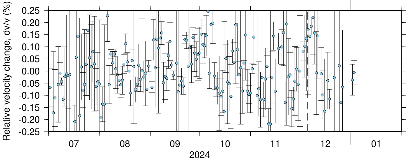
BK_BJES_PB_B934 ZRT 0.10-0.90Hz 011
