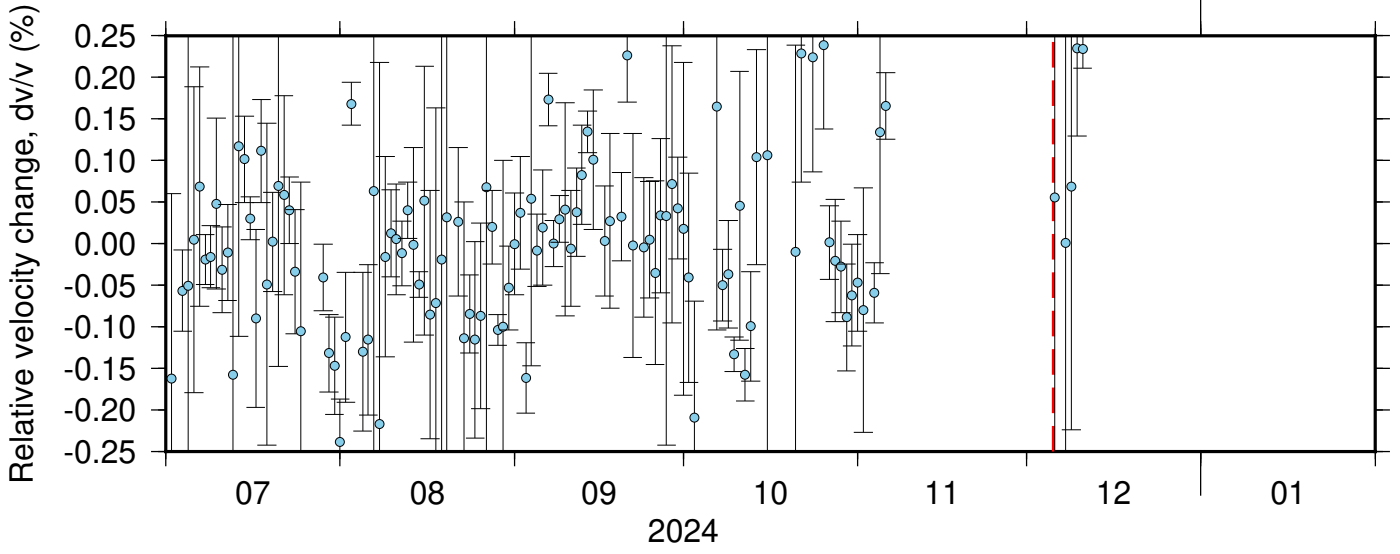
NC_KCT_NC_KSM ZRT 0.10-0.90Hz 011
