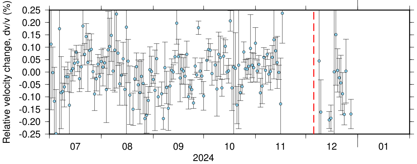
BK_PETL_PB_B049 ZRT 0.10-0.90Hz 011
