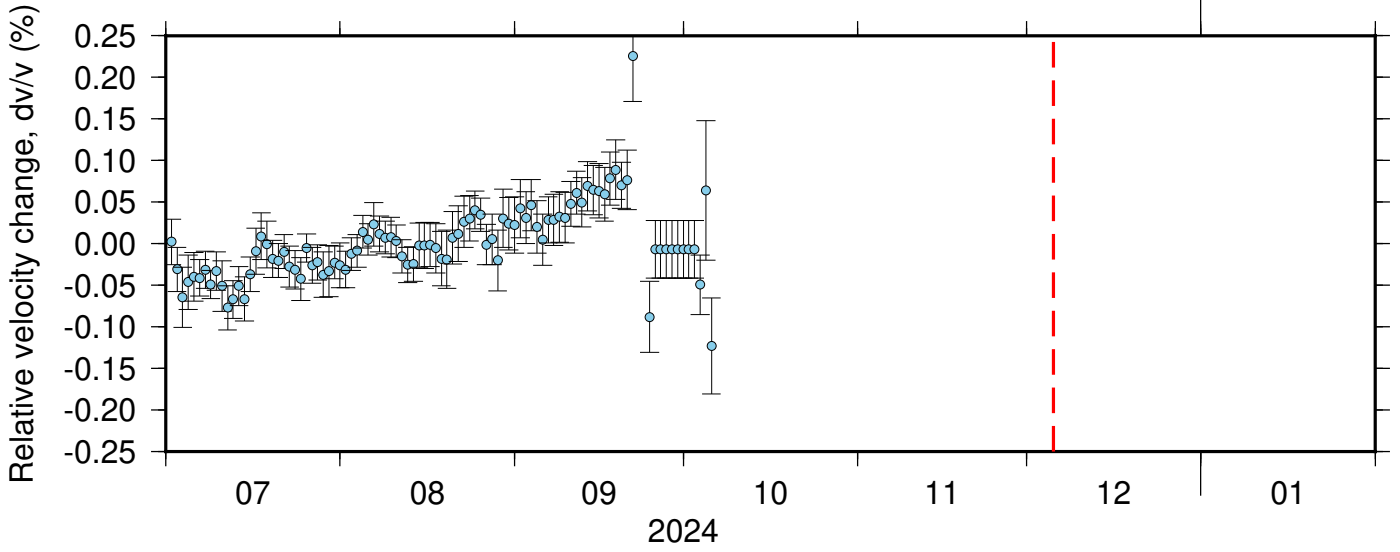
PB_B047_PB_B932 ZRT 0.10-0.90Hz 011
