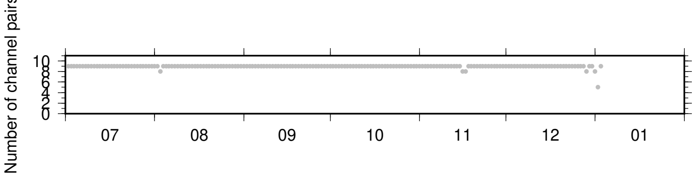
BK_SPRL_PB_B935 ZRT 0.10-0.90Hz 011
