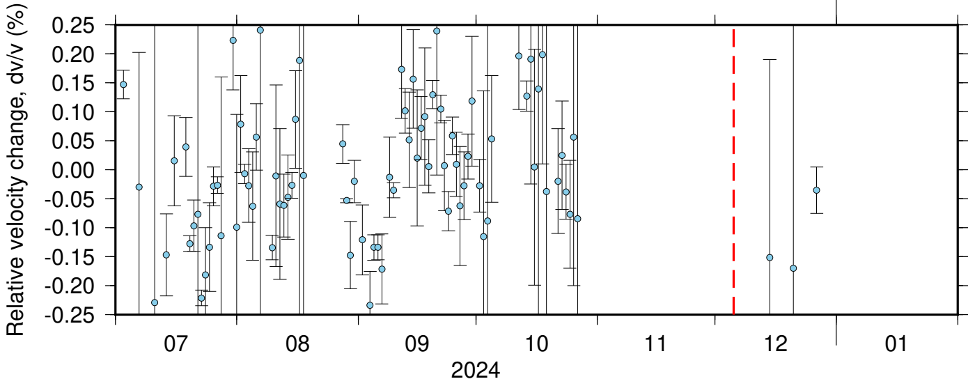
NC_KSM_PB_B934 ZRT 0.10-0.90Hz 011
