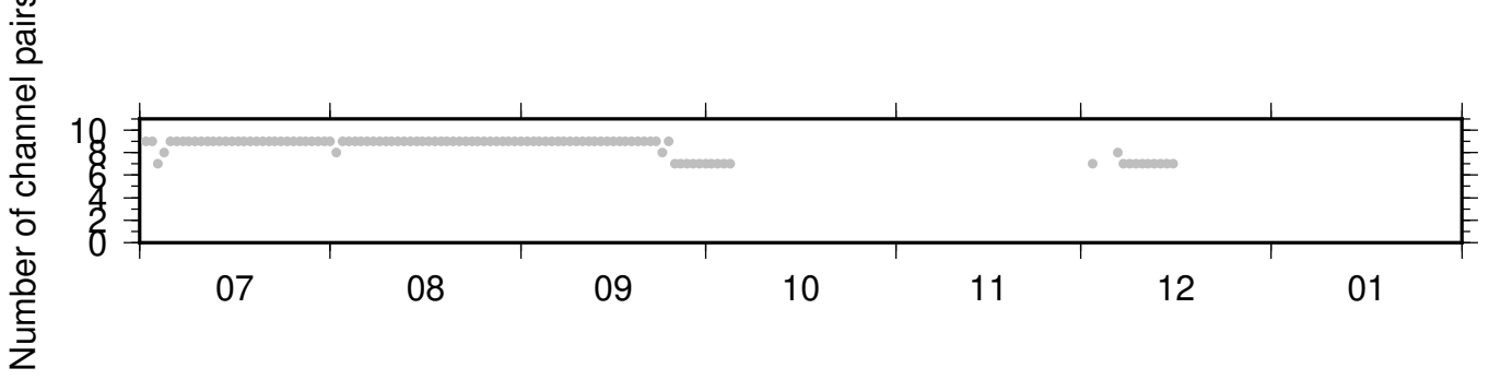
PB_B932_PB_B935 ZRT 0.10-0.90Hz 011
