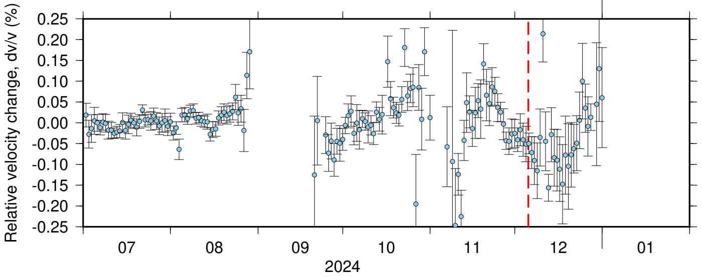
BK_BJES_PB_B045 ZRT 0.10-0.90Hz 011
