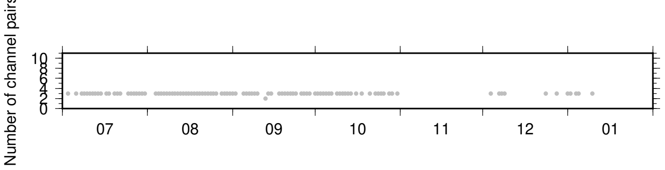
BK_KNEE_NC_KSM ZRT 0.10-0.90Hz 011
