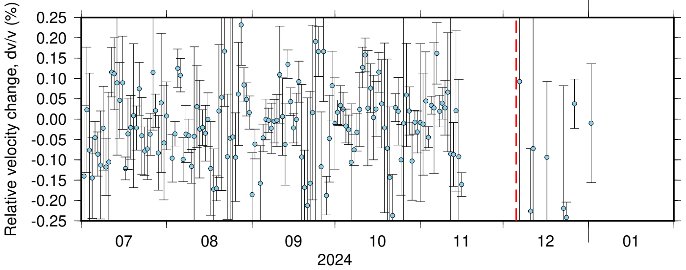
NC_KCT_PB_B049 ZRT 0.10-0.90Hz 011
