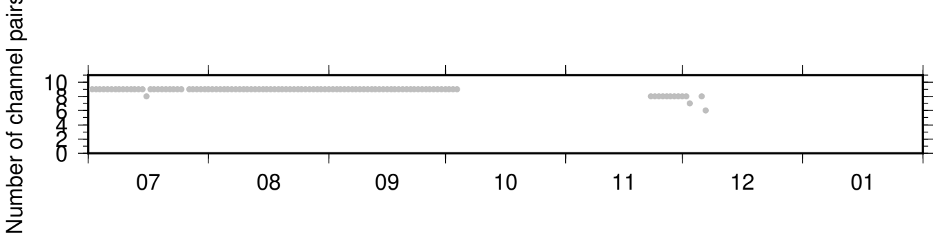
BK_JCC_PB_B932 ZRT 0.10-0.90Hz 011
