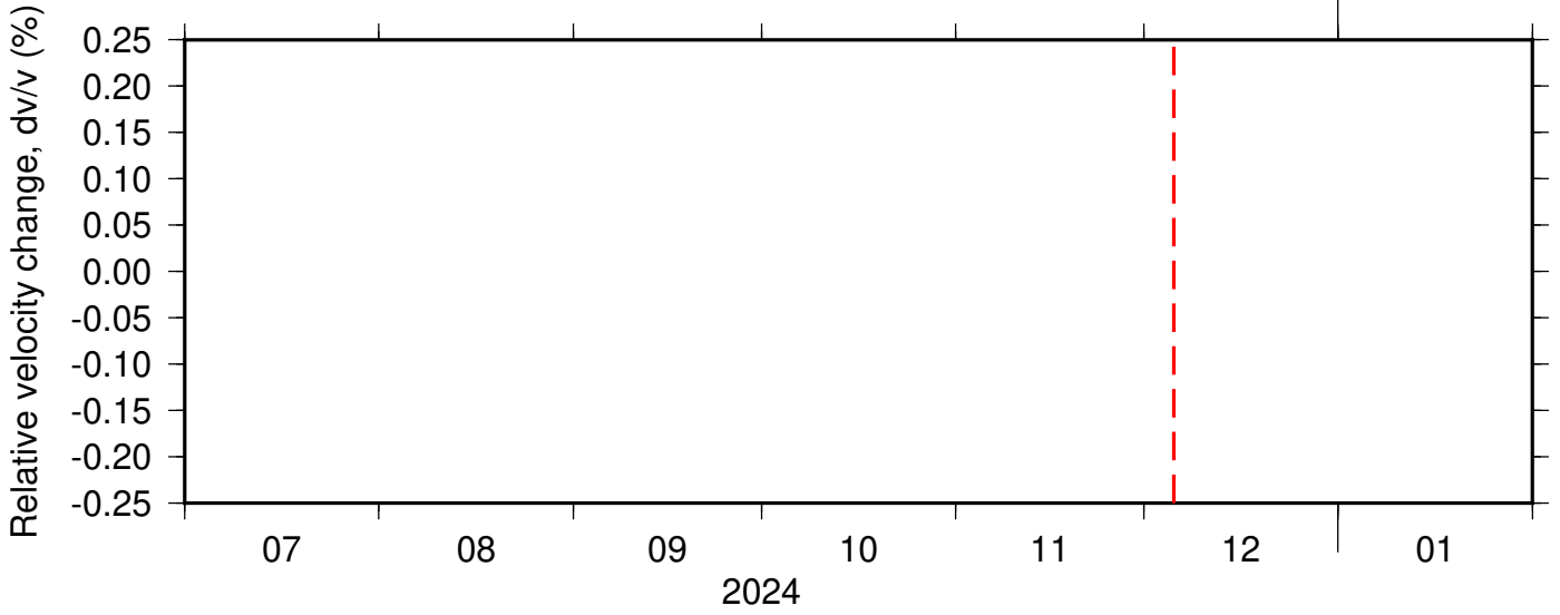
NC_KBU_NC_KSM ZRT 0.10-0.90Hz 011
