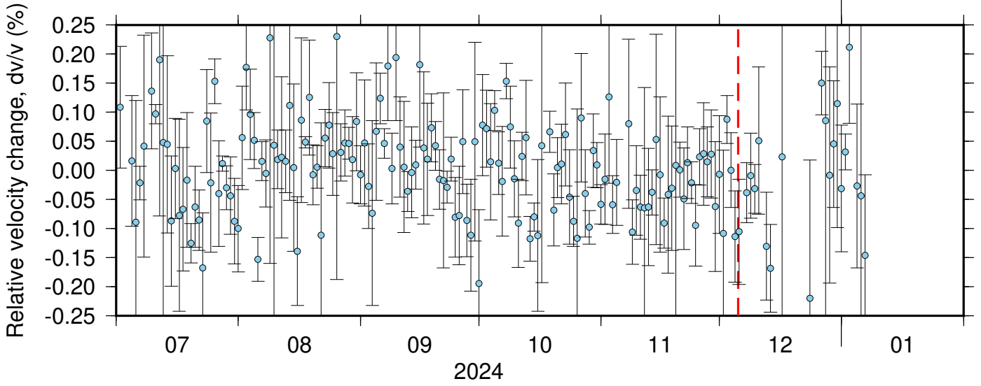
BK_WLKR_NC_KMR ZRT 0.10-0.90Hz 011
