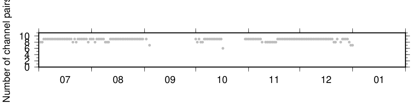
BK_HAYF_PB_B046 ZRT 0.10-0.90Hz 011
