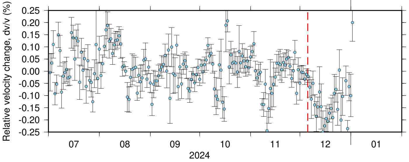
BK_HAYF_PB_B935 ZRT 0.10-0.90Hz 011
