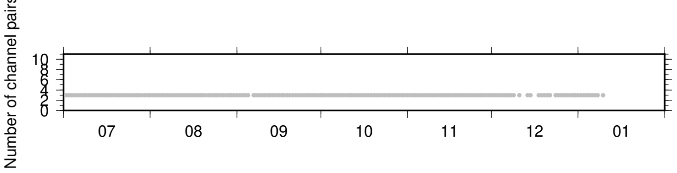
BK_WLKR_NC_KBU ZRT 0.10-0.90Hz 011
