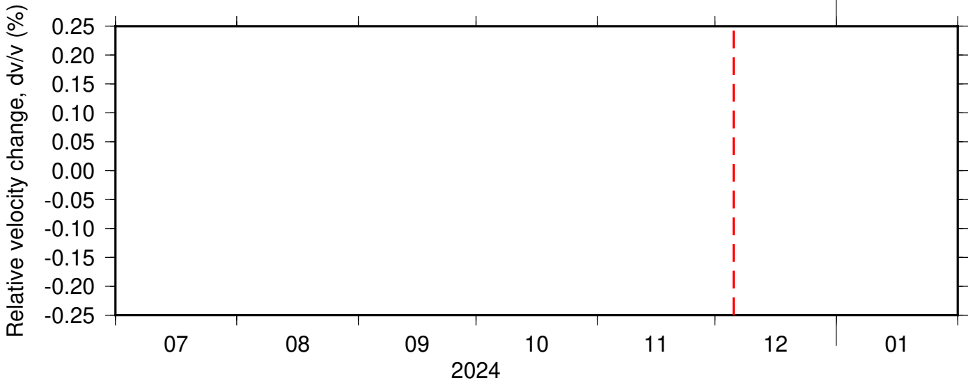
NC_KPR_NC_KSM ZRT 0.10-0.90Hz 011
