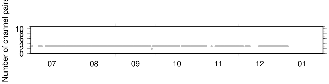
BK_BLAS_NC_KPR ZRT 0.10-0.90Hz 011
