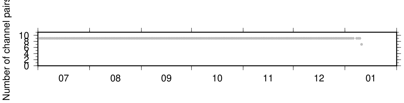
BK_GHOP_BK_KNEE ZRT 0.10-0.90Hz 011
