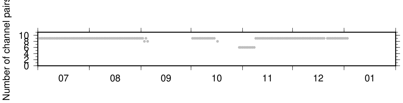
BK_SPRL_PB_B046 ZRT 0.10-0.90Hz 011
