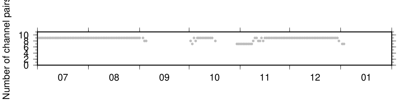
BK_BLAS_PB_B046 ZRT 0.10-0.90Hz 011
