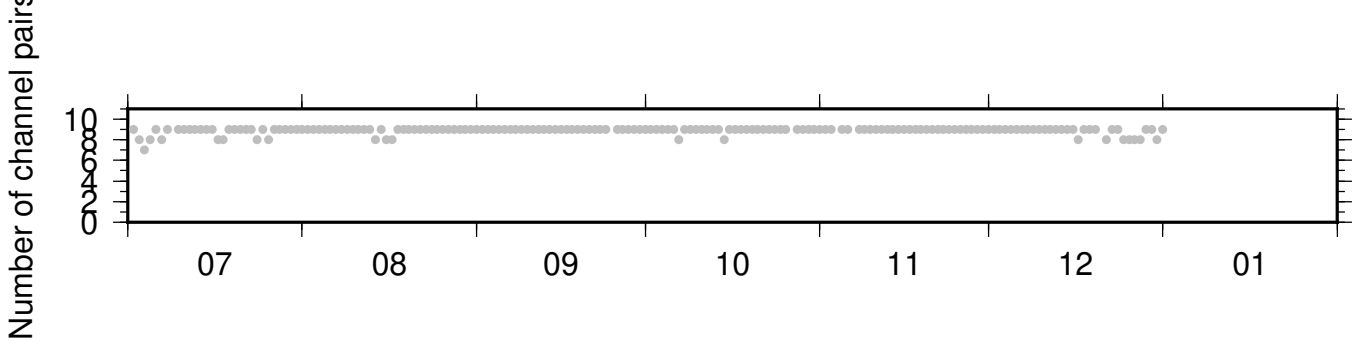
BK_PETL_PB_B935 ZRT 0.10-0.90Hz 011
