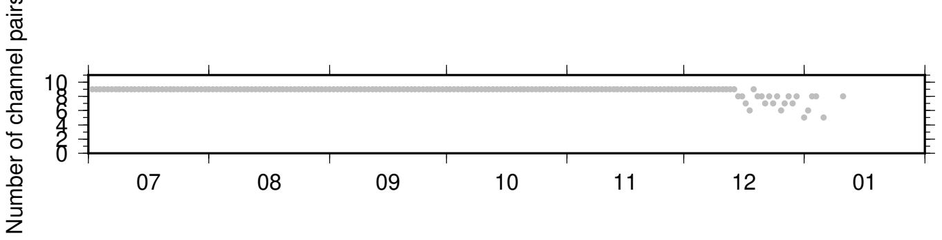
BK_PETL_NC_KCT ZRT 0.10-0.90Hz 011
