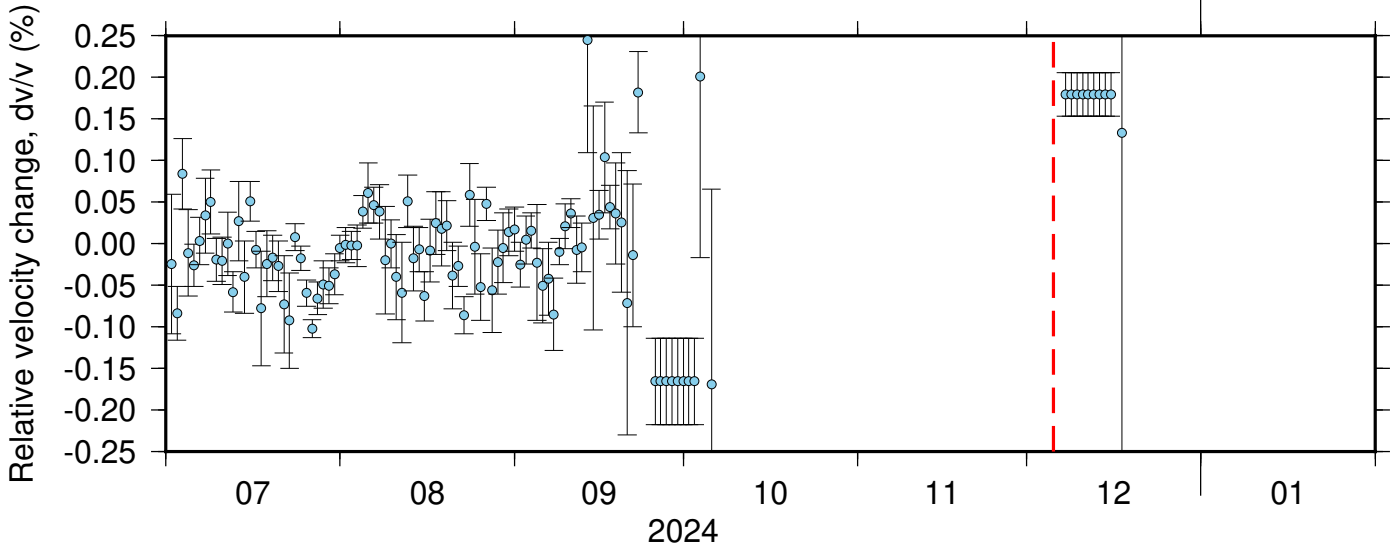
BK_BRIC_PB_B932 ZRT 0.10-0.90Hz 011
