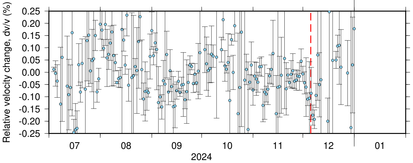
BK_PETL_PB_B934 ZRT 0.10-0.90Hz 011
