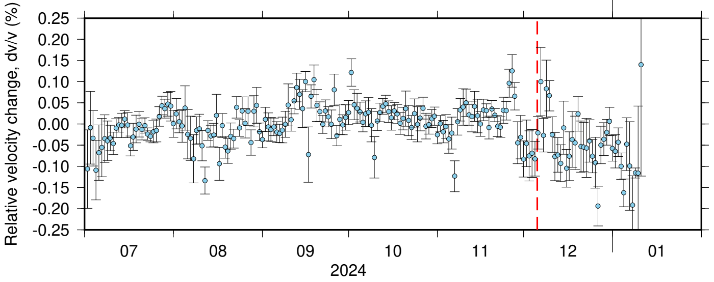
BK_BJES_BK_GHOP ZRT 0.10-0.90Hz 011
