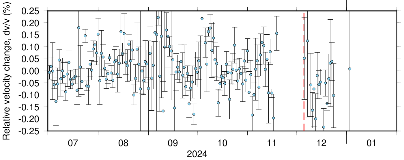
PB_B049_PB_B934 ZRT 0.10-0.90Hz 011
