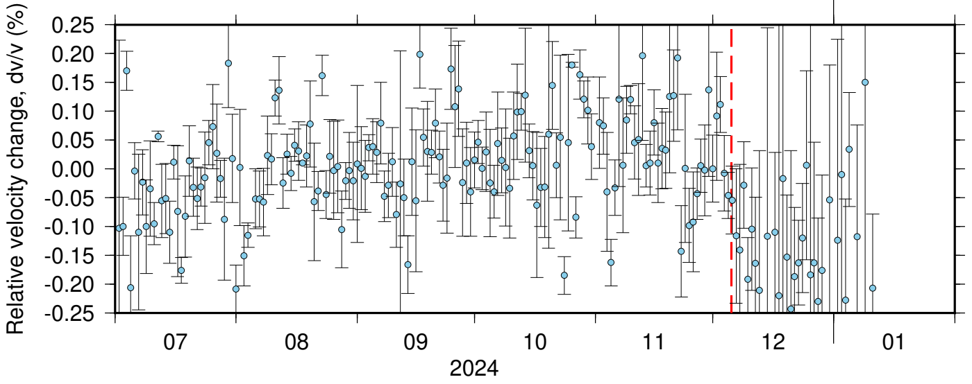
BK_BJES_BK_WLKR ZRT 0.10-0.90Hz 011
