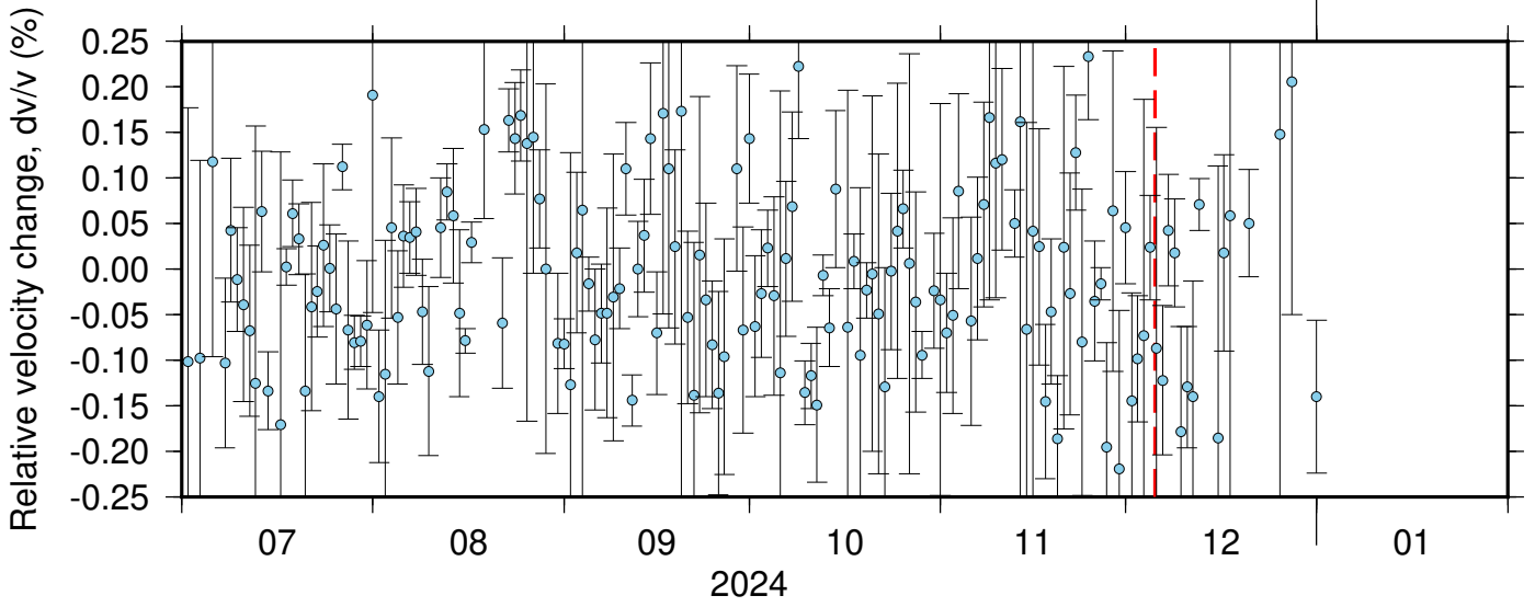
PB_B934_PB_B935 ZRT 0.10-0.90Hz 011
