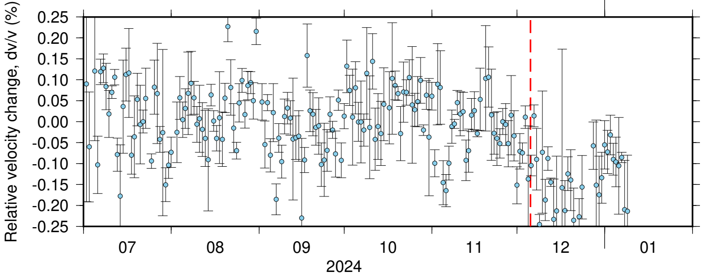
NC_KBU_NC_KMPB ZRT 0.10-0.90Hz 011
