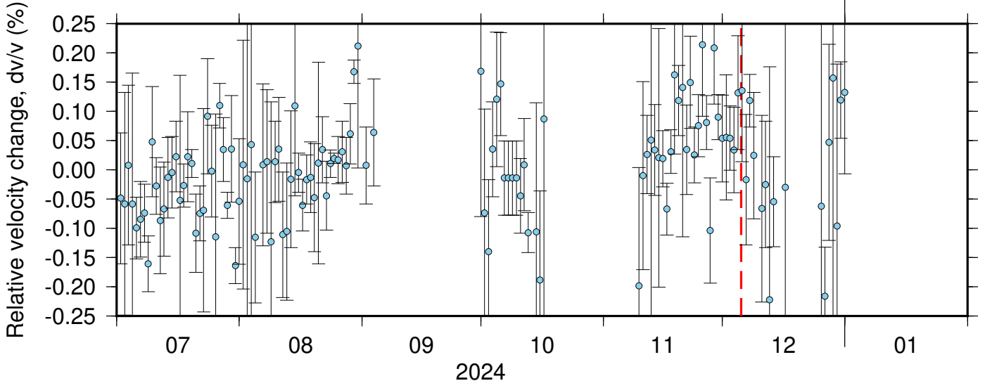
BK_KNEE_PB_B046 ZRT 0.10-0.90Hz 011
