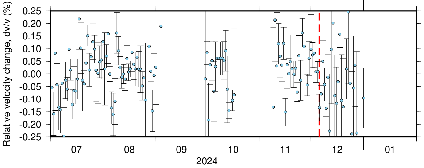
BK_BJES_PB_B046 ZRT 0.10-0.90Hz 011
