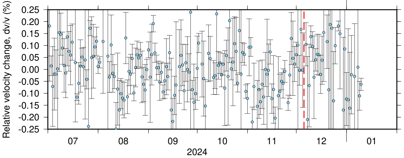
BK_KNEE_BK_WLKR ZRT 0.10-0.90Hz 011
