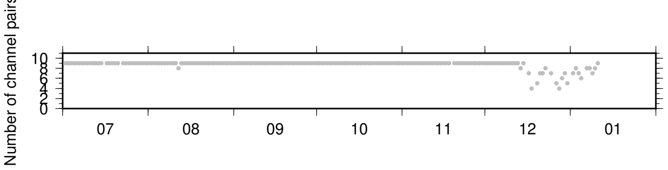
BK_BLAS_NC_KCT ZRT 0.10-0.90Hz 011
