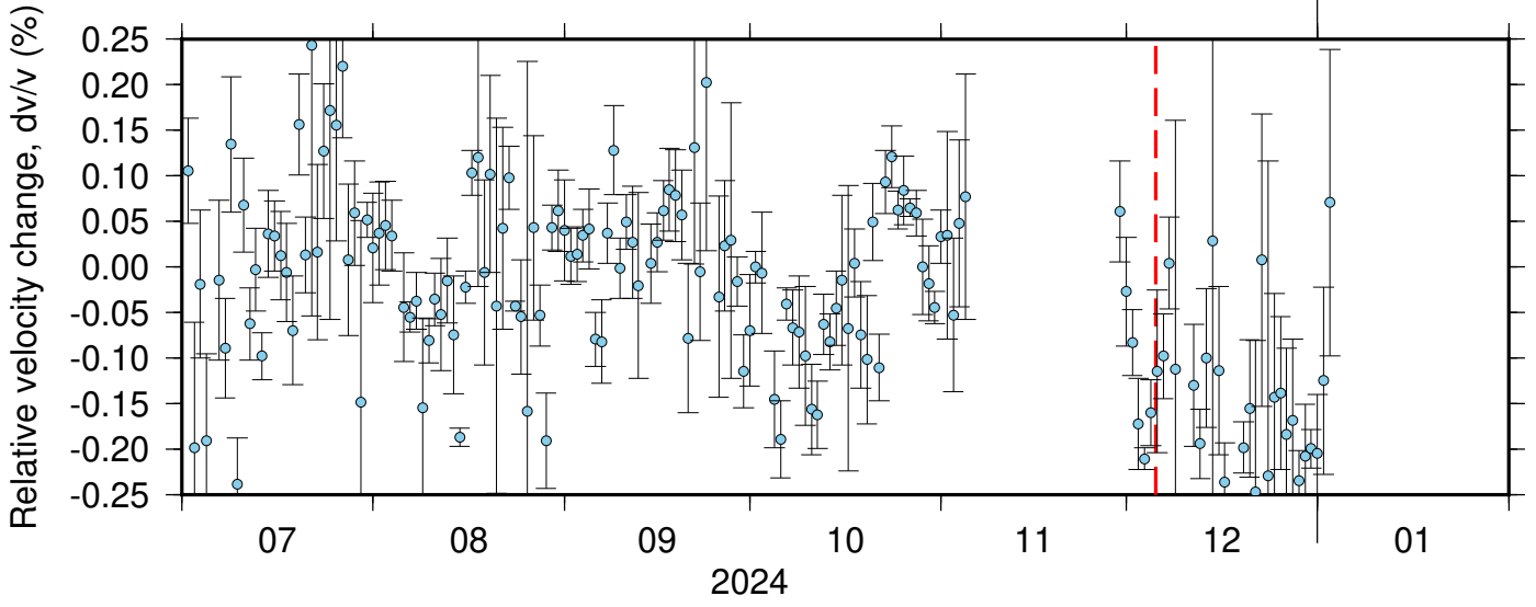
BK_WLKR_NC_KSM ZRT 0.10-0.90Hz 011
