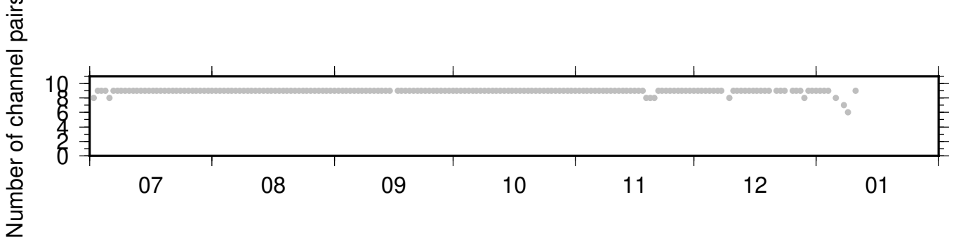
BK_JCC_BK_WLKR ZRT 0.10-0.90Hz 011
