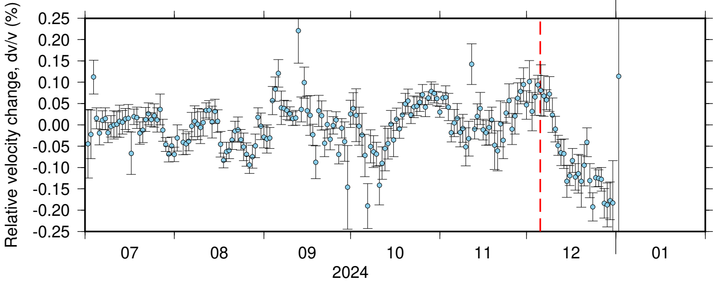
BK_BRIC_PB_B047 ZRT 0.10-0.90Hz 011
