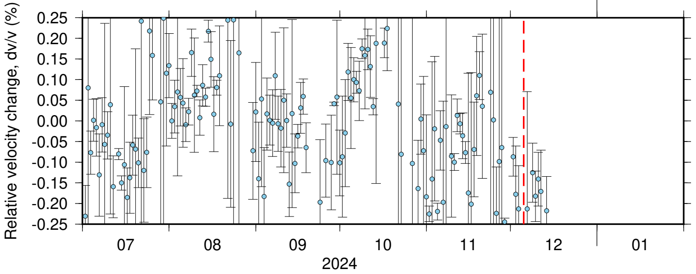
NC_KCT_NC_KPR ZRT 0.10-0.90Hz 011
