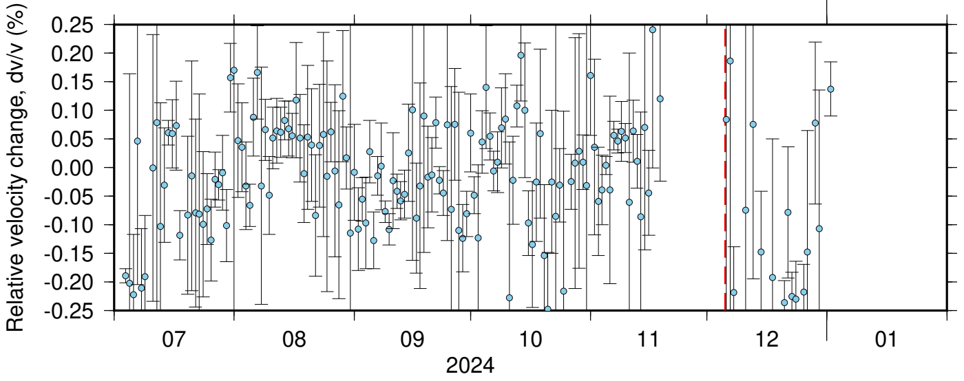
BK_JCC_PB_B049 ZRT 0.10-0.90Hz 011
