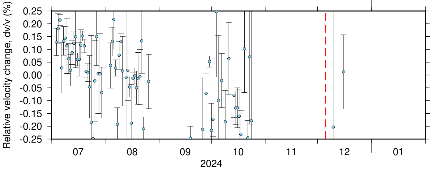
NC_KSM_PB_B045 ZRT 0.10-0.90Hz 011
