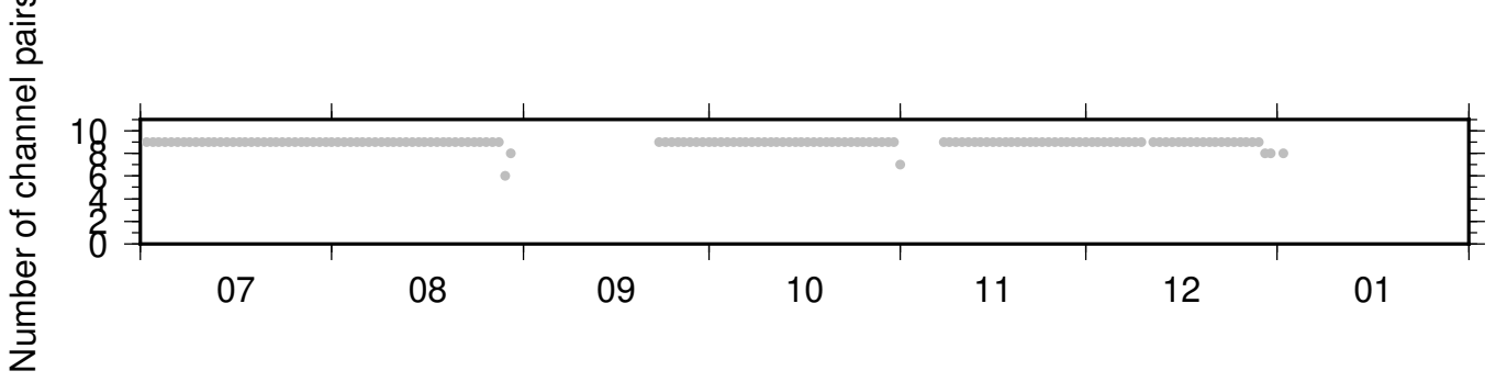
NC_KMR_PB_B045 ZRT 0.10-0.90Hz 011
