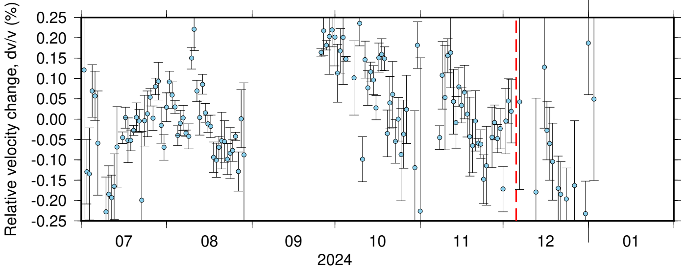
NC_KCR_PB_B045 ZRT 0.10-0.90Hz 011
