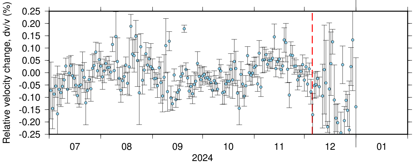
BK_BJES_PB_B935 ZRT 0.10-0.90Hz 011
