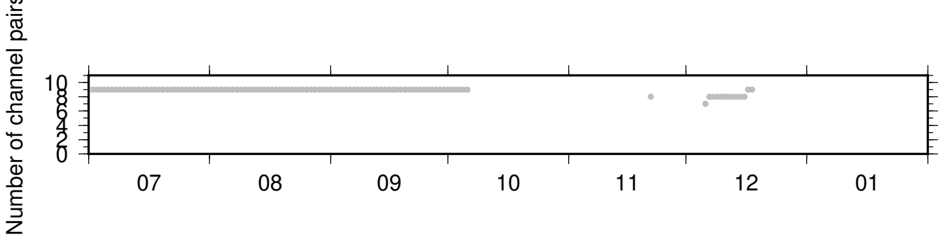
NC_KMPB_PB_B932 ZRT 0.10-0.90Hz 011
