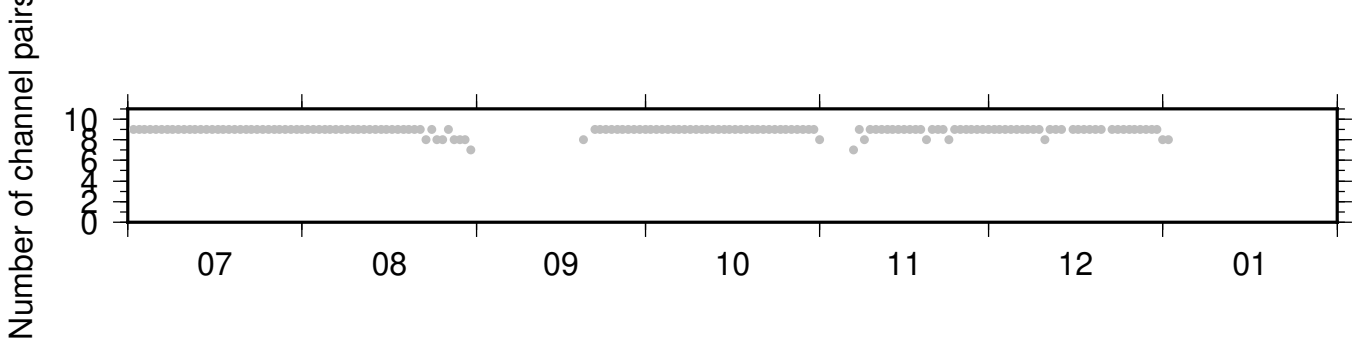
PB_B045_PB_B935 ZRT 0.10-0.90Hz 011
