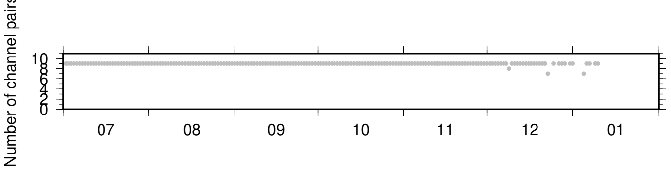
BK_BLAS_BK_WLKR ZRT 0.10-0.90Hz 011
