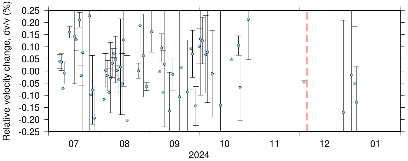
BK_KNEE_NC_KSM ZRT 0.10-0.90Hz 011
