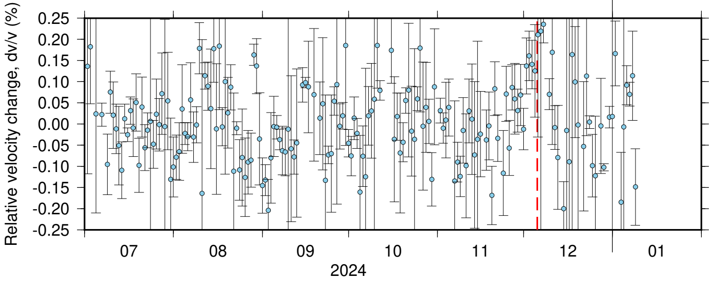
BK_KNEE_BK_SPRL ZRT 0.10-0.90Hz 011
