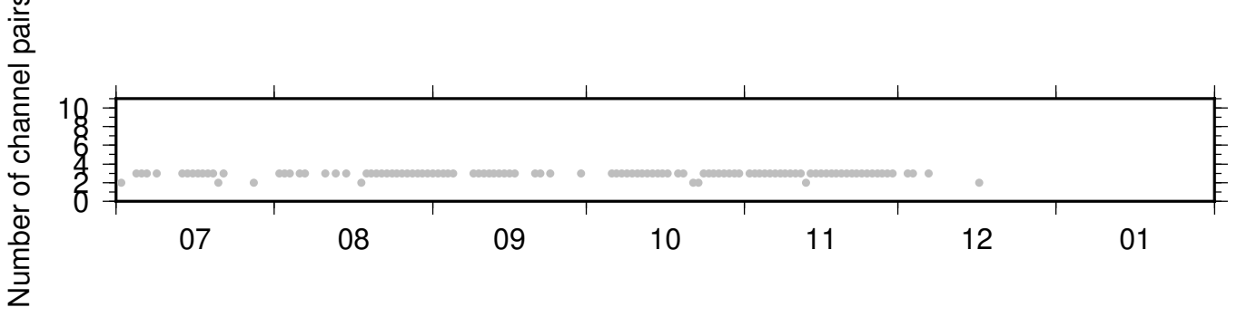
NC_KBU_PB_B934 ZRT 0.10-0.90Hz 011
