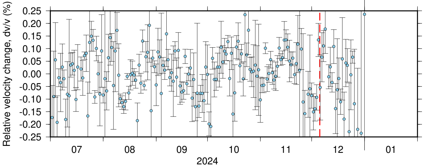
BK_BLAS_PB_B934 ZRT 0.10-0.90Hz 011
