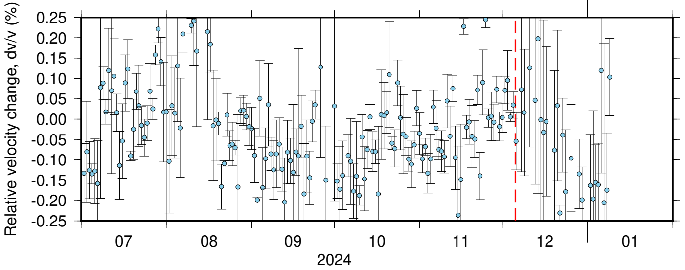
BK_WLKR_NC_KPR ZRT 0.10-0.90Hz 011
