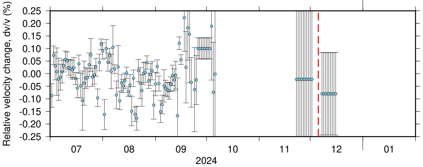
BK_SPRL_PB_B932 ZRT 0.10-0.90Hz 011
