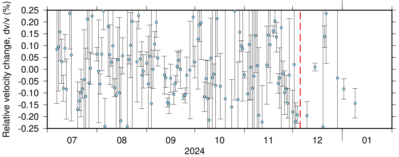
BK_KNEE_NC_KCR ZRT 0.10-0.90Hz 011
