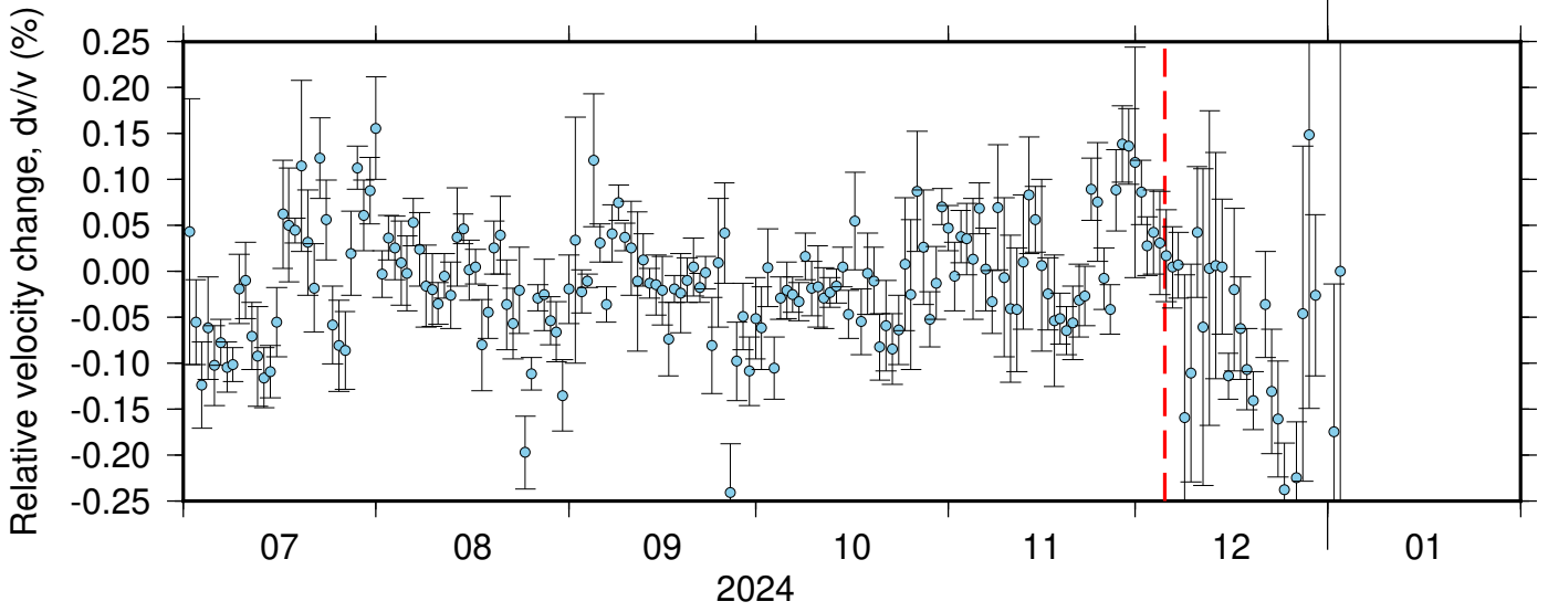
NC_KMR_PB_B047 ZRT 0.10-0.90Hz 011
