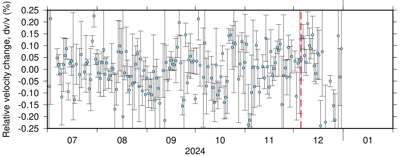
BK_HAYF_PB_B047 ZRT 0.10-0.90Hz 011
