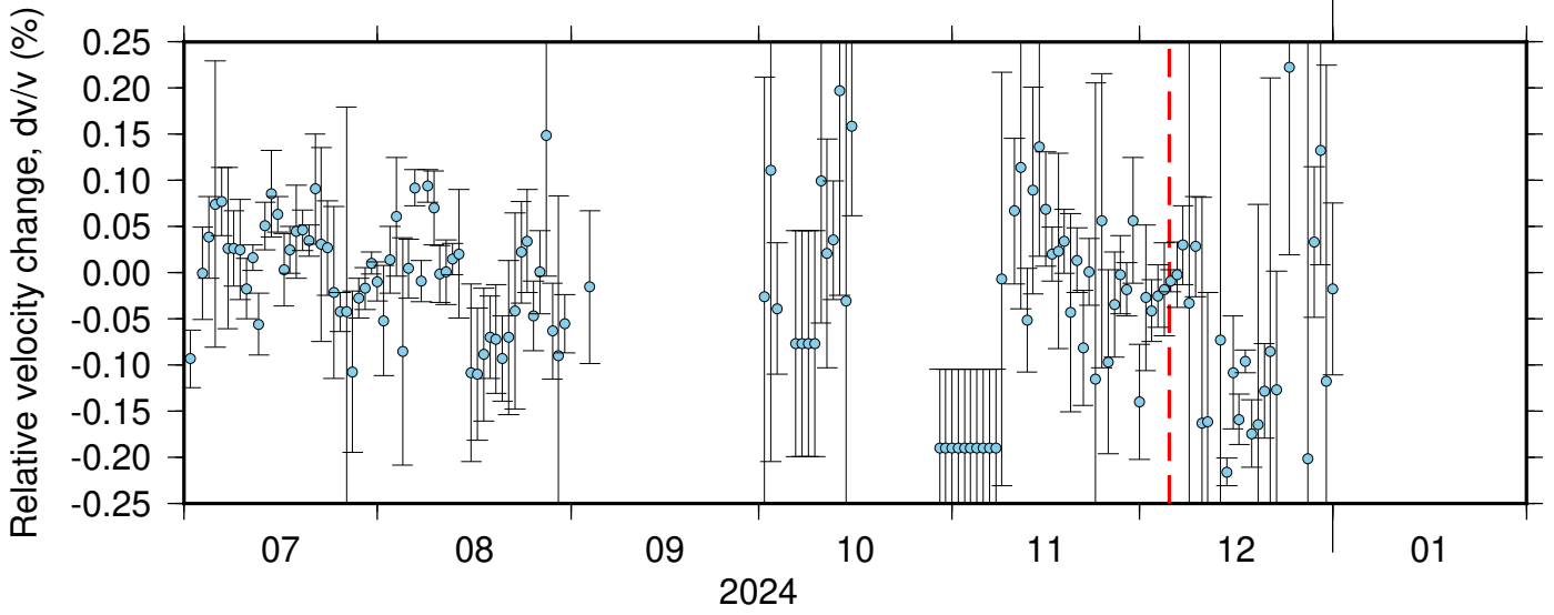
BK_HAYF_PB_B046 ZRT 0.10-0.90Hz 011
