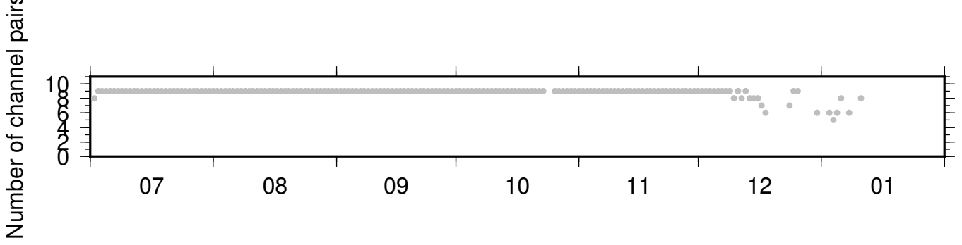
BK_BRIC_NC_KCT ZRT 0.10-0.90Hz 011
