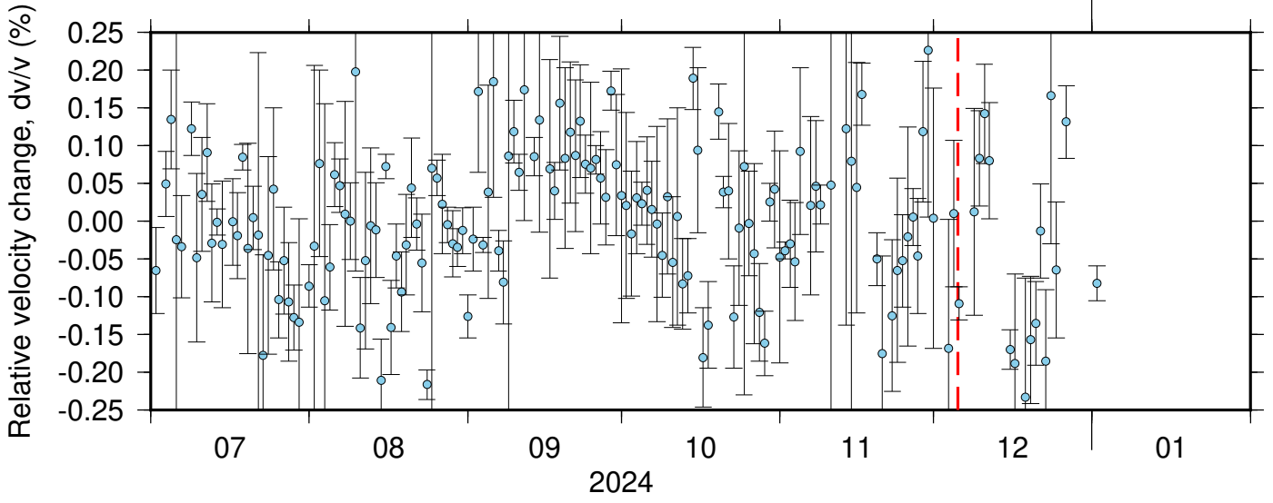
BK_KNEE_PB_B934 ZRT 0.10-0.90Hz 011
