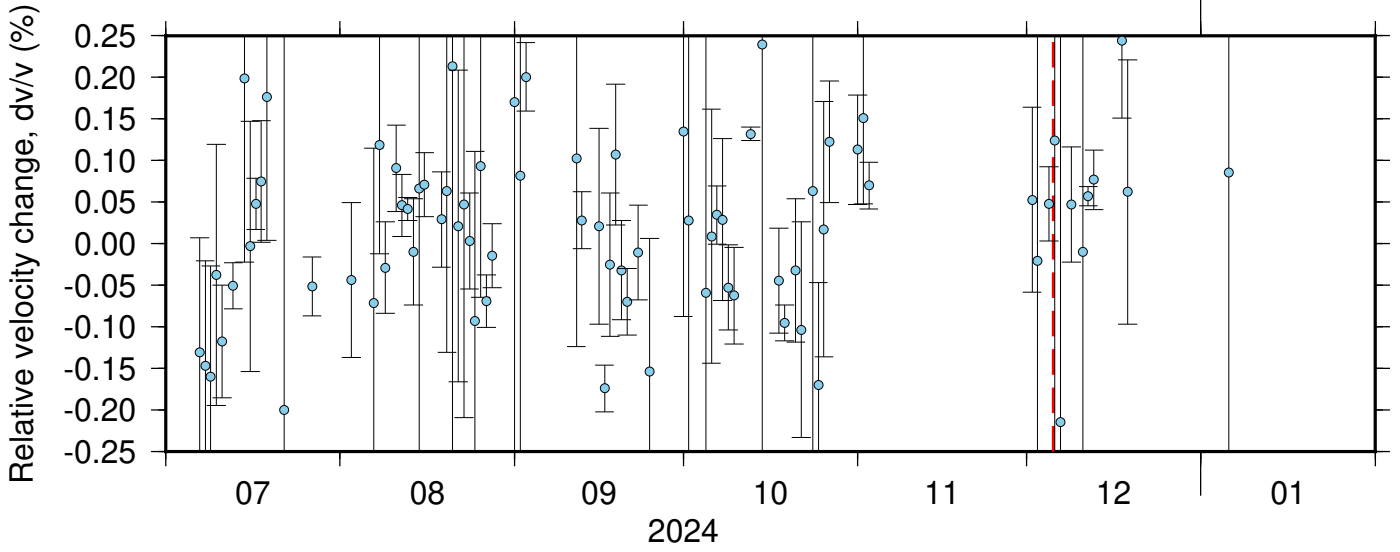
BK_BLAS_NC_KSM ZRT 0.10-0.90Hz 011
