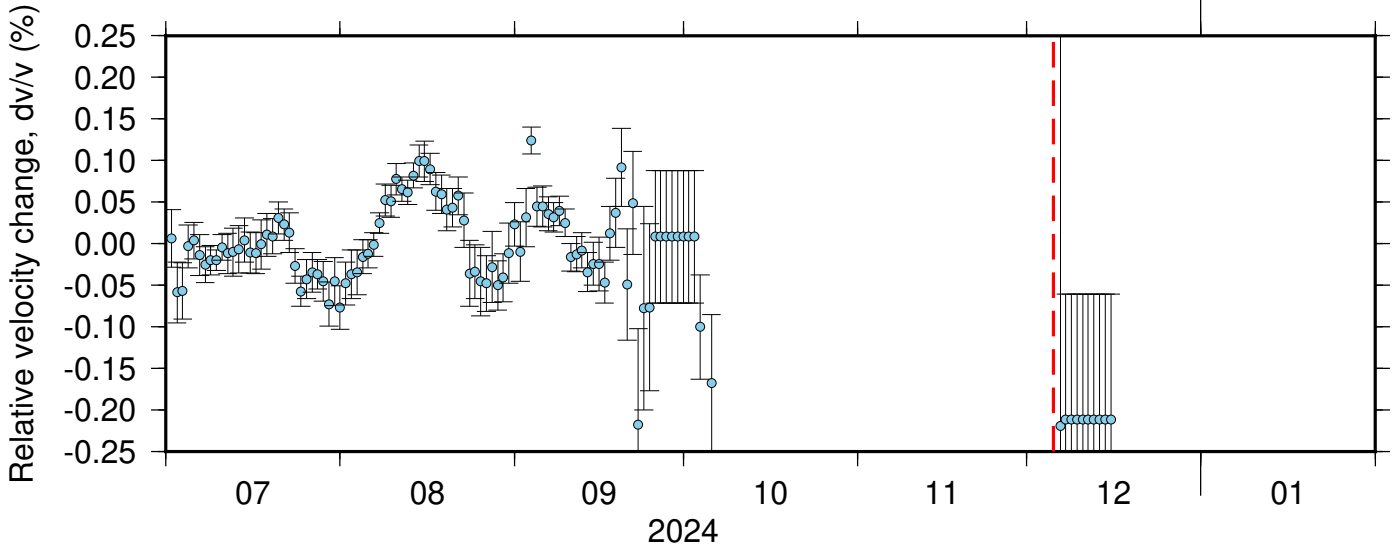
BK_PETL_PB_B932 ZRT 0.10-0.90Hz 011
