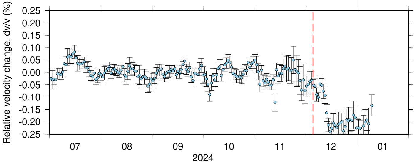
BK_BRIC_BK_PRDS ZRT 0.10-0.90Hz 011
