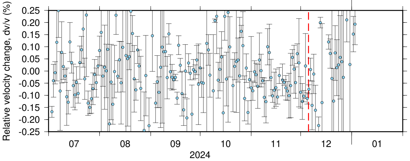
BK_JCC_PB_B047 ZRT 0.10-0.90Hz 011
