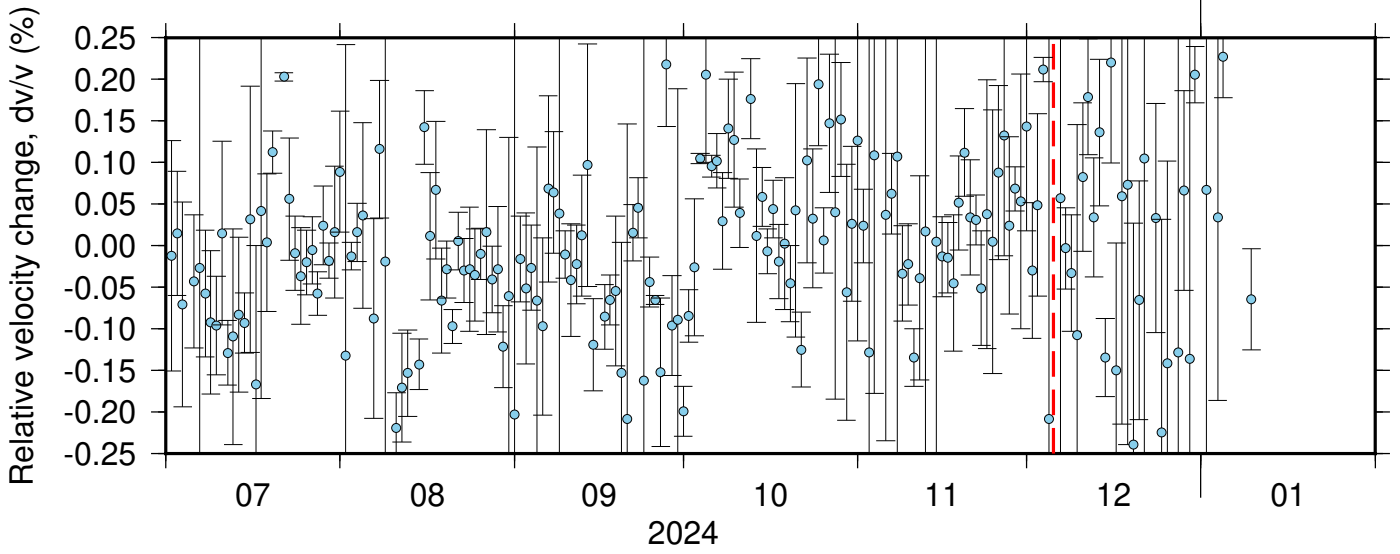
BK_JCC_BK_SPRL ZRT 0.10-0.90Hz 011
