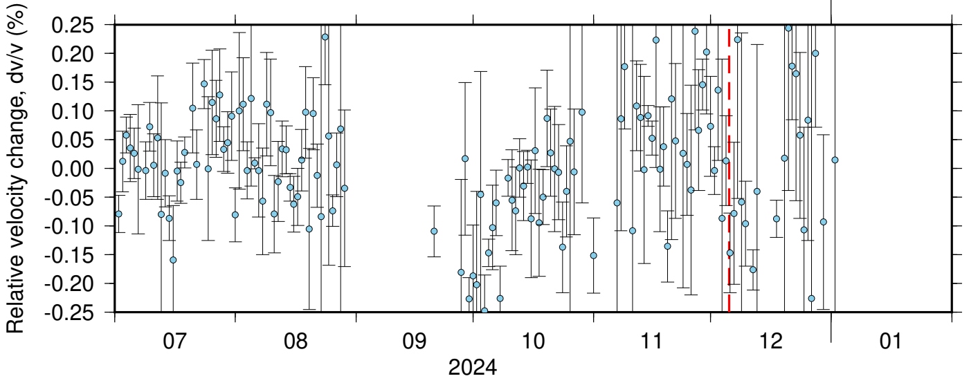
BK_HAYF_PB_B045 ZRT 0.10-0.90Hz 011
