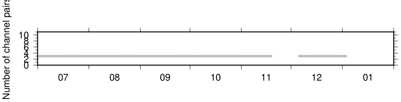
NC_KBU_PB_B049 ZRT 0.10-0.90Hz 011
