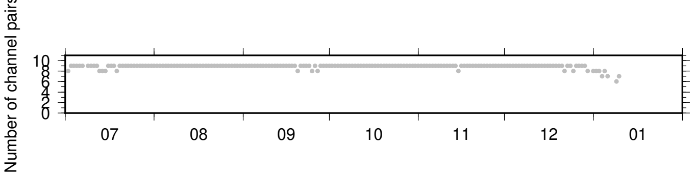
BK_BRIC_BK_HAYF ZRT 0.10-0.90Hz 011
