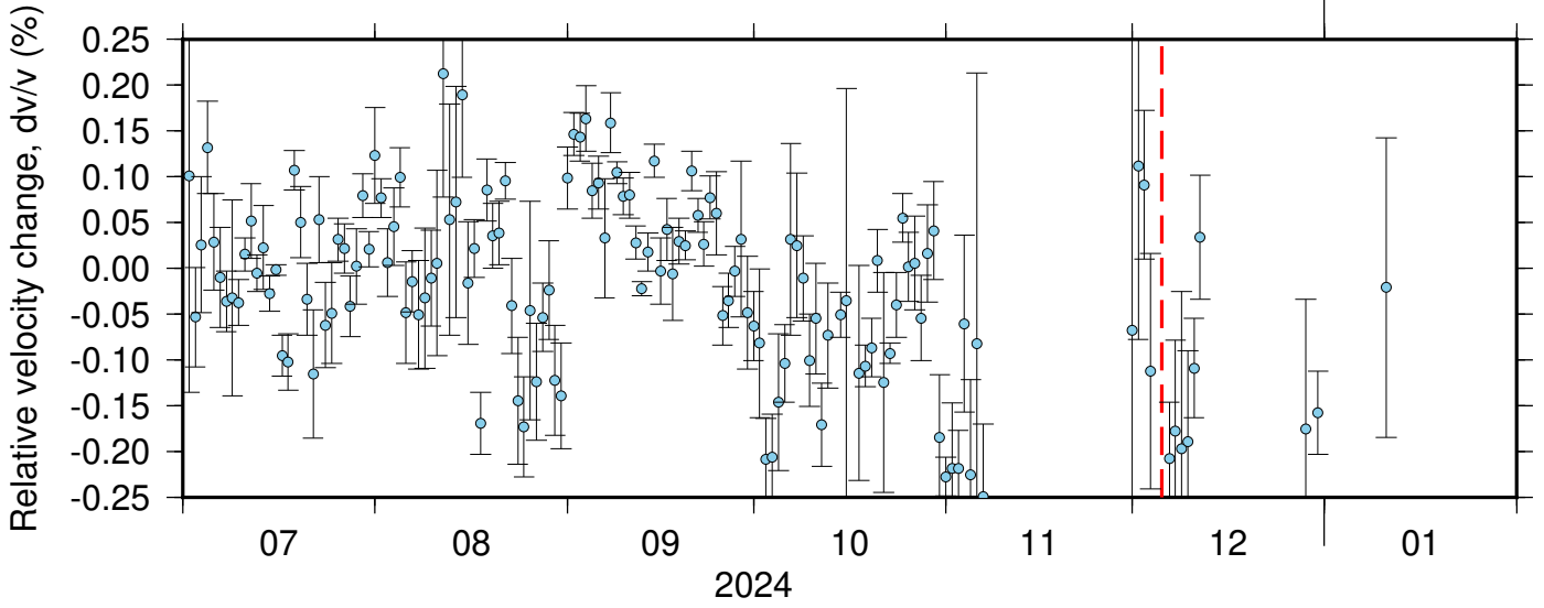
BK_PETL_NC_KSM ZRT 0.10-0.90Hz 011
