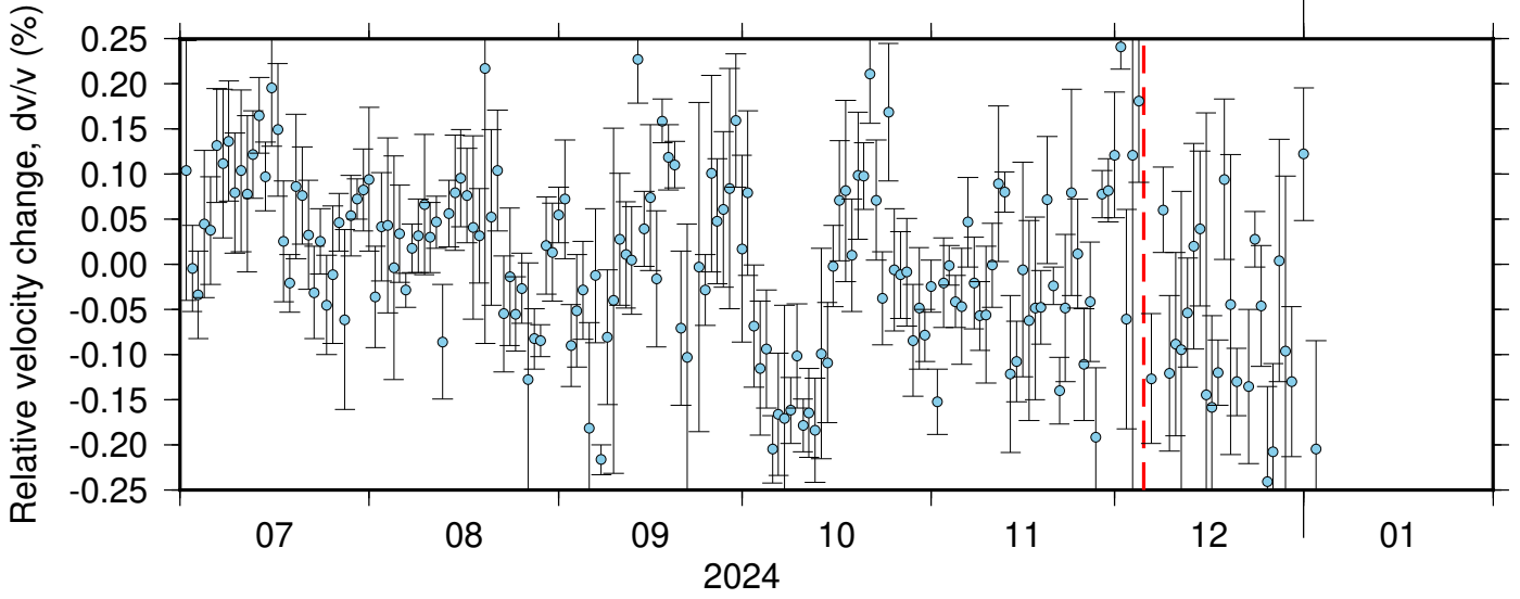
BK_PRDS_PB_B934 ZRT 0.10-0.90Hz 011
