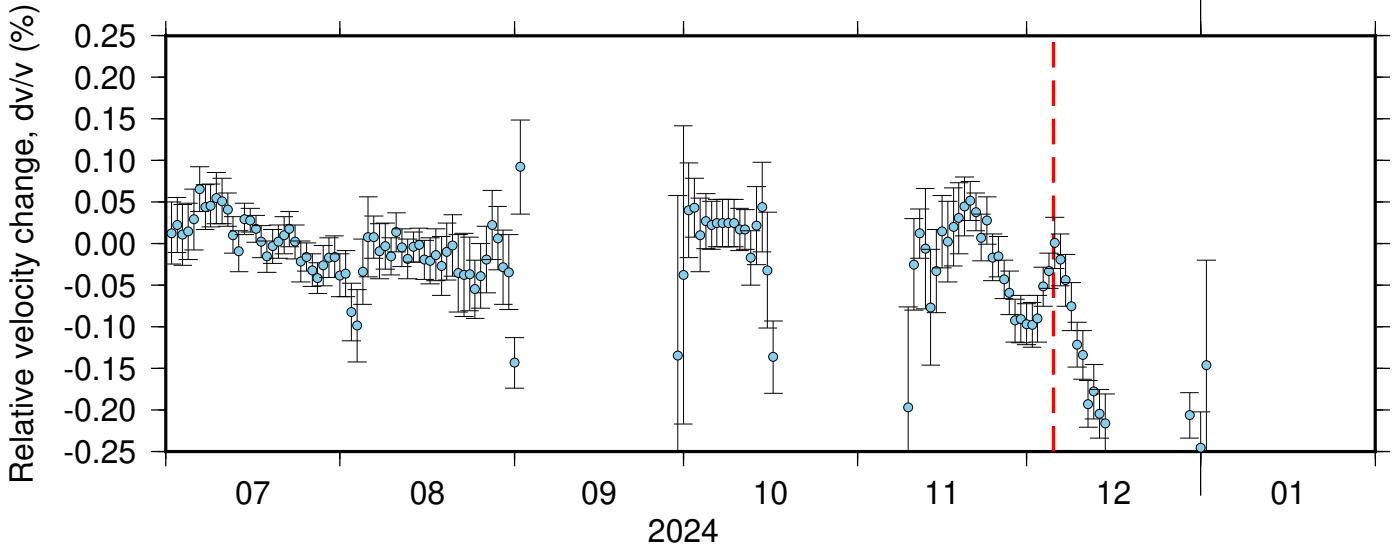
BK_PETL_PB_B046 ZRT 0.10-0.90Hz 011
