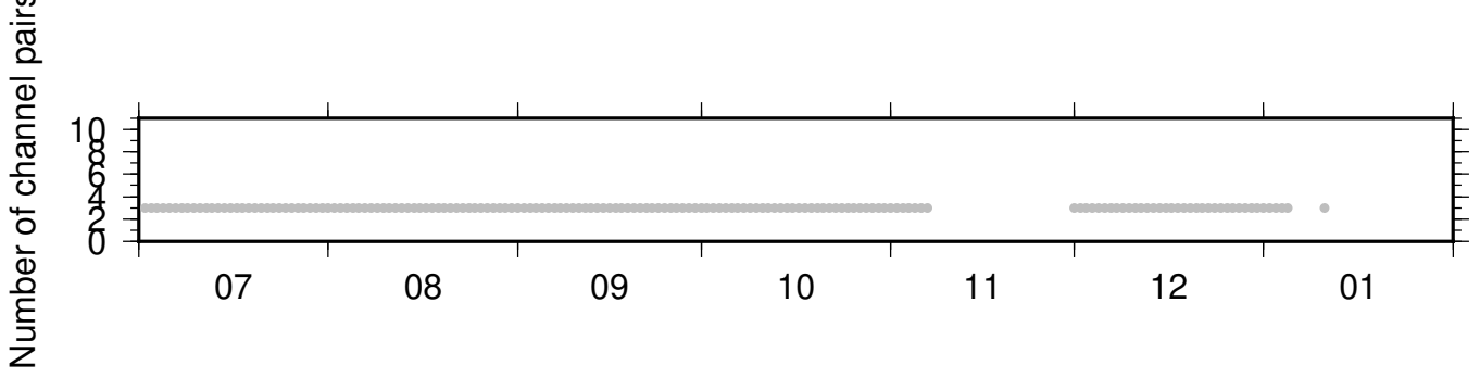
BK_PETL_NC_KSM ZRT 0.10-0.90Hz 011
