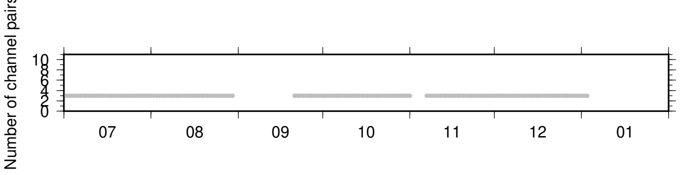
NC_KCR_PB_B045 ZRT 0.10-0.90Hz 011
