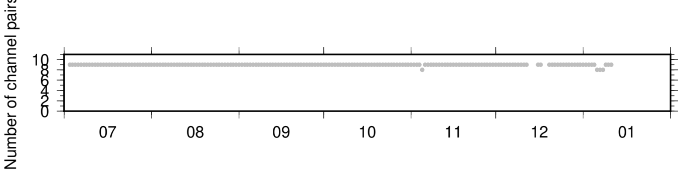
BK_BLAS_BK_RBOW ZRT 0.10-0.90Hz 011
