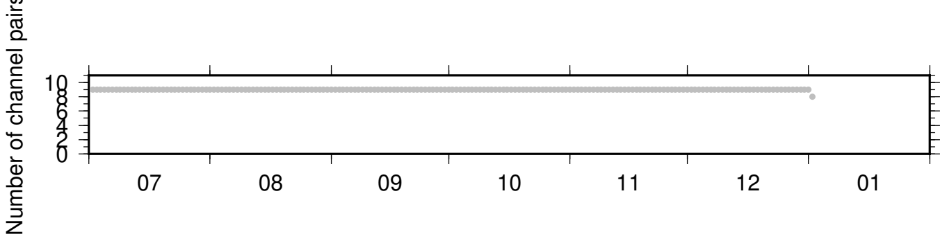
BK_PETL_PB_B047 ZRT 0.10-0.90Hz 011
