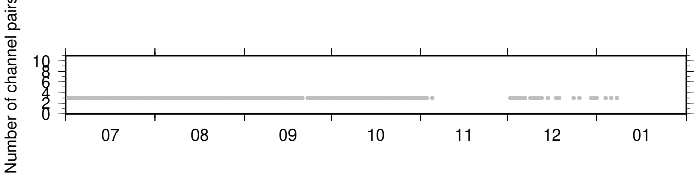
BK_BLAS_NC_KSM ZRT 0.10-0.90Hz 011
