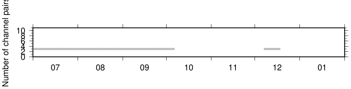
NC_KSM_PB_B932 ZRT 0.10-0.90Hz 011
