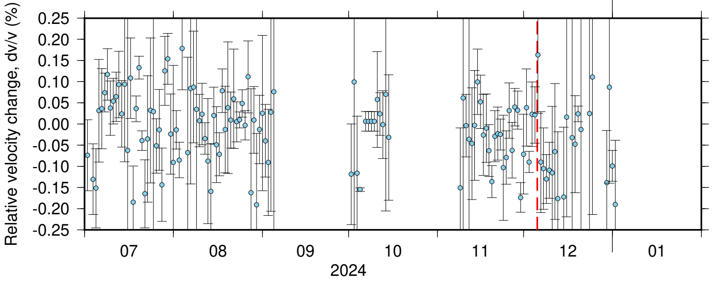
PB_B046_PB_B934 ZRT 0.10-0.90Hz 011
