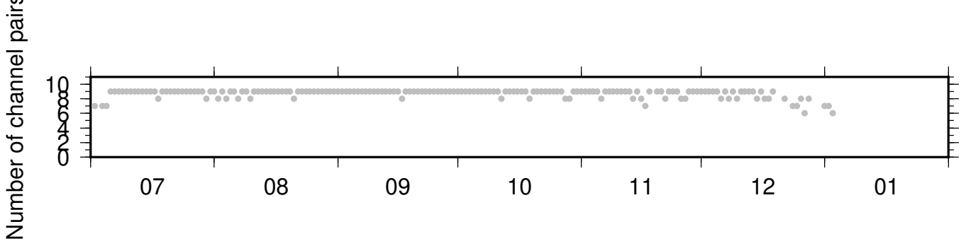
BK_BJES_PB_B934 ZRT 0.10-0.90Hz 011
