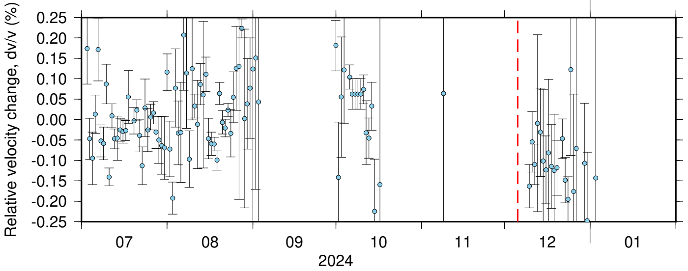
PB_B046_PB_B049 ZRT 0.10-0.90Hz 011
