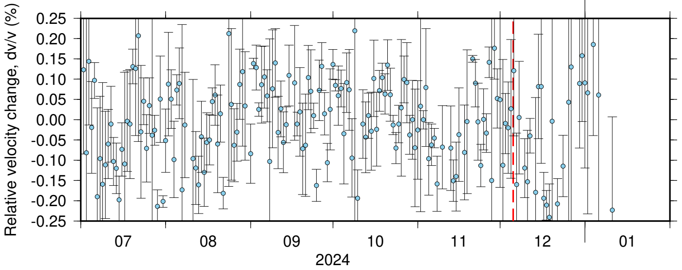
BK_JCC_BK_WLKR ZRT 0.10-0.90Hz 011
