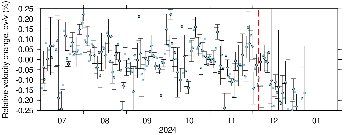
NC_KMPB_NC_KPR ZRT 0.10-0.90Hz 011
