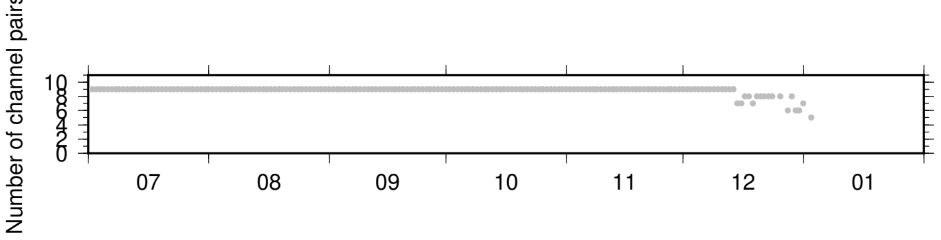
NC_KCT_PB_B047 ZRT 0.10-0.90Hz 011
