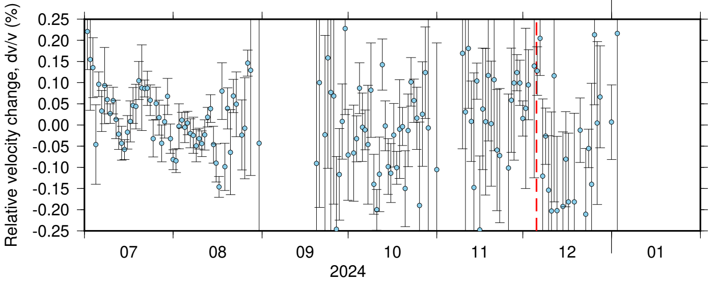
BK_WLKR_PB_B045 ZRT 0.10-0.90Hz 011
