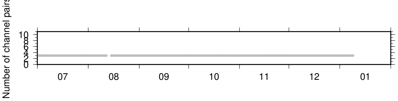
BK_WLKR_NC_KPR ZRT 0.10-0.90Hz 011
