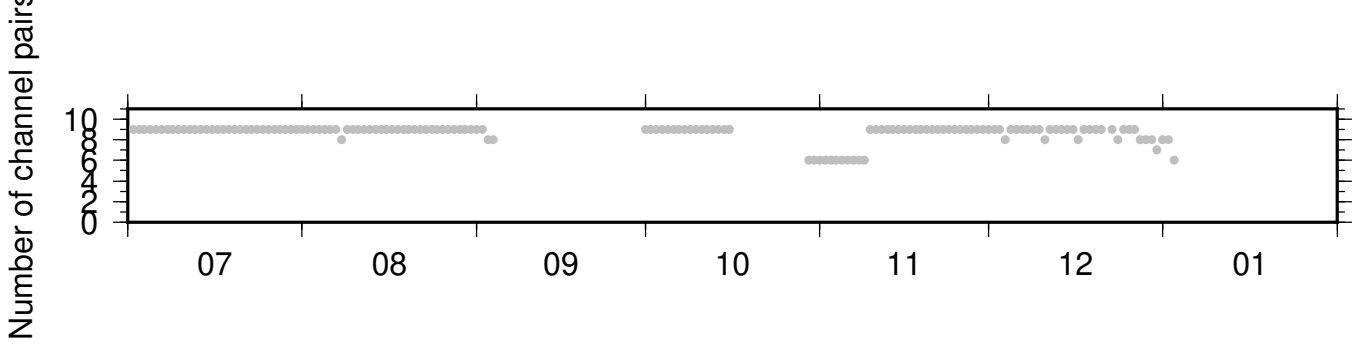
NC_KMR_PB_B046 ZRT 0.10-0.90Hz 011
