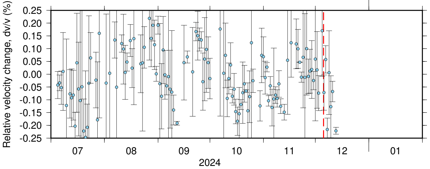
NC_KBU_NC_KCT ZRT 0.10-0.90Hz 011
