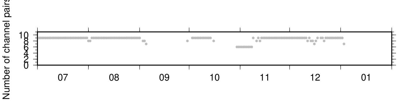
BK_JCC_PB_B046 ZRT 0.10-0.90Hz 011
