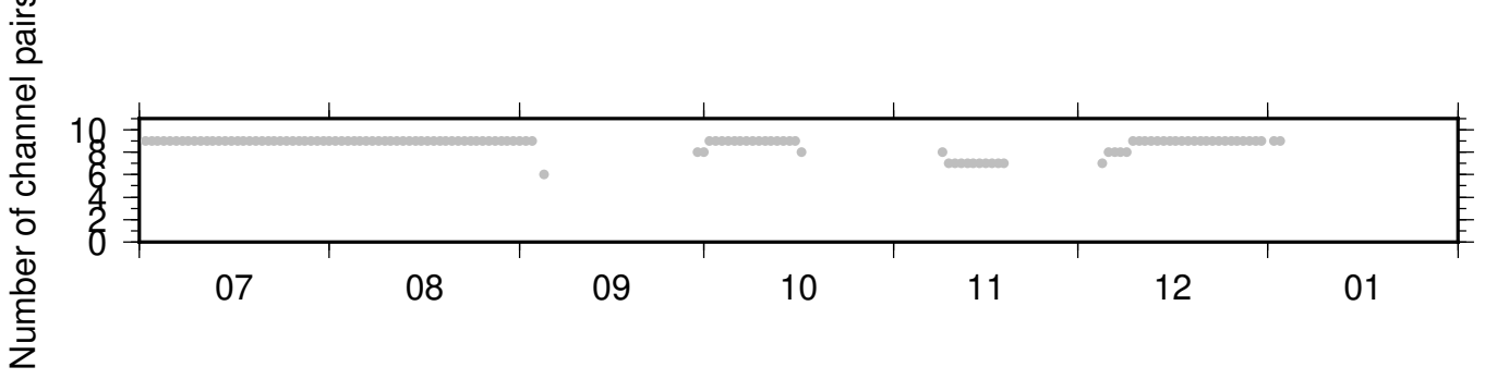
PB_B046_PB_B049 ZRT 0.10-0.90Hz 011
