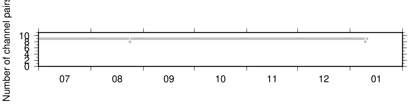
BK_JCC_NC_KMPB ZRT 0.10-0.90Hz 011
