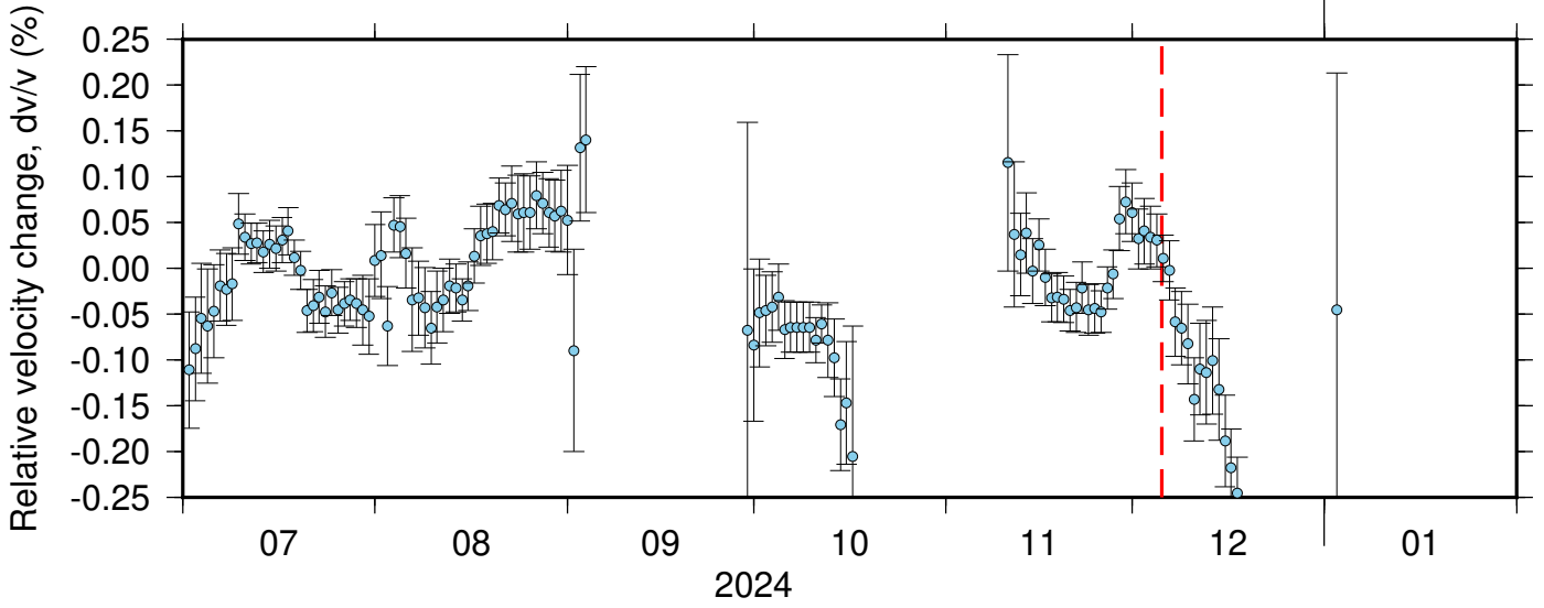
BK_WLKR_PB_B046 ZRT 0.10-0.90Hz 011
