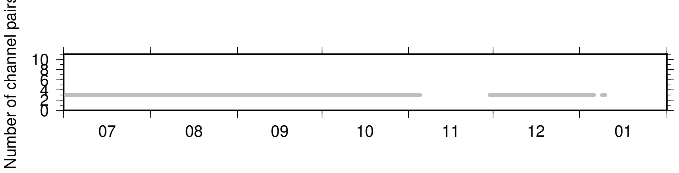
BK_WLKR_NC_KSM ZRT 0.10-0.90Hz 011
