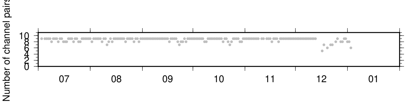
BK_WLKR_PB_B934 ZRT 0.10-0.90Hz 011
