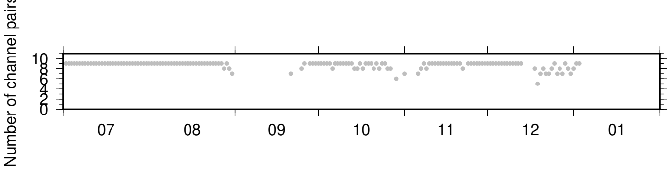
BK_HAYF_PB_B045 ZRT 0.10-0.90Hz 011
