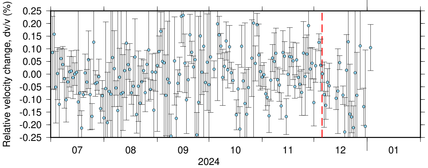
BK_JCC_PB_B935 ZRT 0.10-0.90Hz 011
