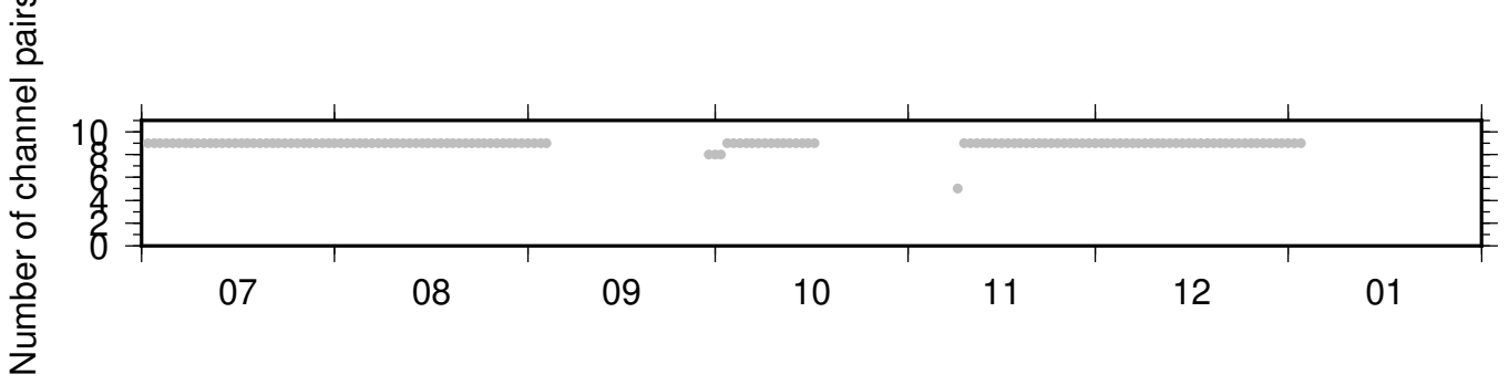
BK_PRDS_PB_B046 ZRT 0.10-0.90Hz 011
