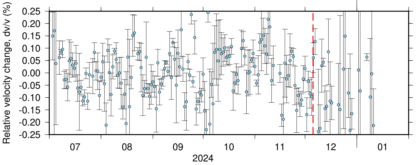
NC_KMR_NC_KPR ZRT 0.10-0.90Hz 011
