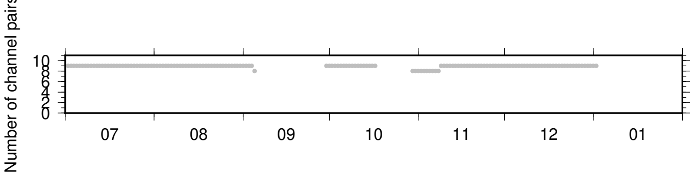
BK_PETL_PB_B046 ZRT 0.10-0.90Hz 011
