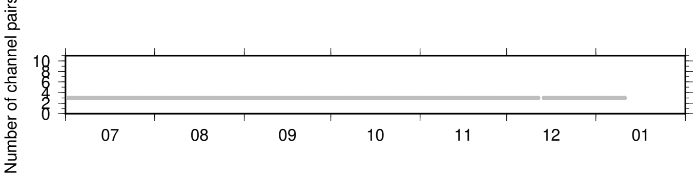
BK_BJES_NC_KCR ZRT 0.10-0.90Hz 011
