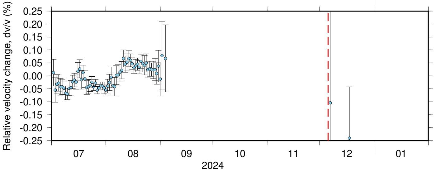
PB_B046_PB_B932 ZRT 0.10-0.90Hz 011
