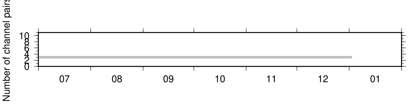
NC_KBU_PB_B047 ZRT 0.10-0.90Hz 011
