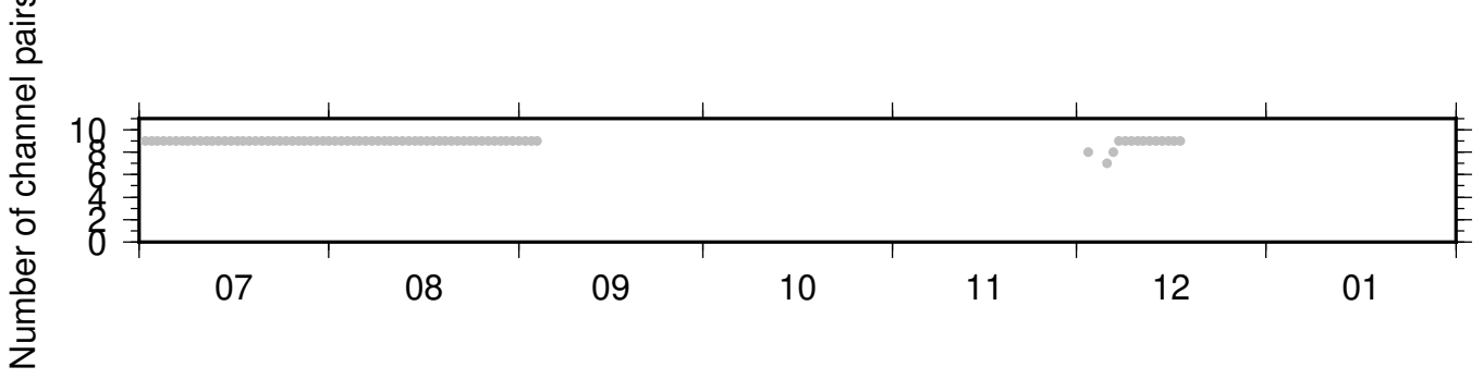
PB_B046_PB_B932 ZRT 0.10-0.90Hz 011
