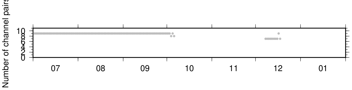
PB_B049_PB_B932 ZRT 0.10-0.90Hz 011
