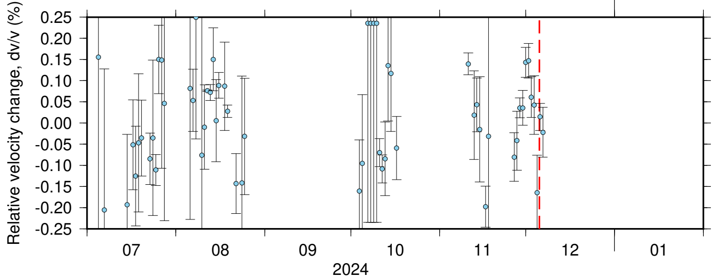
NC_KCR_PB_B046 ZRT 0.10-0.90Hz 011
