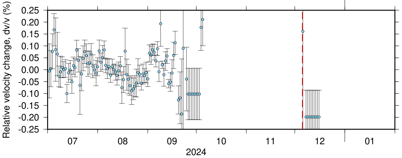
NC_KCT_PB_B932 ZRT 0.10-0.90Hz 011
