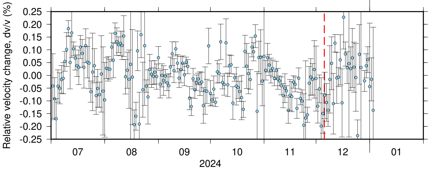
NC_KMR_PB_B934 ZRT 0.10-0.90Hz 011
