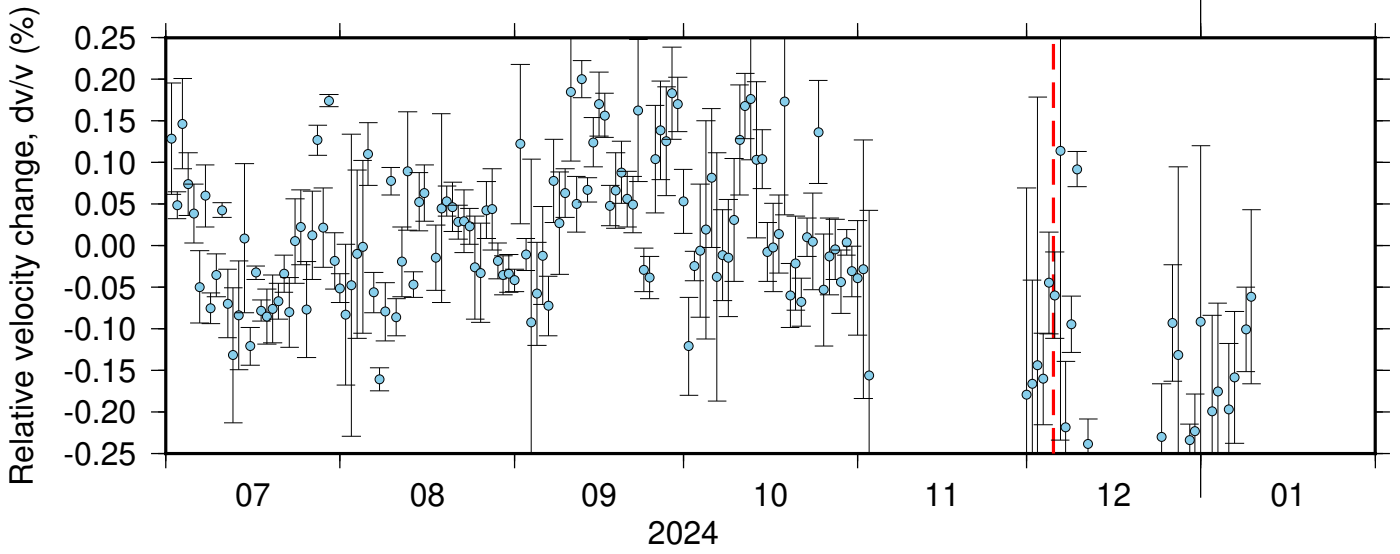
BK_BRIC_NC_KSM ZRT 0.10-0.90Hz 011
