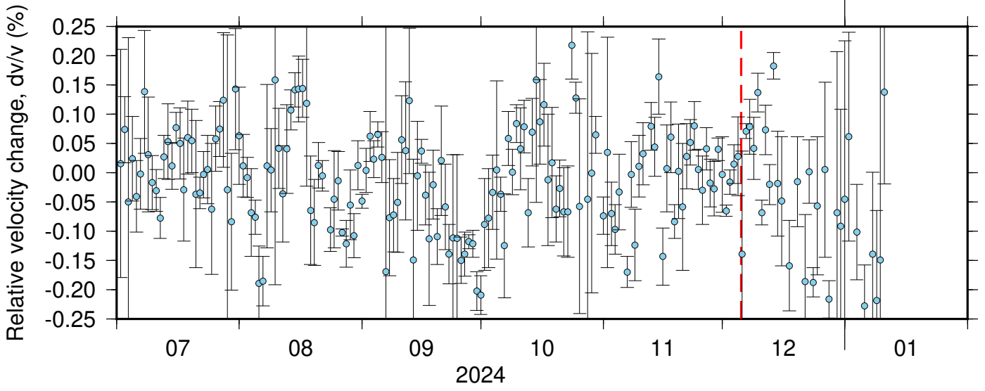
BK_JCC_NC_KMPB ZRT 0.10-0.90Hz 011
