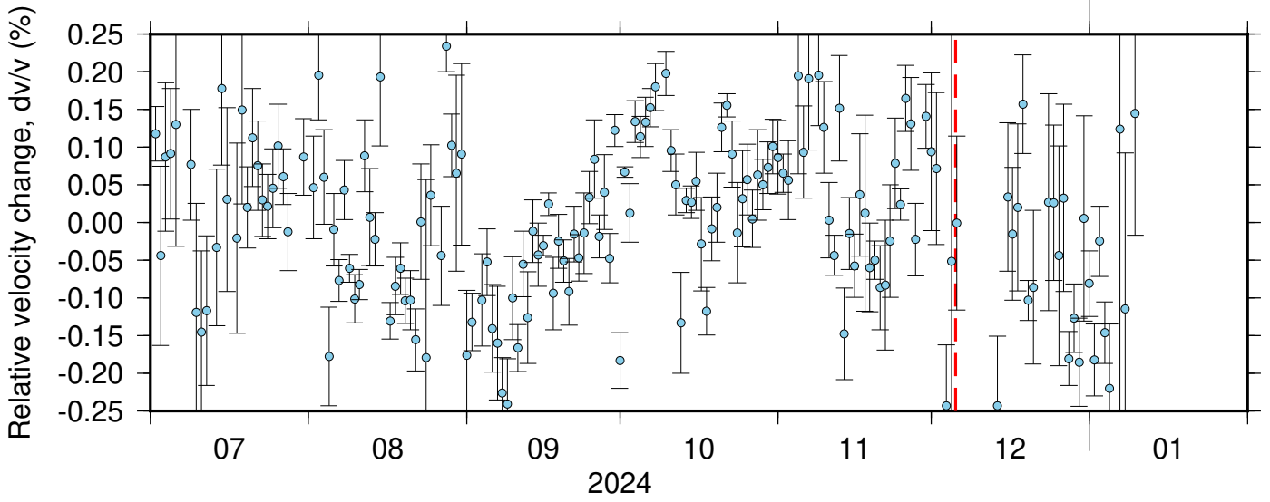
BK_BJES_NC_KCR ZRT 0.10-0.90Hz 011
