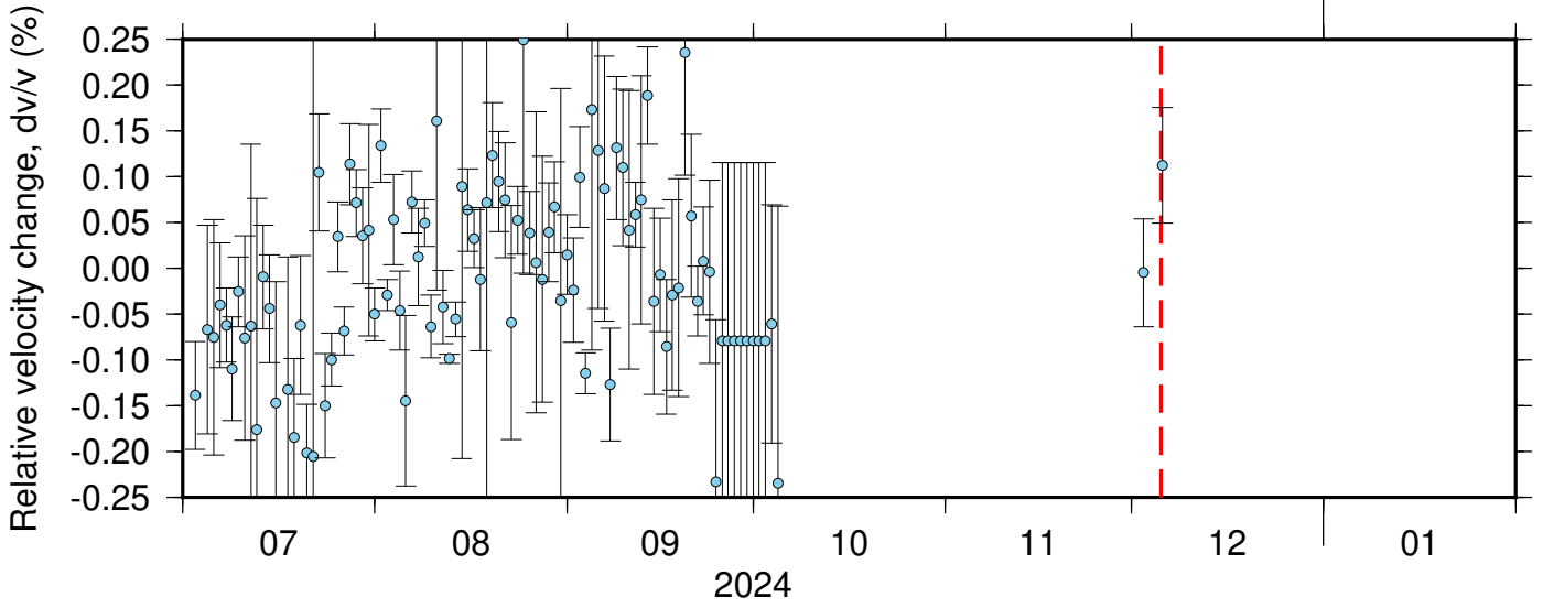
PB_B932_PB_B934 ZRT 0.10-0.90Hz 011
