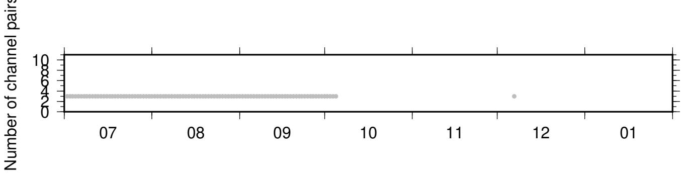
NC_KBU_PB_B932 ZRT 0.10-0.90Hz 011
