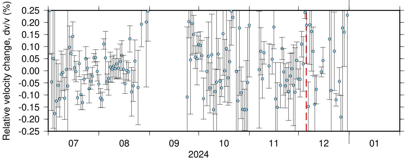
BK_JCC_PB_B045 ZRT 0.10-0.90Hz 011
