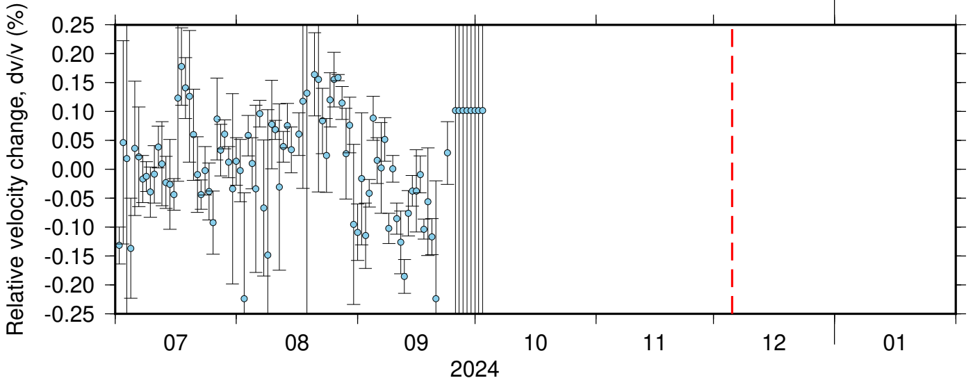
NC_KBU_PB_B932 ZRT 0.10-0.90Hz 011
