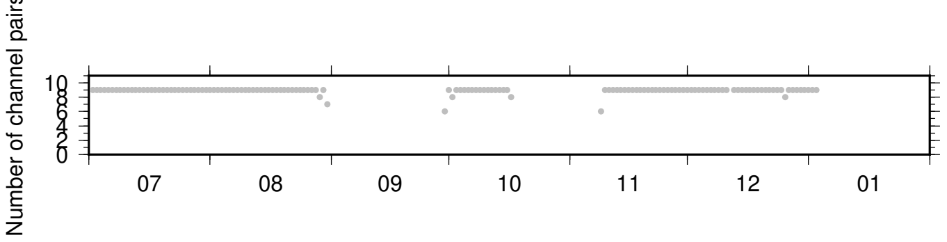
PB_B045_PB_B046 ZRT 0.10-0.90Hz 011
