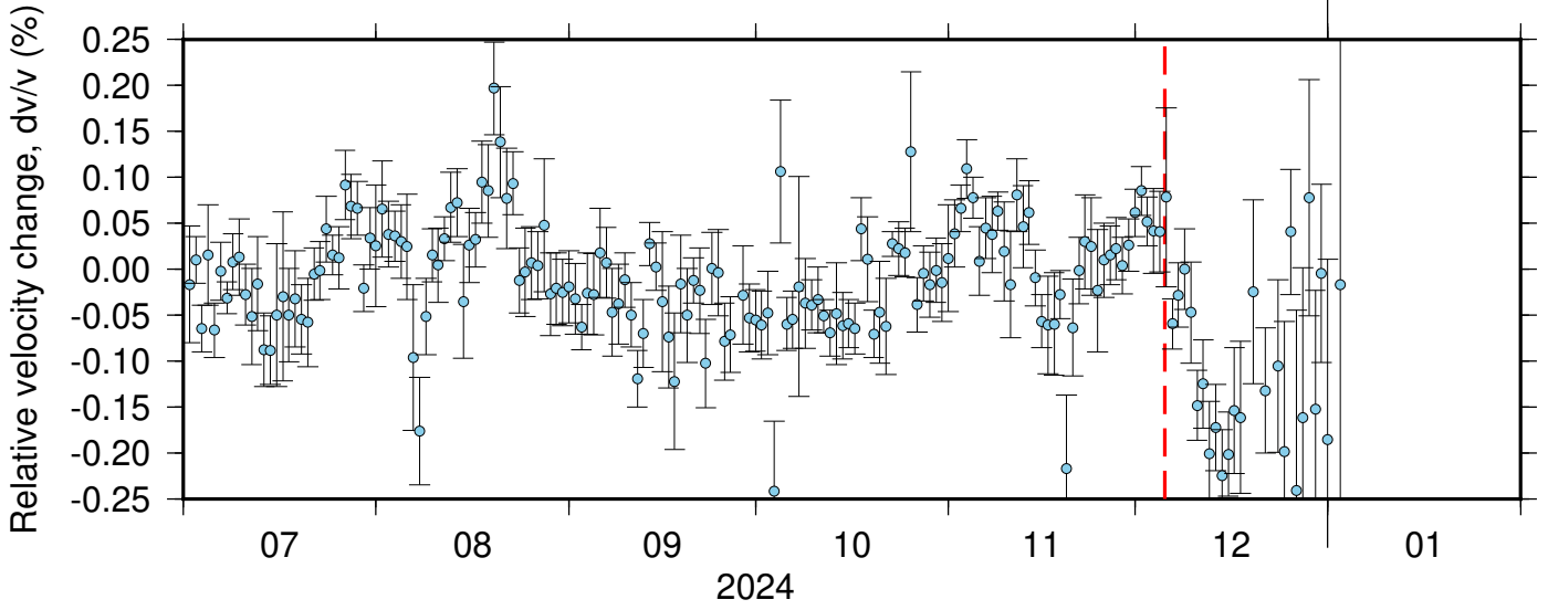
BK_SPRL_PB_B047 ZRT 0.10-0.90Hz 011
