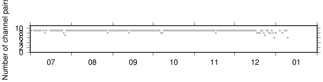
BK_JCC_BK_PRDS ZRT 0.10-0.90Hz 011
