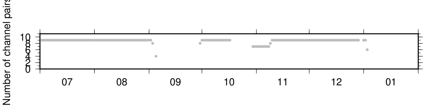
BK_BRIC_PB_B046 ZRT 0.10-0.90Hz 011
