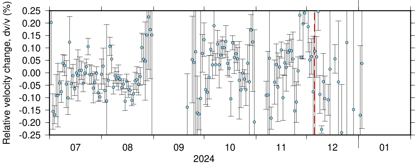
BK_SPRL_PB_B045 ZRT 0.10-0.90Hz 011
