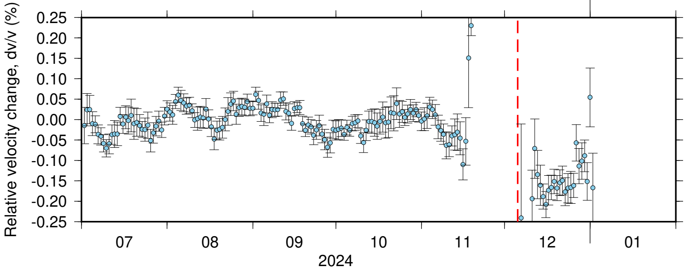
NC_KMR_PB_B049 ZRT 0.10-0.90Hz 011
