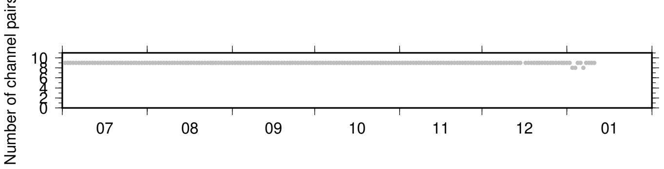
BK_PETL_BK_PRDS ZRT 0.10-0.90Hz 011
