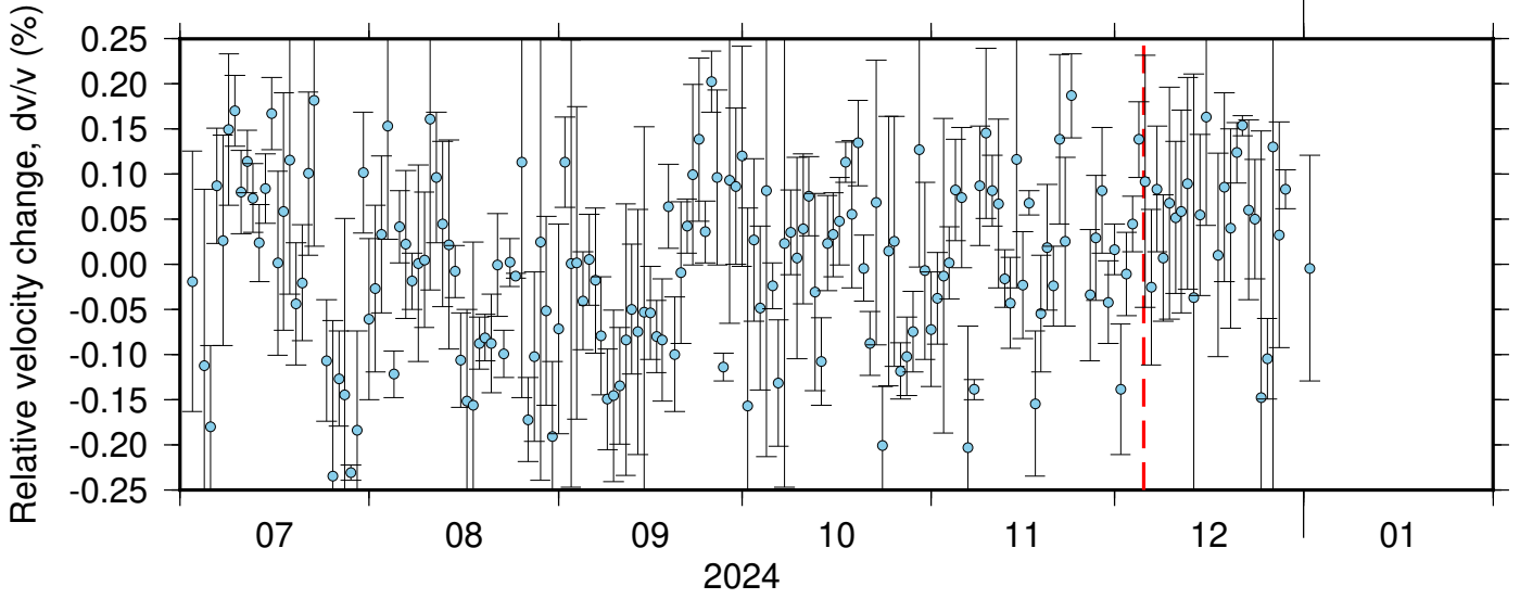
PB_B047_PB_B934 ZRT 0.10-0.90Hz 011
