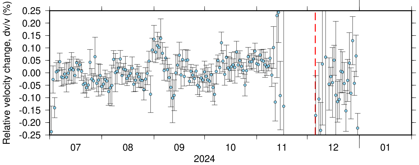
BK_BJES_PB_B049 ZRT 0.10-0.90Hz 011
