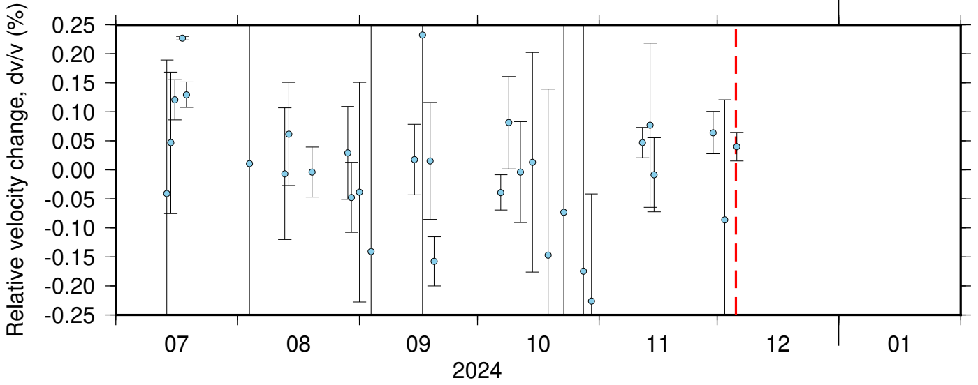
NC_KCR_PB_B934 ZRT 0.10-0.90Hz 011
