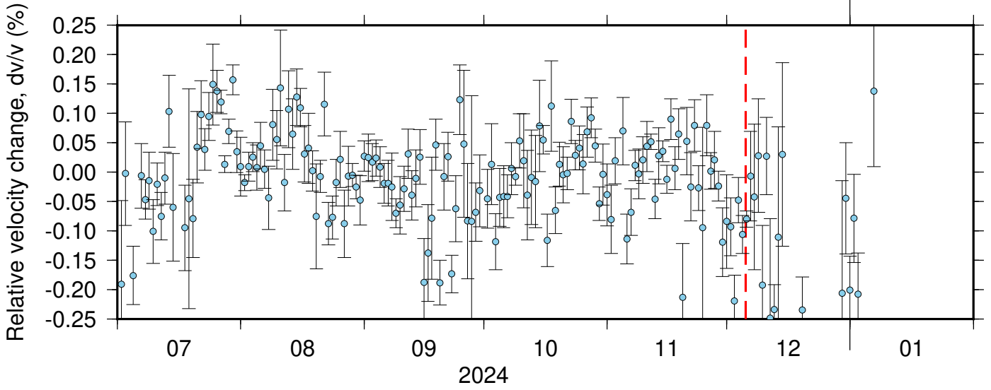
NC_KCT_NC_KMPB ZRT 0.10-0.90Hz 011
