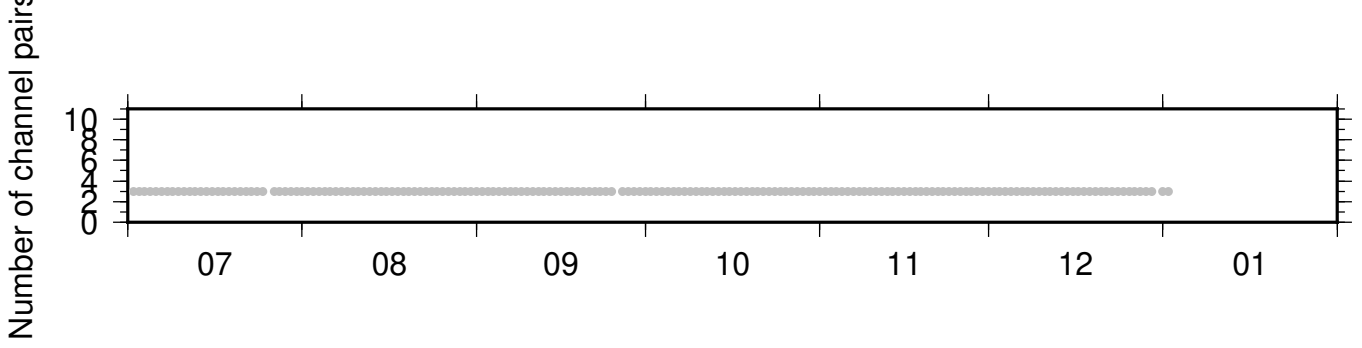
NC_KBU_PB_B935 ZRT 0.10-0.90Hz 011
