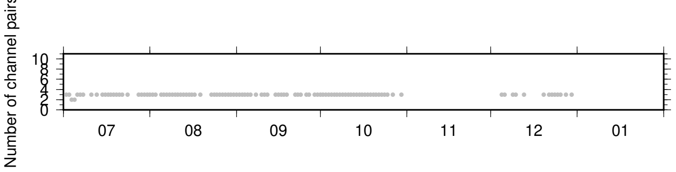
NC_KSM_PB_B935 ZRT 0.10-0.90Hz 011
