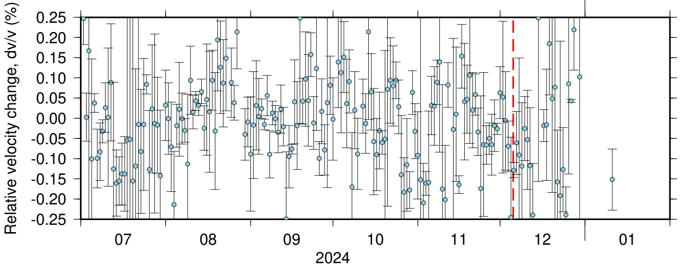
BK_KNEE_BK_PETL ZRT 0.10-0.90Hz 011
