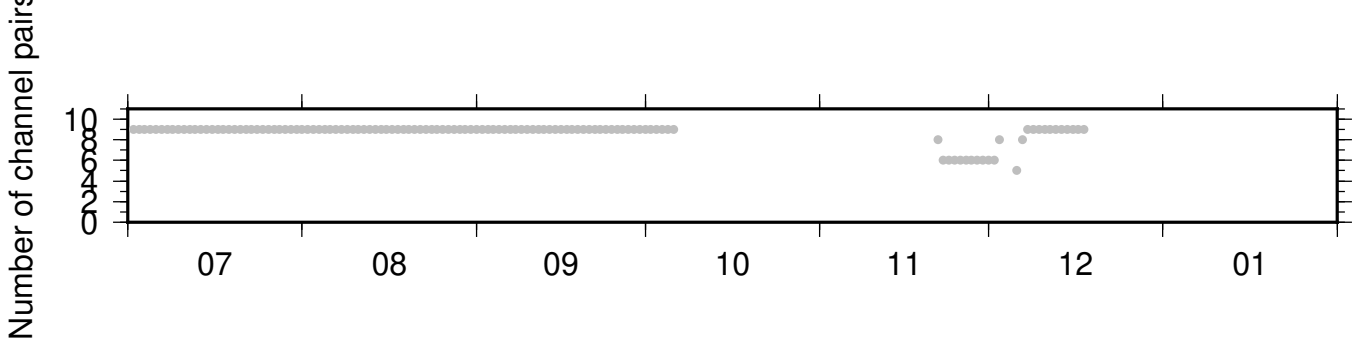
PB_B047_PB_B932 ZRT 0.10-0.90Hz 011
