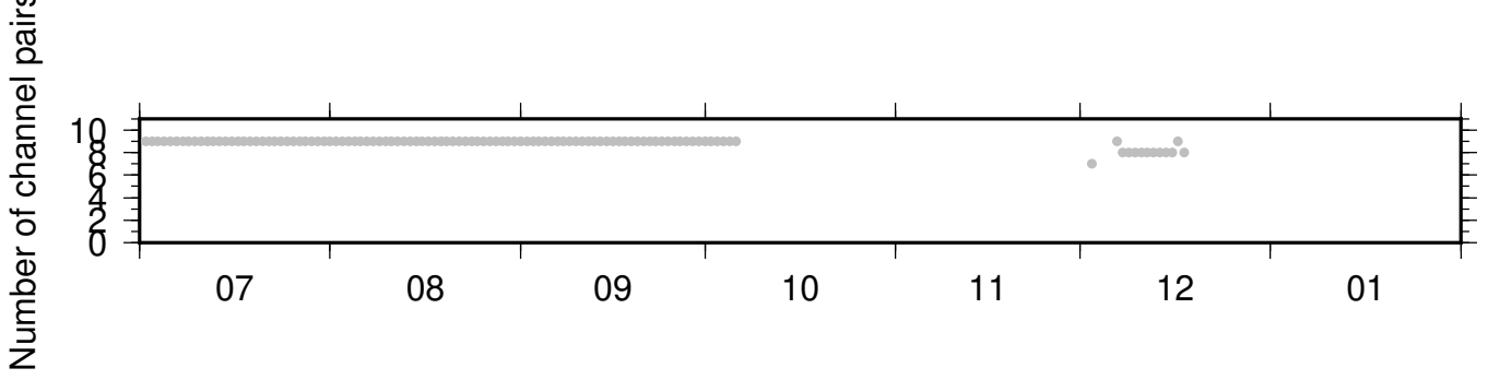
BK_GHOP_PB_B932 ZRT 0.10-0.90Hz 011
