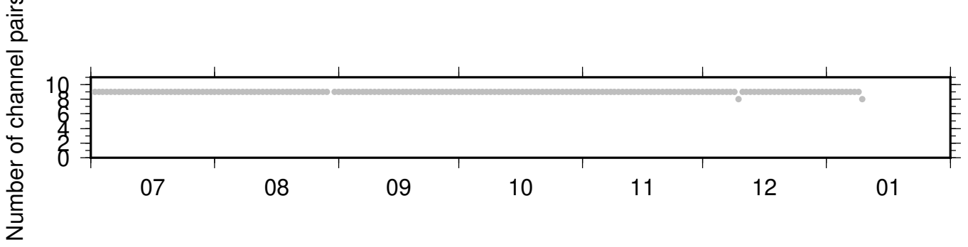
BK_SPRL_BK_WLKR ZRT 0.10-0.90Hz 011
