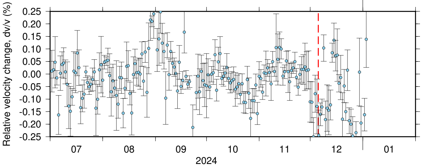
NC_KMR_PB_B935 ZRT 0.10-0.90Hz 011
