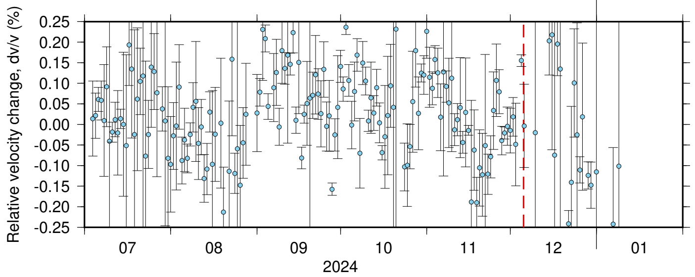
NC_KCR_NC_KMR ZRT 0.10-0.90Hz 011
