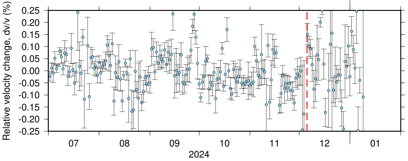
BK_BLAS_BK_BRIC ZRT 0.10-0.90Hz 011
