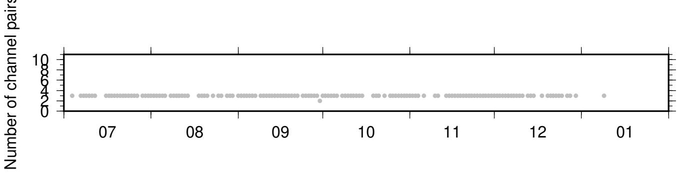
BK_KNEE_NC_KPR ZRT 0.10-0.90Hz 011
