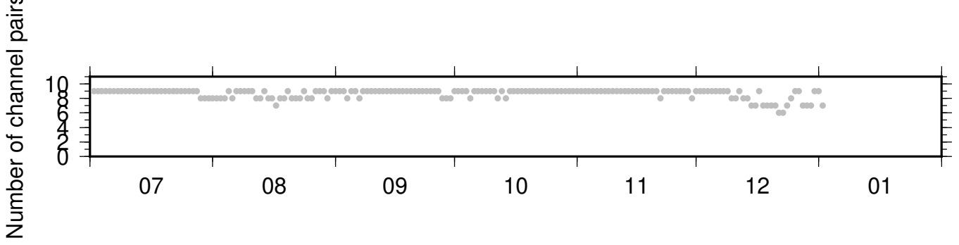
BK_BRIC_PB_B934 ZRT 0.10-0.90Hz 011
