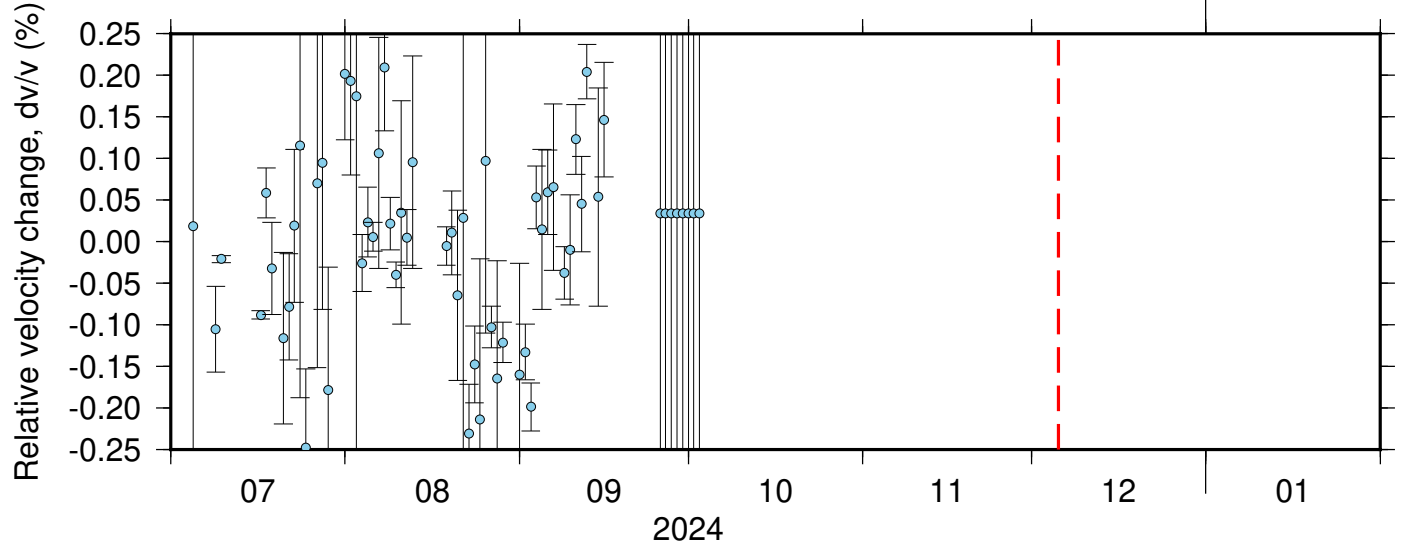
NC_KCR_PB_B932 ZRT 0.10-0.90Hz 011
