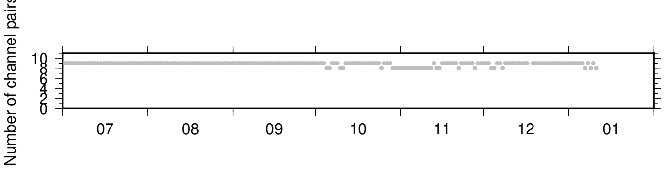
BK_BJES_BK_BRIC ZRT 0.10-0.90Hz 011
