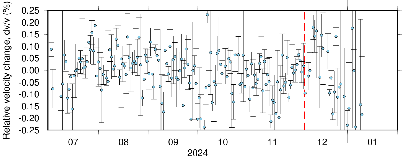
BK_BRIC_BK_HAYF ZRT 0.10-0.90Hz 011
