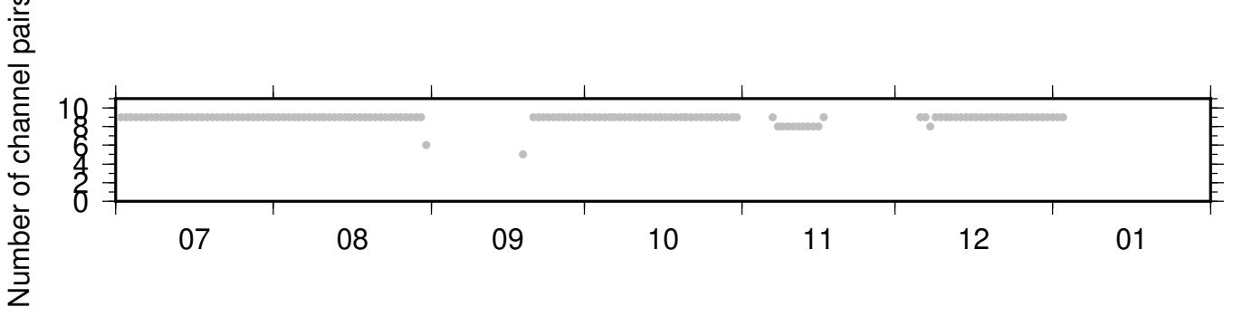
PB_B045_PB_B049 ZRT 0.10-0.90Hz 011
