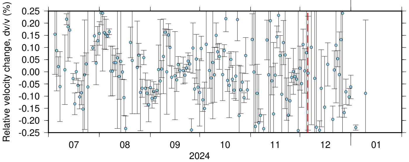
BK_BJES_NC_KPR ZRT 0.10-0.90Hz 011
