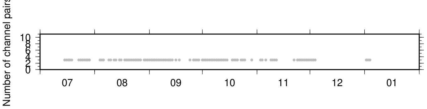
BK_WLKR_NC_KCR ZRT 0.10-0.90Hz 011
