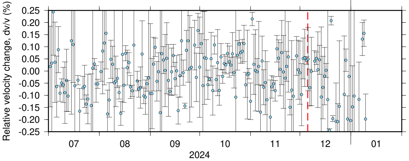
BK_KNEE_BK_PRDS ZRT 0.10-0.90Hz 011
