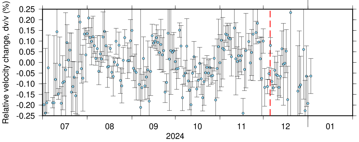
BK_SPRL_PB_B935 ZRT 0.10-0.90Hz 011
