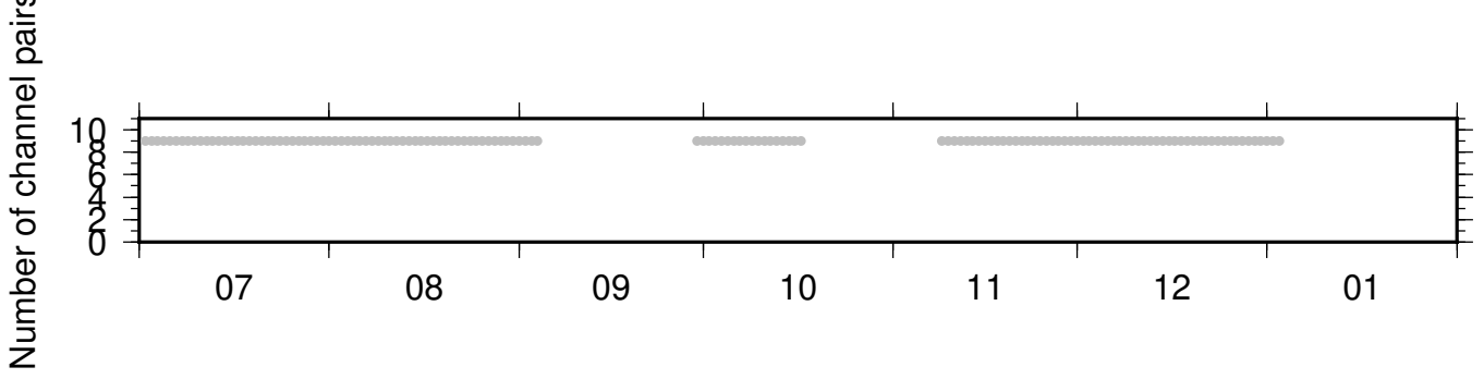
BK_WLKR_PB_B046 ZRT 0.10-0.90Hz 011
