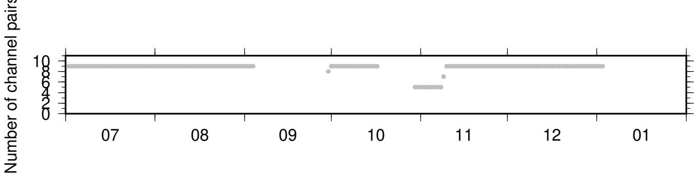
PB_B046_PB_B047 ZRT 0.10-0.90Hz 011
