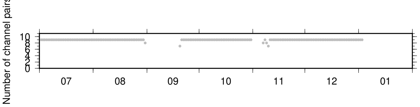
PB_B045_PB_B047 ZRT 0.10-0.90Hz 011
