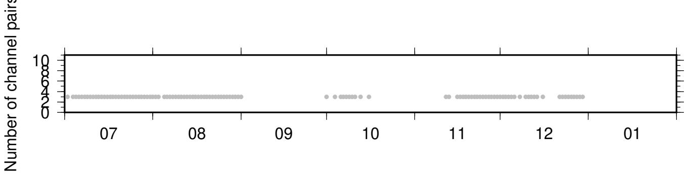
NC_KBU_PB_B046 ZRT 0.10-0.90Hz 011
