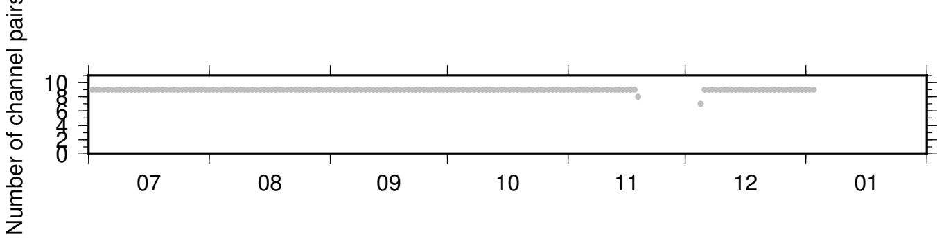
NC_KMR_PB_B049 ZRT 0.10-0.90Hz 011
