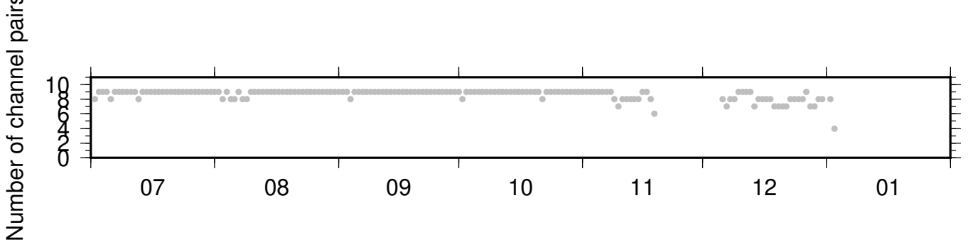
PB_B049_PB_B934 ZRT 0.10-0.90Hz 011
