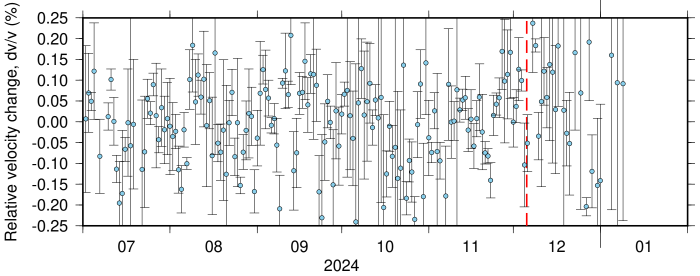
BK_BLAS_BK_WLKR ZRT 0.10-0.90Hz 011
