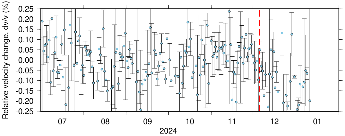
BK_HAYF_BK_RBOW ZRT 0.10-0.90Hz 011
