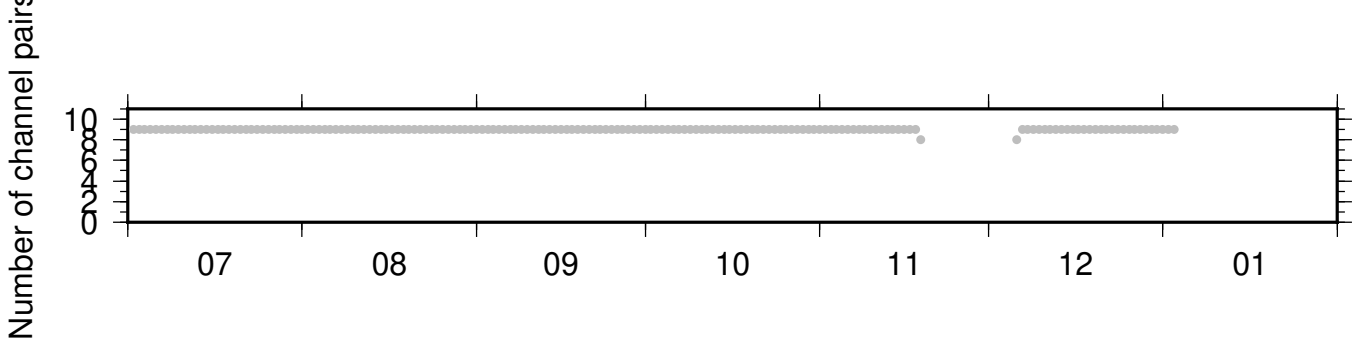
BK_SPRL_PB_B049 ZRT 0.10-0.90Hz 011
