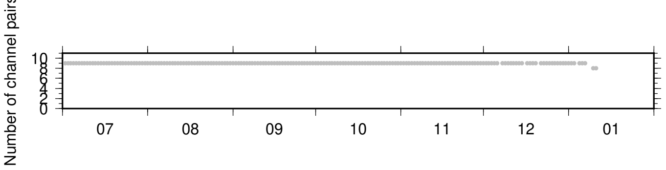
BK_WLKR_NC_KMR ZRT 0.10-0.90Hz 011
