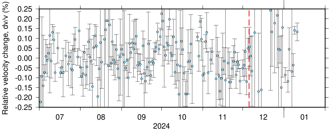
BK_BLAS_NC_KCT ZRT 0.10-0.90Hz 011
