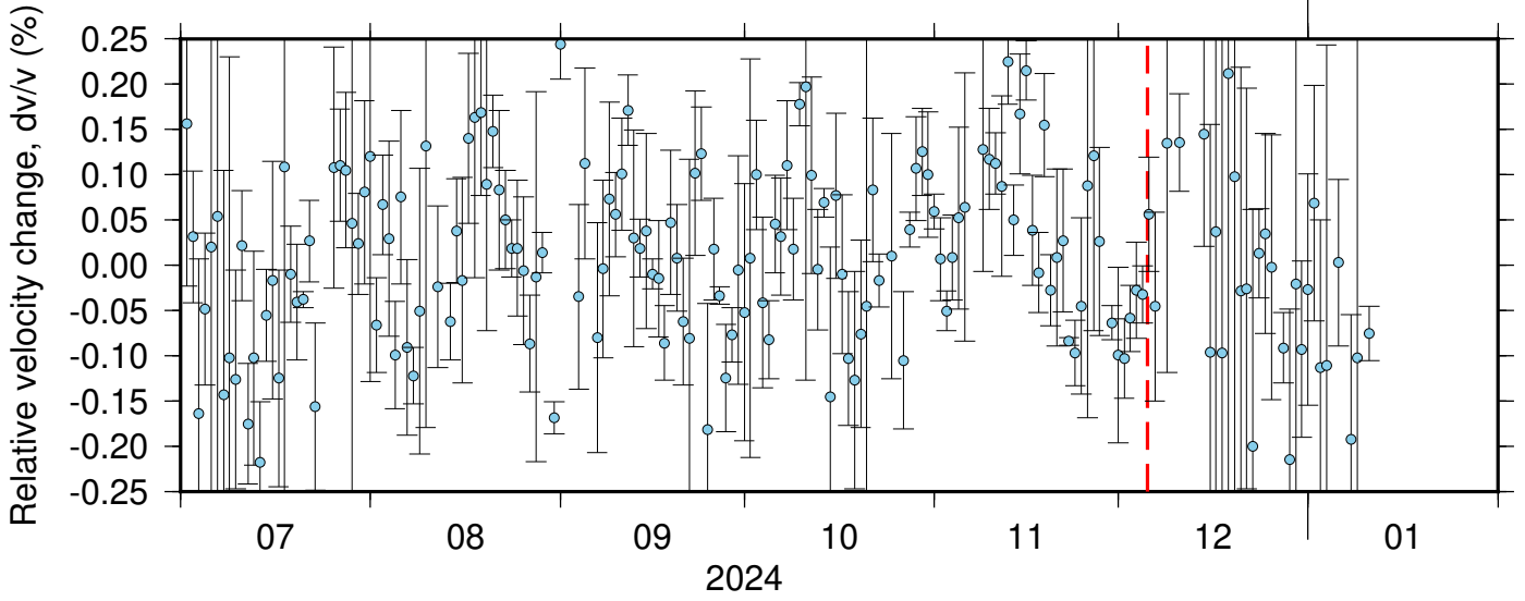
BK_JCC_BK_RBOW ZRT 0.10-0.90Hz 011
