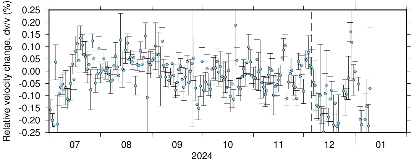
BK_PRDS_BK_WLKR ZRT 0.10-0.90Hz 011
