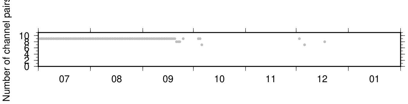
BK_BLAS_PB_B932 ZRT 0.10-0.90Hz 011
