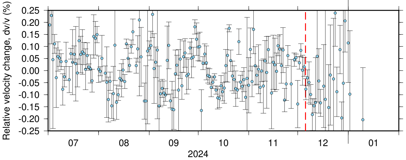
BK_BJES_BK_SPRL ZRT 0.10-0.90Hz 011
