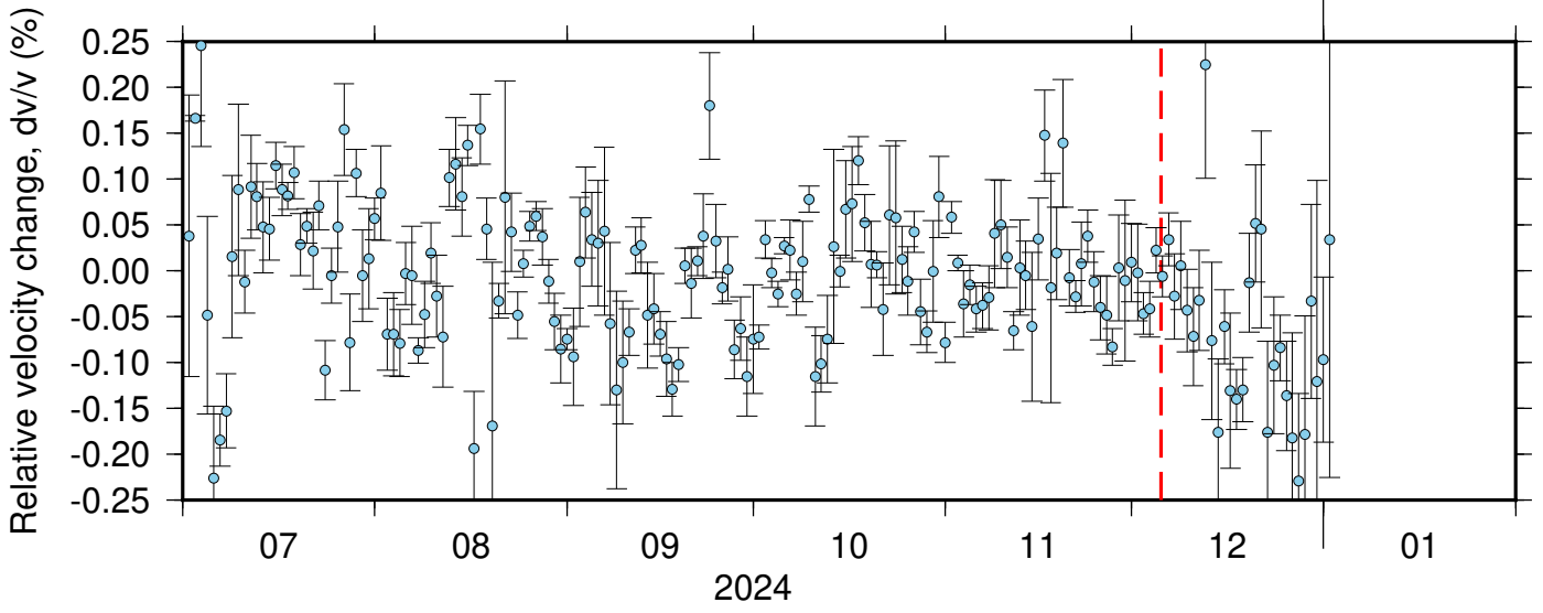
NC_KBU_PB_B047 ZRT 0.10-0.90Hz 011
