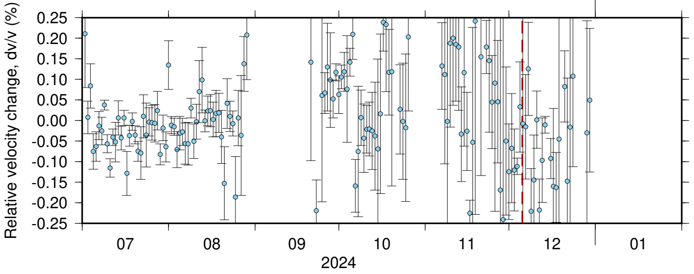
BK_KNEE_PB_B045 ZRT 0.10-0.90Hz 011
