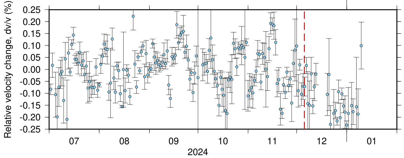
BK_BRIC_NC_KPR ZRT 0.10-0.90Hz 011
