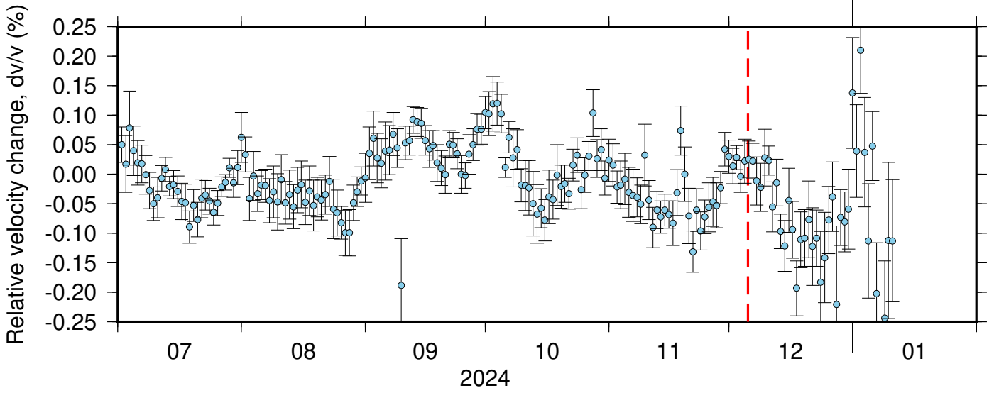
BK_BJES_BK_KNEE ZRT 0.10-0.90Hz 011
