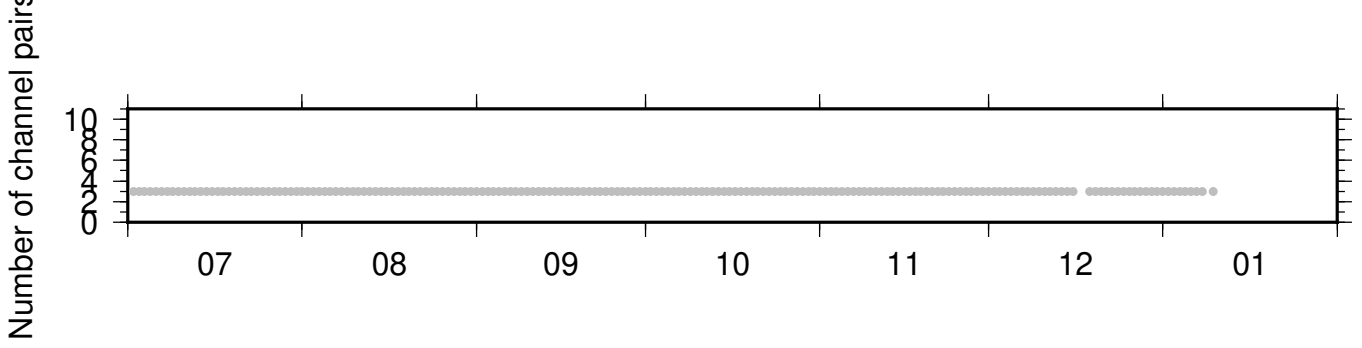
BK_BJES_NC_KBU ZRT 0.10-0.90Hz 011
