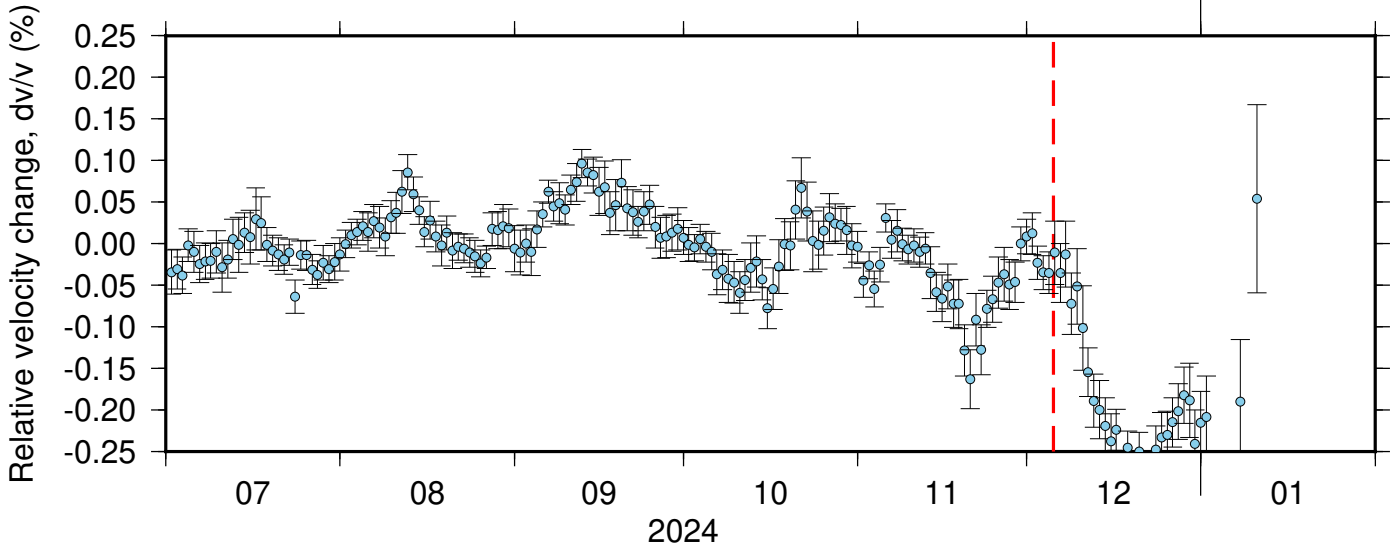
BK_BRIC_BK_SPRL ZRT 0.10-0.90Hz 011
