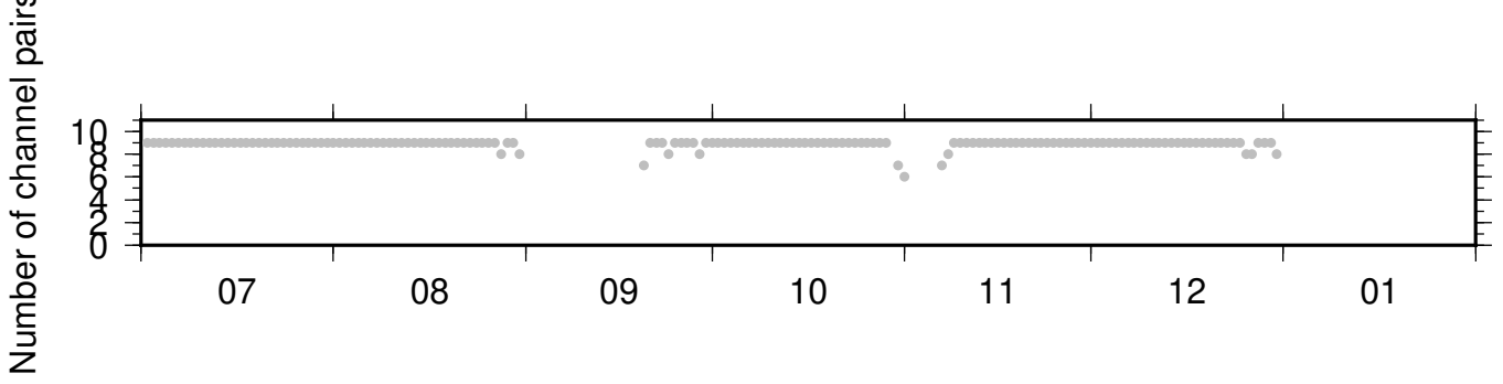
BK_PETL_PB_B045 ZRT 0.10-0.90Hz 011
