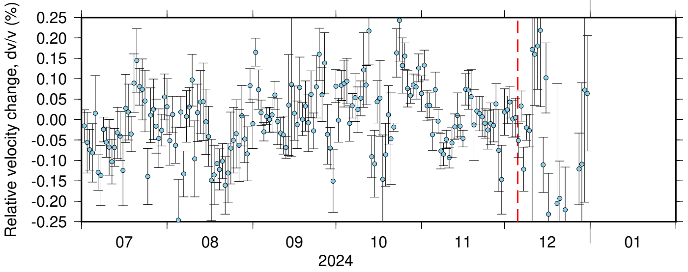
NC_KCT_PB_B047 ZRT 0.10-0.90Hz 011
