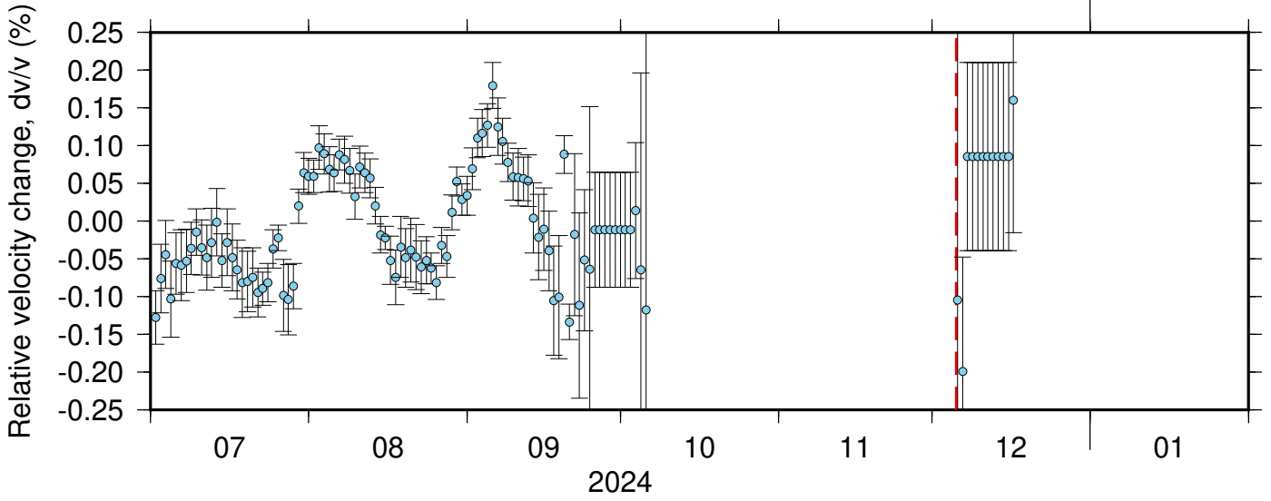
NC_KMPB_PB_B932 ZRT 0.10-0.90Hz 011
