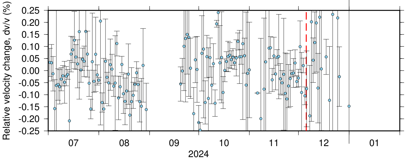
PB_B045_PB_B934 ZRT 0.10-0.90Hz 011
