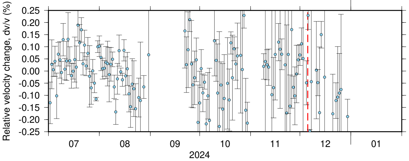
PB_B045_PB_B935 ZRT 0.10-0.90Hz 011
