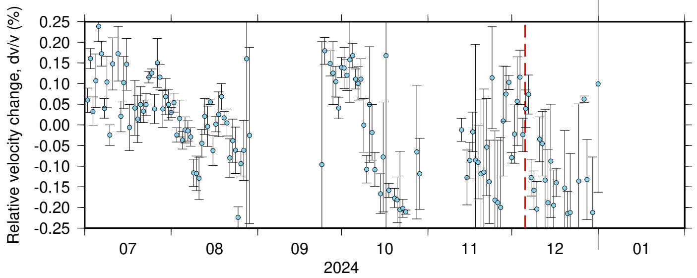
NC_KBU_PB_B045 ZRT 0.10-0.90Hz 011
