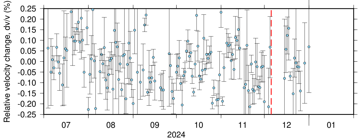
NC_KCR_PB_B935 ZRT 0.10-0.90Hz 011
