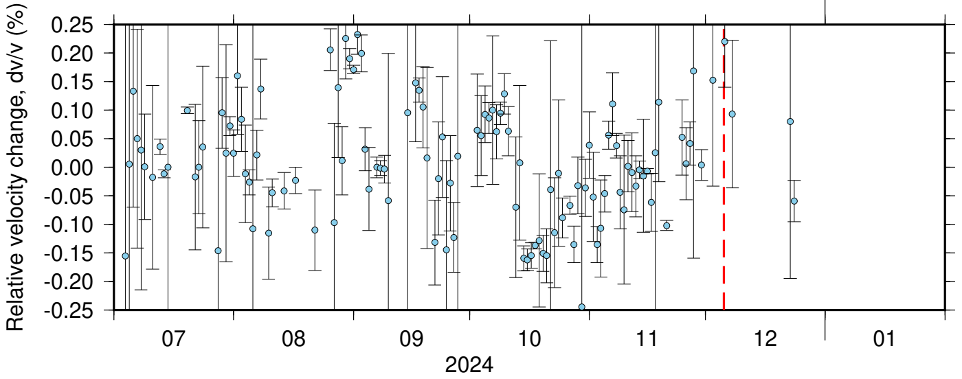
BK_HAYF_NC_KPR ZRT 0.10-0.90Hz 011
