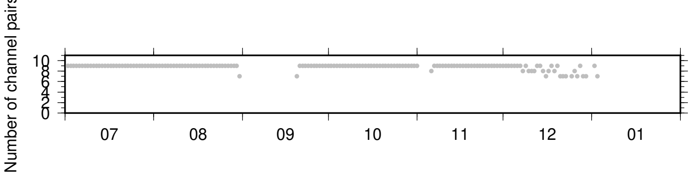
NC_KCT_PB_B045 ZRT 0.10-0.90Hz 011
