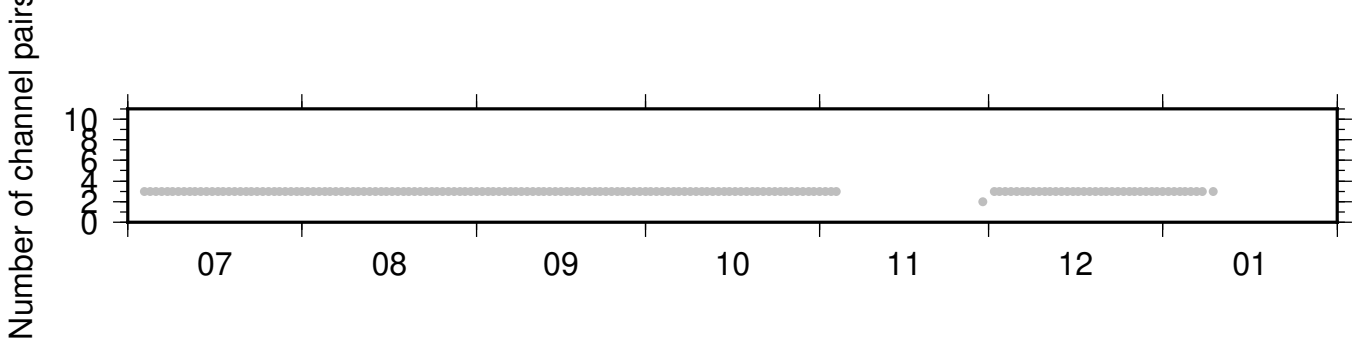
NC_KMR_NC_KSM ZRT 0.10-0.90Hz 011
