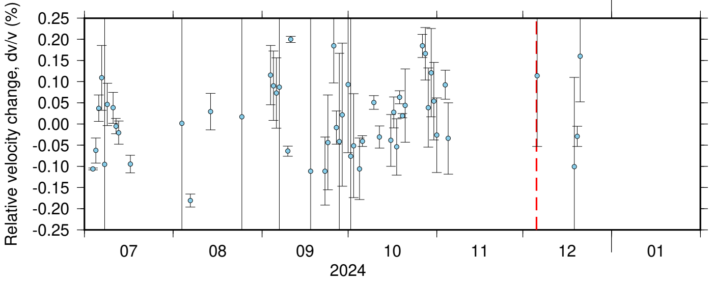
BK_HAYF_NC_KSM ZRT 0.10-0.90Hz 011
