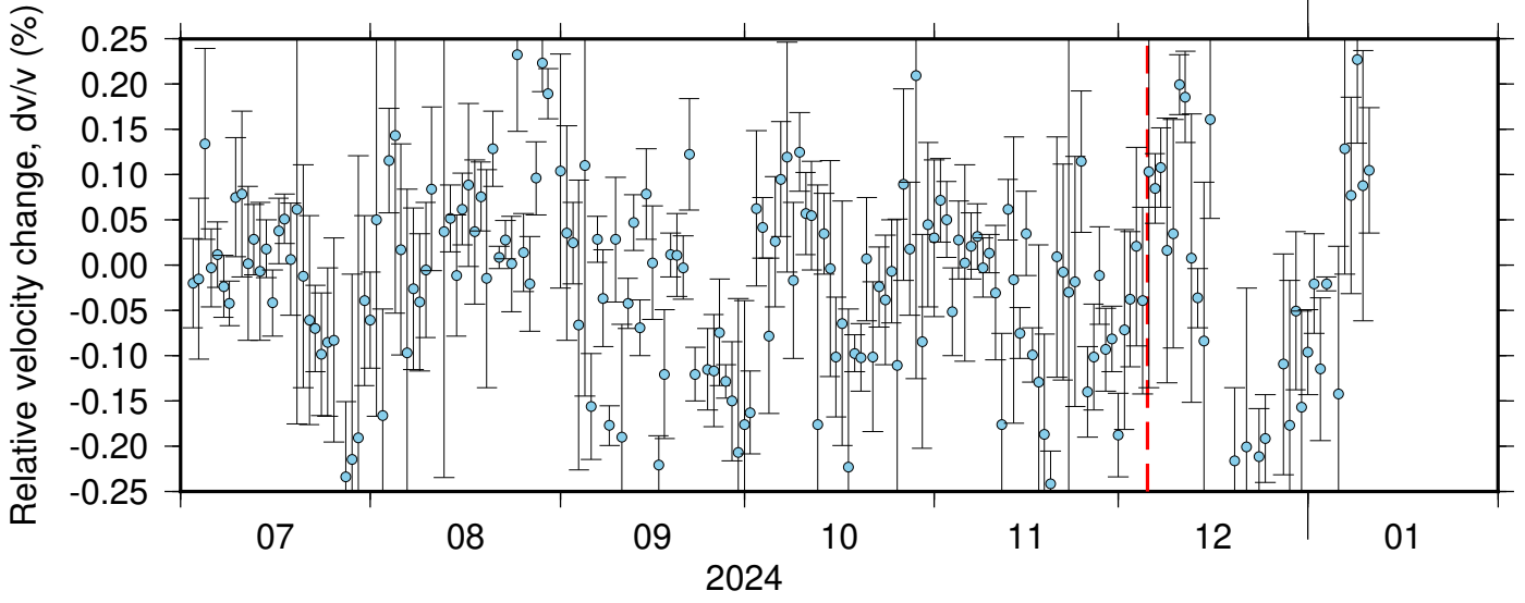
BK_BJES_BK_HAYF ZRT 0.10-0.90Hz 011
