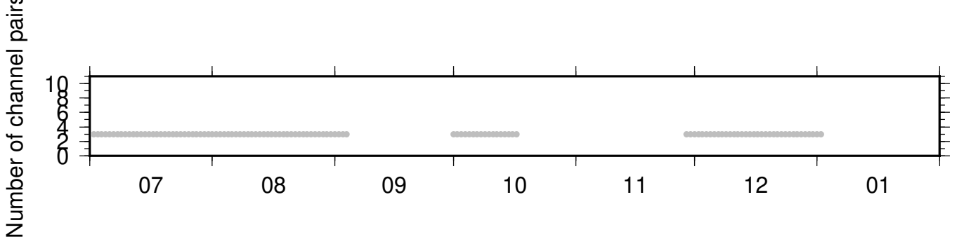
NC_KSM_PB_B046 ZRT 0.10-0.90Hz 011
