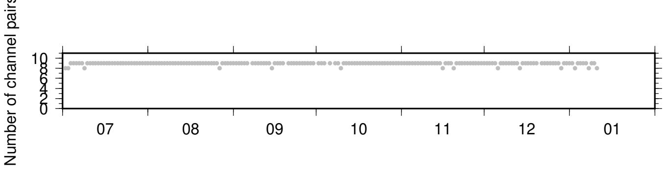
BK_HAYF_BK_RBOW ZRT 0.10-0.90Hz 011
