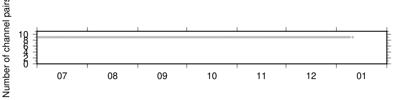
BK_KNEE_NC_KMPB ZRT 0.10-0.90Hz 011
