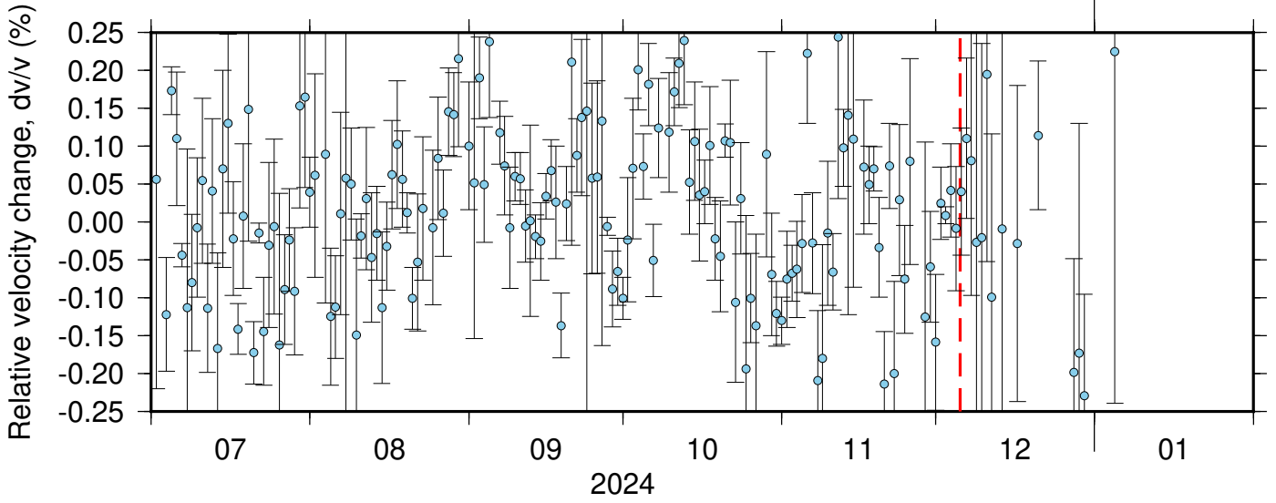
BK_KNEE_NC_KCT ZRT 0.10-0.90Hz 011
