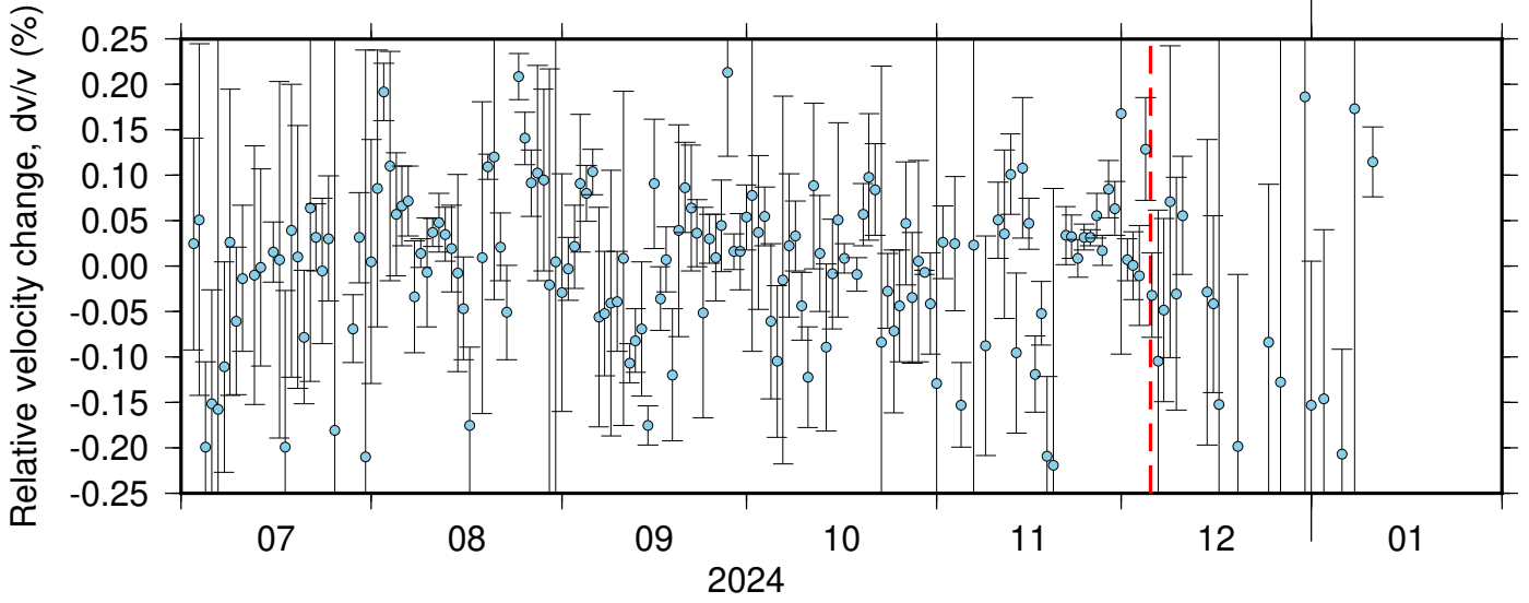
BK_HAYF_NC_KCT ZRT 0.10-0.90Hz 011
