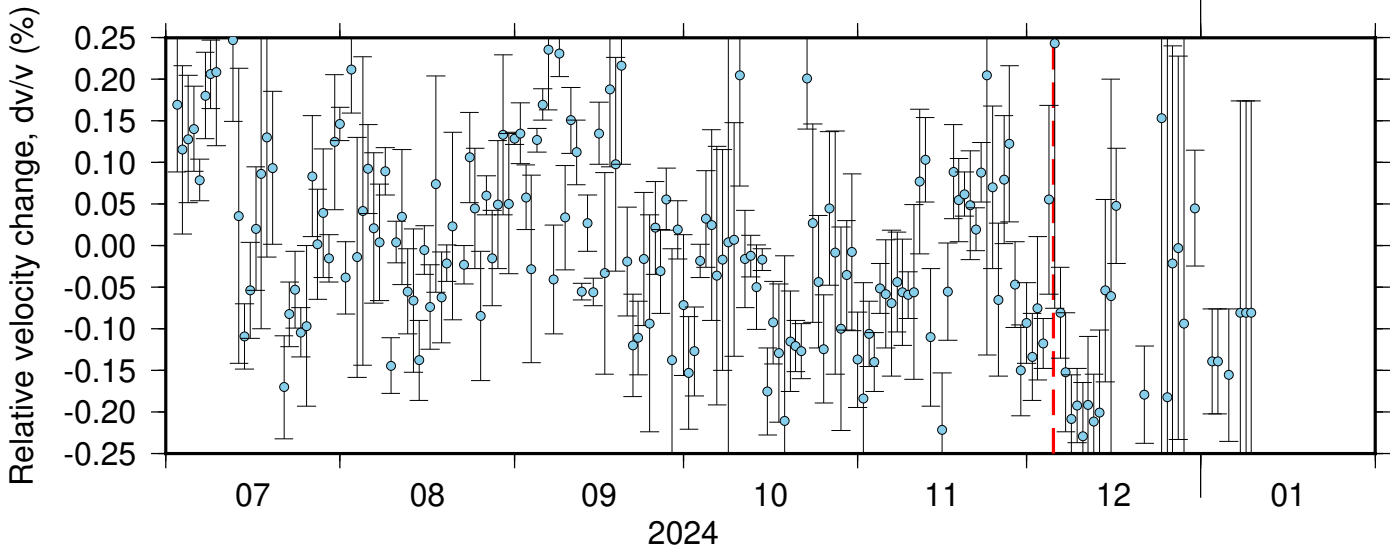
BK_PETL_NC_KPR ZRT 0.10-0.90Hz 011
