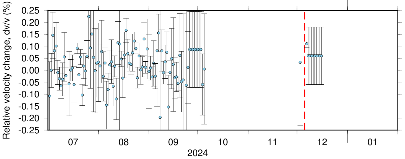
PB_B932_PB_B935 ZRT 0.10-0.90Hz 011
