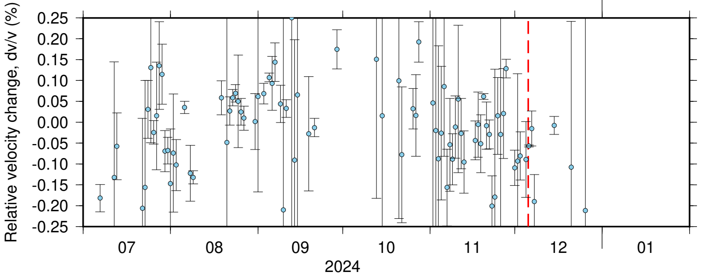
BK_JCC_NC_KPR ZRT 0.10-0.90Hz 011
