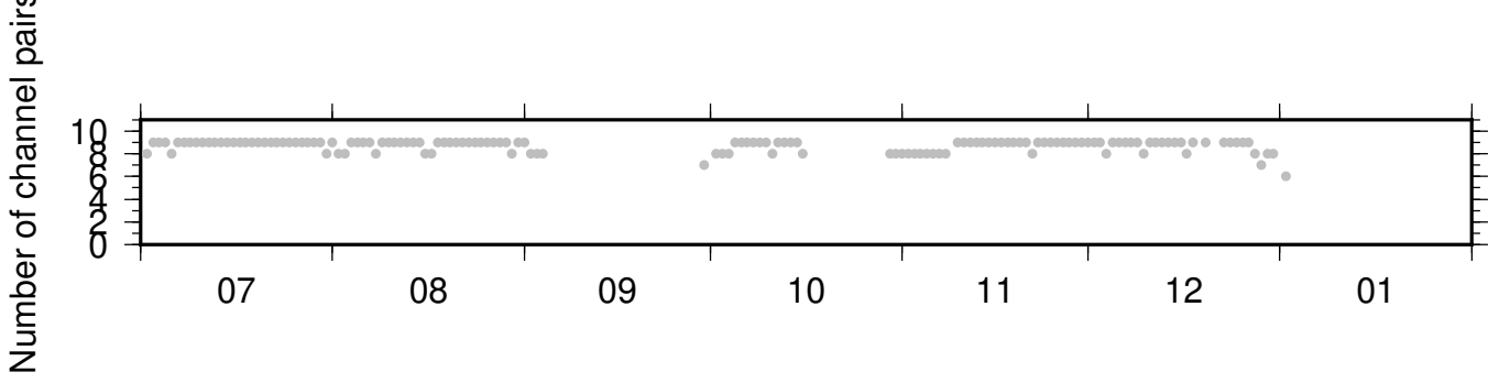
PB_B046_PB_B935 ZRT 0.10-0.90Hz 011
