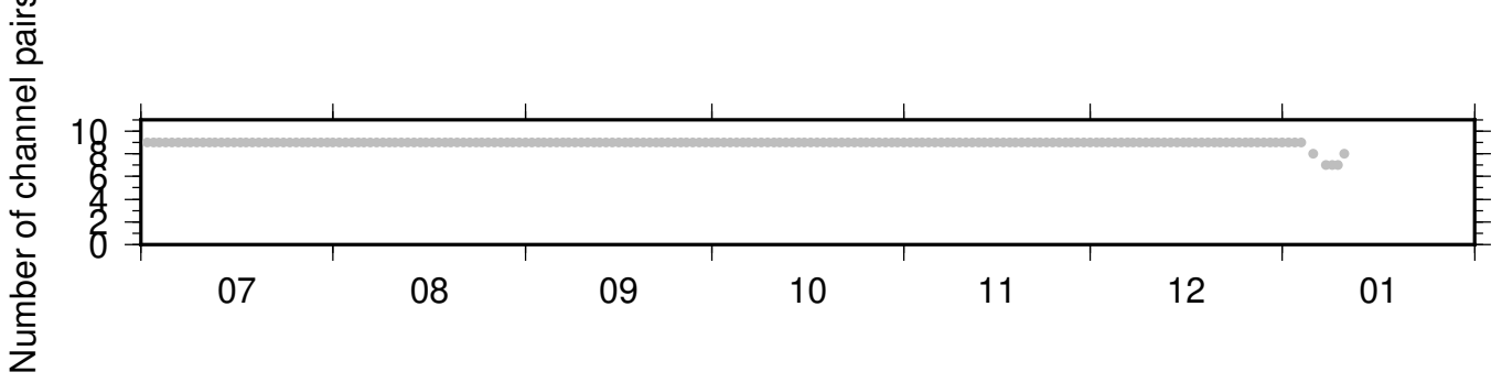
BK_BRIC_BK_PETL ZRT 0.10-0.90Hz 011
