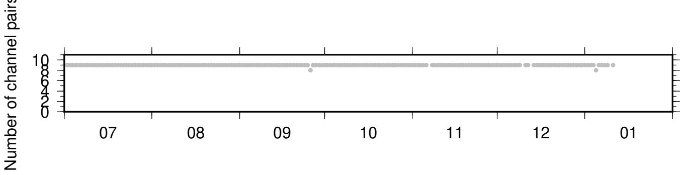
BK_JCC_BK_RBOW ZRT 0.10-0.90Hz 011
