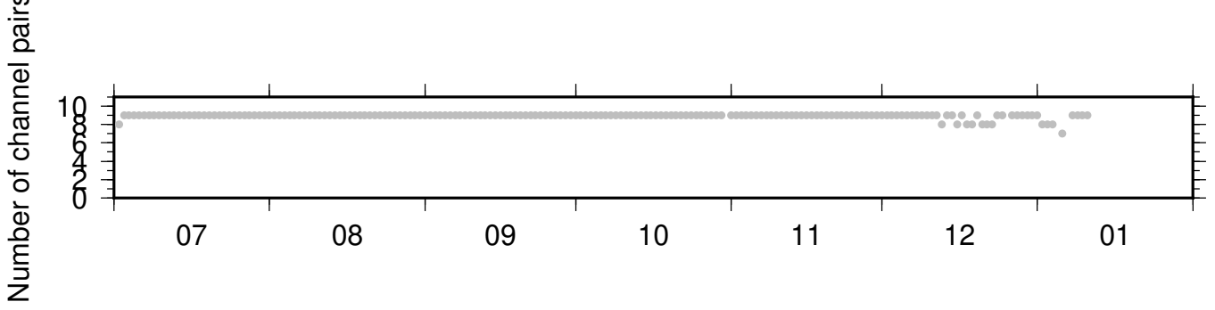
BK_BJES_BK_PETL ZRT 0.10-0.90Hz 011
