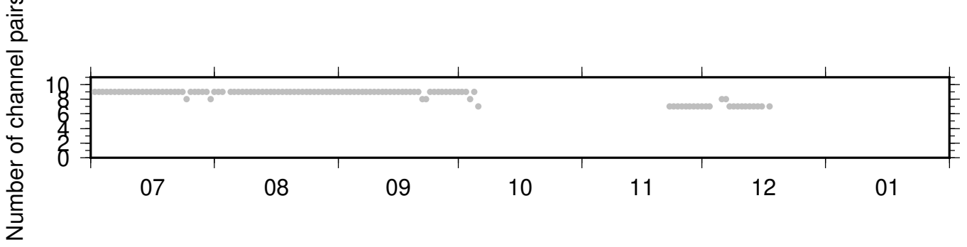
BK_HAYF_PB_B932 ZRT 0.10-0.90Hz 011
