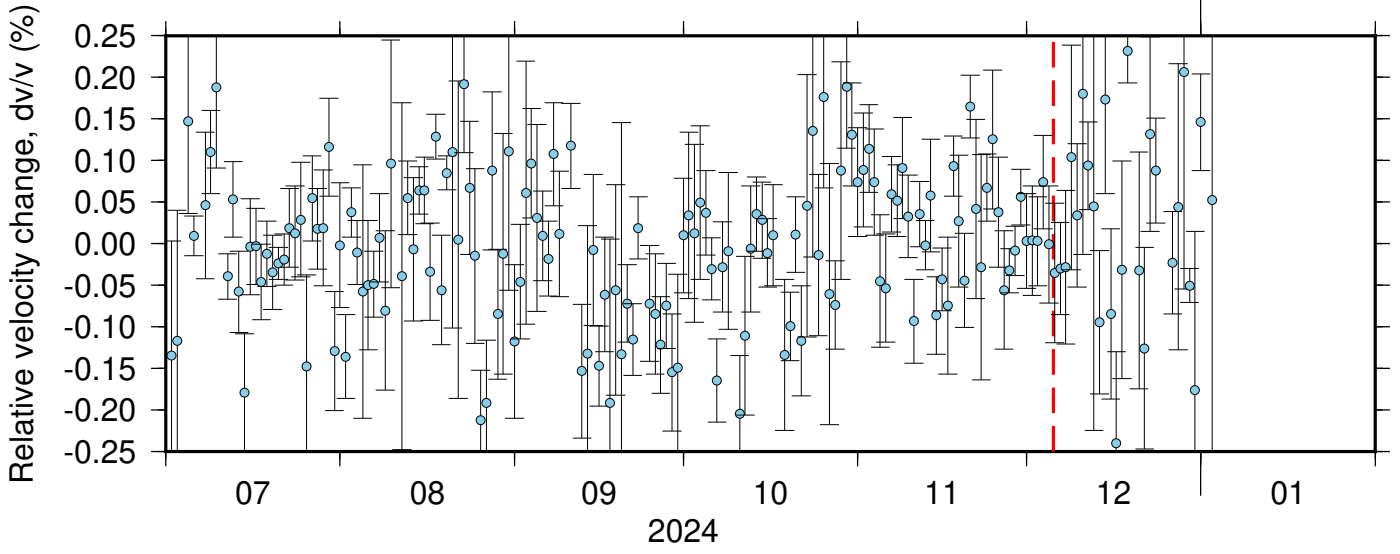
BK_KNEE_PB_B935 ZRT 0.10-0.90Hz 011
