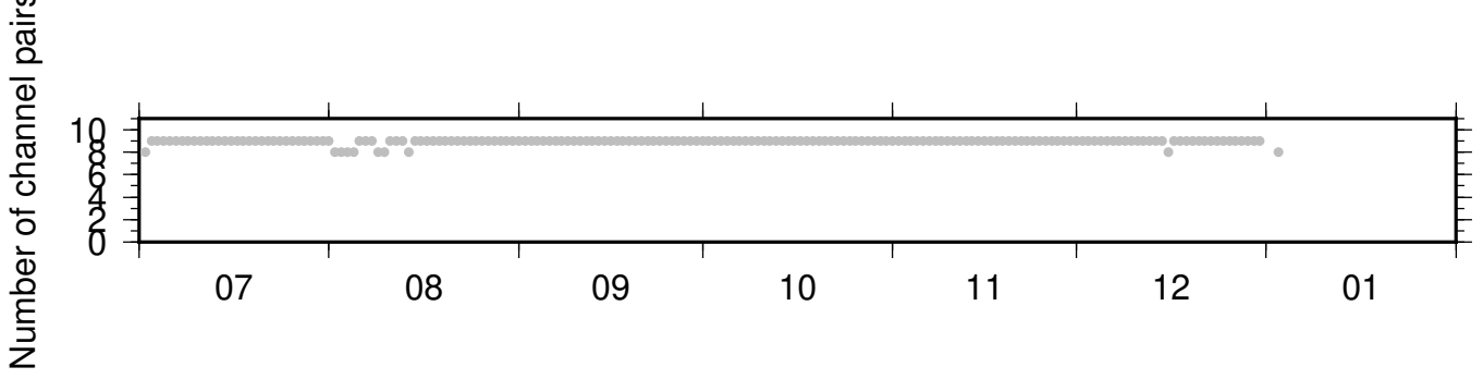
BK_JCC_PB_B935 ZRT 0.10-0.90Hz 011
