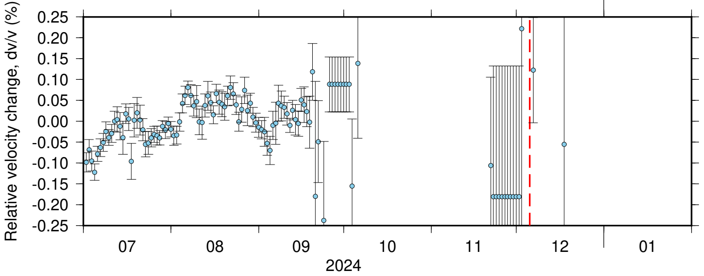
BK_PRDS_PB_B932 ZRT 0.10-0.90Hz 011
