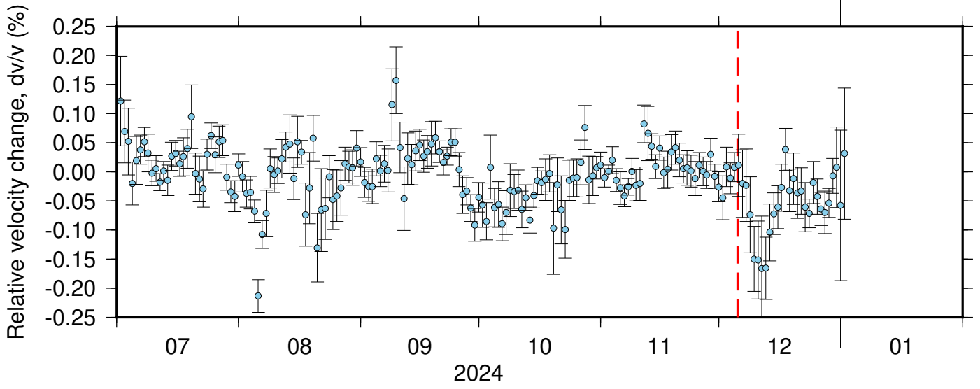
BK_BLAS_PB_B935 ZRT 0.10-0.90Hz 011
