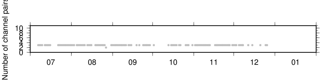
BK_JCC_NC_KPR ZRT 0.10-0.90Hz 011
