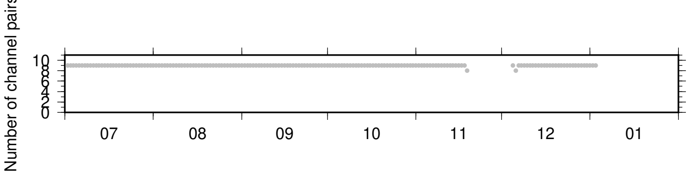
BK_BRIC_PB_B049 ZRT 0.10-0.90Hz 011
