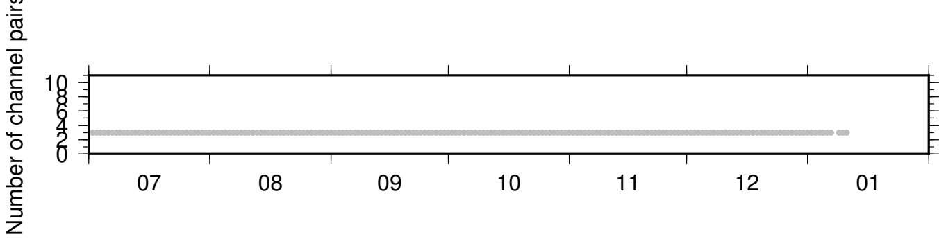
NC_KMR_NC_KPR ZRT 0.10-0.90Hz 011
