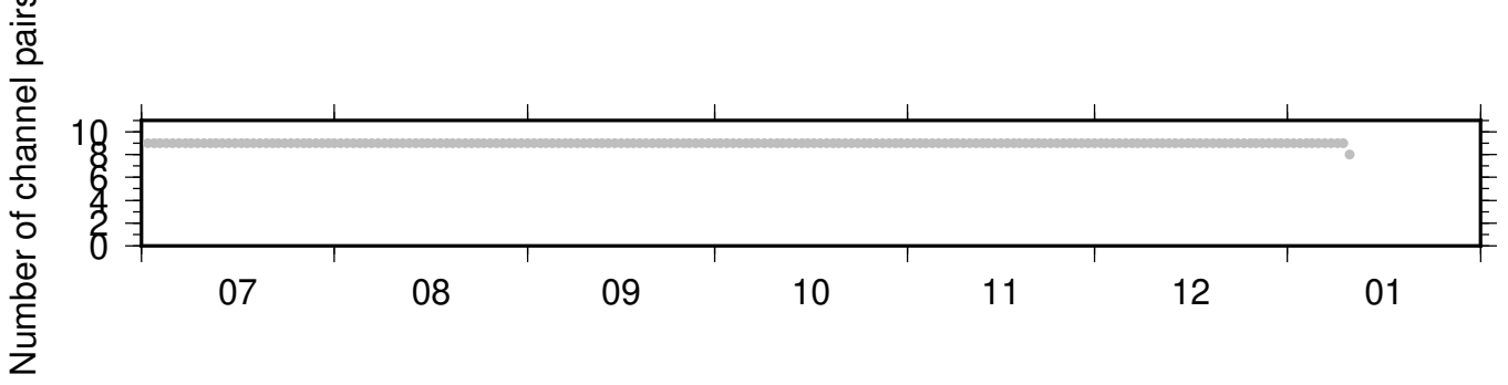
BK_WLKR_NC_KMPB ZRT 0.10-0.90Hz 011
