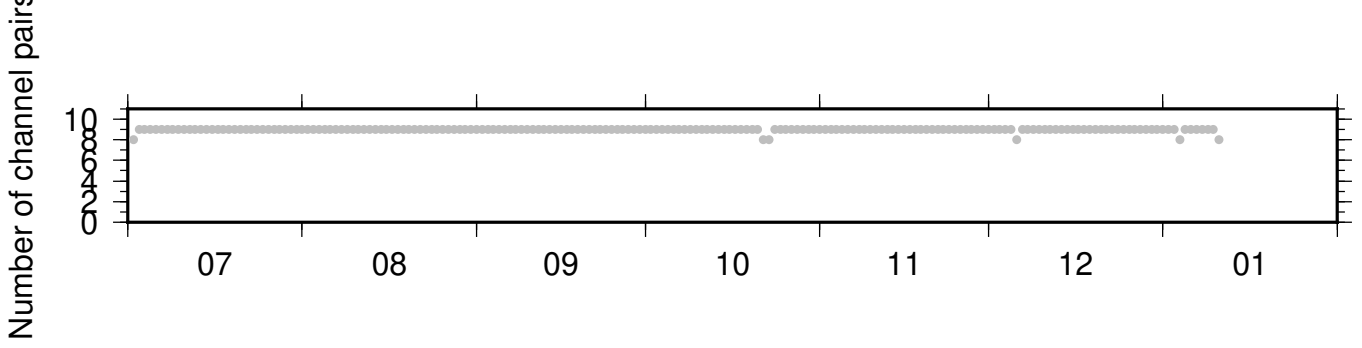
BK_HAYF_BK_KNEE ZRT 0.10-0.90Hz 011
