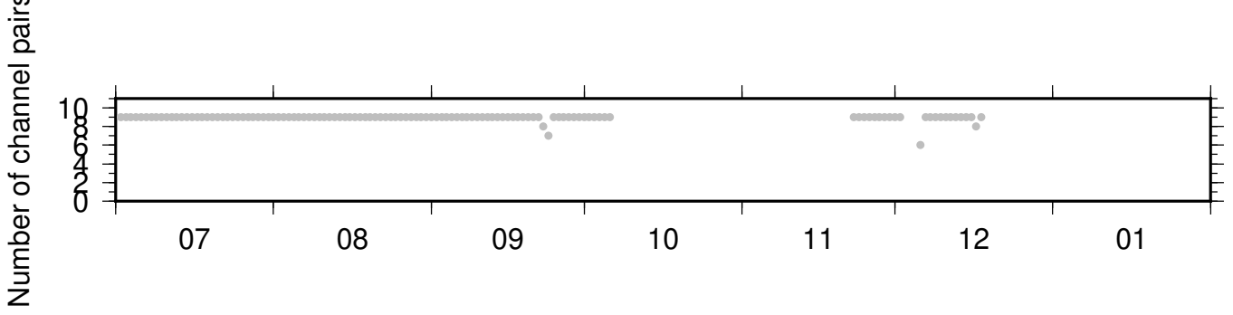
BK_SPRL_PB_B932 ZRT 0.10-0.90Hz 011
