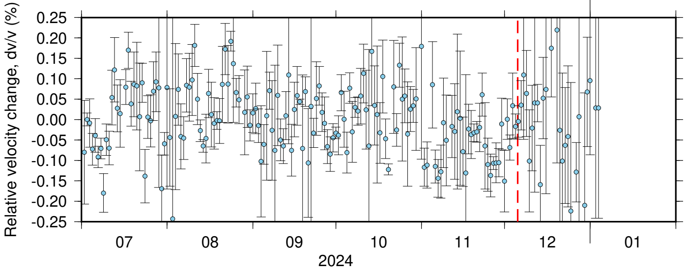
BK_BJES_BK_PETL ZRT 0.10-0.90Hz 011
