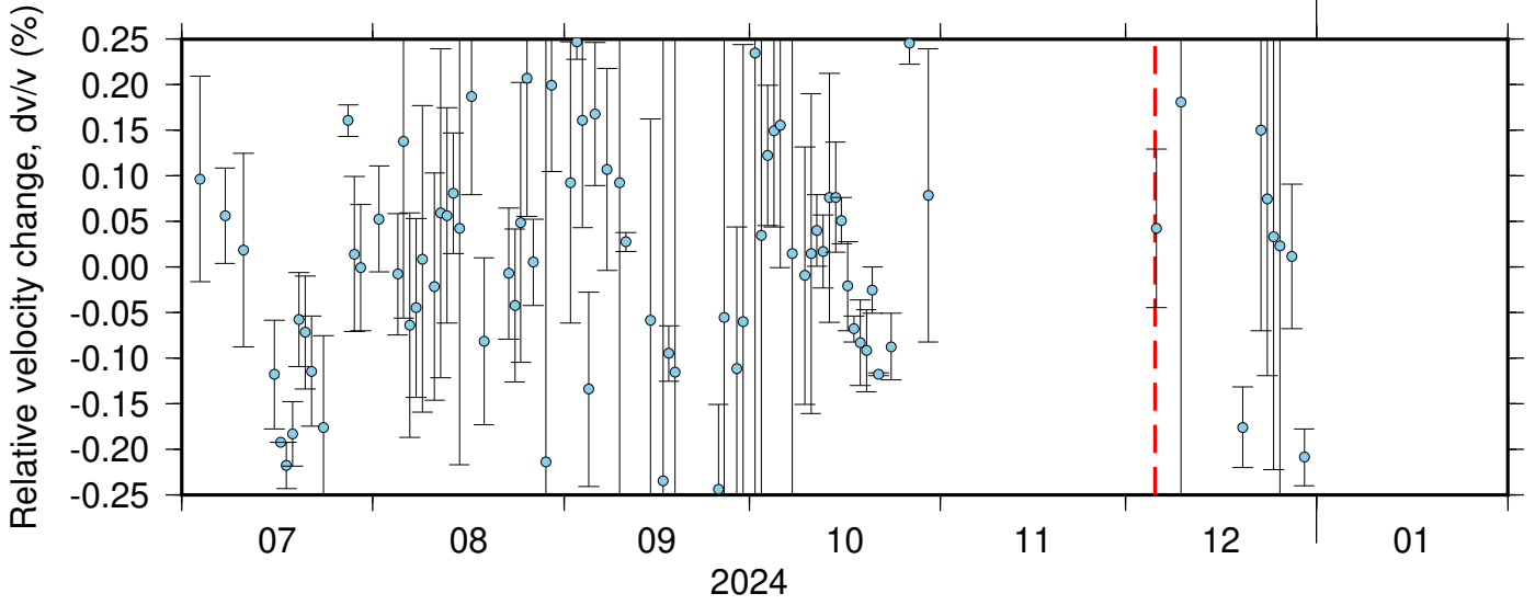
NC_KSM_PB_B935 ZRT 0.10-0.90Hz 011
