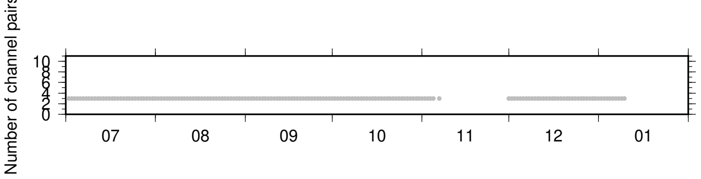
BK_BRIC_NC_KSM ZRT 0.10-0.90Hz 011
