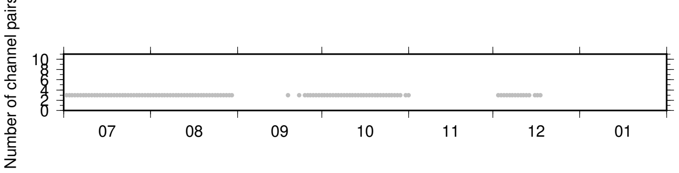
NC_KSM_PB_B045 ZRT 0.10-0.90Hz 011
