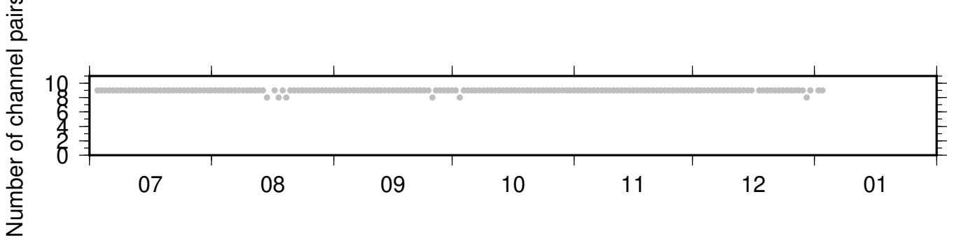
BK_JCC_PB_B047 ZRT 0.10-0.90Hz 011
