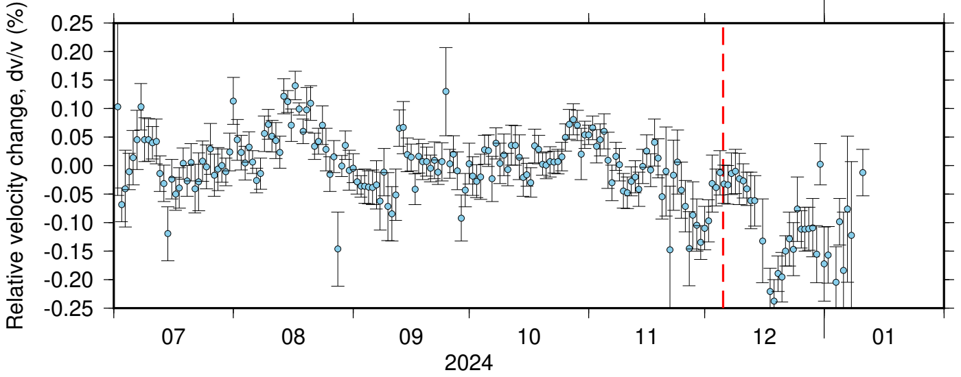
BK_BRIC_BK_RBOW ZRT 0.10-0.90Hz 011
