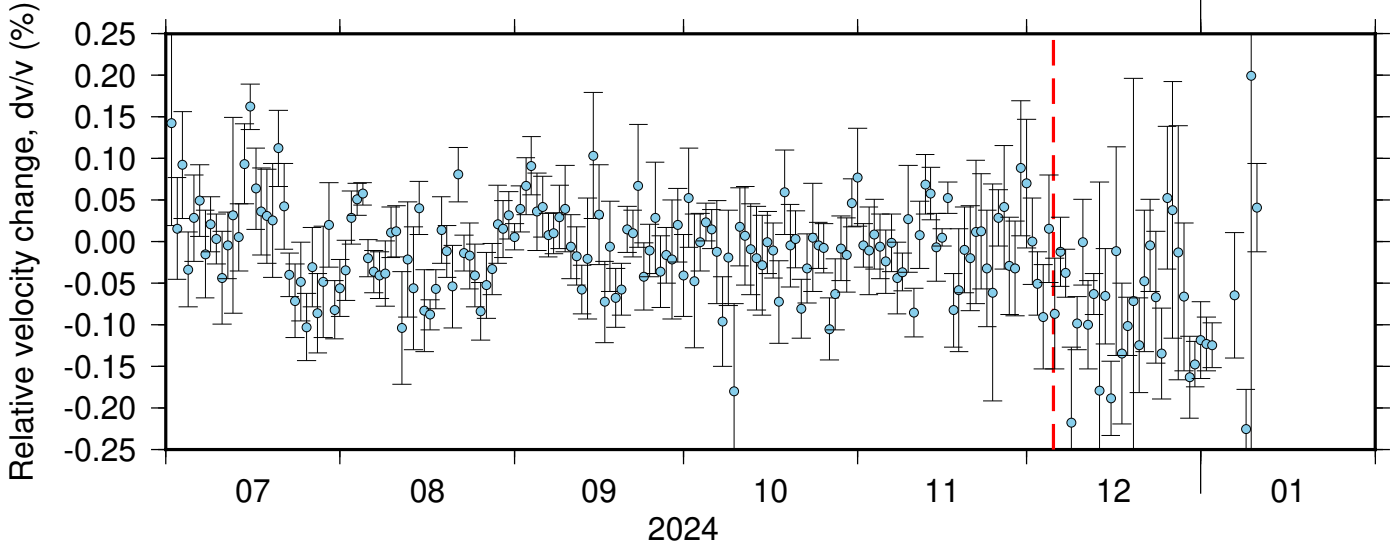
BK_BRIC_NC_KMPB ZRT 0.10-0.90Hz 011
