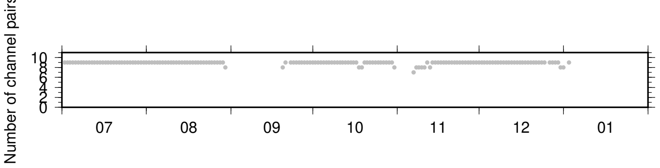
BK_KNEE_PB_B045 ZRT 0.10-0.90Hz 011
