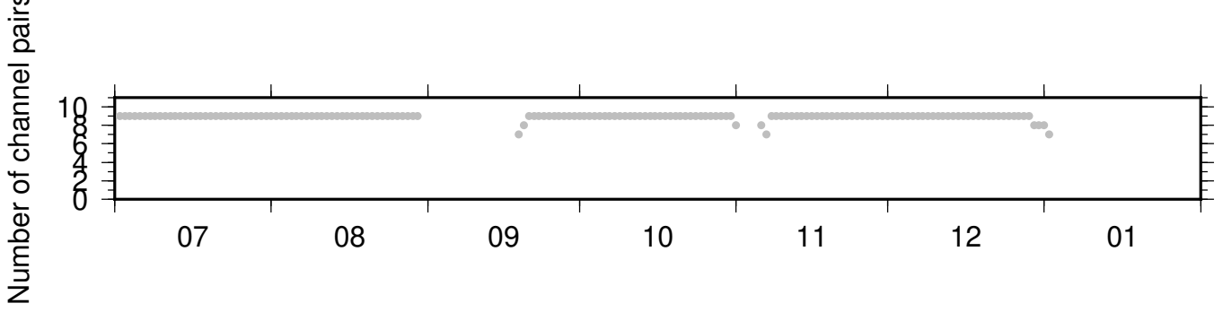
BK_BLAS_PB_B045 ZRT 0.10-0.90Hz 011
