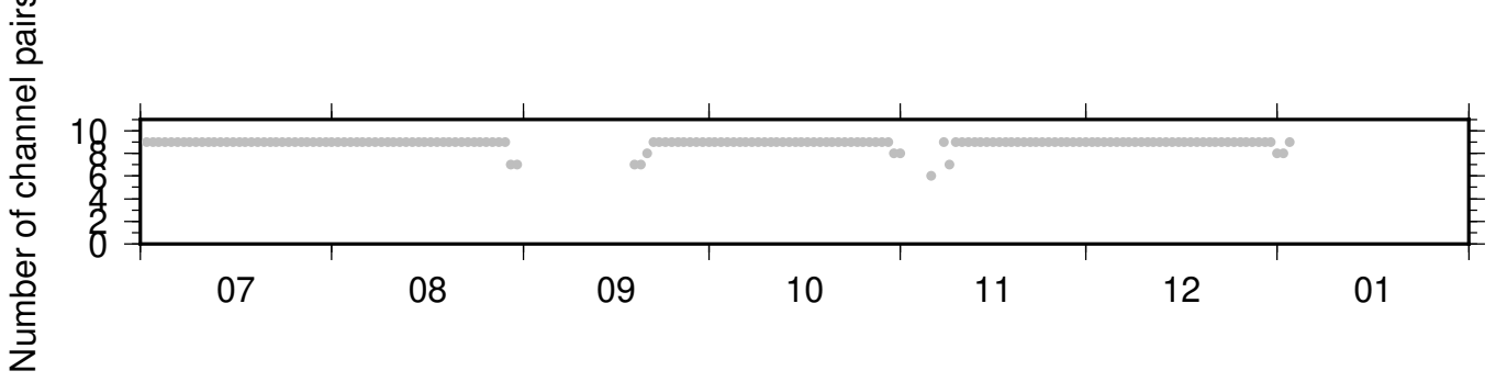
BK_WLKR_PB_B045 ZRT 0.10-0.90Hz 011
