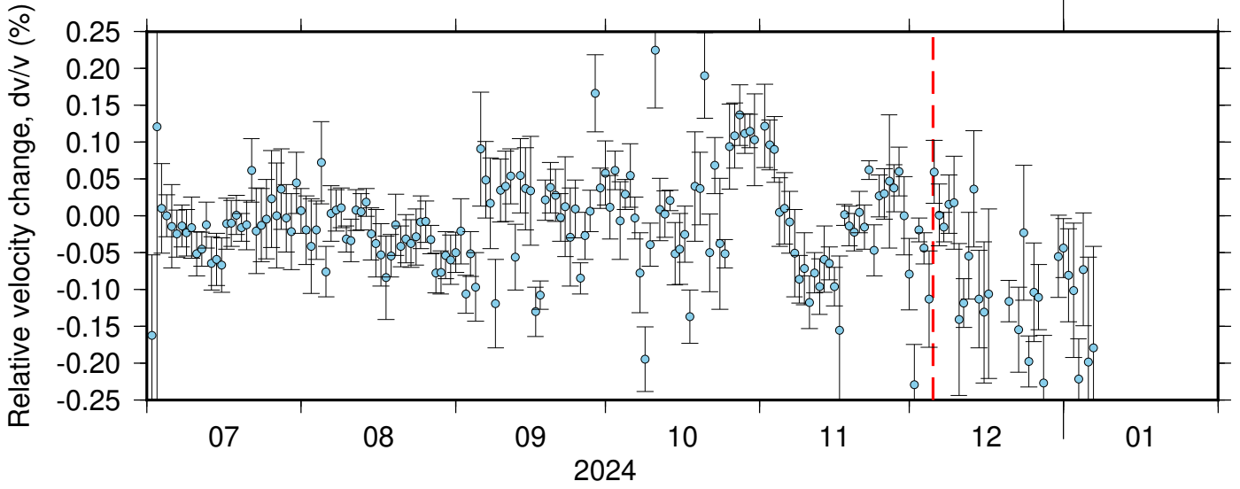
BK_GHOP_BK_WLKR ZRT 0.10-0.90Hz 011
