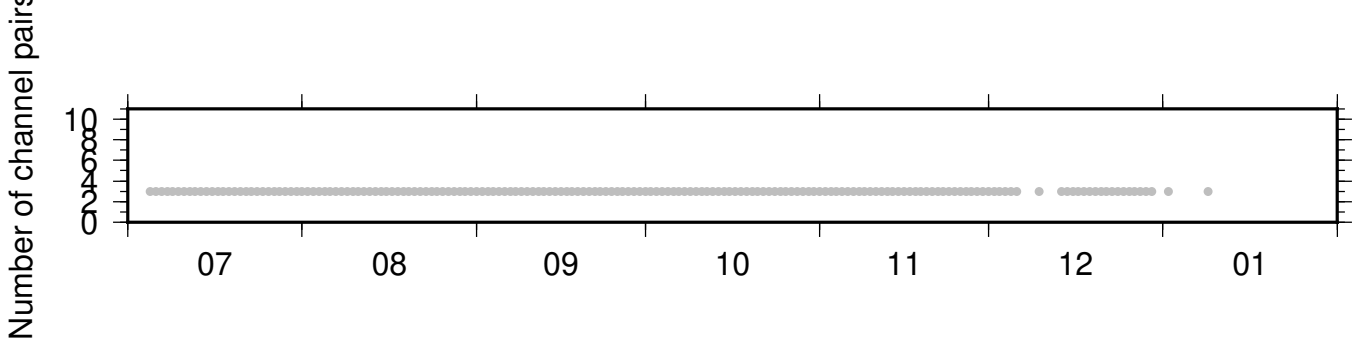
BK_KNEE_NC_KCR ZRT 0.10-0.90Hz 011
