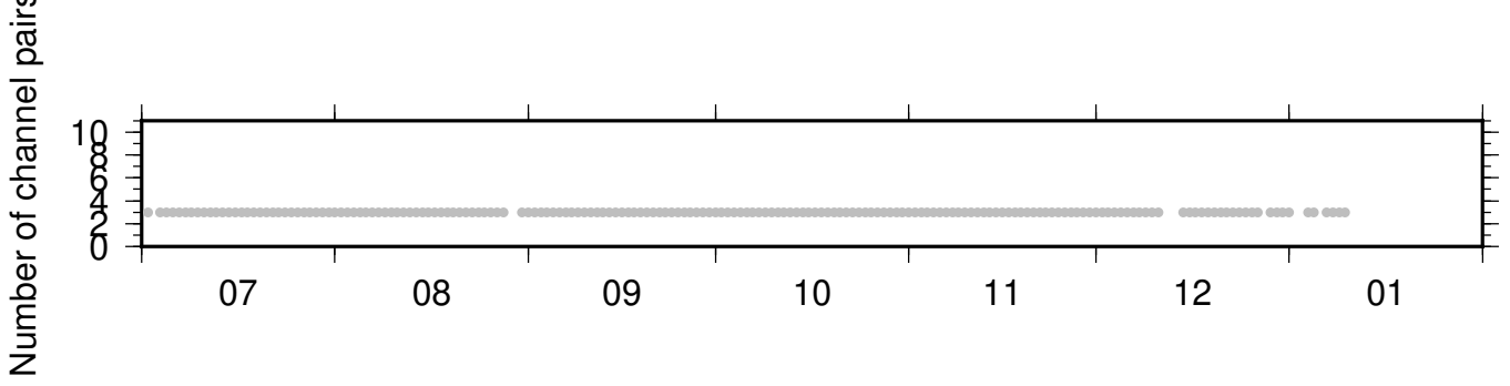
NC_KCR_NC_KMR ZRT 0.10-0.90Hz 011
