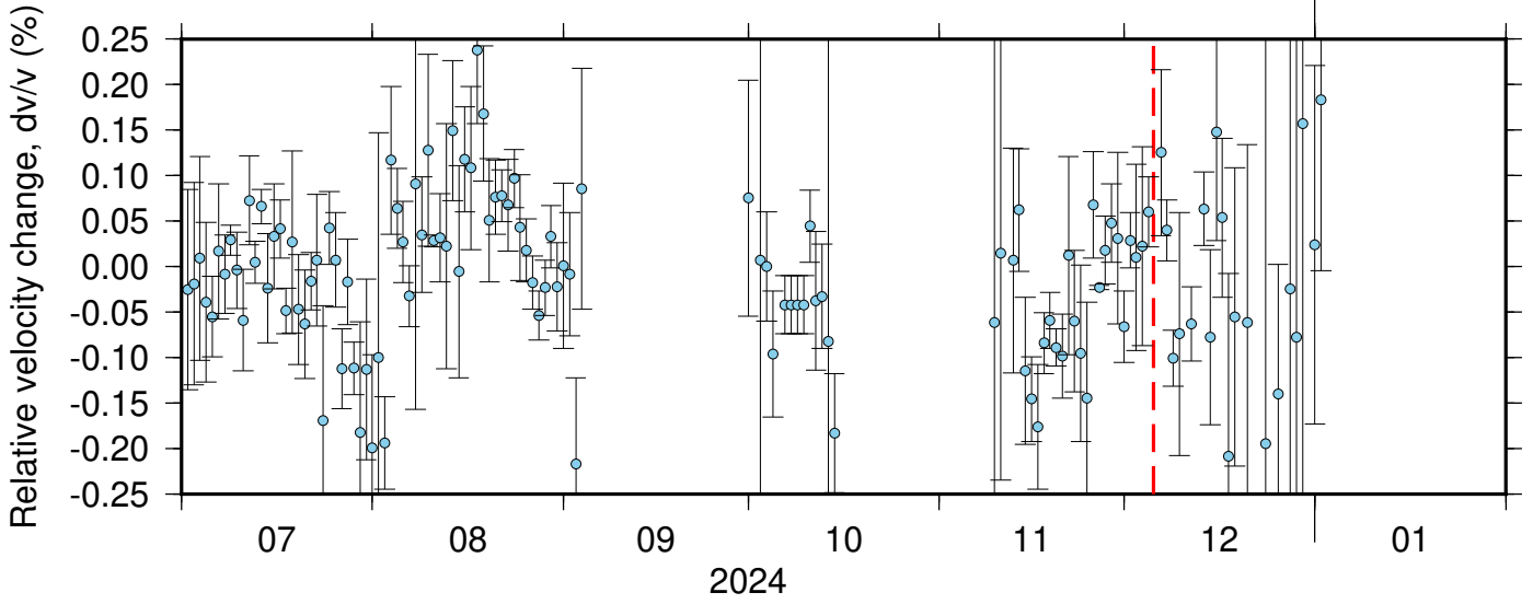
NC_KMR_PB_B046 ZRT 0.10-0.90Hz 011
