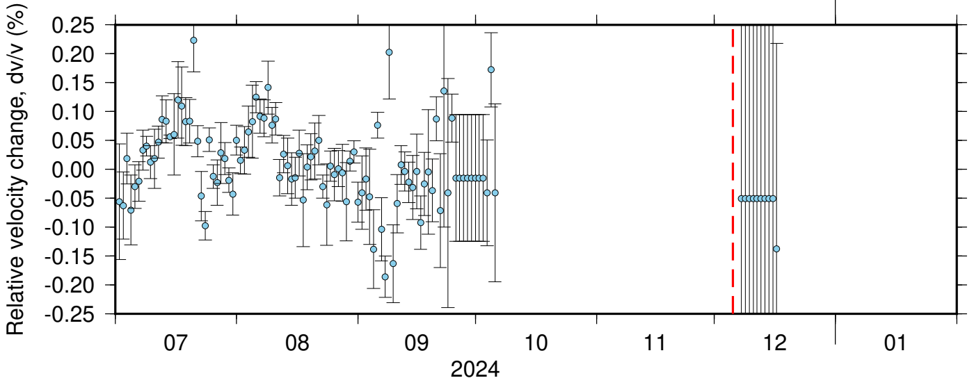
PB_B049_PB_B932 ZRT 0.10-0.90Hz 011
