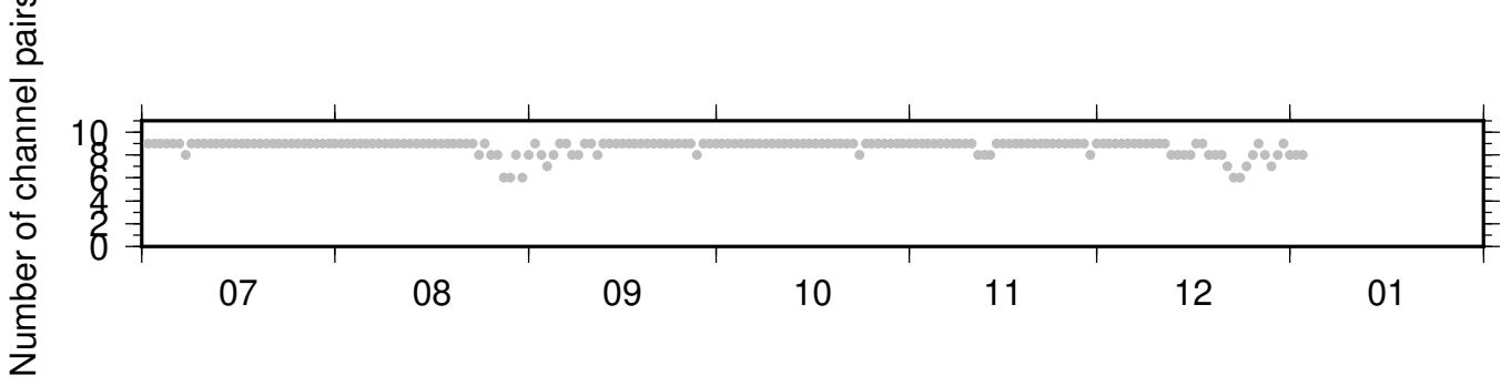
BK_SPRL_PB_B934 ZRT 0.10-0.90Hz 011
