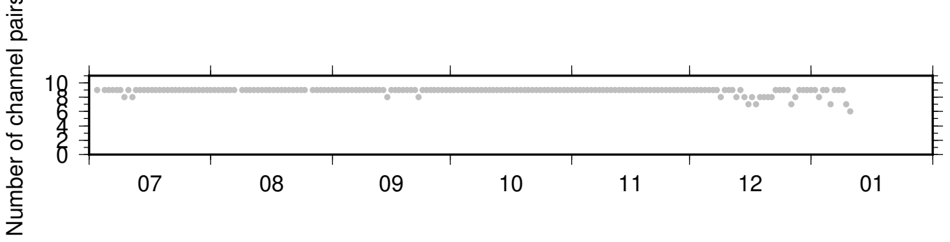
BK_KNEE_NC_KMR ZRT 0.10-0.90Hz 011
