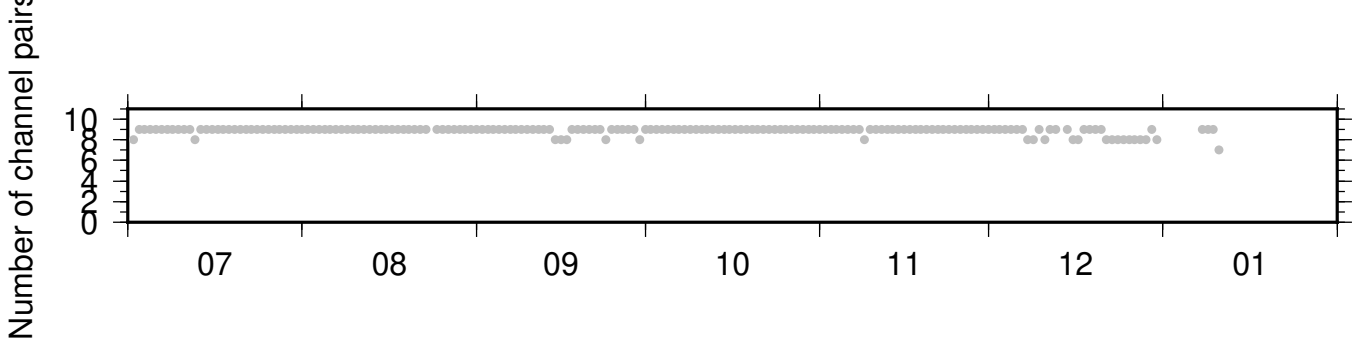
BK_KNEE_BK_PETL ZRT 0.10-0.90Hz 011
