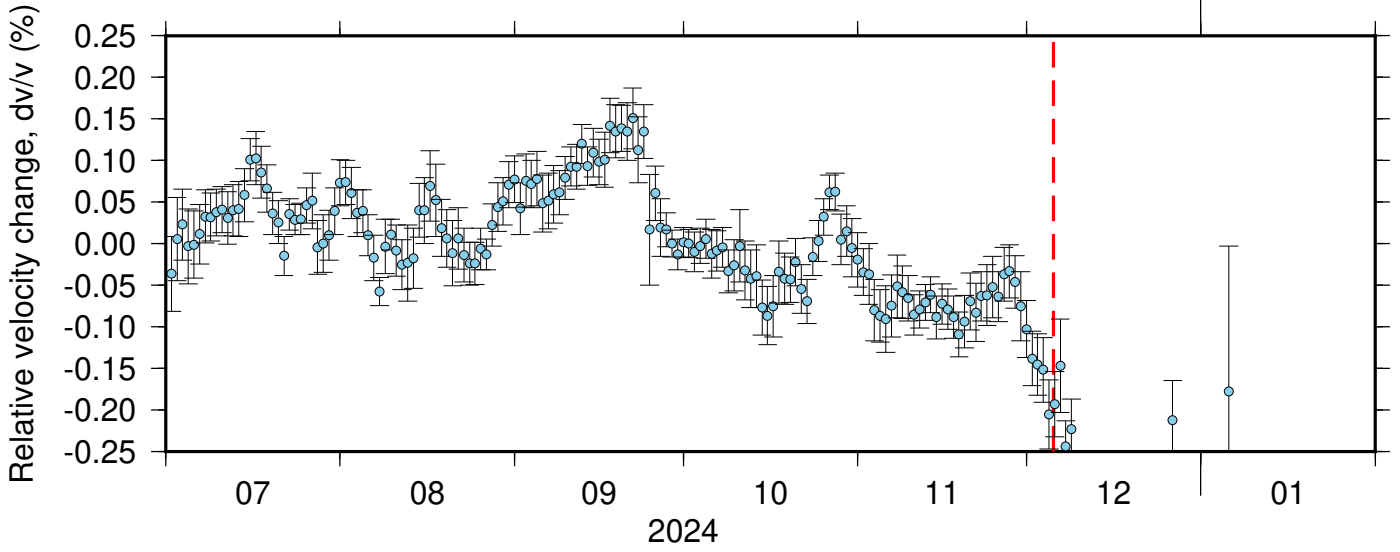
BK_PETL_BK_WLKR ZRT 0.10-0.90Hz 011
