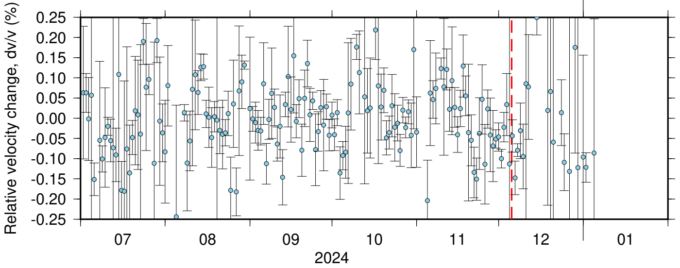
BK_JCC_BK_PETL ZRT 0.10-0.90Hz 011
