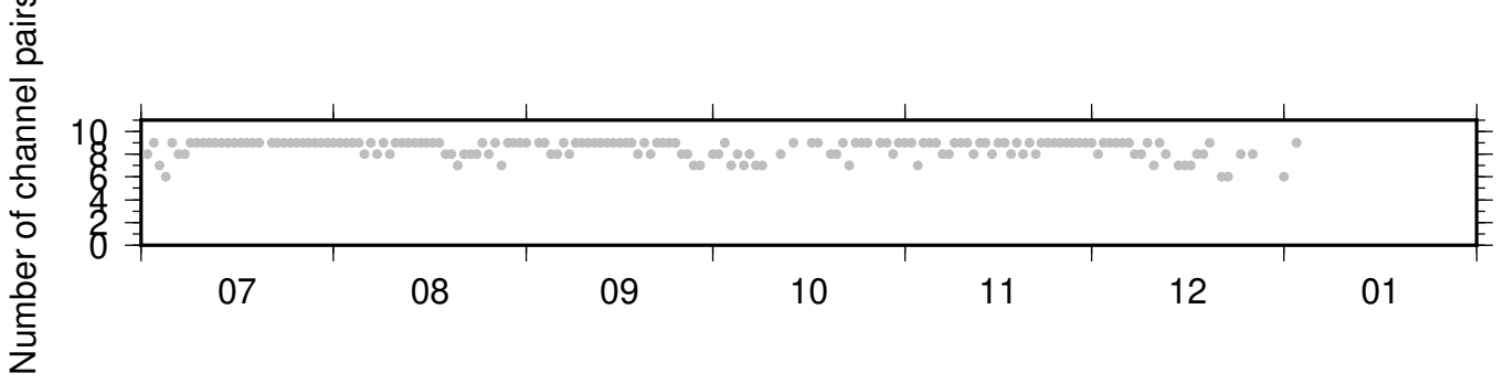
BK_JCC_PB_B934 ZRT 0.10-0.90Hz 011
