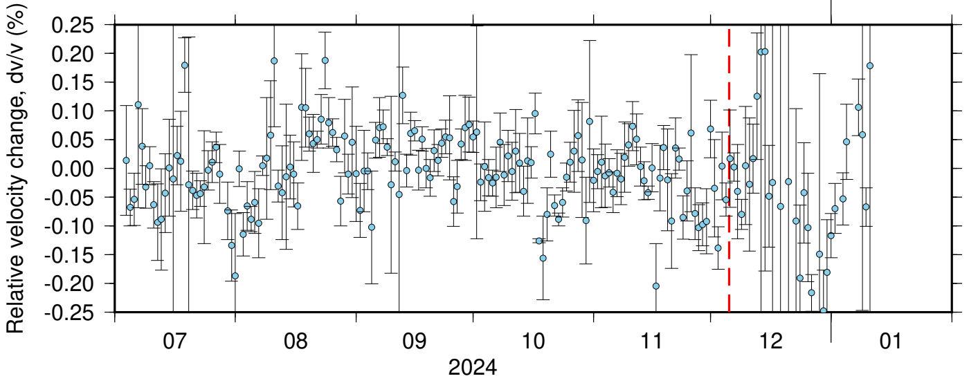
BK_BJES_BK_BRIC ZRT 0.10-0.90Hz 011
