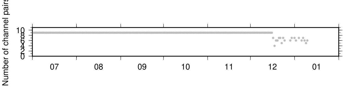
BK_BJES_NC_KCT ZRT 0.10-0.90Hz 011
