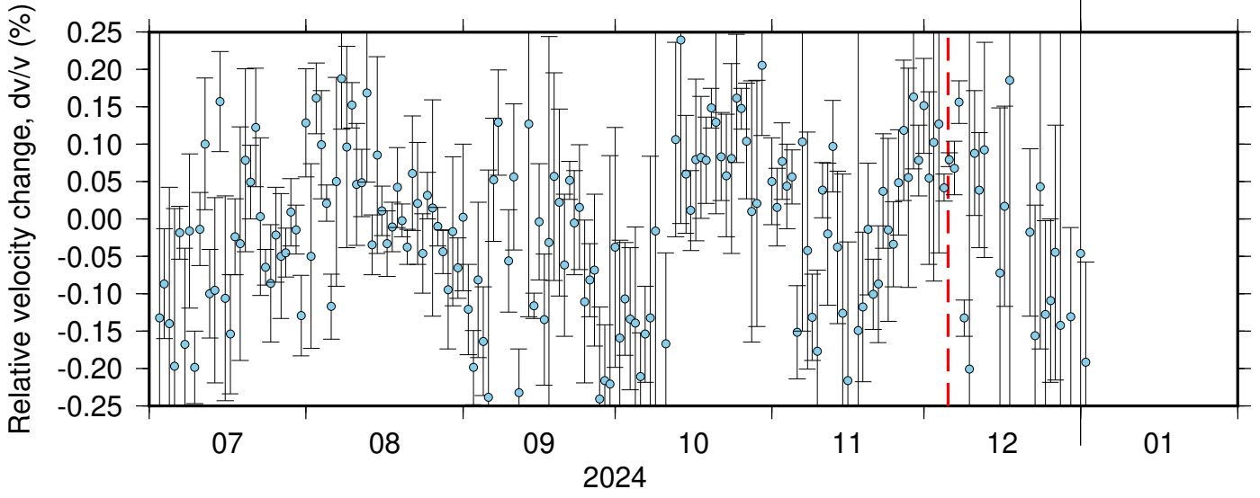
BK_PRDS_PB_B935 ZRT 0.10-0.90Hz 011
