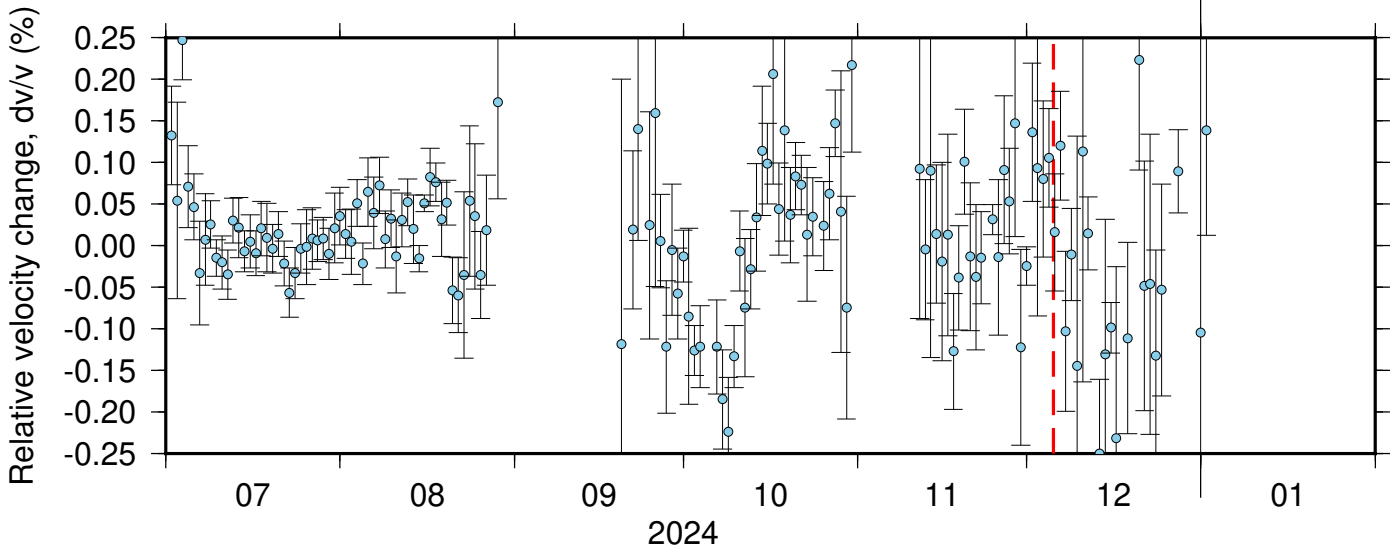
PB_B045_PB_B047 ZRT 0.10-0.90Hz 011
