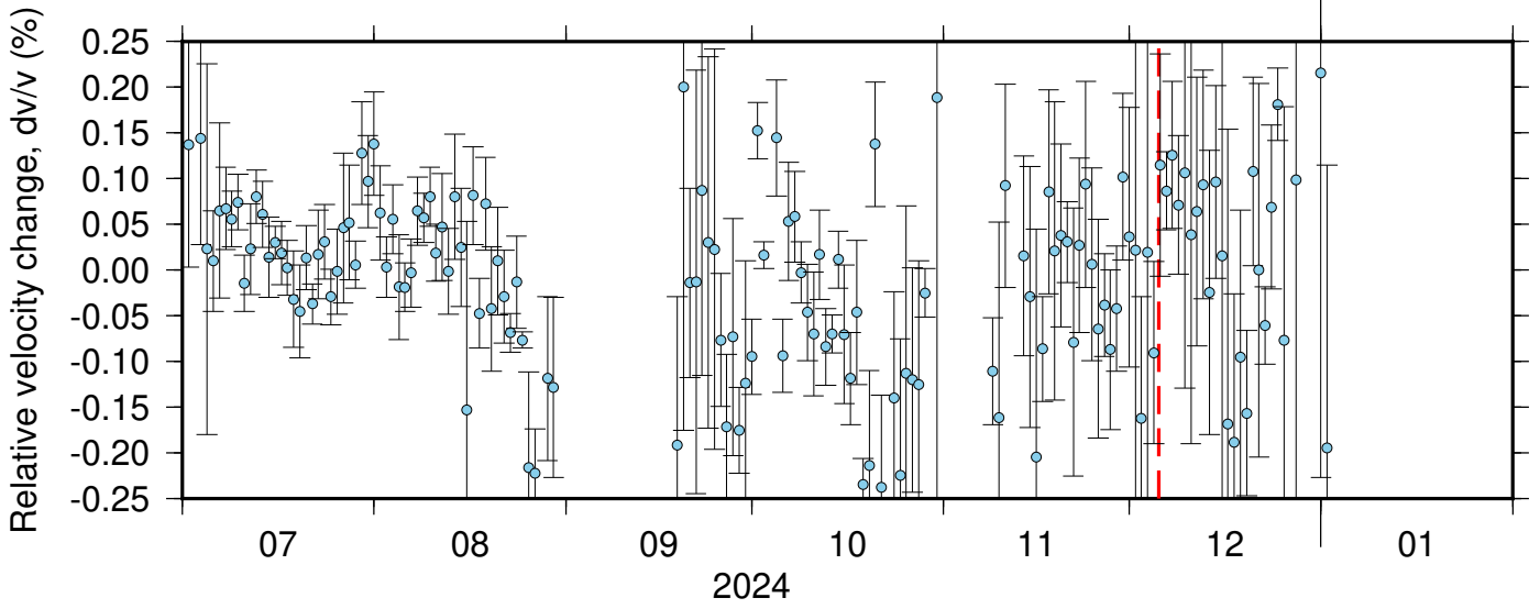
BK_BLAS_PB_B045 ZRT 0.10-0.90Hz 011
