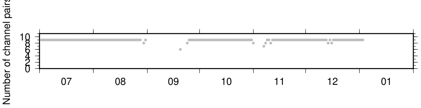
BK_JCC_PB_B045 ZRT 0.10-0.90Hz 011
