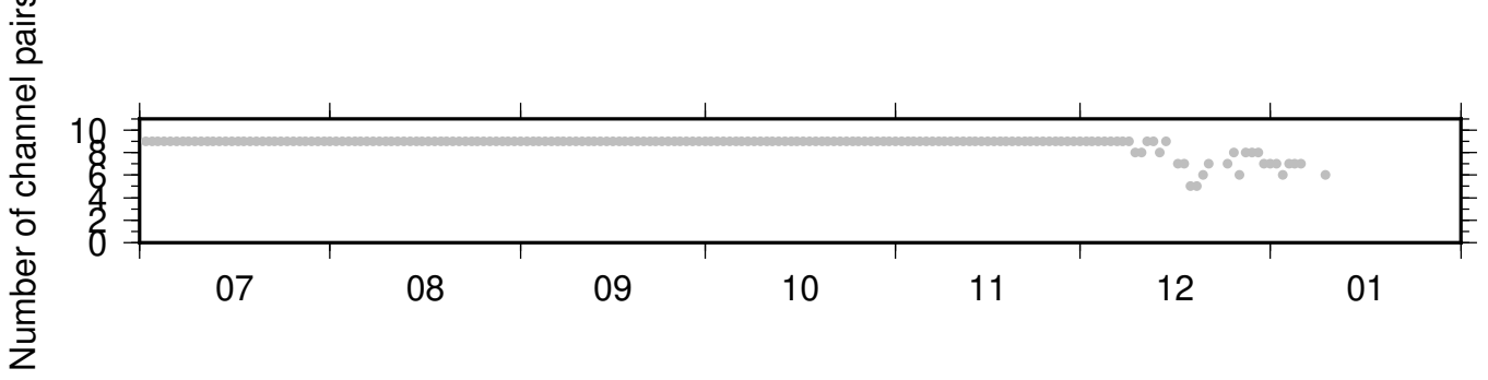
BK_KNEE_NC_KCT ZRT 0.10-0.90Hz 011
