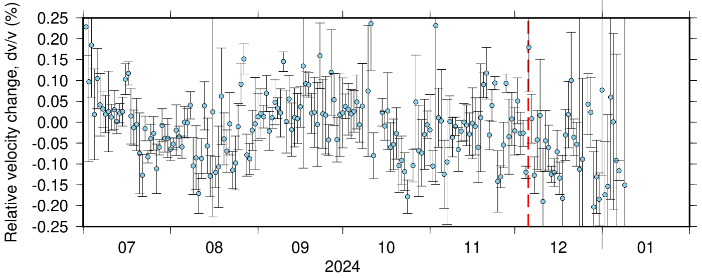
BK_BRIC_BK_WLKR ZRT 0.10-0.90Hz 011
