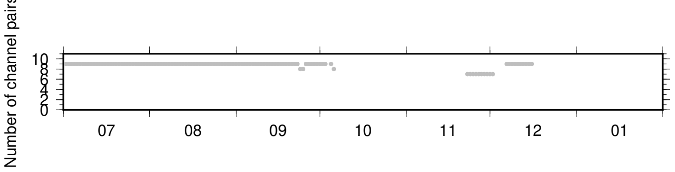
BK_BJES_PB_B932 ZRT 0.10-0.90Hz 011
