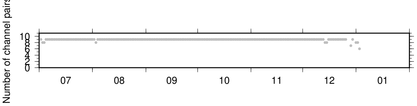
PB_B047_PB_B935 ZRT 0.10-0.90Hz 011
