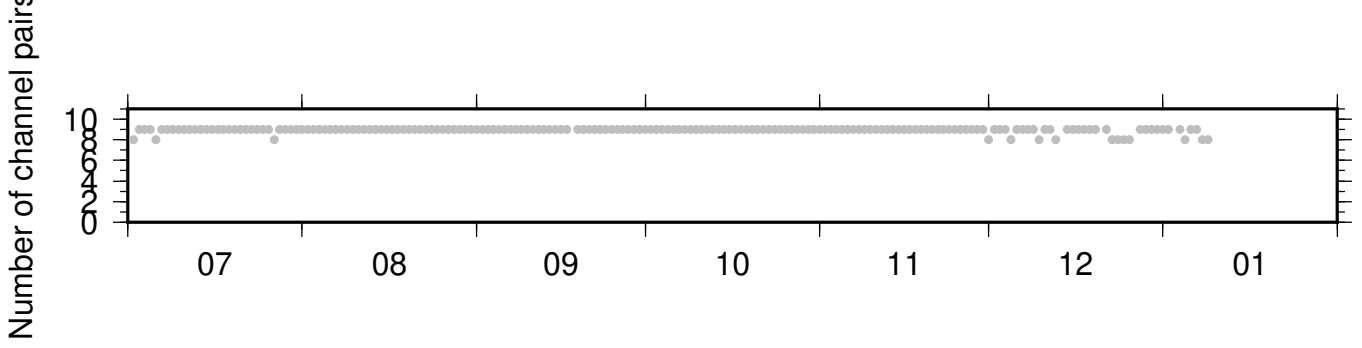
BK_KNEE_BK_SPRL ZRT 0.10-0.90Hz 011
