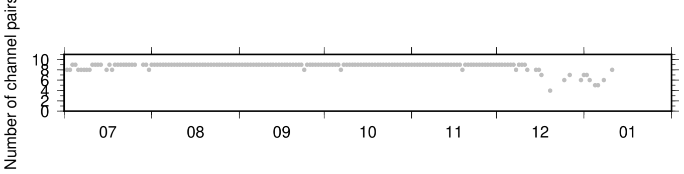
BK_HAYF_NC_KCT ZRT 0.10-0.90Hz 011
