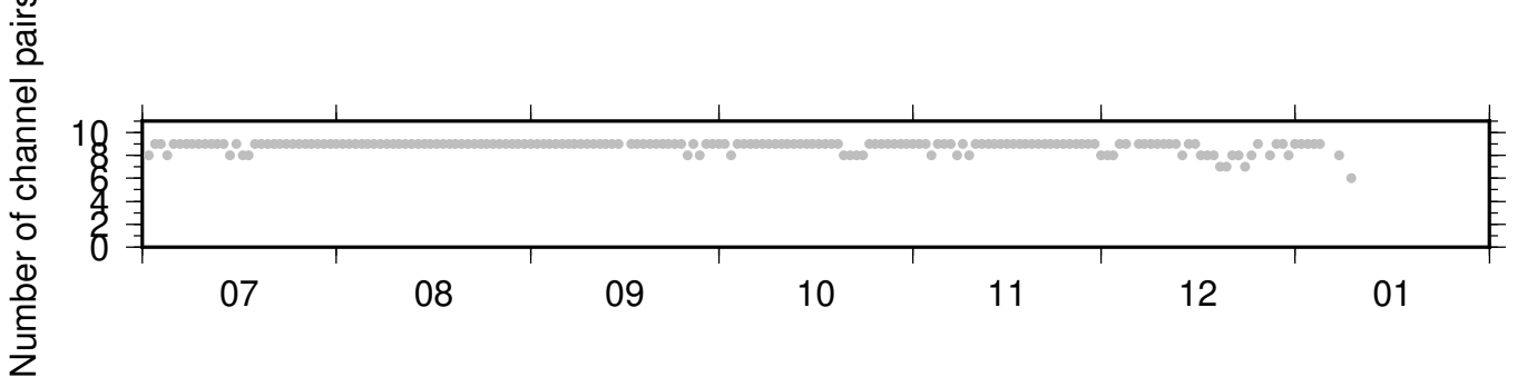
BK_JCC_BK_SPRL ZRT 0.10-0.90Hz 011
