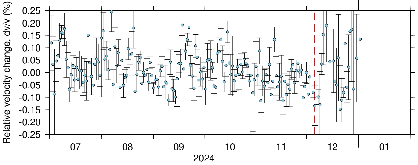
BK_BJES_PB_B047 ZRT 0.10-0.90Hz 011
