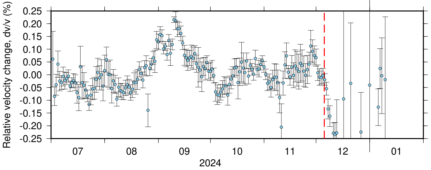
BK_WLKR_NC_KCT ZRT 0.10-0.90Hz 011
