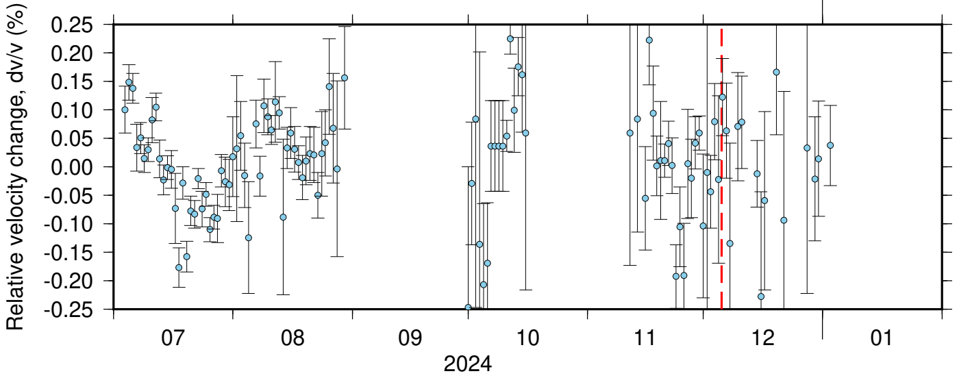
PB_B045_PB_B046 ZRT 0.10-0.90Hz 011
