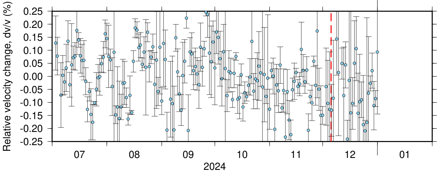
BK_BRIC_PB_B935 ZRT 0.10-0.90Hz 011
