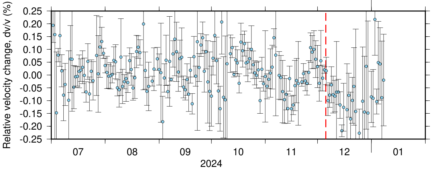
BK_SPRL_BK_WLKR ZRT 0.10-0.90Hz 011
