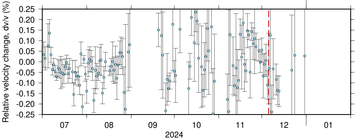
BK_PETL_PB_B045 ZRT 0.10-0.90Hz 011
