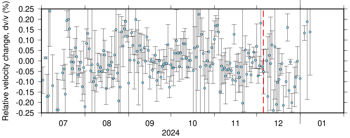
BK_JCC_BK_PRDS ZRT 0.10-0.90Hz 011
