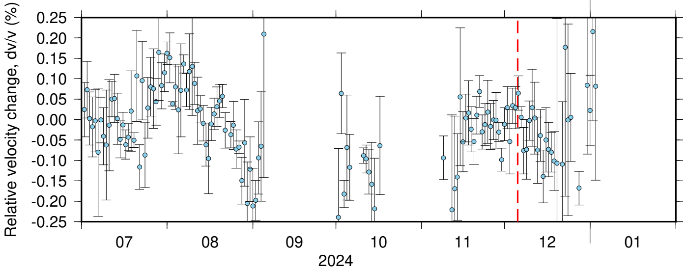
BK_SPRL_PB_B046 ZRT 0.10-0.90Hz 011
