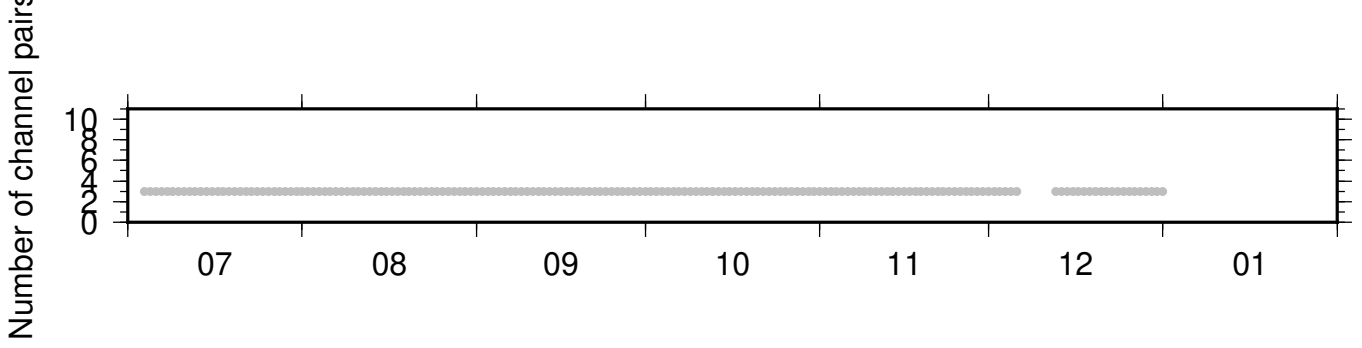
NC_KCR_PB_B935 ZRT 0.10-0.90Hz 011
