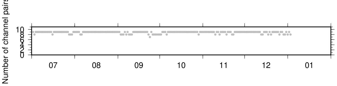
NC_KMR_PB_B934 ZRT 0.10-0.90Hz 011
