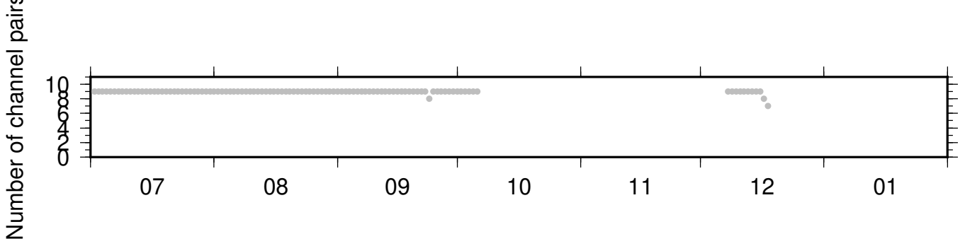
BK_BRIC_PB_B932 ZRT 0.10-0.90Hz 011
