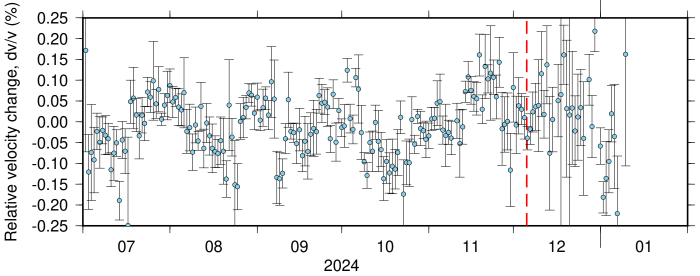
BK_BJES_BK_BLAS ZRT 0.10-0.90Hz 011
