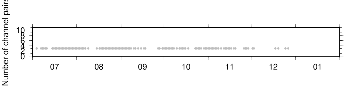
BK_KNEE_NC_KBU ZRT 0.10-0.90Hz 011
