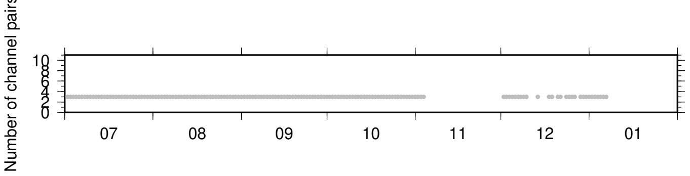
BK_BJES_NC_KSM ZRT 0.10-0.90Hz 011
