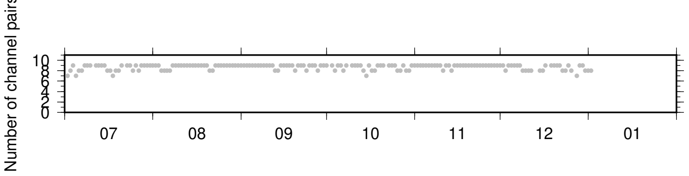
BK_PETL_PB_B934 ZRT 0.10-0.90Hz 011
