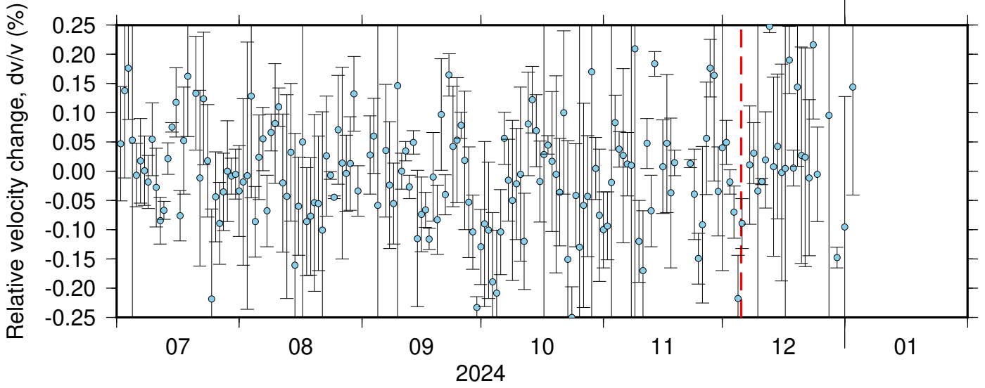
BK_HAYF_PB_B934 ZRT 0.10-0.90Hz 011
