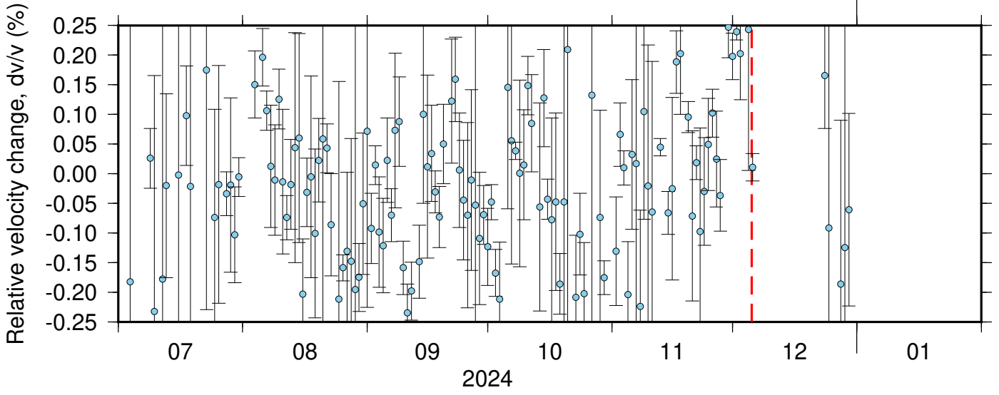
NC_KCR_PB_B047 ZRT 0.10-0.90Hz 011
