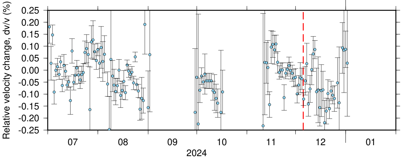
BK_PRDS_PB_B046 ZRT 0.10-0.90Hz 011
