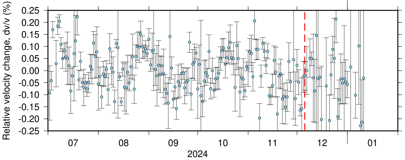
BK_BJES_BK_PRDS ZRT 0.10-0.90Hz 011
