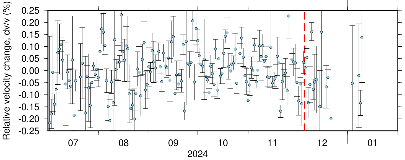
BK_BJES_NC_KCT ZRT 0.10-0.90Hz 011
