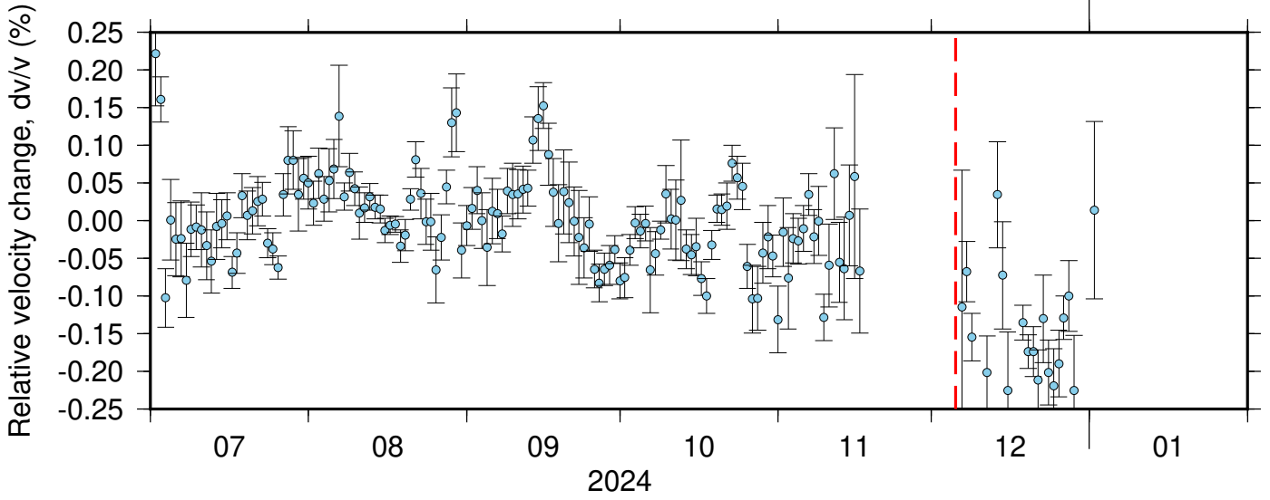
BK_SPRL_PB_B049 ZRT 0.10-0.90Hz 011
