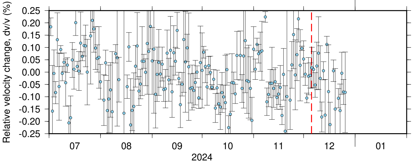
BK_KNEE_PB_B047 ZRT 0.10-0.90Hz 011
