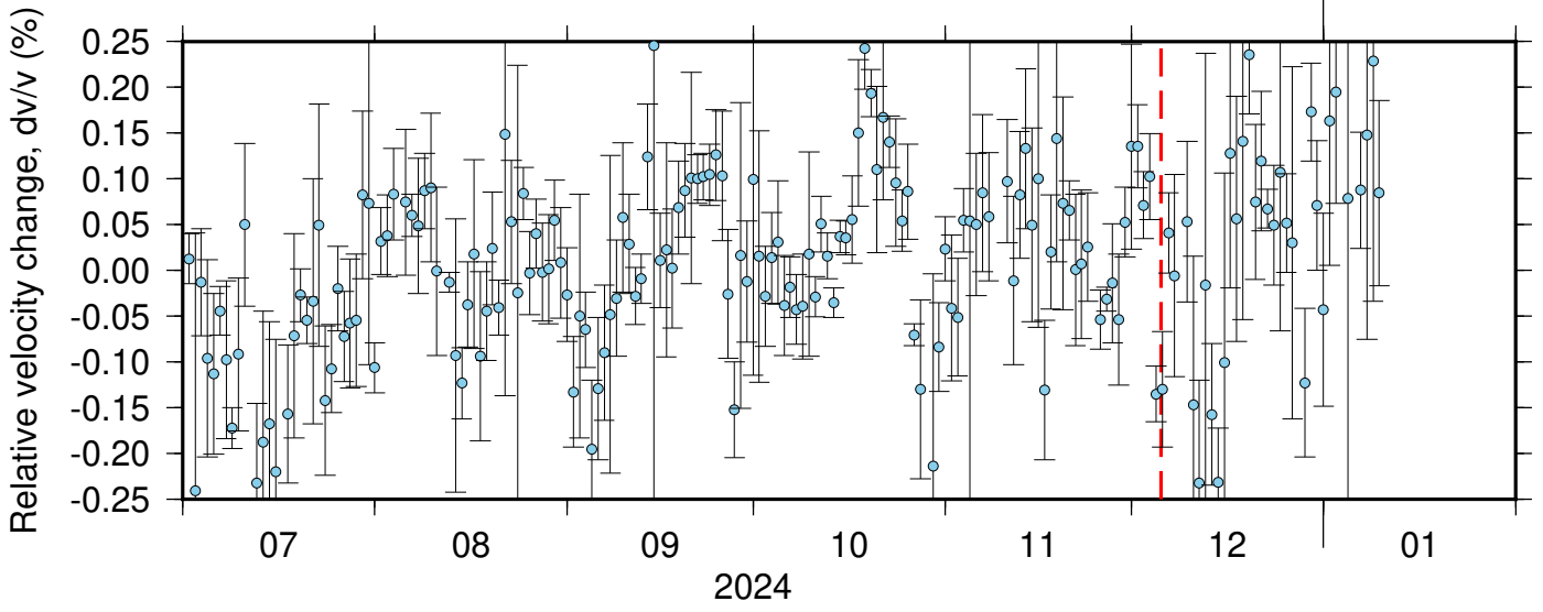
BK_HAYF_BK_KNEE ZRT 0.10-0.90Hz 011
