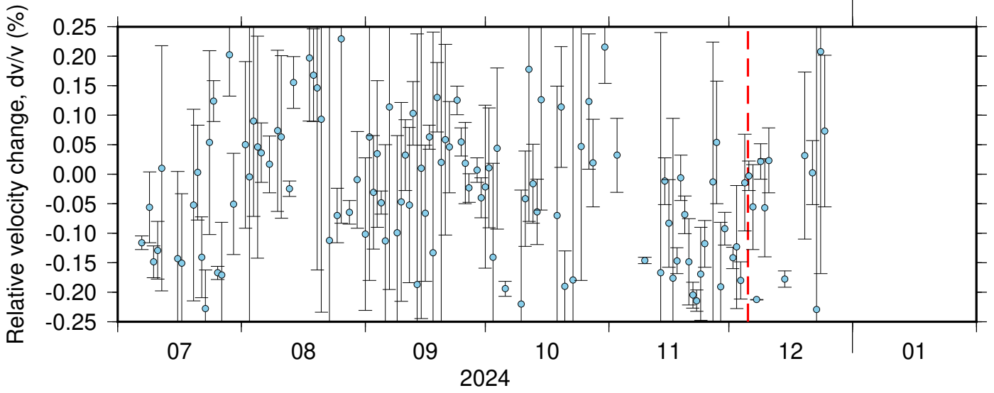
BK_KNEE_NC_KPR ZRT 0.10-0.90Hz 011
