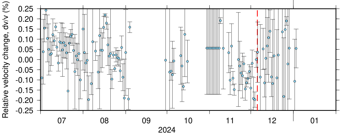
BK_JCC_PB_B046 ZRT 0.10-0.90Hz 011
