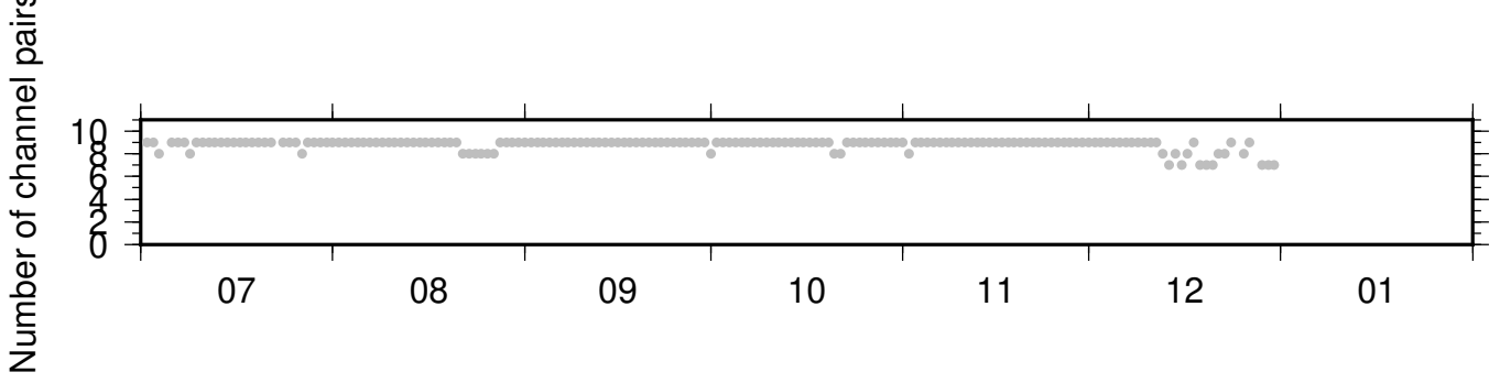
BK_HAYF_PB_B047 ZRT 0.10-0.90Hz 011
