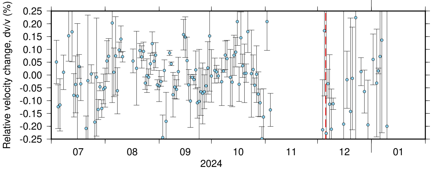
NC_KMR_NC_KSM ZRT 0.10-0.90Hz 011
