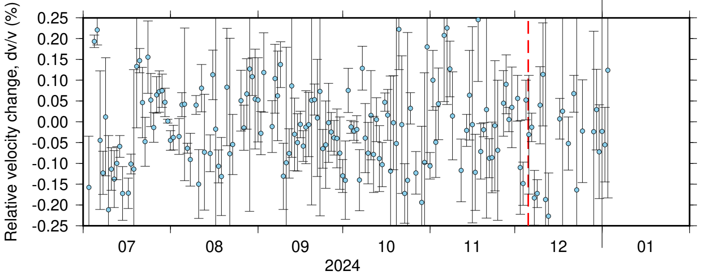
BK_WLKR_PB_B934 ZRT 0.10-0.90Hz 011
