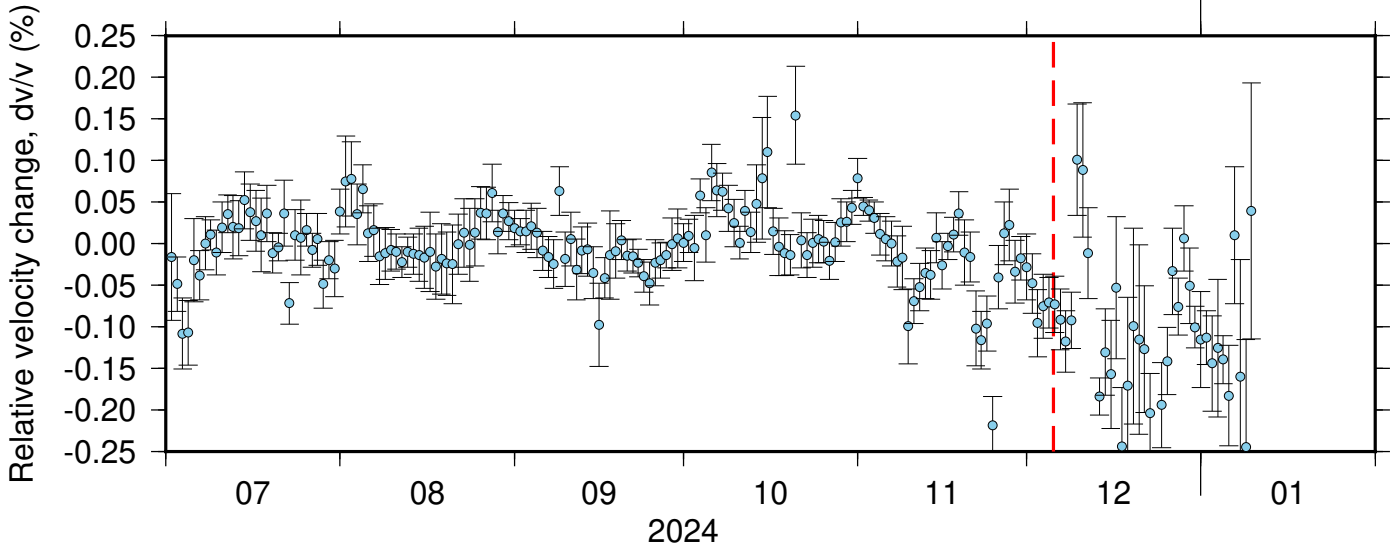
BK_BJES_NC_KMPB ZRT 0.10-0.90Hz 011
