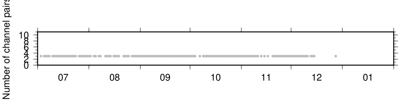
NC_KBU_NC_KCT ZRT 0.10-0.90Hz 011
