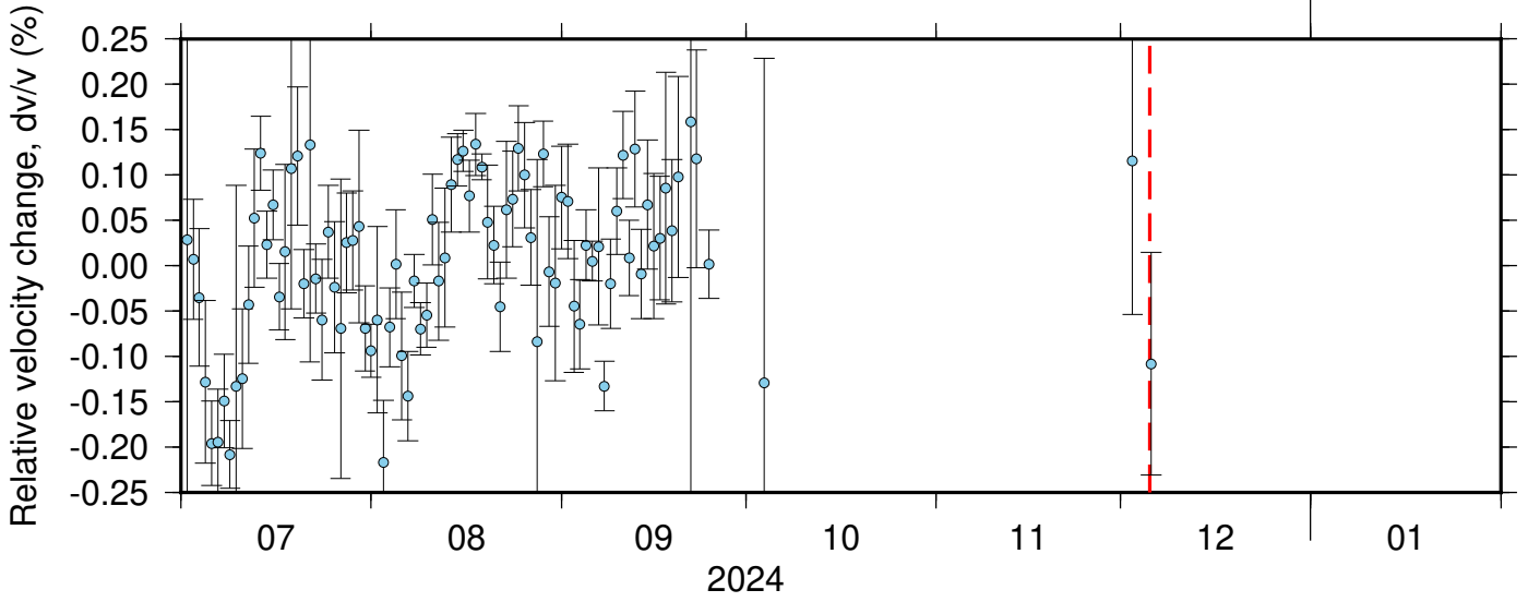
BK_BLAS_PB_B932 ZRT 0.10-0.90Hz 011
