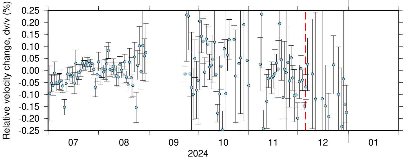
NC_KMR_PB_B045 ZRT 0.10-0.90Hz 011
