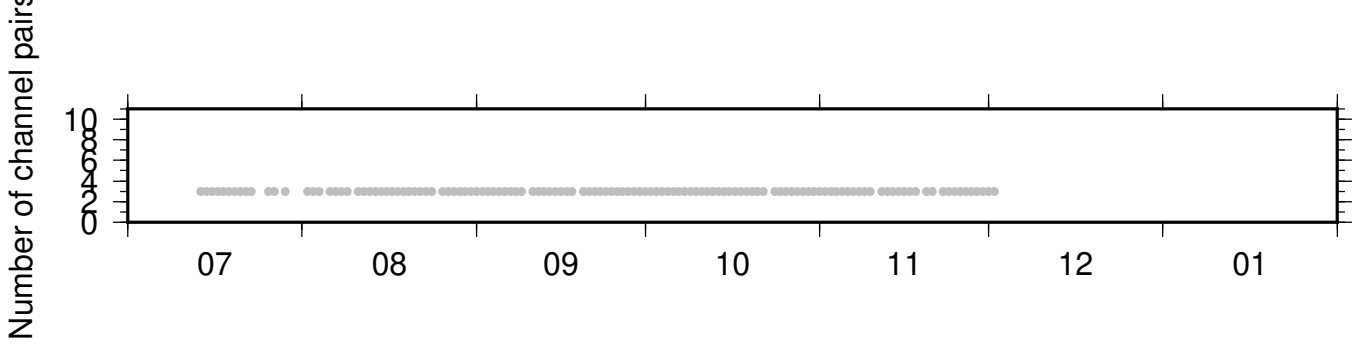
NC_KCR_NC_KCT ZRT 0.10-0.90Hz 011
