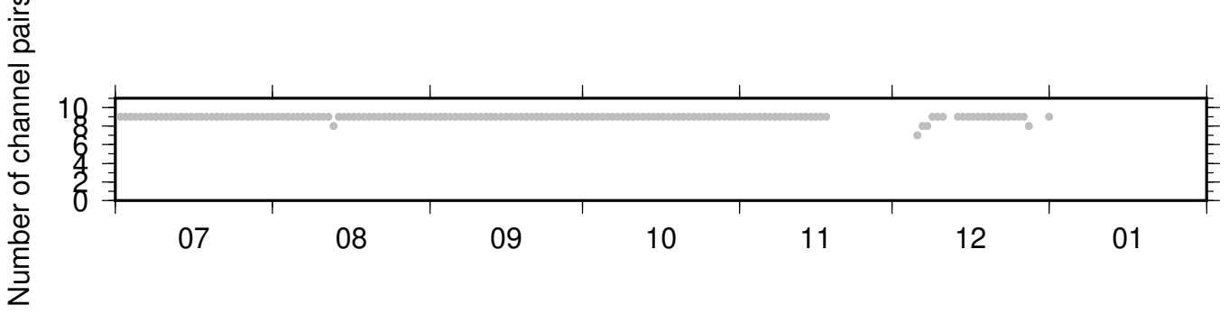
BK_PETL_PB_B049 ZRT 0.10-0.90Hz 011
