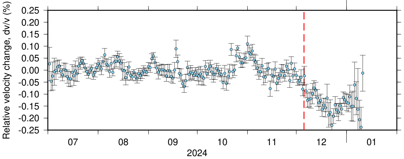
BK_BRIC_BK_GHOP ZRT 0.10-0.90Hz 011
