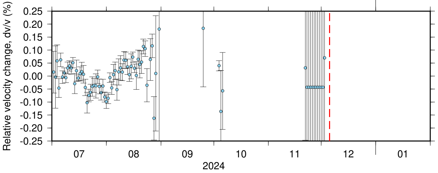
PB_B045_PB_B932 ZRT 0.10-0.90Hz 011
