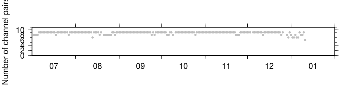
BK_BRIC_BK_JCC ZRT 0.10-0.90Hz 011
