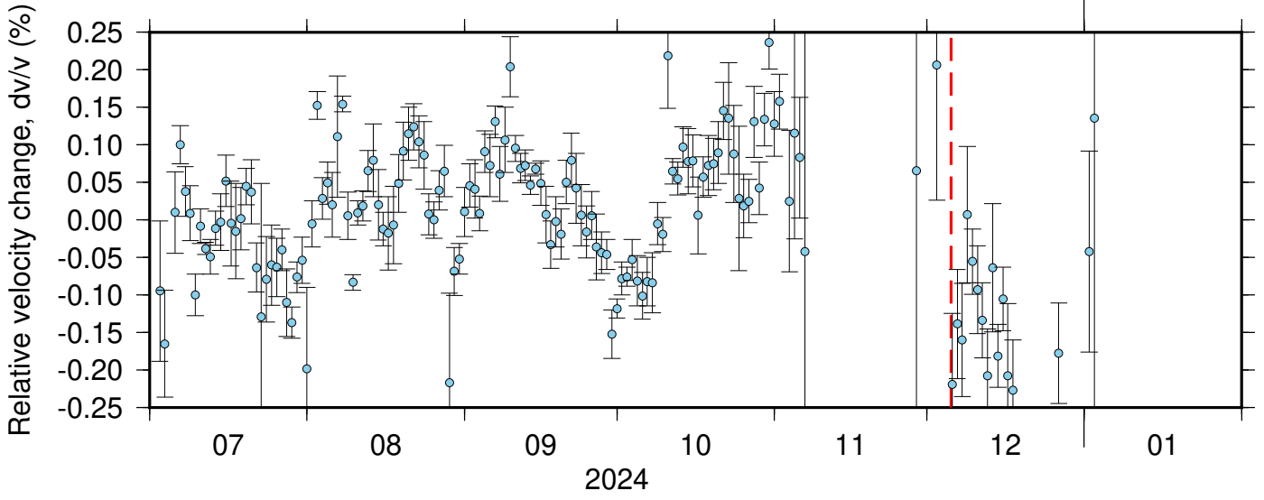
NC_KSM_PB_B047 ZRT 0.10-0.90Hz 011
