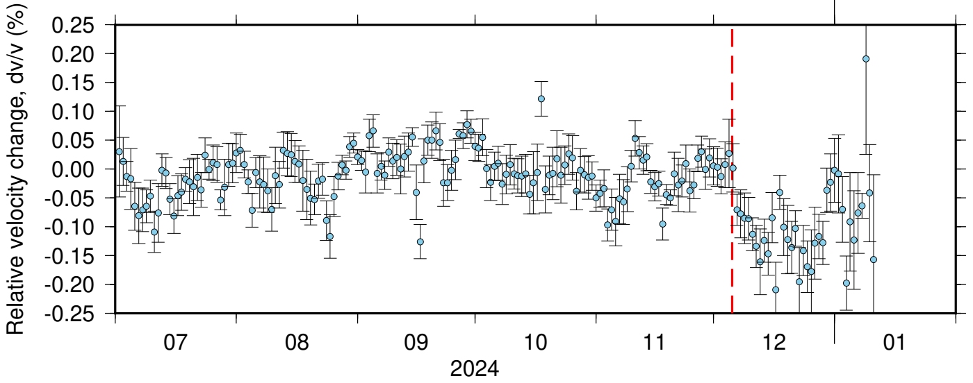
BK_JCC_BK_KNEE ZRT 0.10-0.90Hz 011
