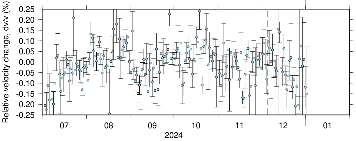
BK_BRIC_PB_B934 ZRT 0.10-0.90Hz 011
