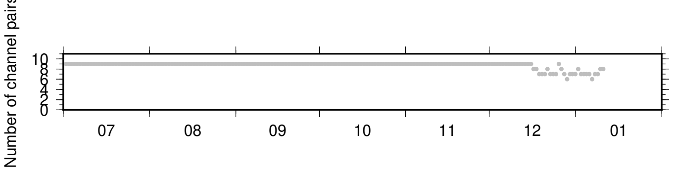
BK_WLKR_NC_KCT ZRT 0.10-0.90Hz 011
