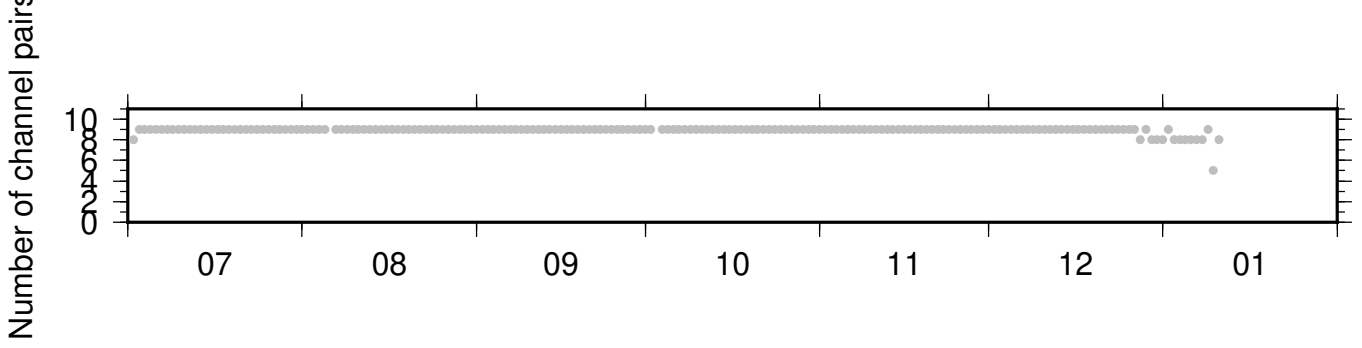
BK_KNEE_BK_WLKR ZRT 0.10-0.90Hz 011
