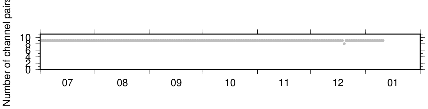
BK_PRDS_BK_WLKR ZRT 0.10-0.90Hz 011
