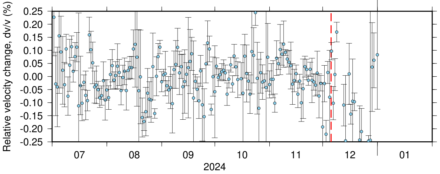
BK_BLAS_PB_B047 ZRT 0.10-0.90Hz 011
