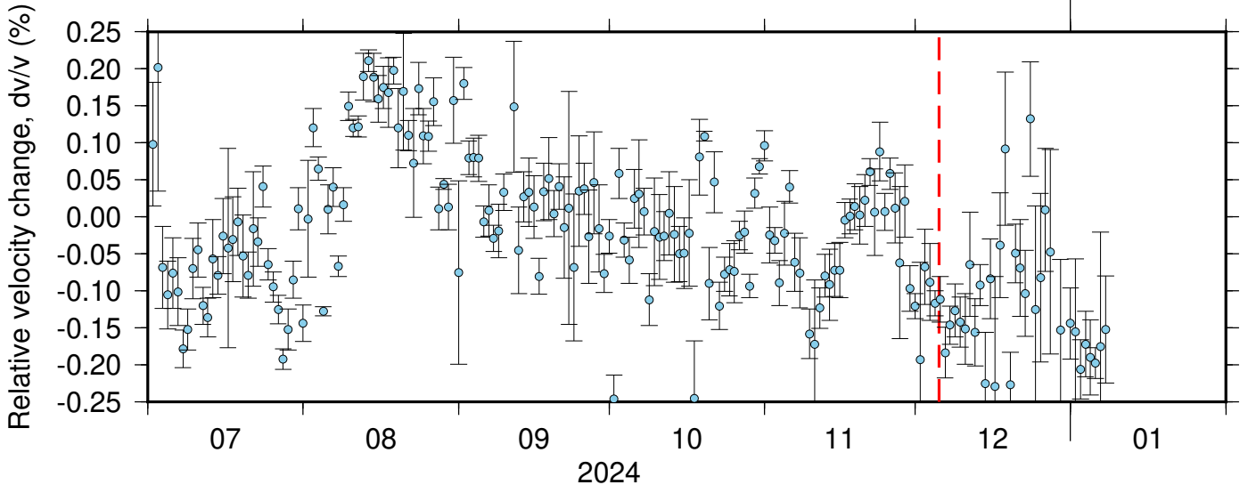
NC_KBU_NC_KMR ZRT 0.10-0.90Hz 011
