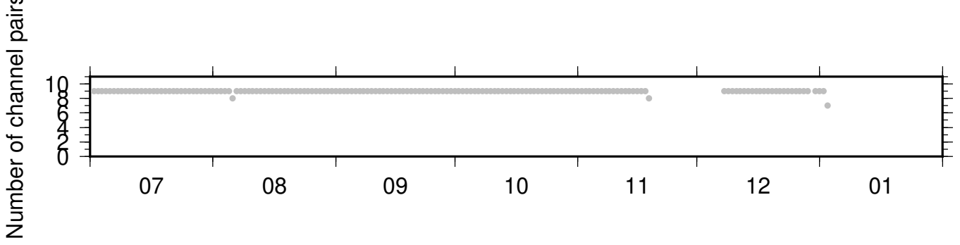
PB_B049_PB_B935 ZRT 0.10-0.90Hz 011
