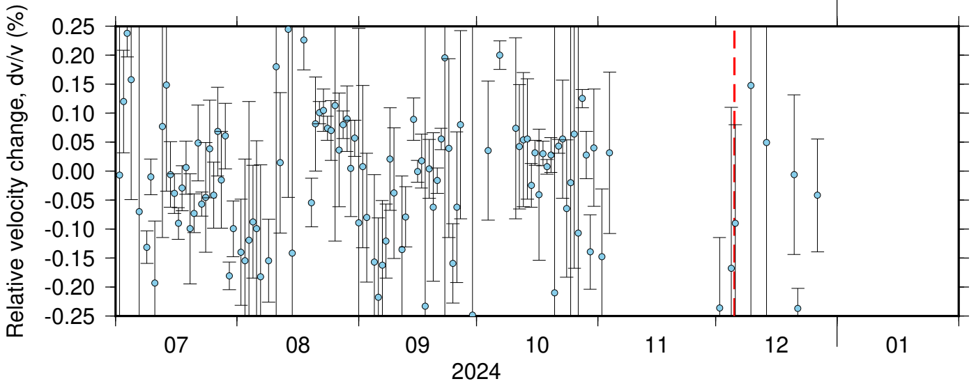
BK_BJES_NC_KSM ZRT 0.10-0.90Hz 011
