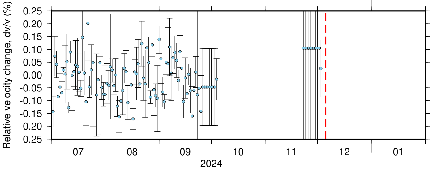
BK_JCC_PB_B932 ZRT 0.10-0.90Hz 011
