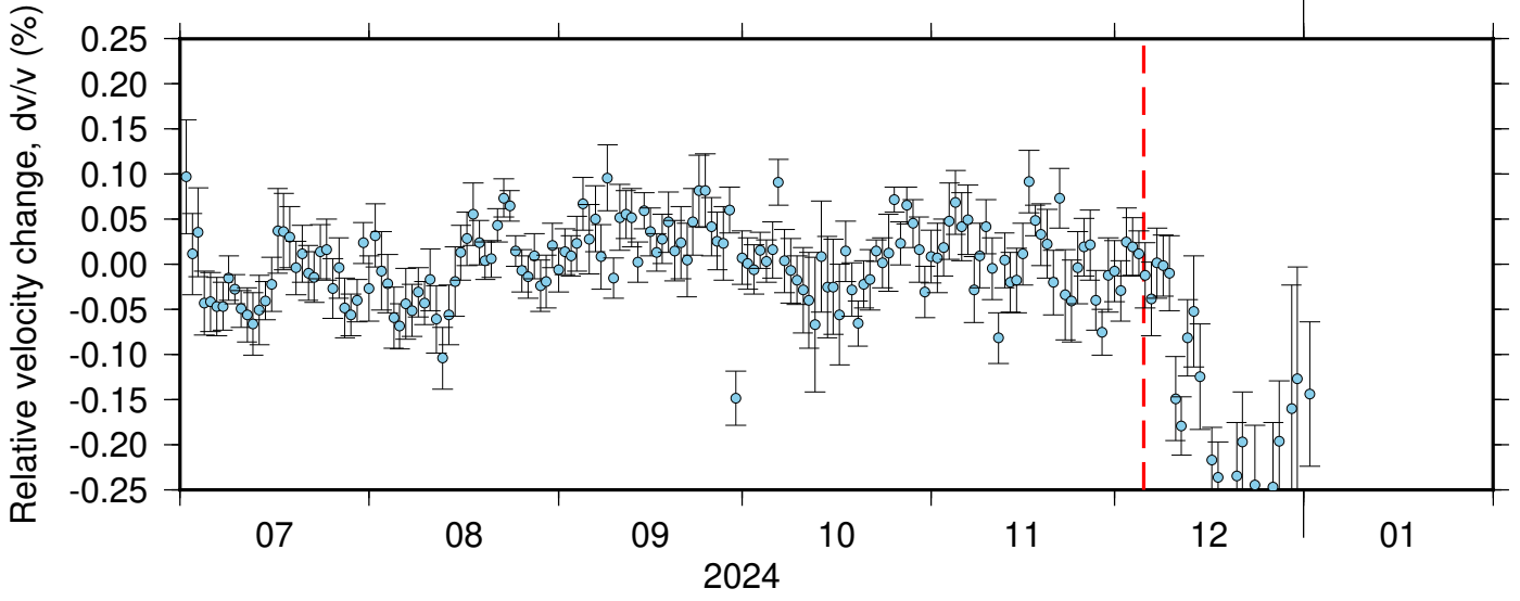
BK_WLKR_PB_B047 ZRT 0.10-0.90Hz 011
