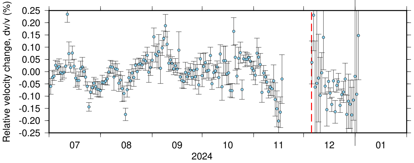
BK_BLAS_PB_B049 ZRT 0.10-0.90Hz 011
