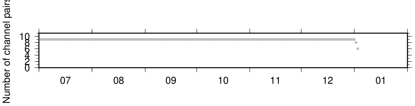
BK_BJES_PB_B935 ZRT 0.10-0.90Hz 011
