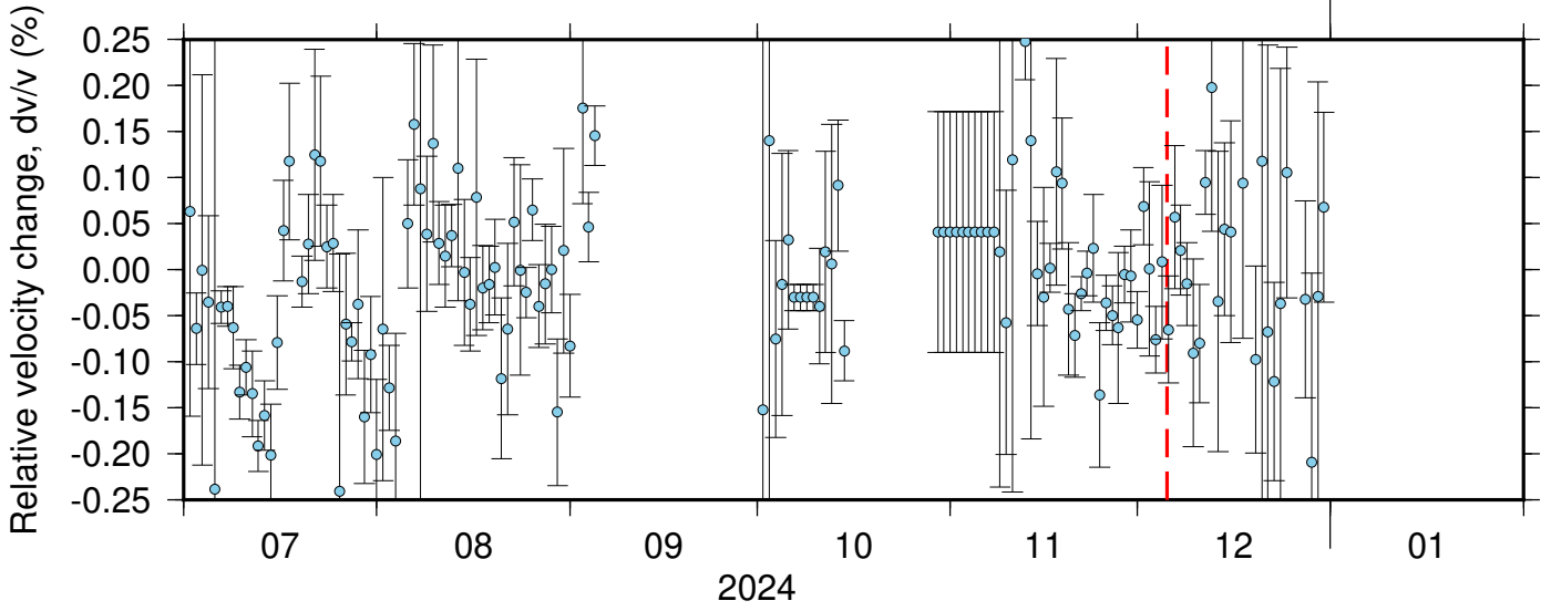
BK_BLAS_PB_B046 ZRT 0.10-0.90Hz 011
