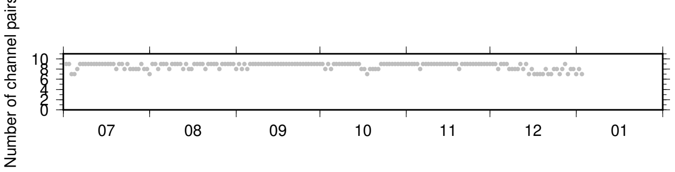
BK_PRDS_PB_B934 ZRT 0.10-0.90Hz 011
