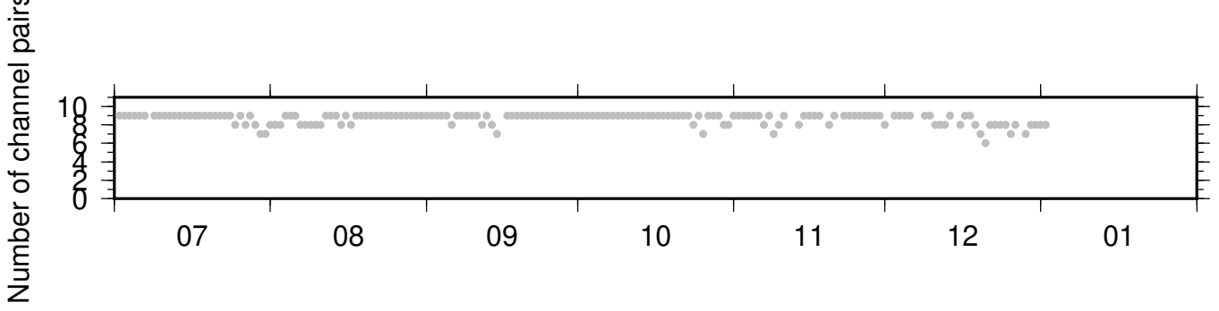
BK_KNEE_PB_B934 ZRT 0.10-0.90Hz 011
