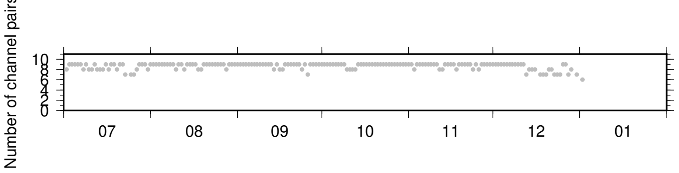
PB_B047_PB_B934 ZRT 0.10-0.90Hz 011
