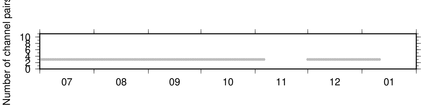
NC_KMPB_NC_KSM ZRT 0.10-0.90Hz 011
