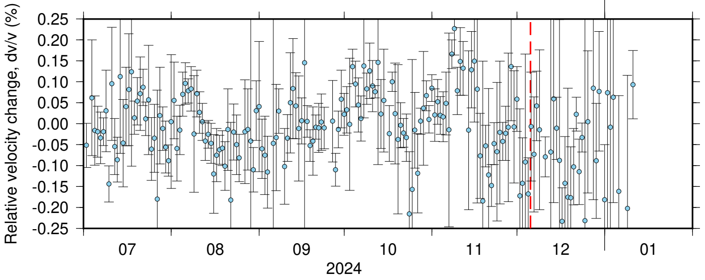
BK_KNEE_BK_RBOW ZRT 0.10-0.90Hz 011
