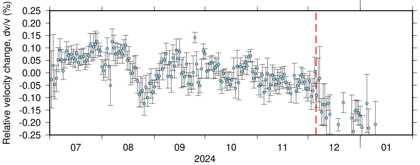
BK_WLKR_NC_KMPB ZRT 0.10-0.90Hz 011
