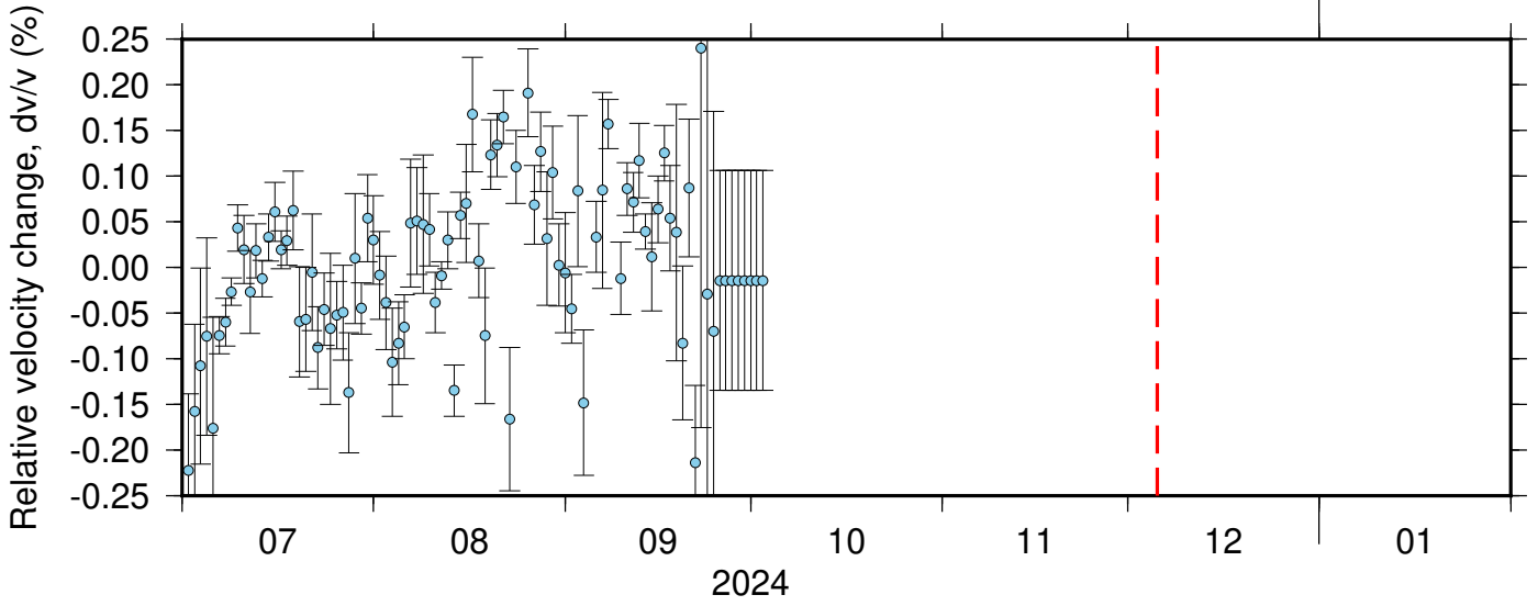
BK_BJES_PB_B932 ZRT 0.10-0.90Hz 011
