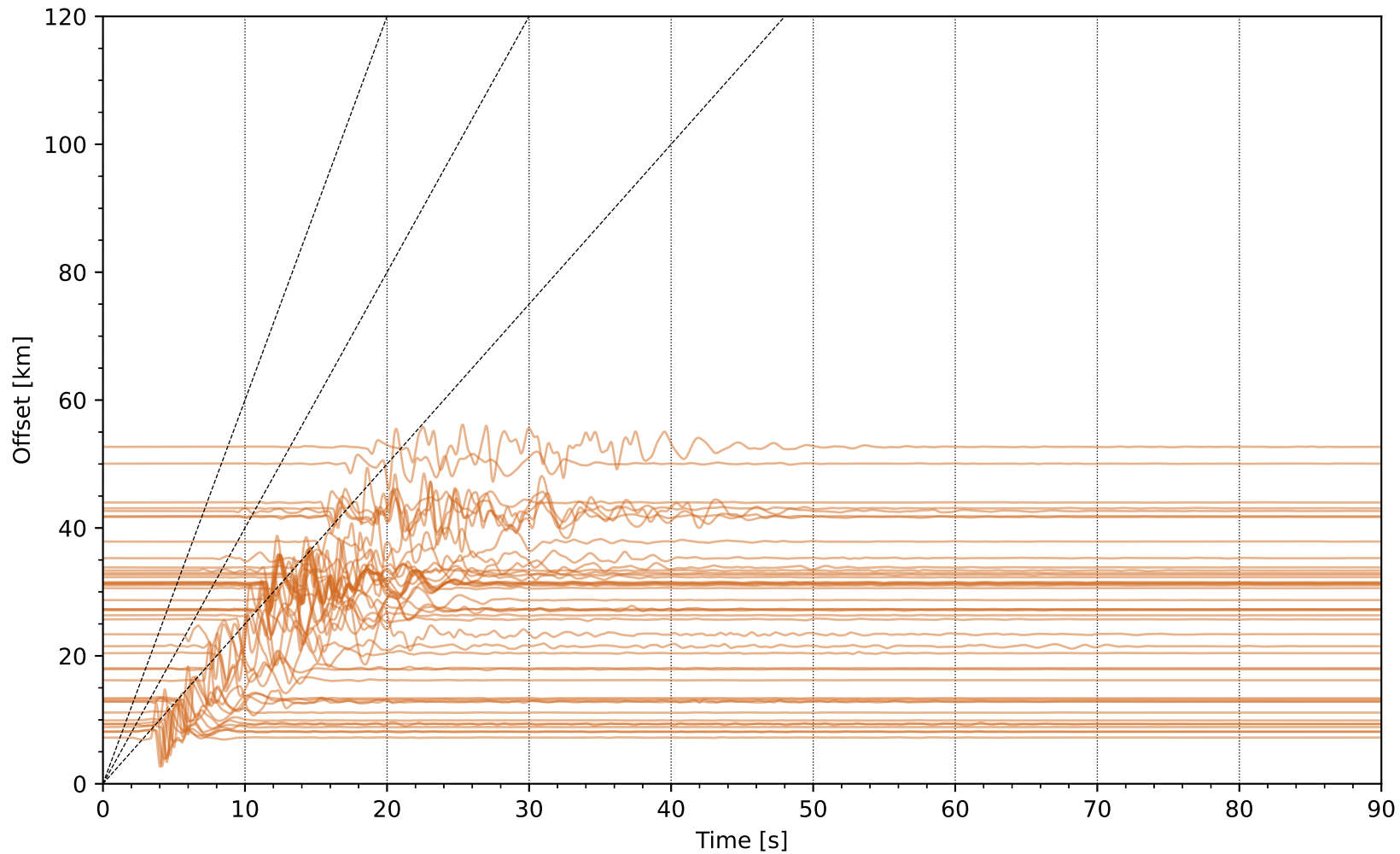
EventD uwsm1 Network: NP [HST] - (44 traces / 2007-07-20T11:42:22.5)
