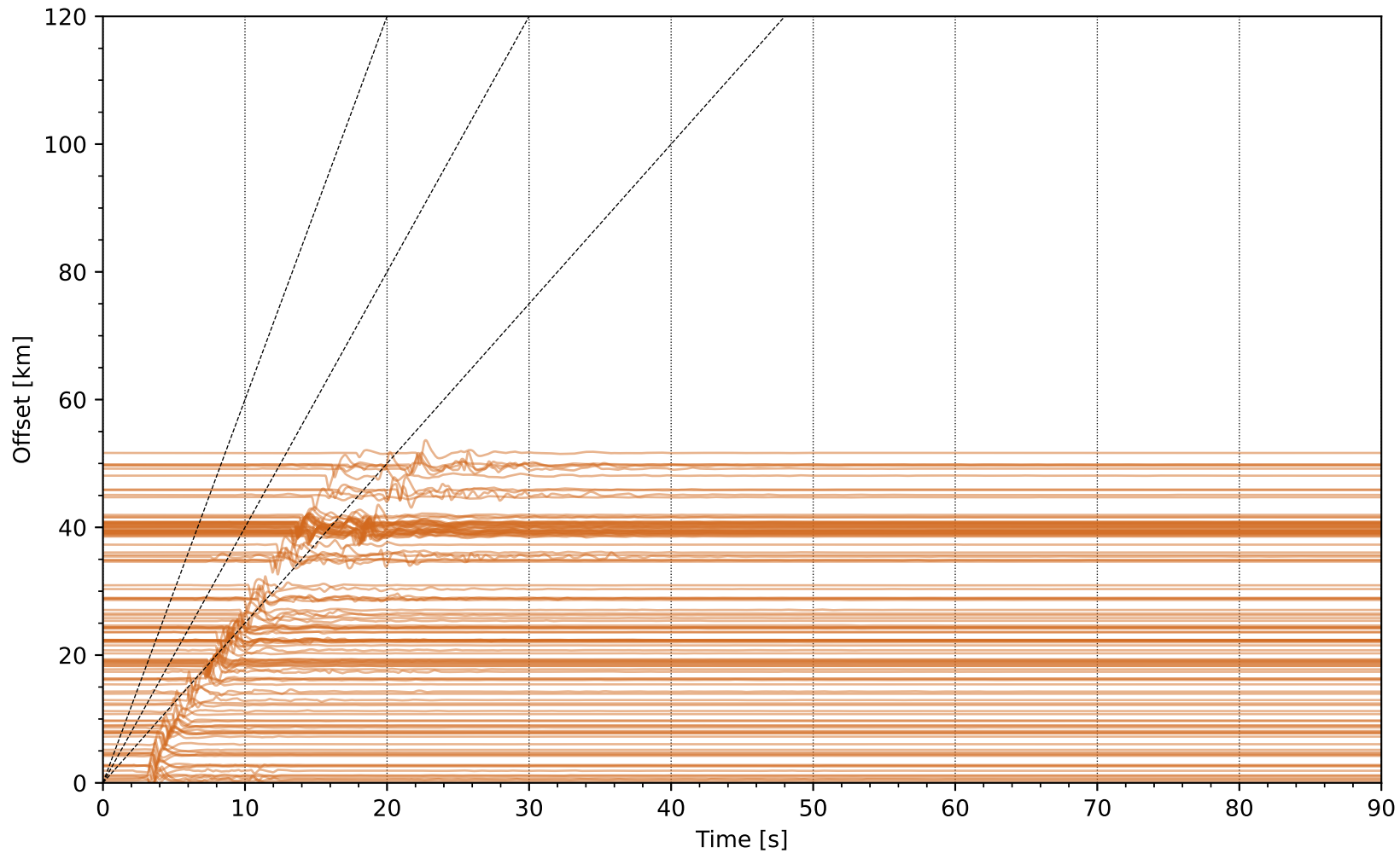
Event] uwsml Network: NP [HST] - (120 traces / 2011-10-27T12:36:44.48)
