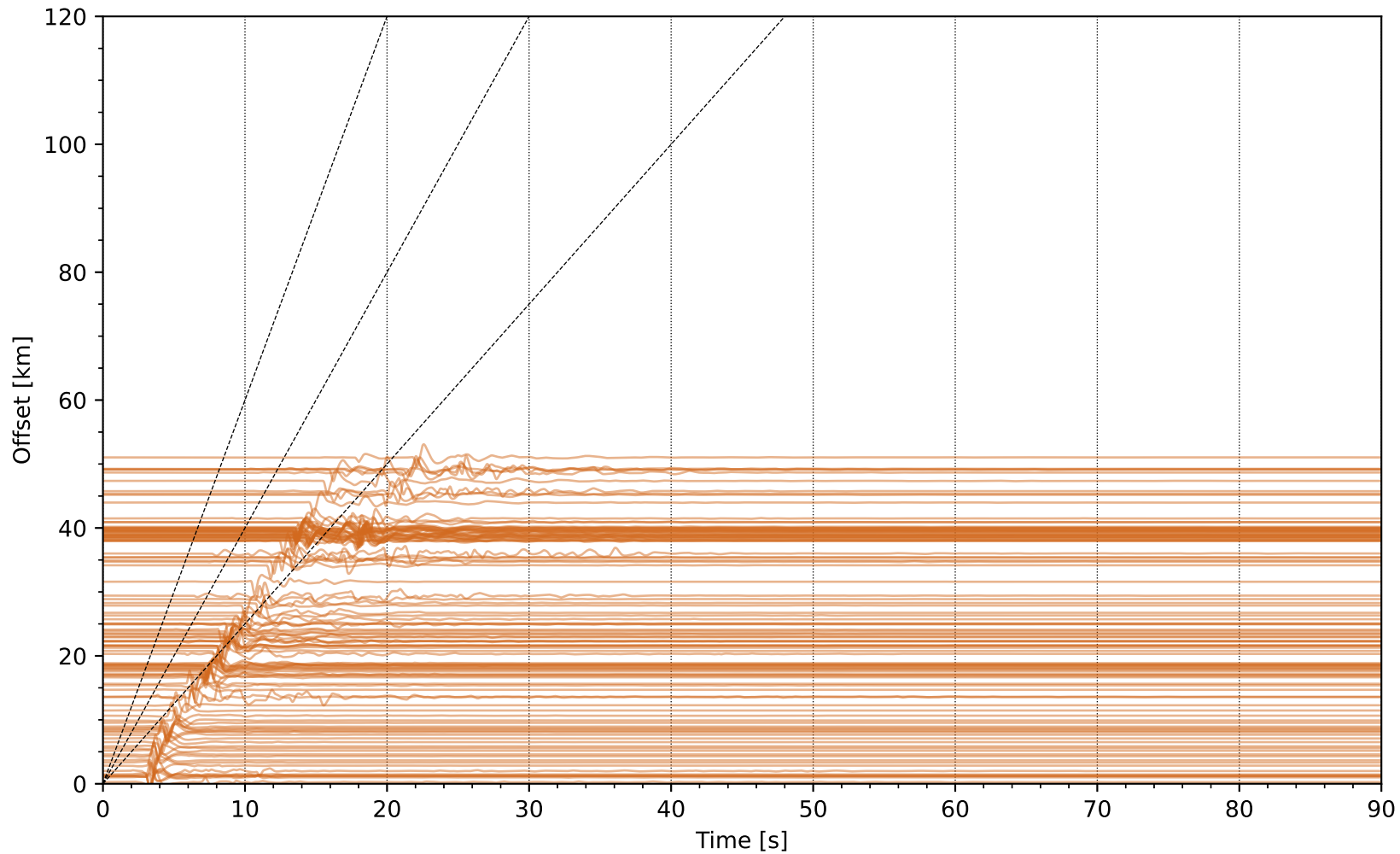
Event1 uwsm1 Network: NP [HST] - (117 traces / 2011-10-21T03:16:05.31)
