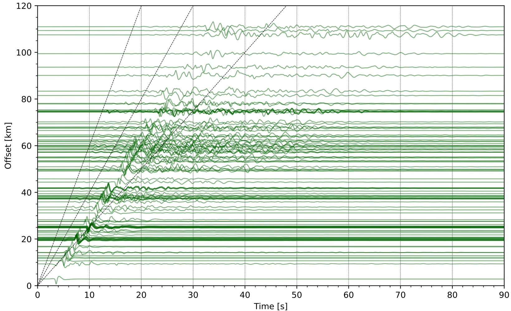
EventF th09sm1 Network: NP [HST] - (112 traces / 2010-01-07T18:09:35.28)
