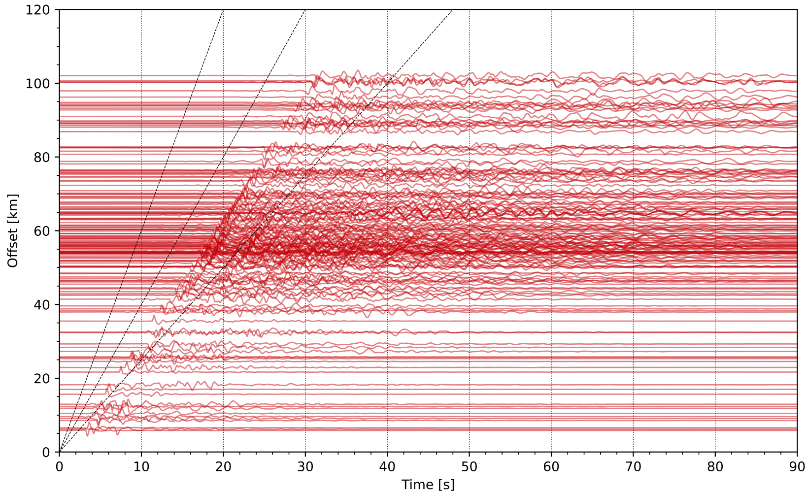
EventR usgs_v21_1 Network: WR [HST] - (158 traces / 2019-02-17T09:55:24.22)
