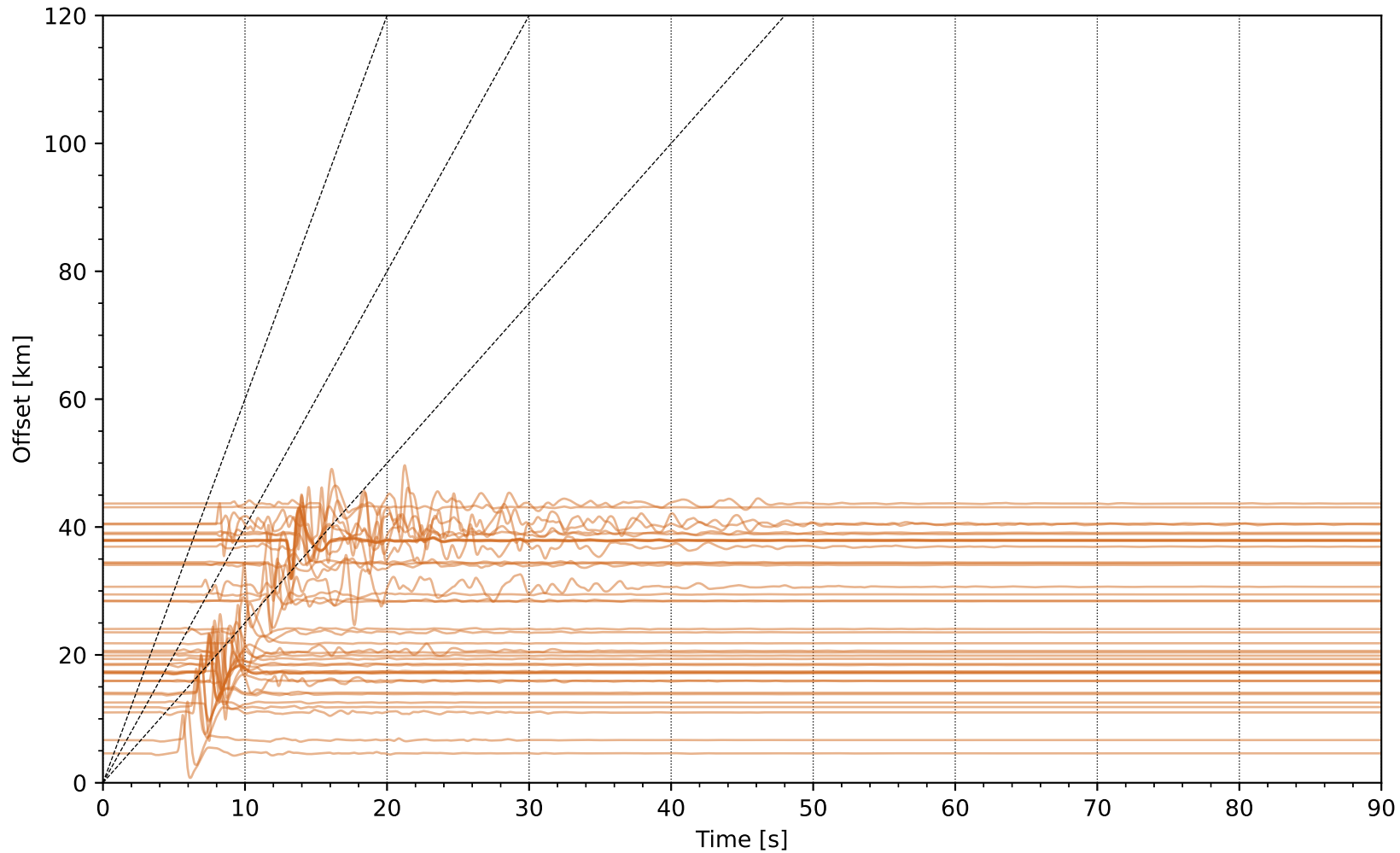
EventC uwsm1 Network: NP [HST] - (40 traces / 2007-03-02T04:40:01.08)
