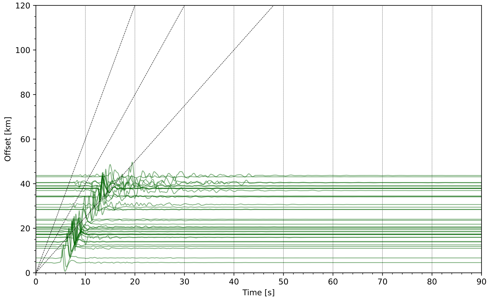
EventC th09sm1 Network: NP [HST] - (40 traces / 2007-03-02T04:40:01.08)
