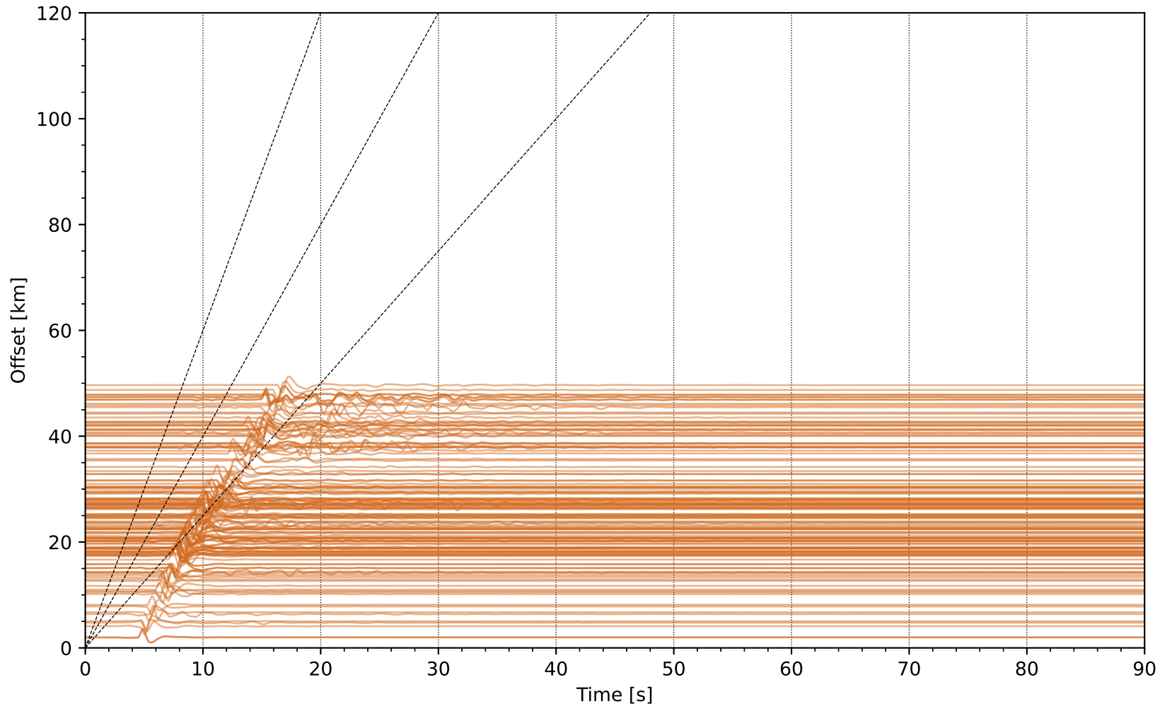
EventT uwsm1 Network: NP [HST] - (148 traces / 2019-10-15T05:33:42.12)
