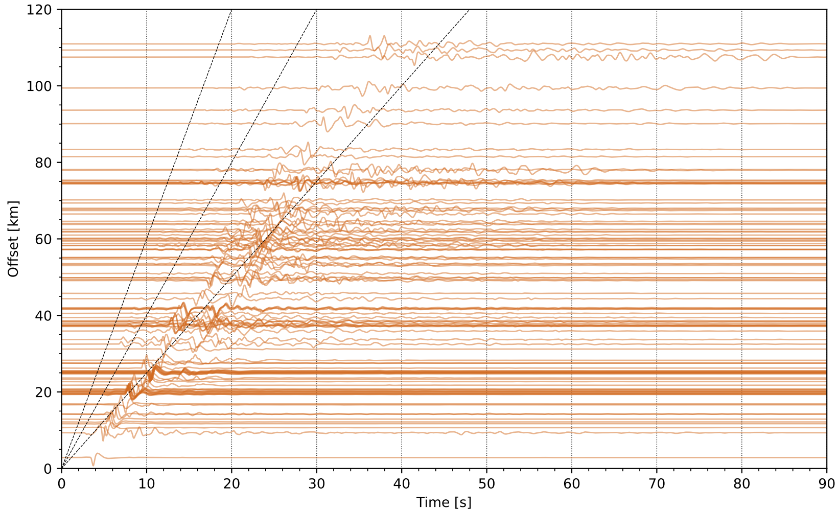
EventF uwsm1 Network: NP [HST] - (112 traces / 2010-01-07T18:09:35.28)
