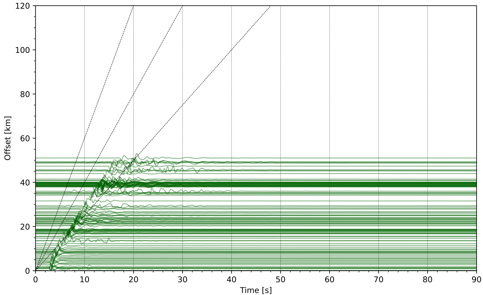
Event th09sm1 Network: NP [HST] - (117 traces / 2011-10-21T03:16:05.31)
