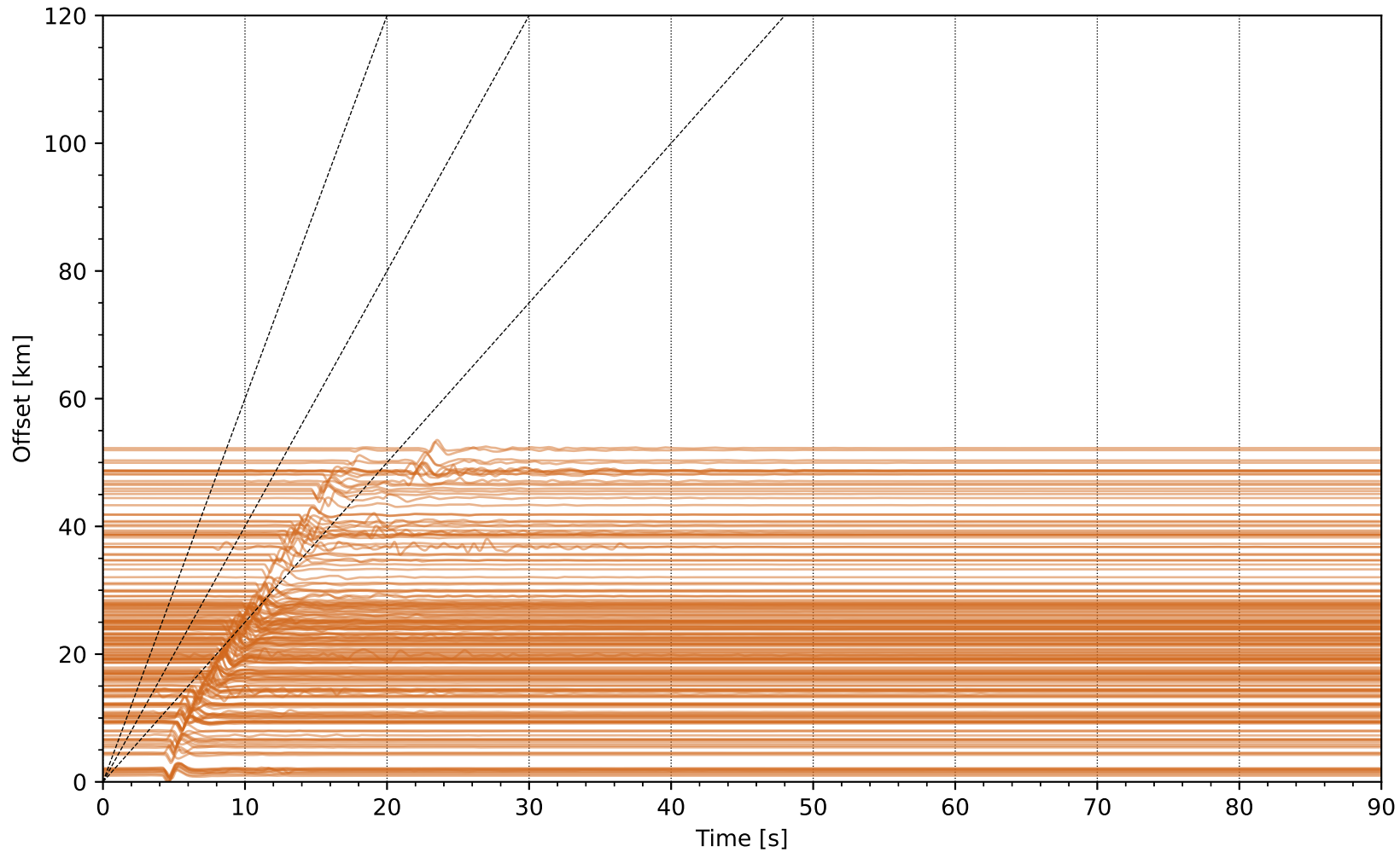
EventQ uwsm1 Network: NP [HST] - (189 traces / 2018-01-04T10:39:37.69)
