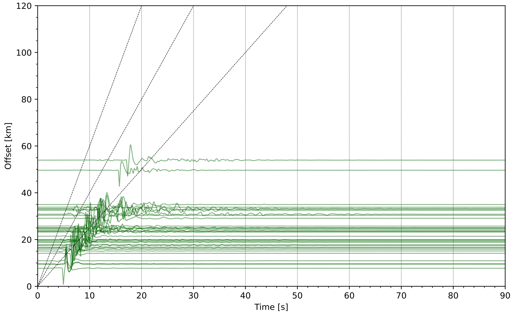
EventA th09sm1 Network: NP [HST] - (35 traces / 2006-03-21T21:41:42.43)
