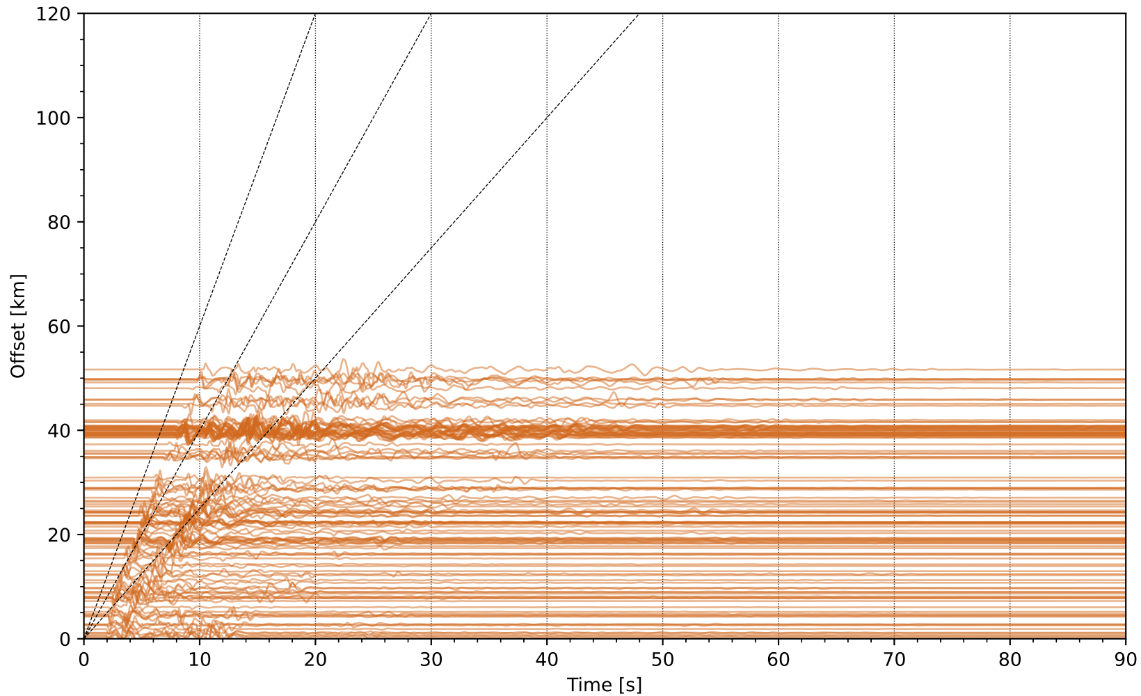
Event] uwsm1 Network: NP [HSZ] - (120 traces / 2011-10-27T12:36:44.48)
