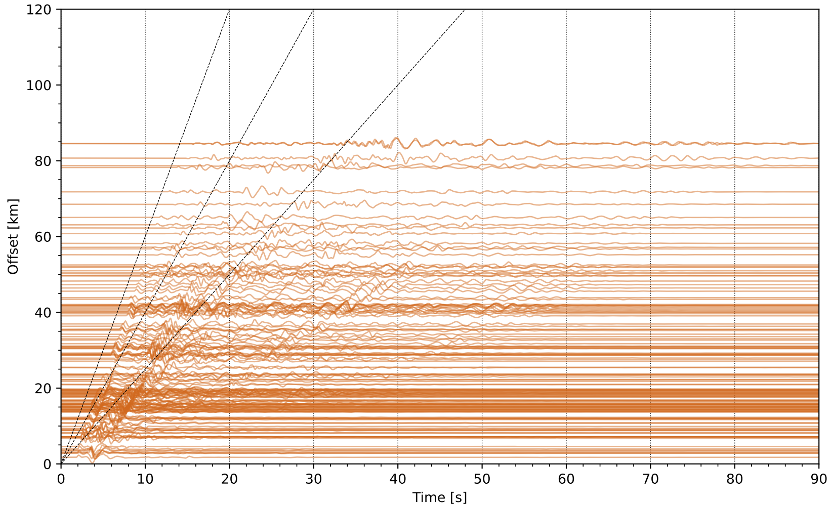
EventN uwsm1 Network: NP [HSZ] - (158 traces / 2015-07-21T09:41:14.46)
