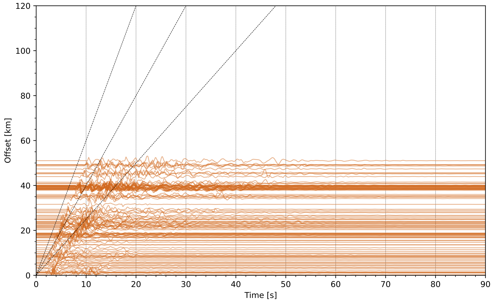
Eventl uwsm1 Network: NP [HSZ] - (117 traces / 2011-10-21T03:16:05.31)
