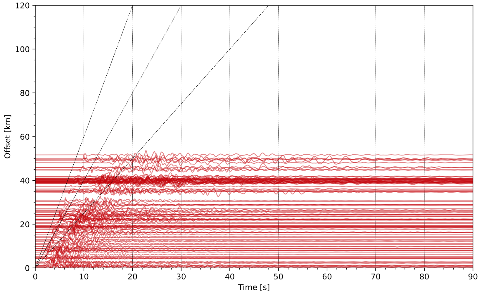
Event| usgs_v21_1 Network: NP [HSZ] - (120 traces / 2011-10-27T12:36:44.48)
