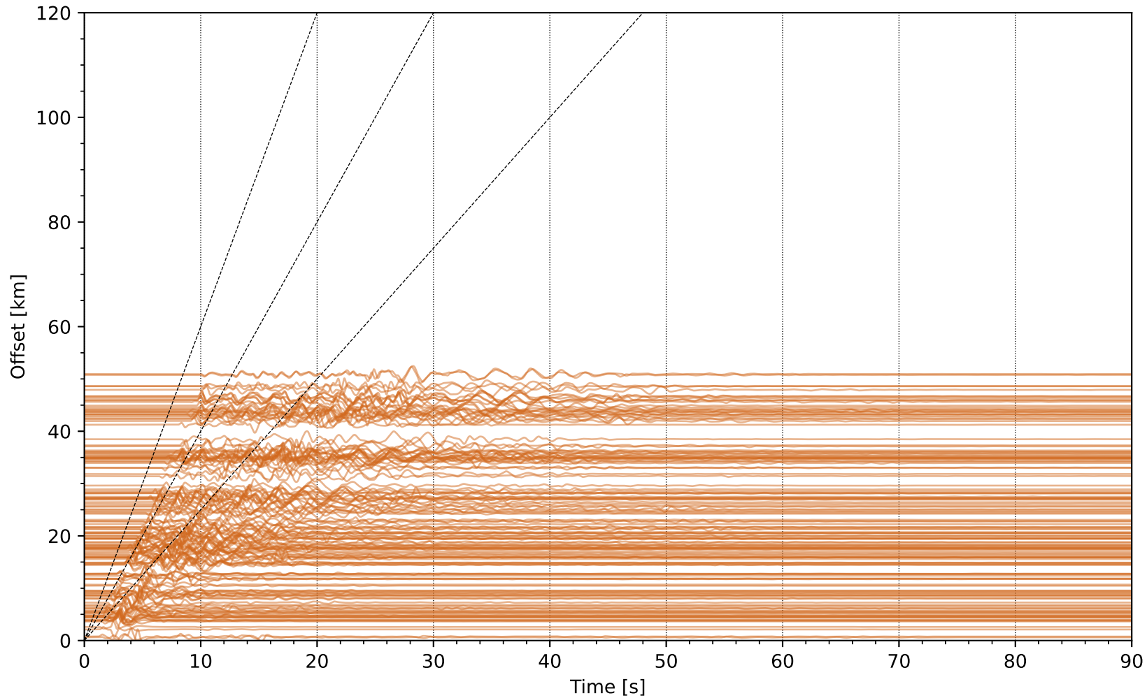
EventO uwsm1 Network: NP [HSZ] - (156 traces / 2015-08-17T13:49:17.32)
