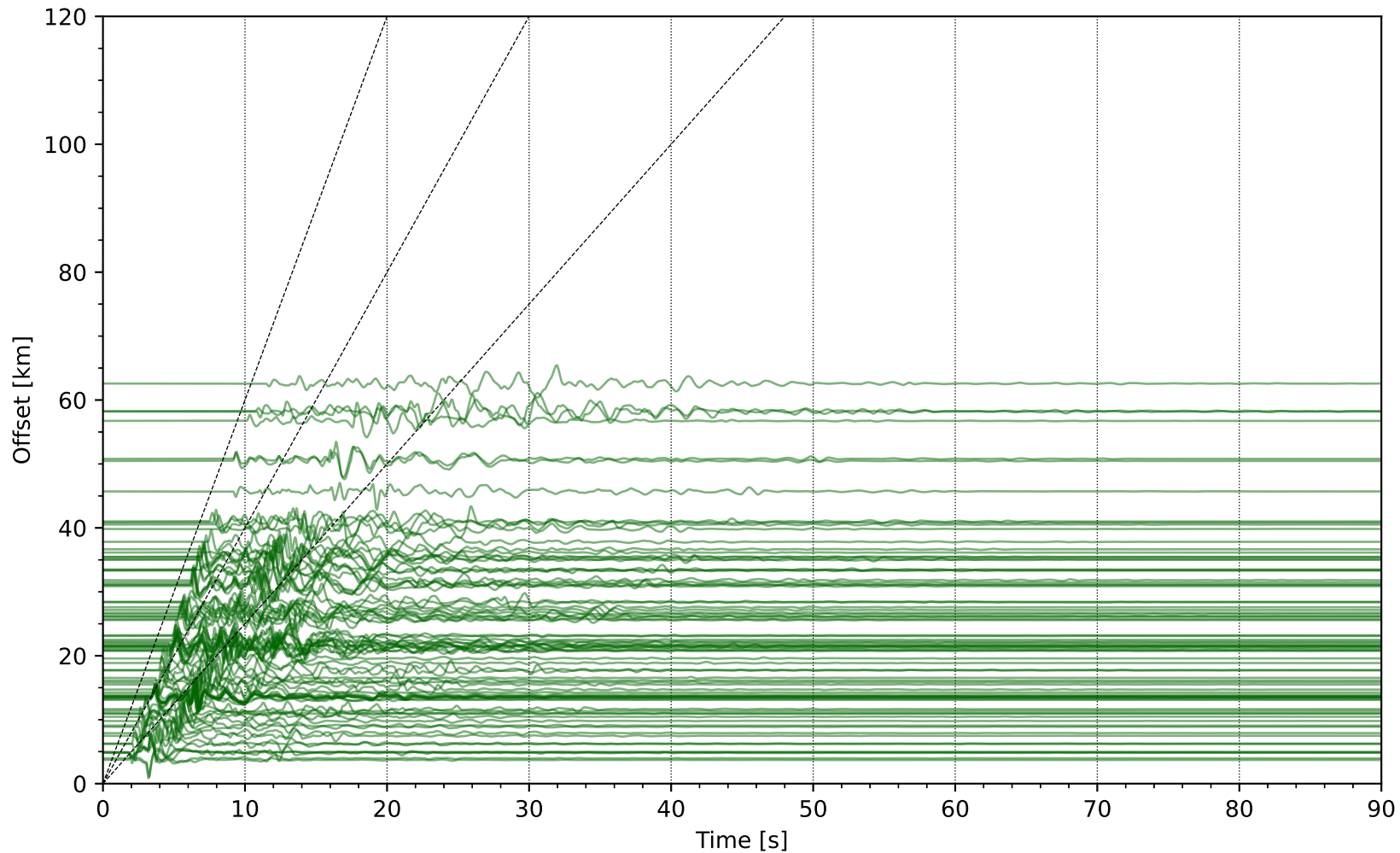
EventP th09sm1 Network: NP [HSZ] - (84 traces / 2015-10-19T23:21:17.88)
