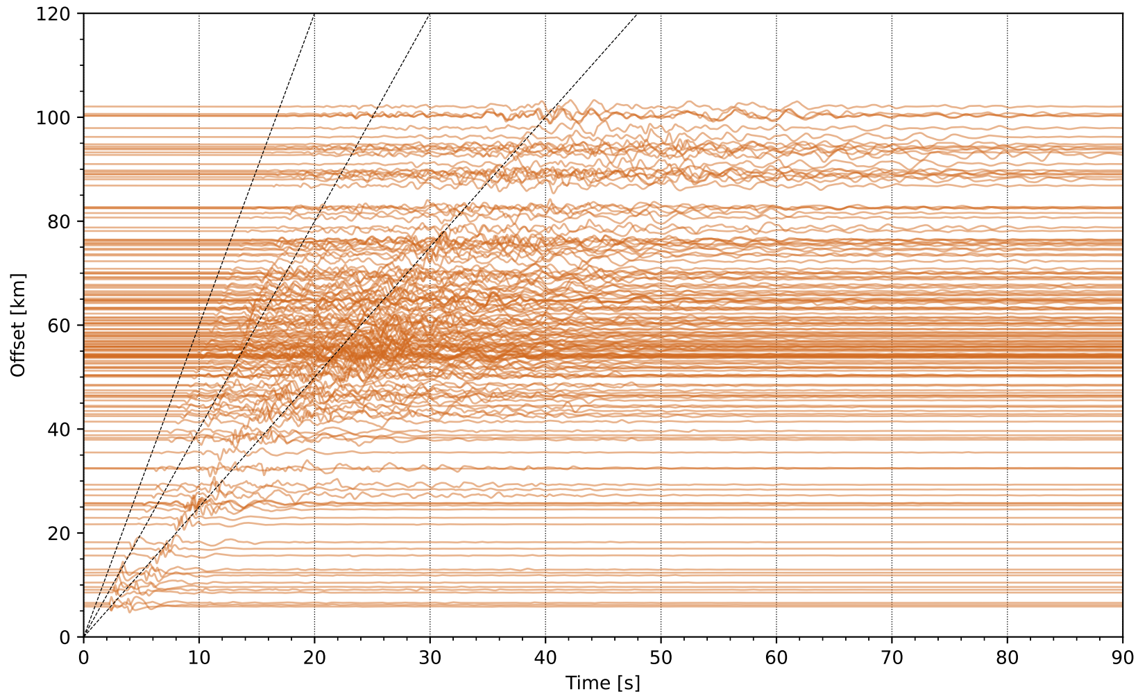
EventR uwsm1 Network: WR [HSZ] - (158 traces / 2019-02-17T09:55:24.22)
