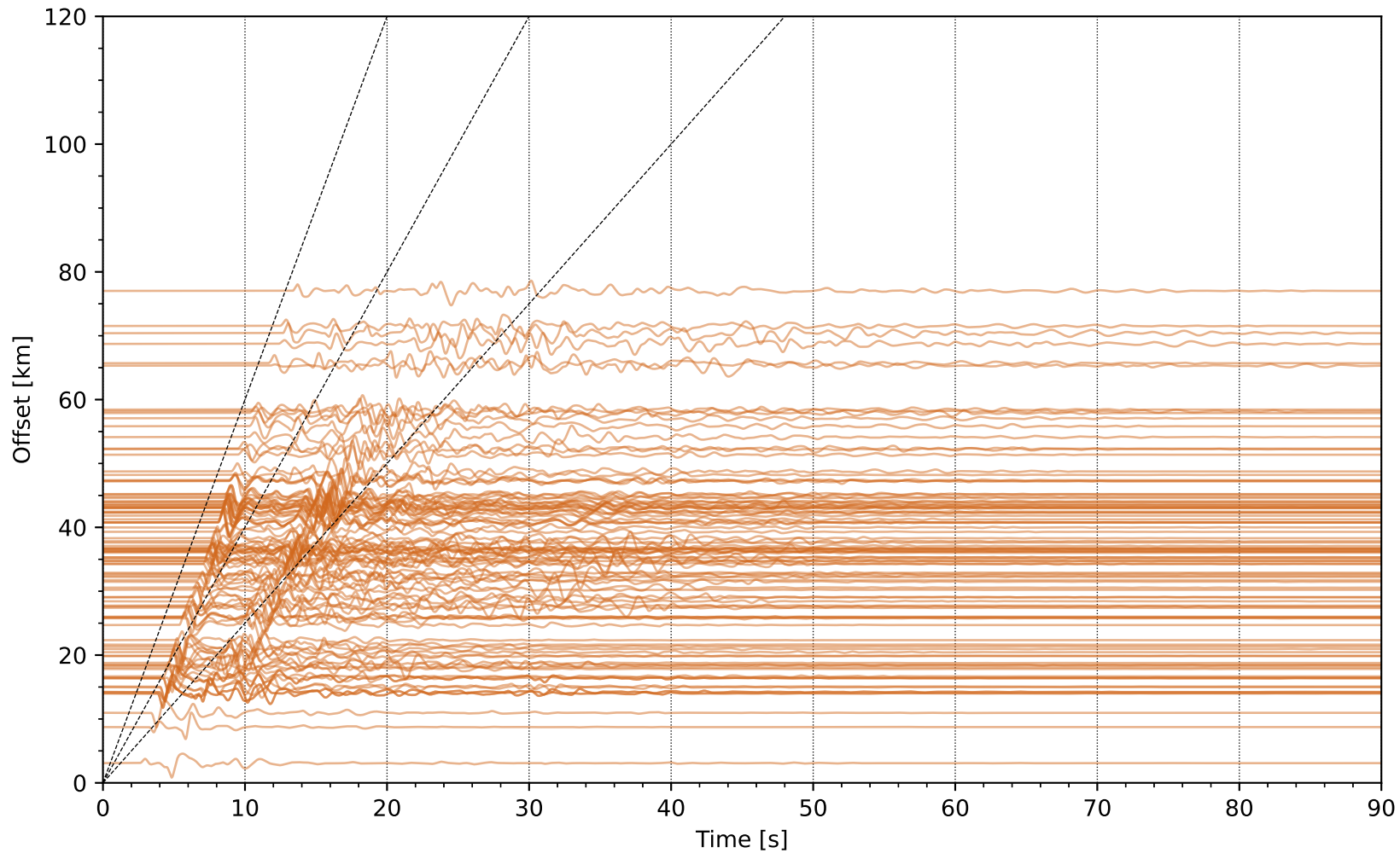
EventS uwsm1 Network: NP [HSZ] - (106 traces / 2019-07-16T20:11:01.73)
