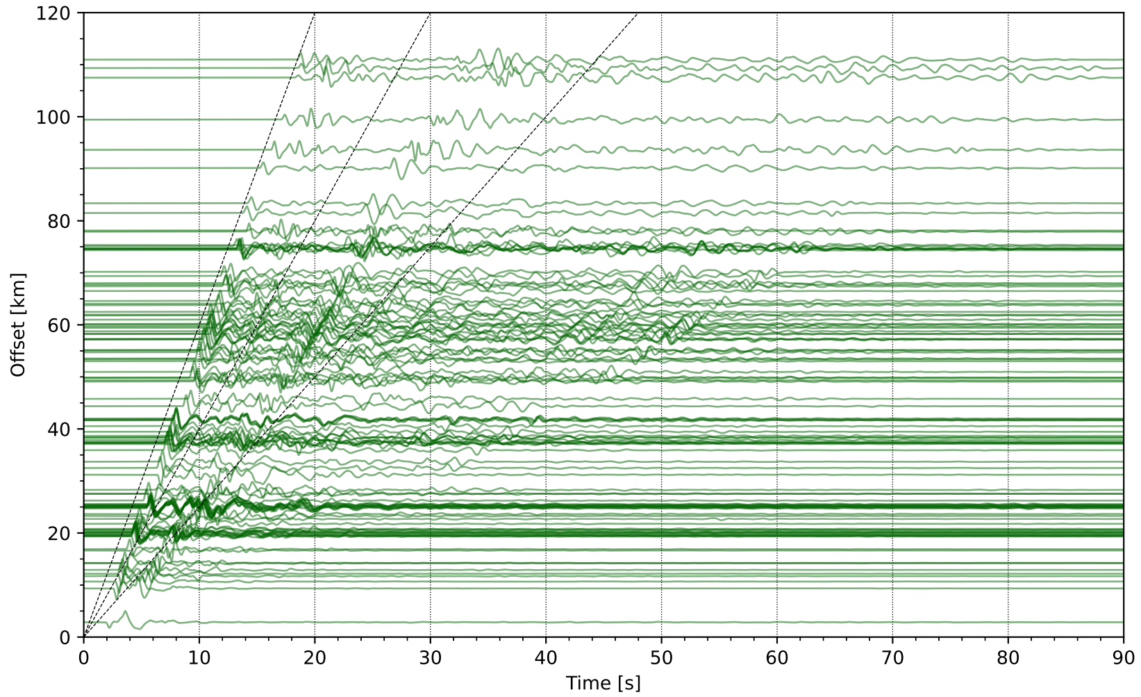
EventF th09sm1 Network: NP [HSZ] - (112 traces / 2010-01-07T18:09:35.28)
