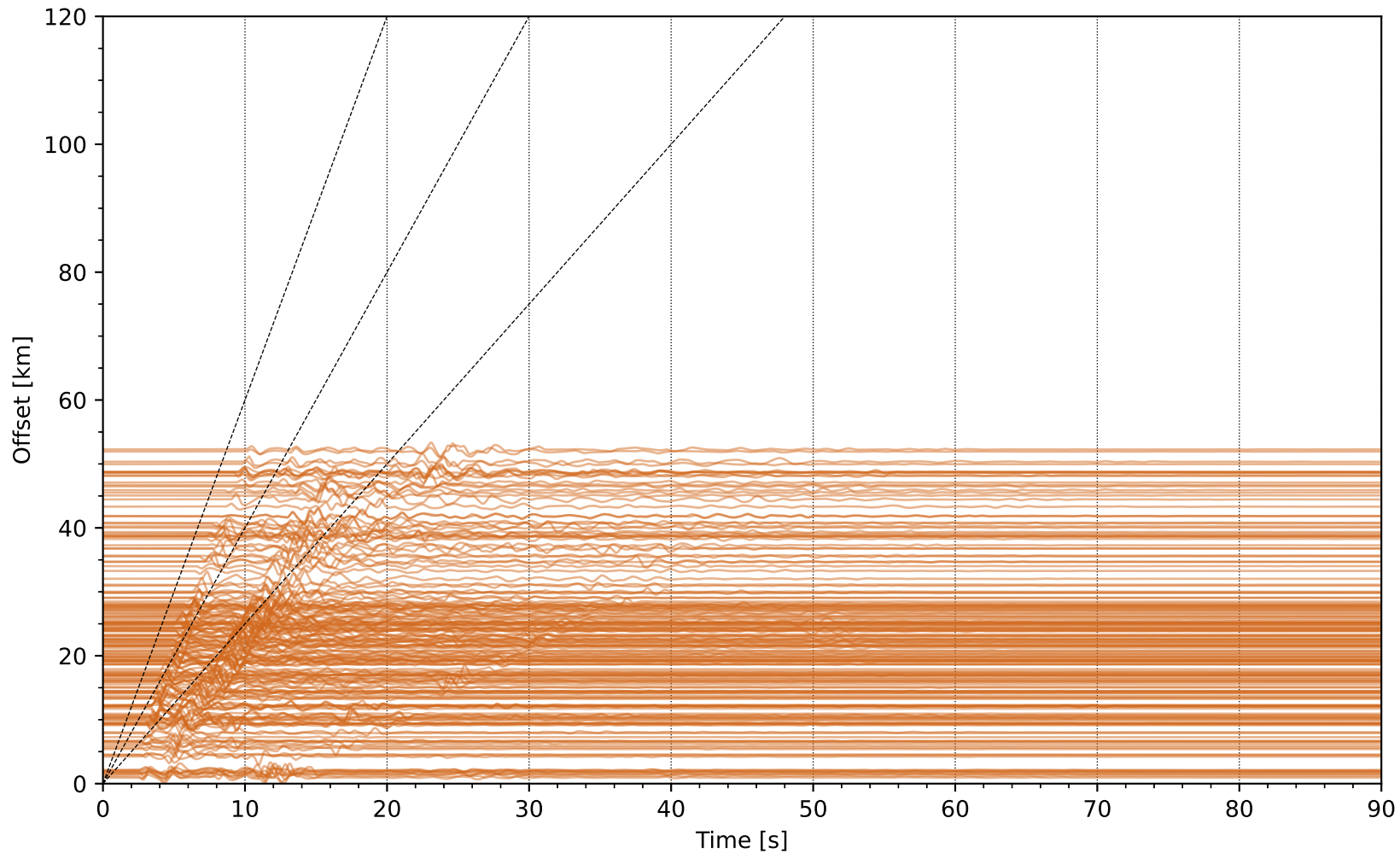
EventQ uwsm1 Network: NP [HSZ] - (189 traces / 2018-01-04T10:39:37.69)
