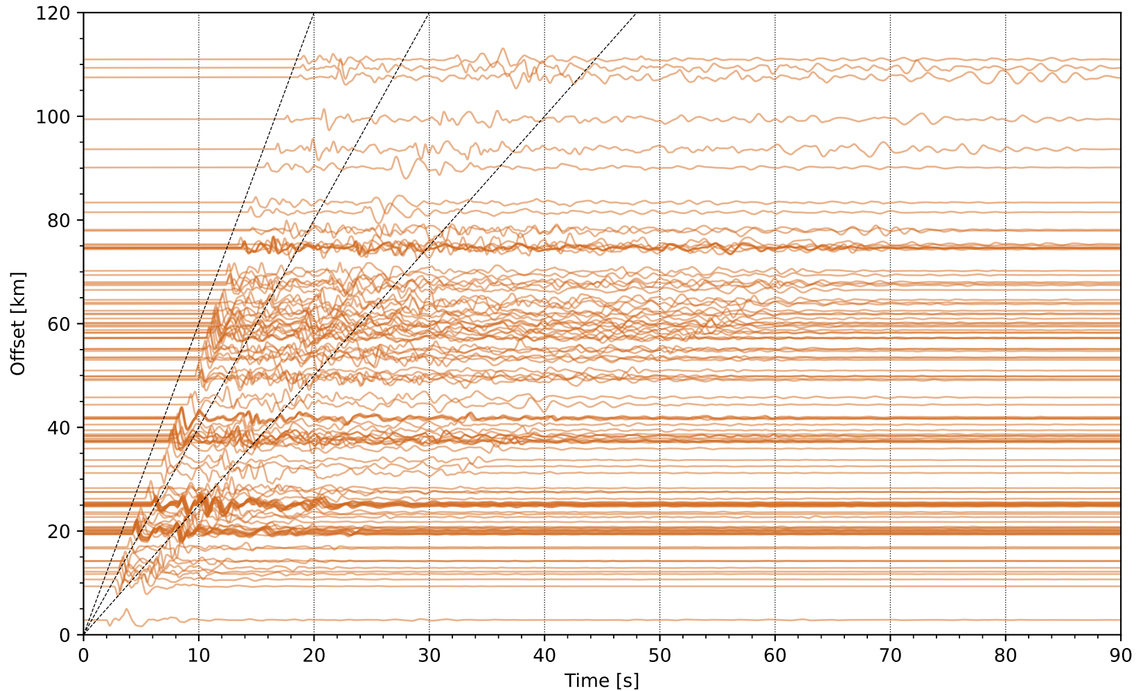
EventF uwsm1 Network: NP [HSZ] - (112 traces / 2010-01-07T18:09:35.28)
