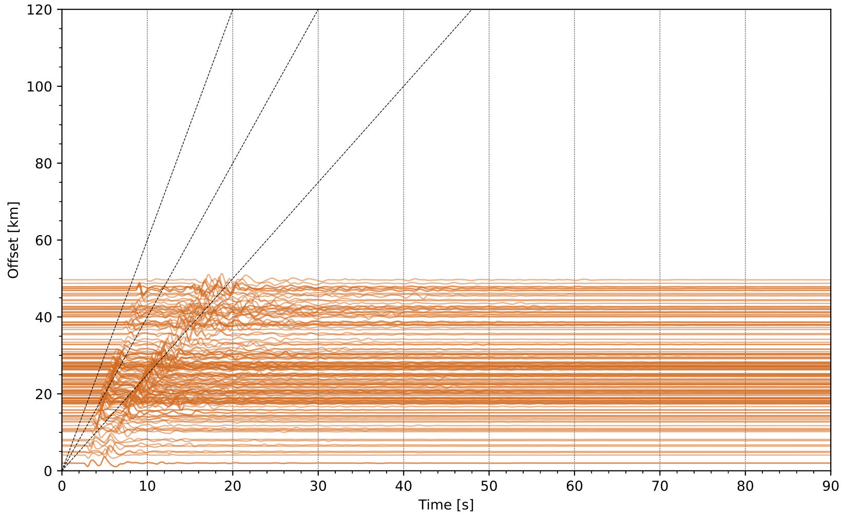
EventT uwsm1 Network: NP [HSZ] - (148 traces / 2019-10-15T05:33:42.12)
