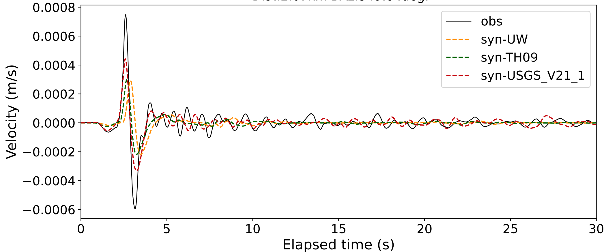
EventQ BK.BRK (0.16-0.5Hz; Component R) Dist:2.07km BAz:349.84deg.
