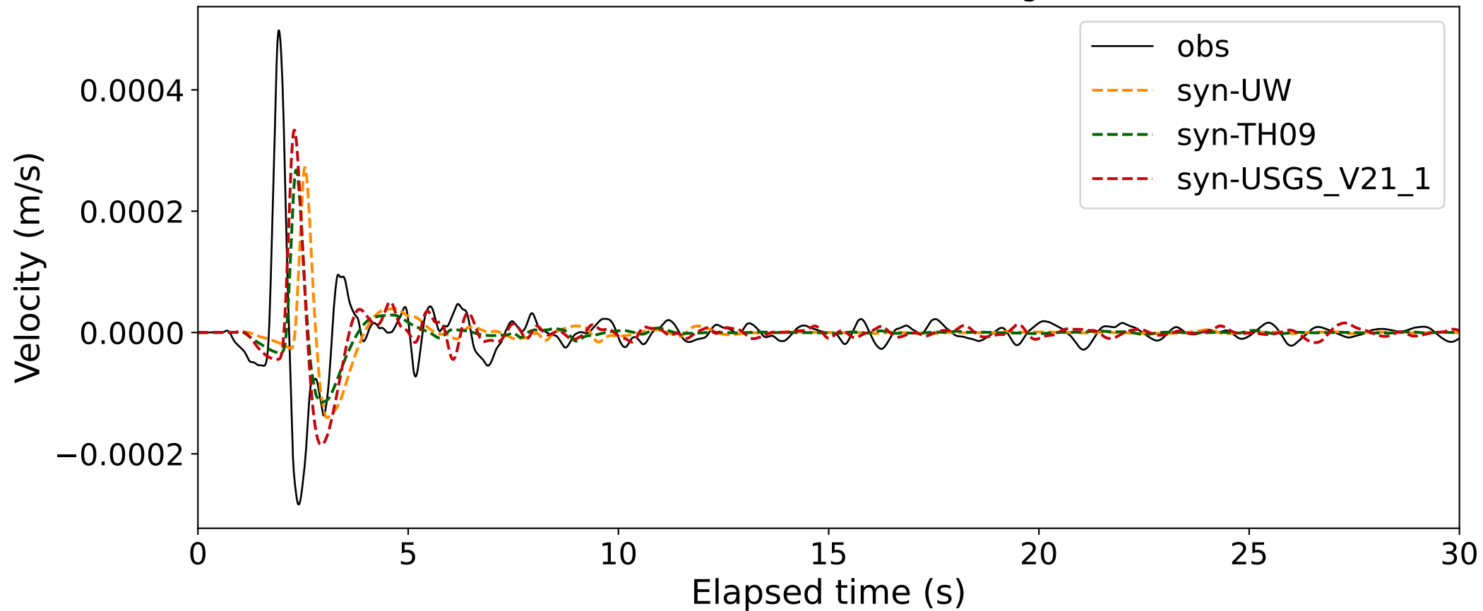
EventH BK.BRK (0.16-0.5Hz; Component R) Dist:1.48km BAz:316.76deg.
