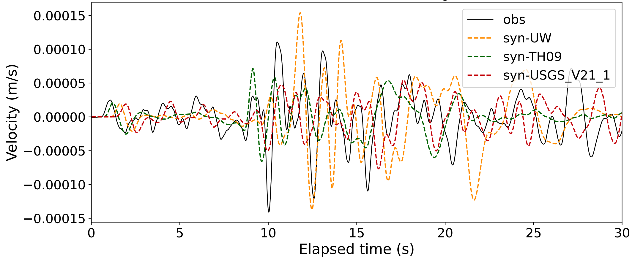
EventB BK.BRK (0.16-0.5Hz; Component R) Dist:61.51km BAz:152.05deg.
