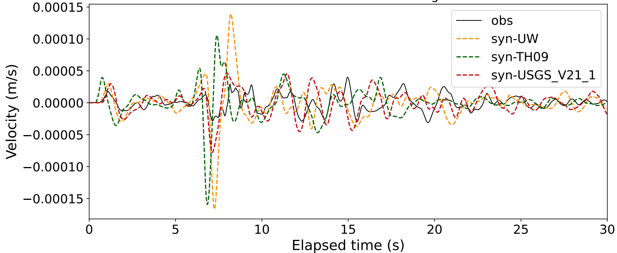
EventS BK.BRK (0.16-0.5Hz; Component R) Dist:44.79km BAz:277.97deg.
