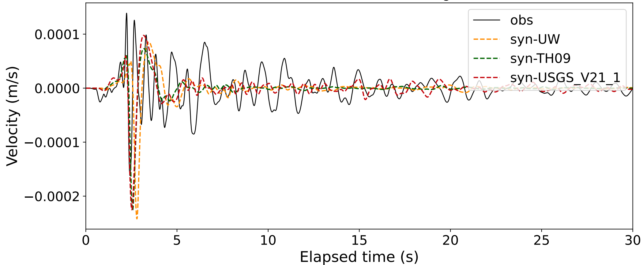
EventK BK.BRK (0.16-0.5Hz; Component R) Dist:7.34km BAz:143.73deg.
