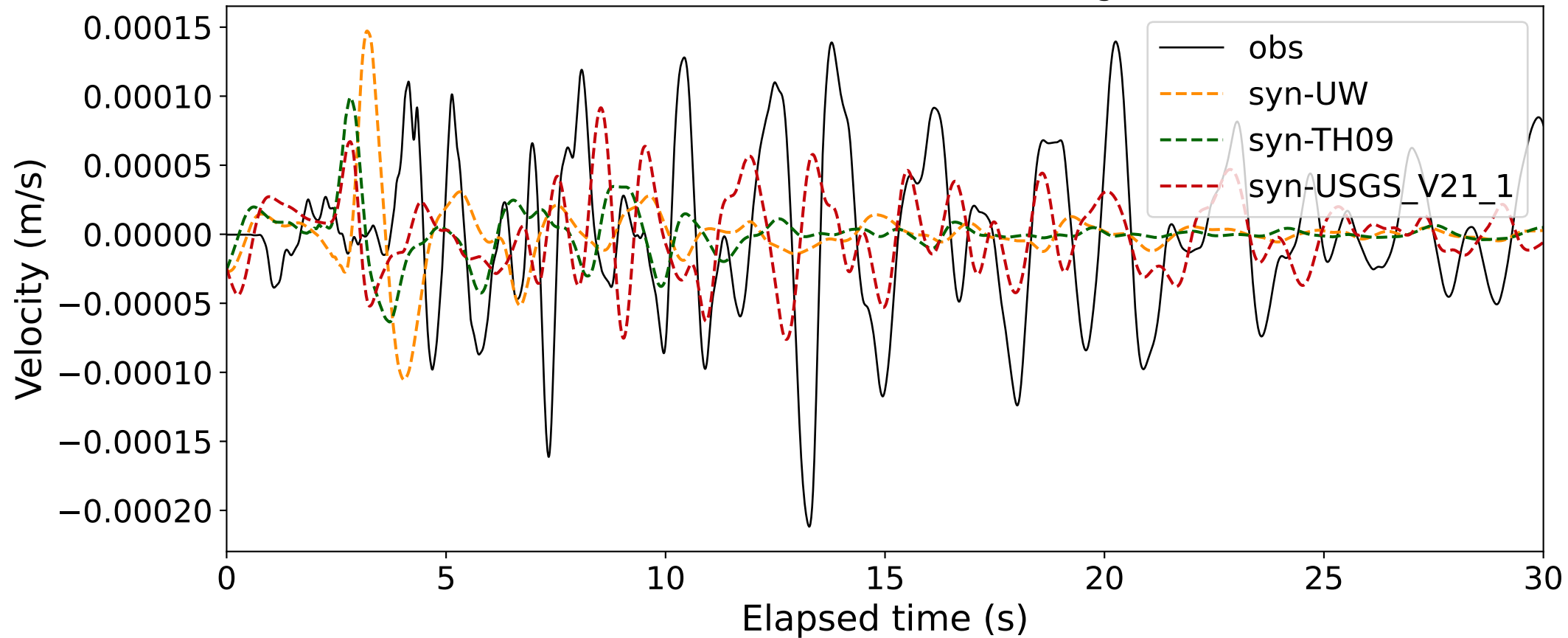
EventT BK.BRK (0.16-0.5Hz; Component R) Dist:19.31km BAz:248.31deg.
