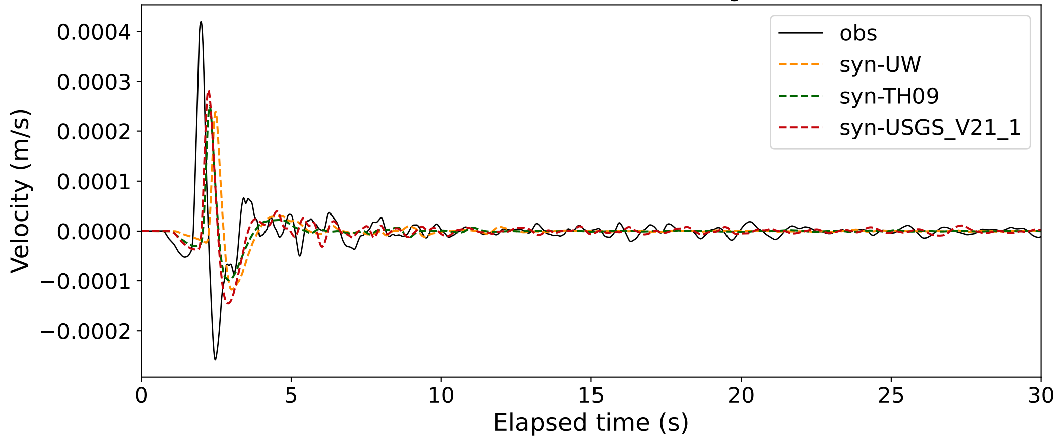
Event1 BK.BRK (0.16-0.5Hz; Component R) Dist:0.97km BAz:303.77deg.
