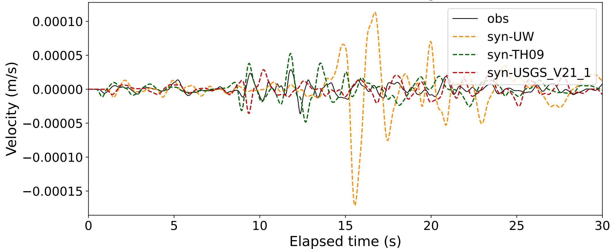
EventM BK.BRK (0.16-0.5Hz; Component R) Dist:61.96km BAz:180.87deg.
