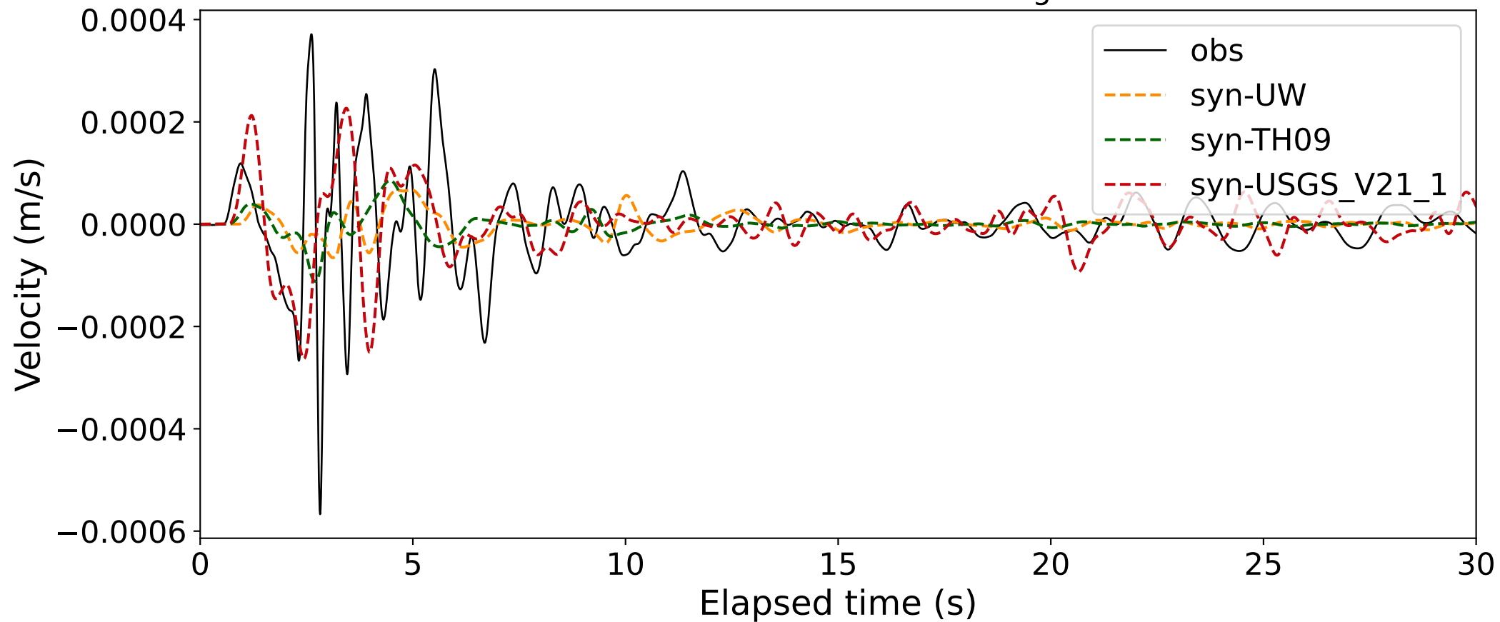
EventD BK.BRK (0.16-0.5Hz; Component R) Dist:9.76km BAz:322.22deg.
