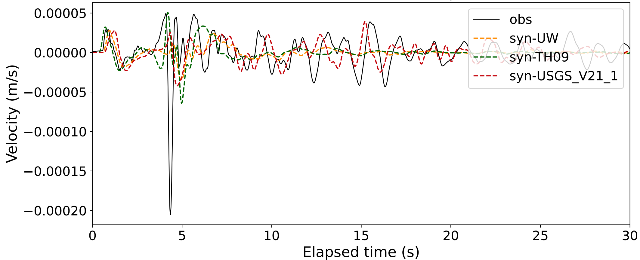
EventE BK.BRK (0.16-0.5Hz; Component R) Dist:22.79km BAz:273.25deg.
