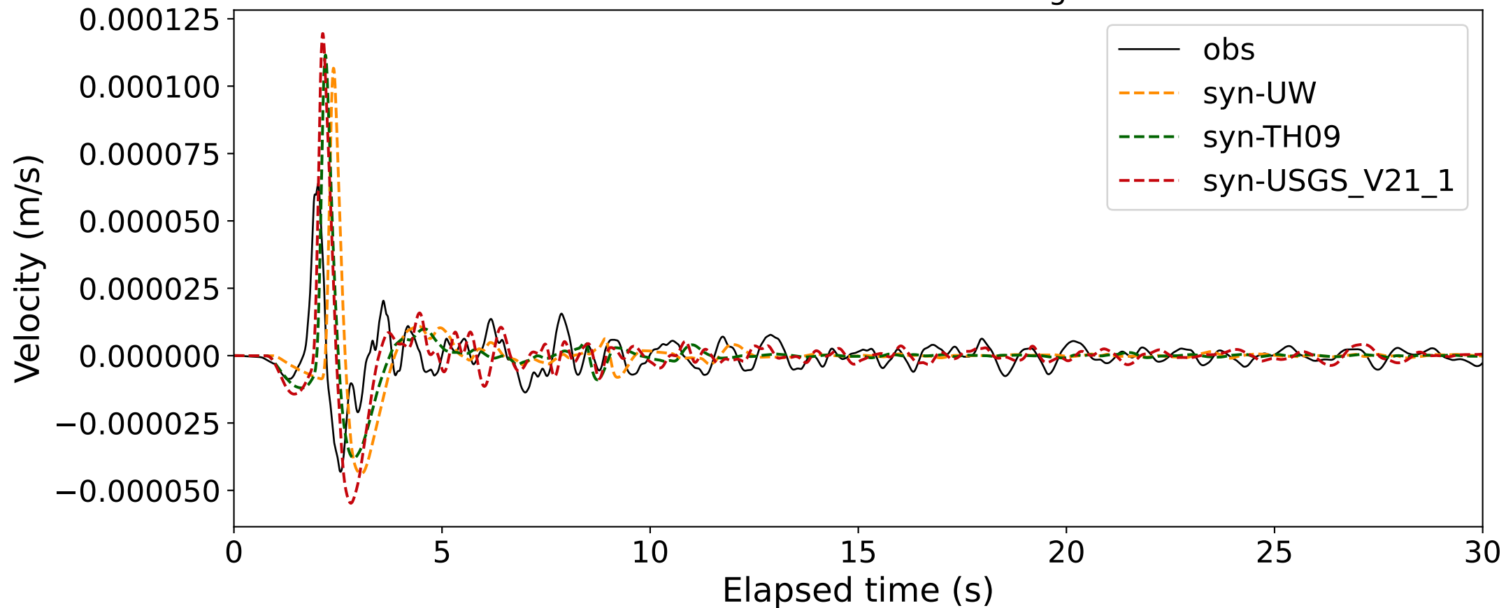
Eventj BK.BRK (0.16-0.5Hz; Component R) Dist:0.85km BAz:276.38deg.
