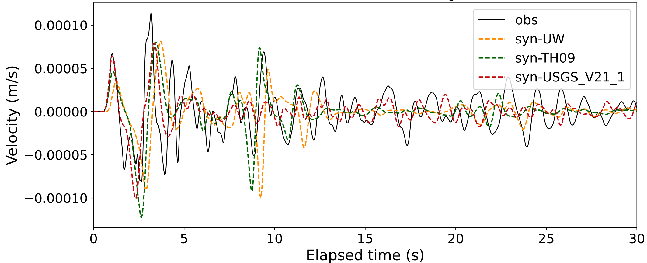
EventQ BK.BRK (0.16-0.5Hz; Component Z) Dist:2.07km BAz:349.84deg.
