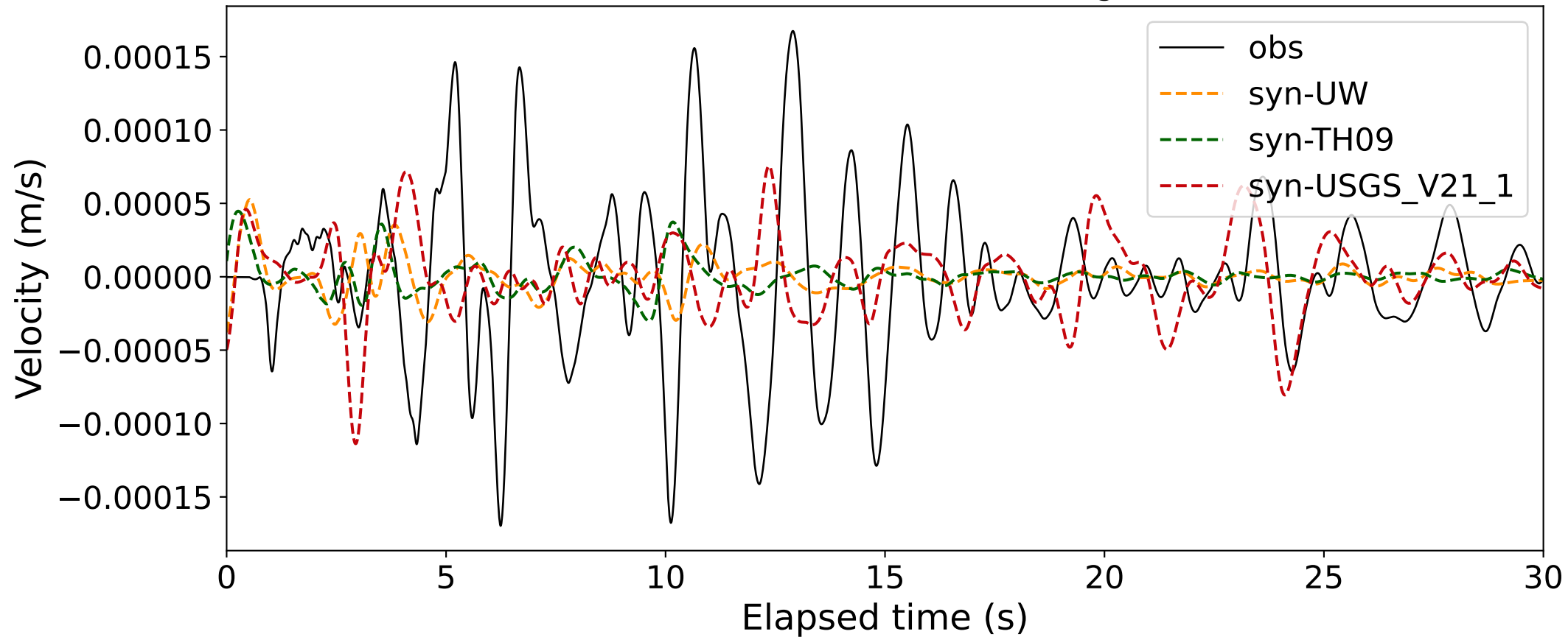
EventT BK.BRK (0.16-0.5Hz; Component Z) Dist:19.31km BAz:248.31deg.
