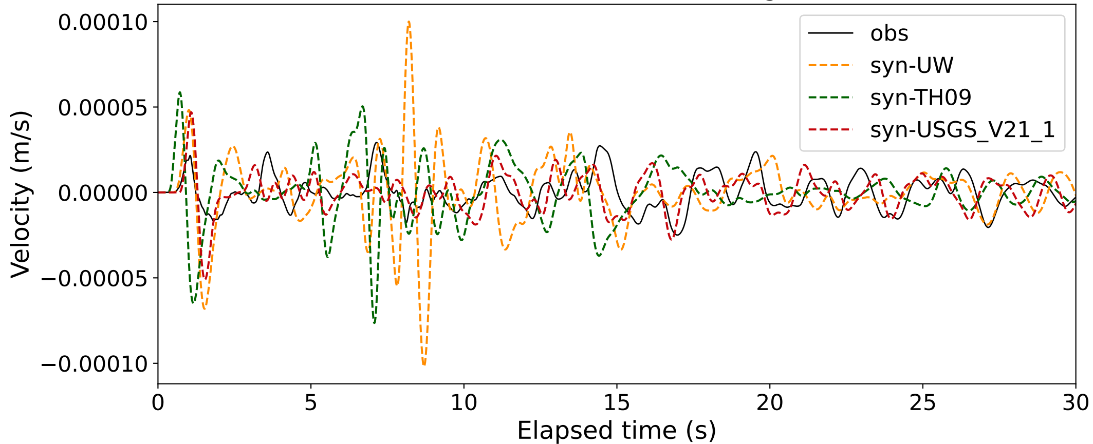
EventS BK.BRK (0.16-0.5Hz; Component Z) Dist:44.79km BAz:277.97deg.
