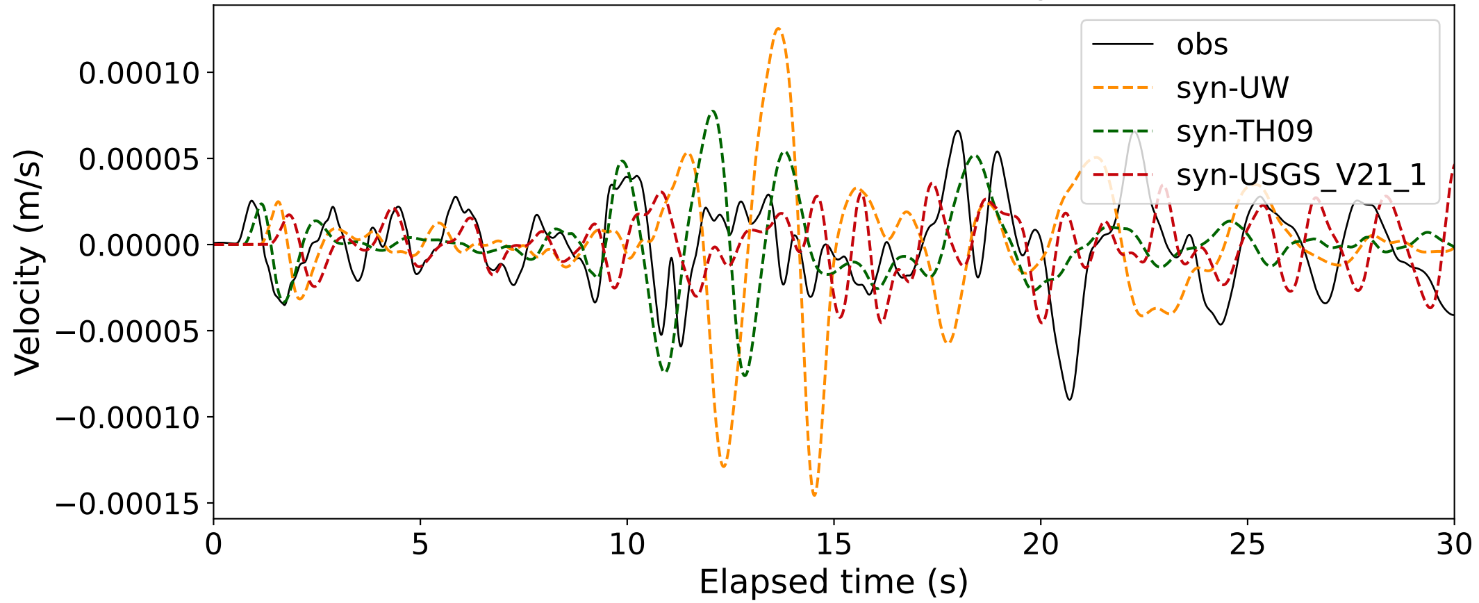
EventB BK.BRK (0.16-0.5Hz; Component Z) Dist:61.51km BAz:152.05deg.
