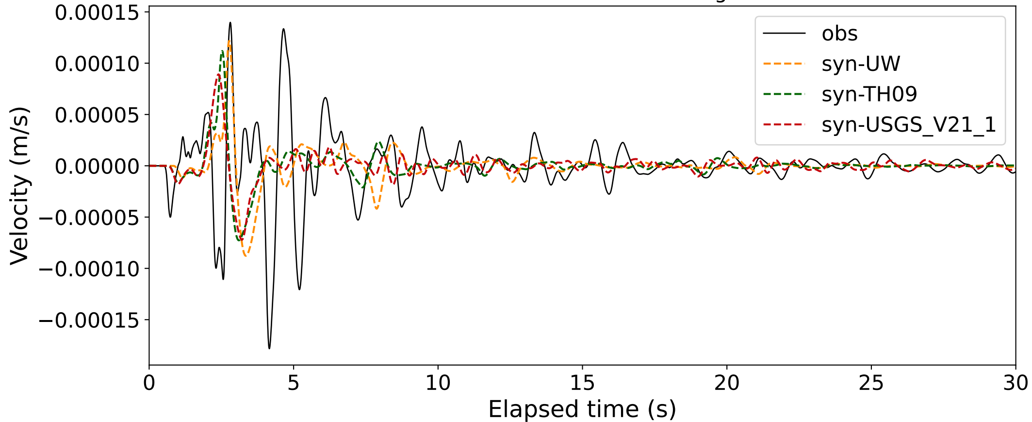
EventK BK.BRK (0.16-0.5Hz; Component Z) Dist:7.34km BAz:143.73deg.
