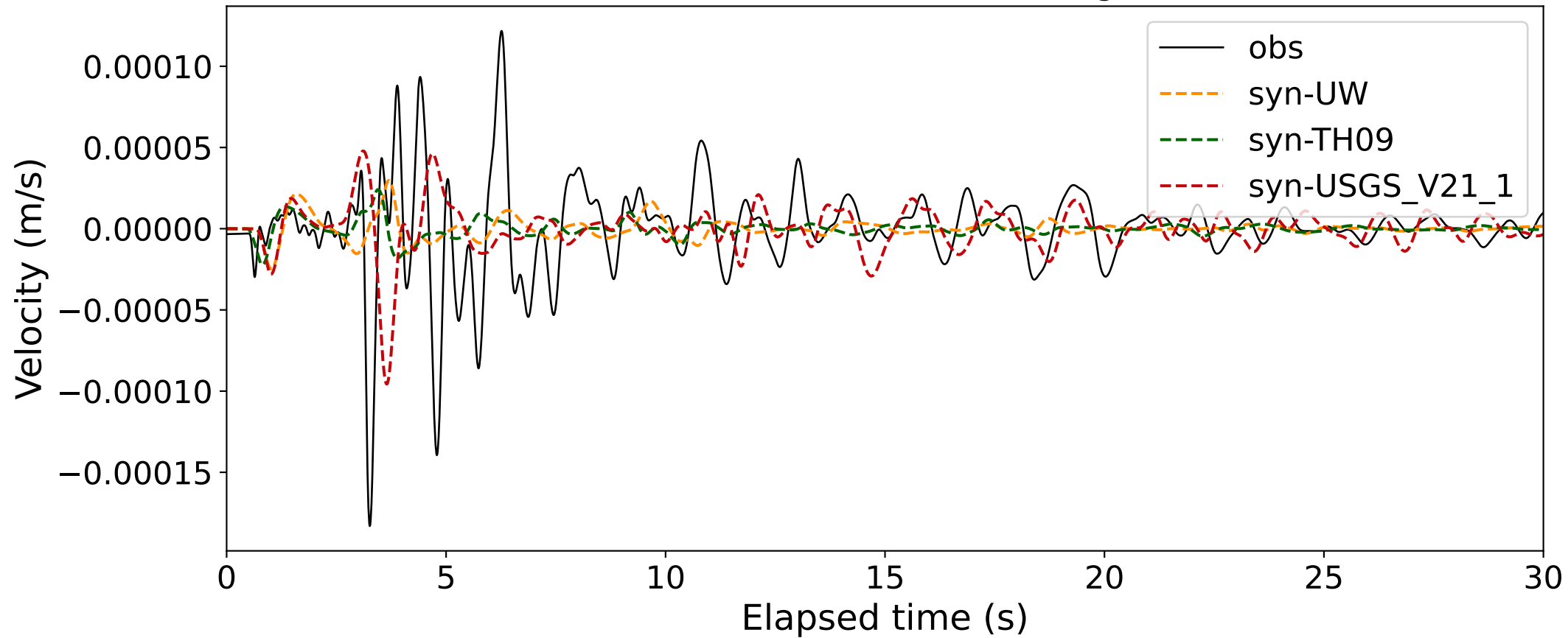
EventC BK.BRK (0.16-0.5Hz; Component Z) Dist:13.41km BAz:259.08deg.
