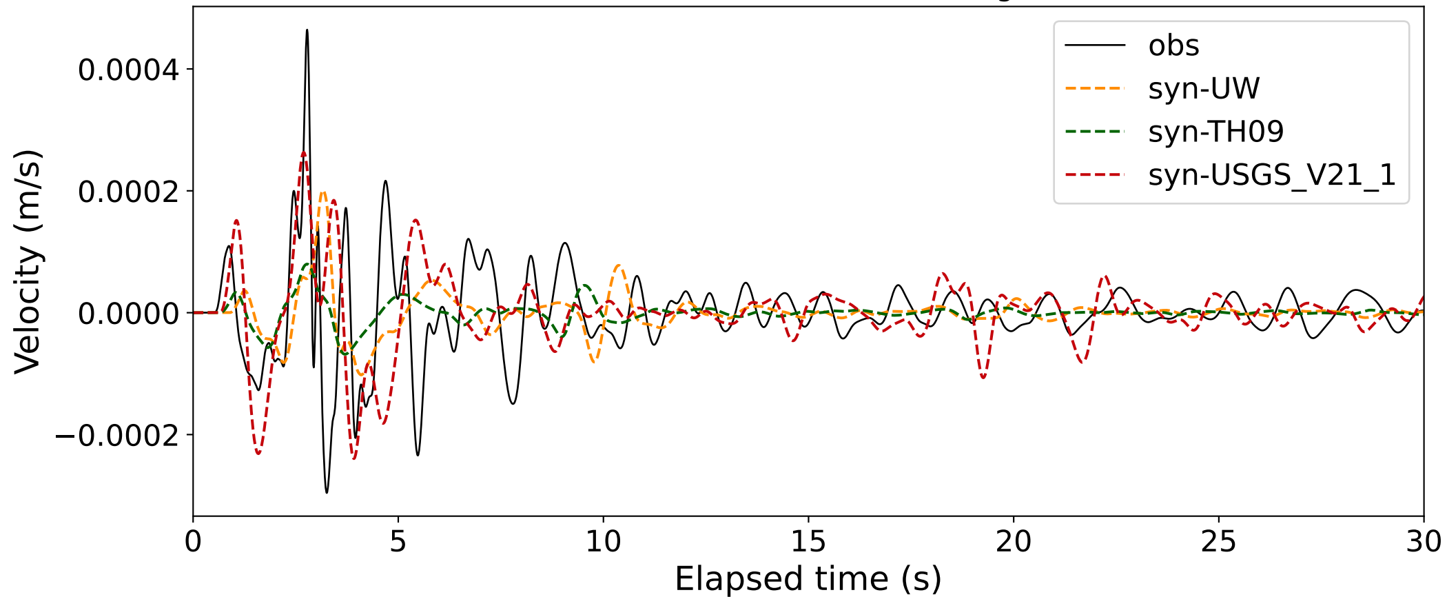
EventD BK.BRK (0.16-0.5Hz; Component Z) Dist:9.76km BAz:322.22deg.
