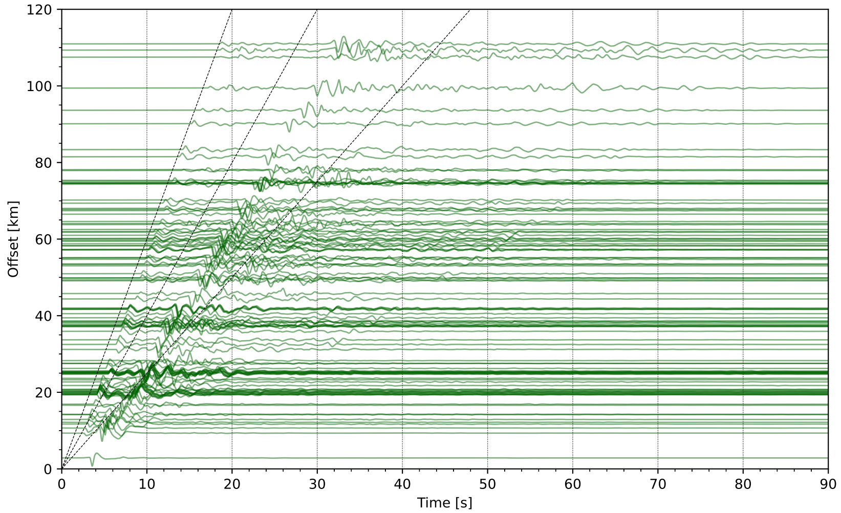
EventF th09sm1 Network: NP [HSR] - (112 traces / 2010-01-07T18:09:35.28)
